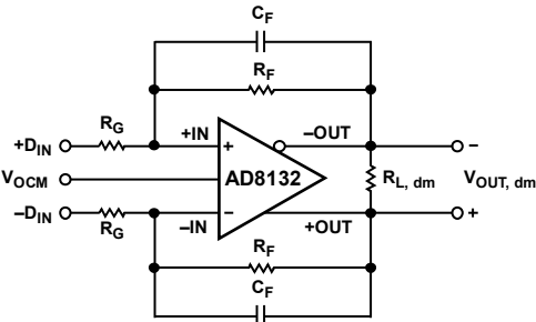
Figure 64. Circuit Definitions
