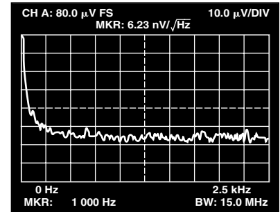
TPC 27. Voltage Noise Density vs. Frequency V_S = \pm 15\text{ V}
