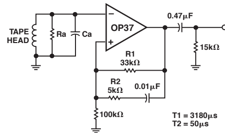
Figure 9. Tape-Head Preamplifier
