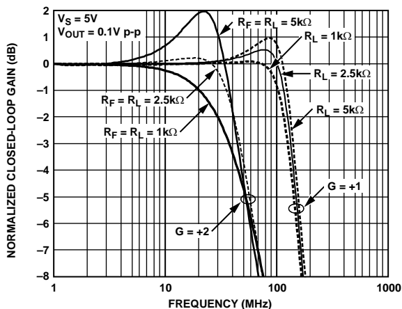
Figure 55. Frequency Response for Various Feedback/Load Resistances
