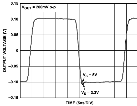
Figure 17. Small Signal Transient Response vs. Supply Voltage
