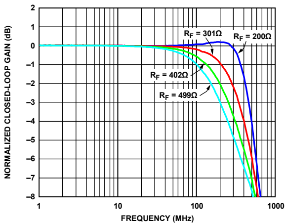
Figure 6. Small Signal Frequency Response vs. Feedback Resistor
