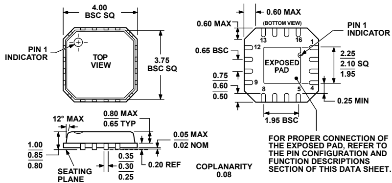
Figure 45.16-Lead Frame Chip Scale Package [LFCSP_VQ] 4 mm × 4 mm Body, Very Thin Quad (CP-16-4) Dimensions shown in millimeters
