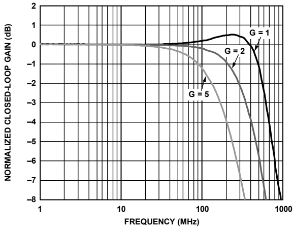
Figure 4. Small Signal Frequency Response vs. Gain
