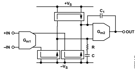
Figure 46. High Level Design Schematic
