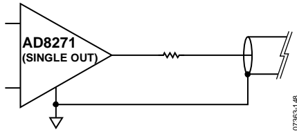
Figure 55. Driving Cabling
