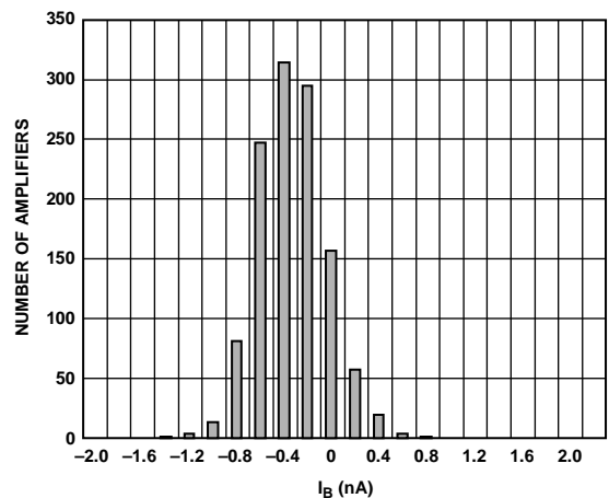
Figure 8. Input Bias Current, V S = ±5 V
