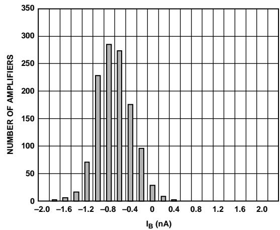
Figure 7. Input Bias Current, V S = ±15 V
