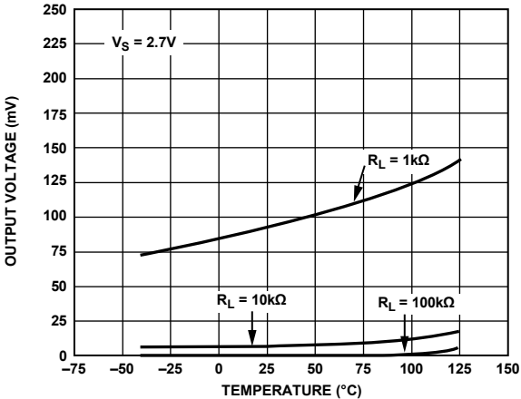
Figure 48. Output Voltage to Supply Rail vs. Temperature
