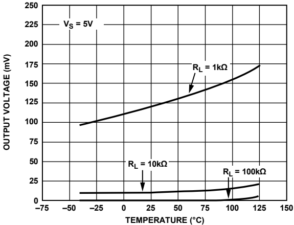
Figure 49. Output Voltage to Supply Rail vs. Temperature
