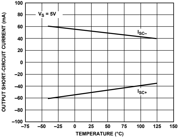
Figure 47. Output Short-Circuit Current vs. Temperature
