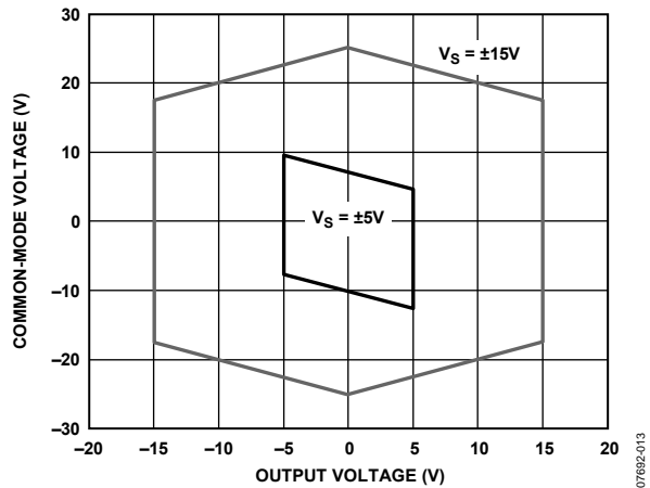
Figure 13. Input Common-Mode Voltage vs. Output Voltage, \pm 15\text{ V} and \pm 5\text{ V} Supplies
