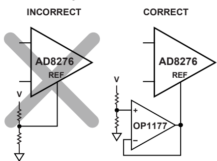
Figure 37. Driving the Reference Pin
