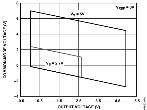
Figure 15. Input Common-Mode Voltage vs. Output Voltage, 5 V and 2.7 V Supplies, V_{REF} = 0\text{ V}
