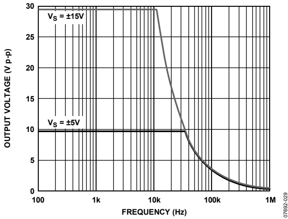
Figure 29. Maximum Output Voltage vs. Frequency, V_S = \pm 15\text{ V}, \pm 5\text{ V}
