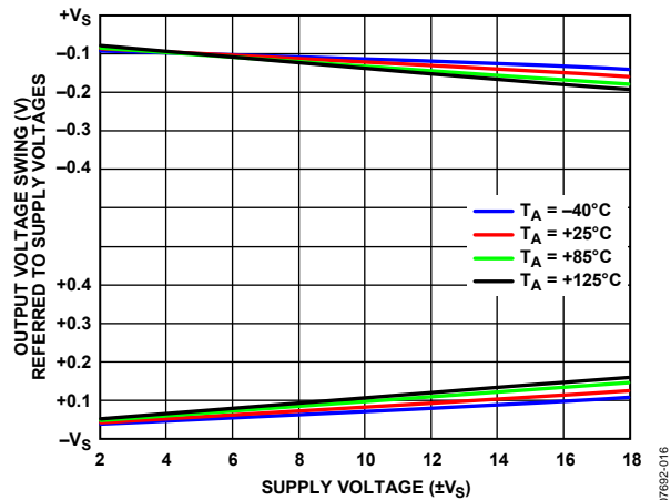
Figure 16. Output Voltage Swing vs. Supply Voltage and Temperature, R_L = 10\text{ k}\Omega
