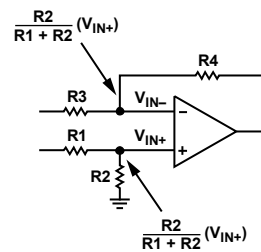
Figure 36. Voltage Division in the Difference Amplifier Configuration
