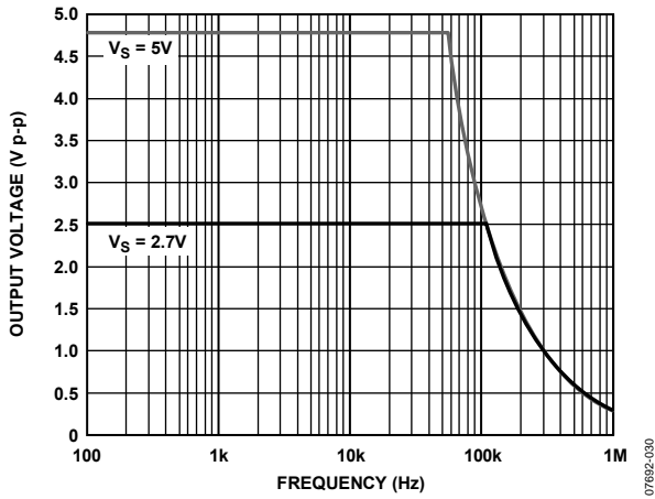
Figure 30. Maximum Output Voltage vs. Frequency, V_S = 5\text{ V}, 2.7\text{ V}
