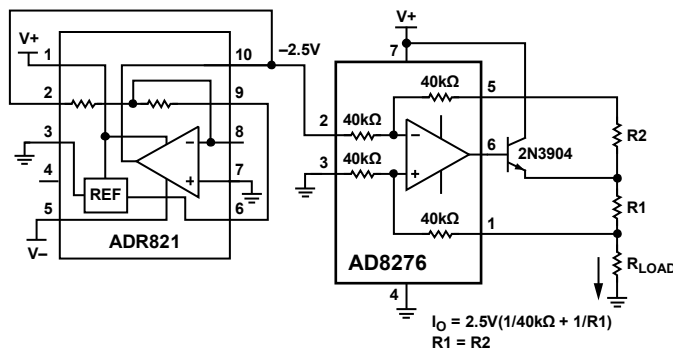
Figure 45. Constant Current Source
