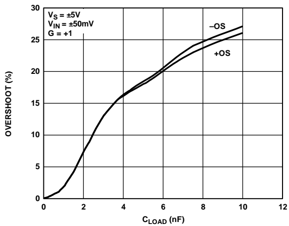
Figure 26. Overshoot vs. Capacitive Load
