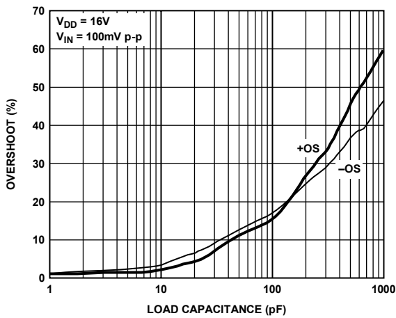
Figure 21. Small-Signal Overshoot vs. Load Capacitance
