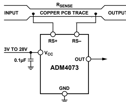
Figure 26. Using PCB Trace for Current Sensing
