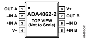
Figure 1. 8-Lead Narrow-Body SOIC and 8-Lead MSOP
