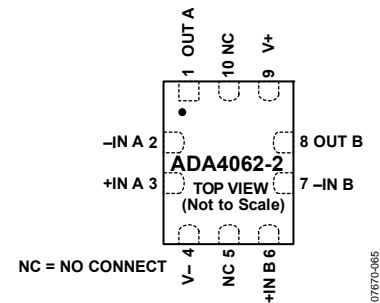
Figure 2. 10-Lead LFCSP
