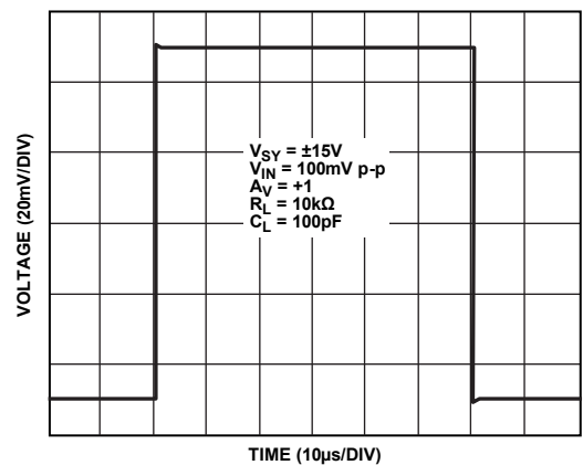
Figure 39. Small-Signal Transient Response
