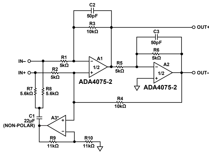
*A3 REDUCES THE DEGRADATION OF CMRR (SEE THE BALANCED LINE RECEIVER SECTION FOR MORE DETAILS).
