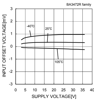
Fig.57 Input Offset Voltage - Supply Voltage
