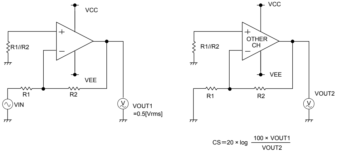
Fig.97 Test circuit 3
