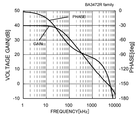
Fig.67 Voltage Gain - Frequency ( V_{CC}/V_{EE}=7.5[V]/-7.5[V] , A_v=40[dB] , R_L=2[k\Omega] , C_L=100[pF] , T_a=25[^\circ C] )
