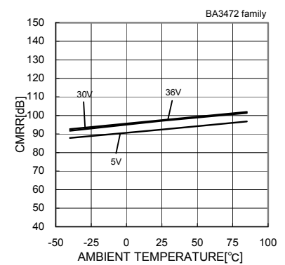
Fig.18 Common Mode Rejection Ratio -Ambient Temperature
