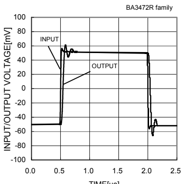
Fig.69 Input / Output Voltage - Time ( V_{CC}/V_{EE}=15[V]/-15[V] , A_v=0[dB] , R_L=2[k\Omega] , C_L=100[pF] , T_a=25[^\circ C] )
