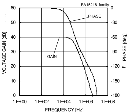
Fig. 220 Voltage Gain - Frequency (V CC /V EE =+15[V]/-15[V], A v =40[dB], R L =2[kΩ], T a =25[°C])
