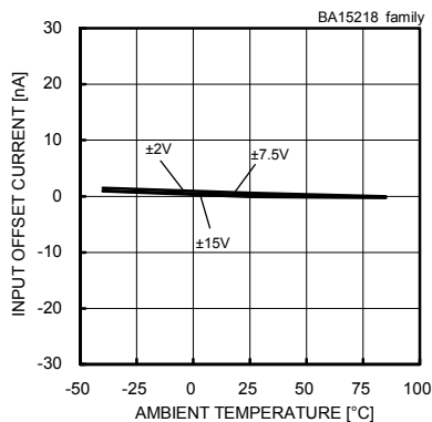
Fig. 212 Input Offset Current - Ambient Temperature (V icm =0[V], V out =0[V])
