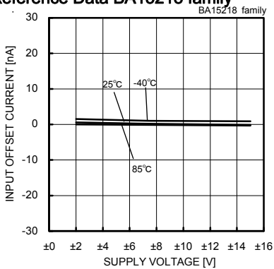
Fig. 211 Input Offset Current - Supply Voltage (V icm =0[V], V out =0[V])
