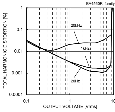
Fig. 86 Total Harmonic Distortion - Output Voltage (VCC/VEE=+15[V]/-15[V], Av=20[dB], RL=2[kΩ], 80[kHz]-LPF, Ta=25[°C])
