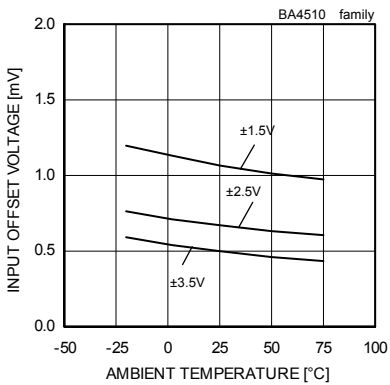
Fig. 274 Input Offset Voltage - Ambient Temperature (Vcm=0[V], Vout=0[V])
