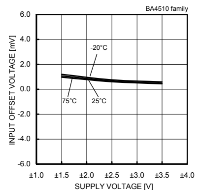
Fig. 273 Input Offset Voltage - Supply Voltage (Vcm=0[V], Vout=0[V])
