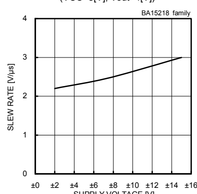
Fig. 216 Slew Rate - Supply Voltage (C L =100[pF], R L =2[kΩ], T a =25[°C])
