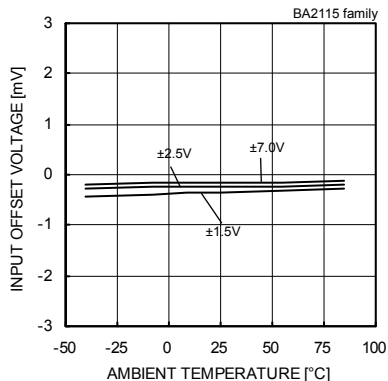
Fig. 297 Input Offset Voltage - Ambient Temperature (Vicm=0[V], Vout=0[V])
