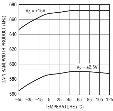
Gain Bandwidth Product vs Temperature
