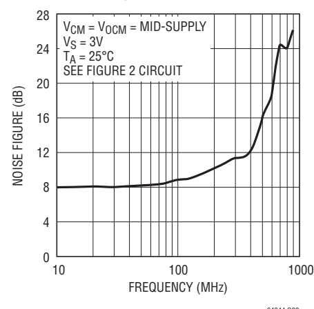
LTC6404-4 Noise Figure vs Frequency
