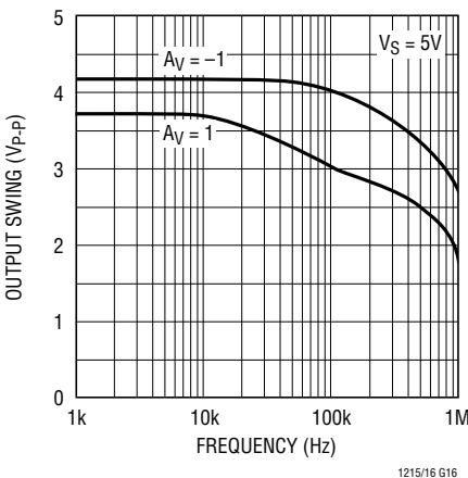
Undistorted Output Swing vs Frequency, VS = 5V
