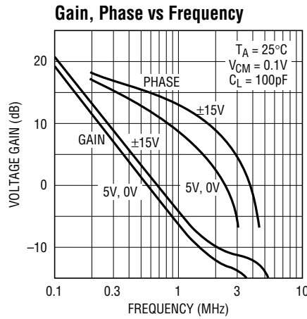
LT1413 • TA13
