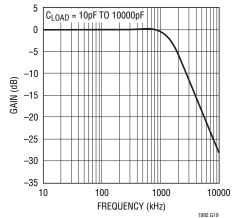
V OCM Gain vs Frequency, V S = ±2.5V
