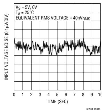
LT6013/LT6014 0.1Hz to 10Hz Voltage Noise
