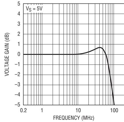
Figure 9. Video Line Driver Frequency Response
