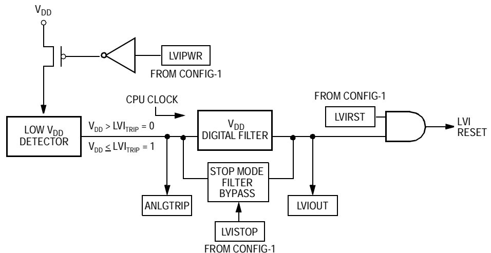
Figure 15-1. LVI Module Block Diagram
