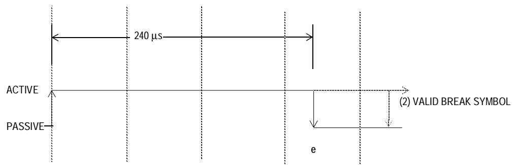
Figure 21-11. J1850 VPW Received BREAK Symbol Times
