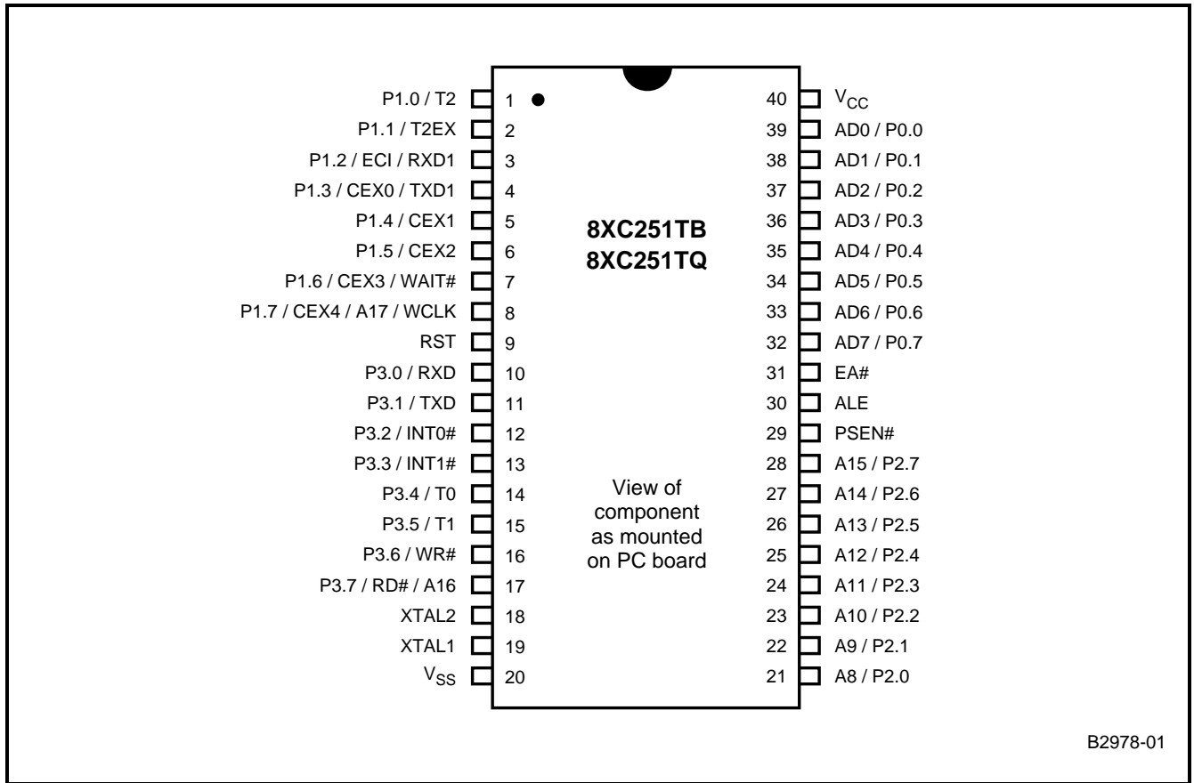
Figure 4. 8xC251TB/TQ 40-pin PDIP Packages
