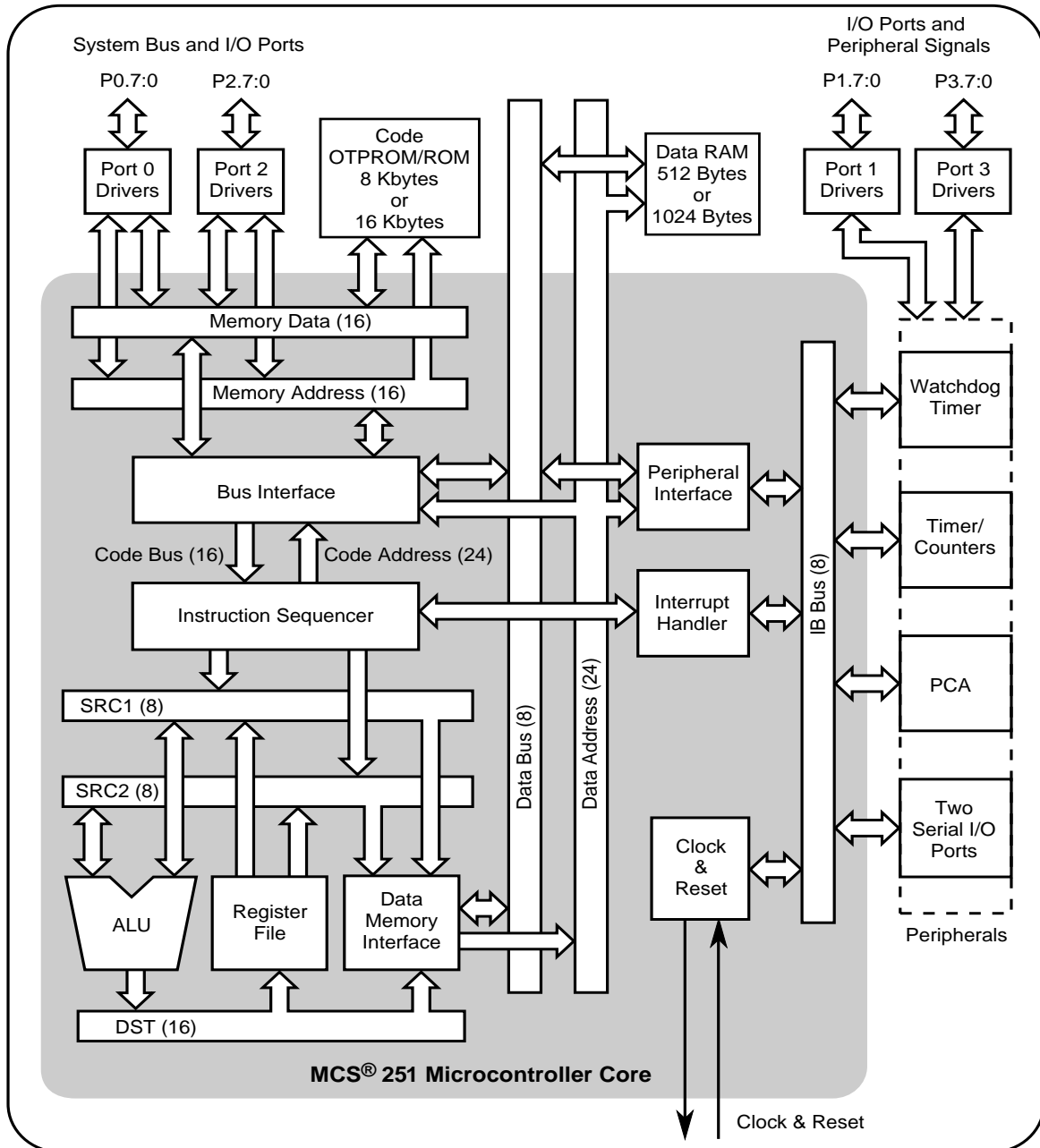
Figure 1. 8xC251TB/TQ Block Diagram
