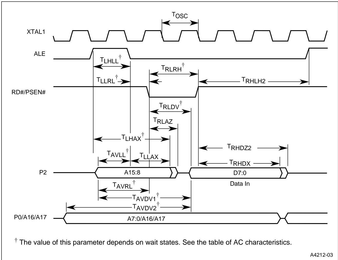
Figure 9. External Bus Cycle: Data Read (Page Mode)
