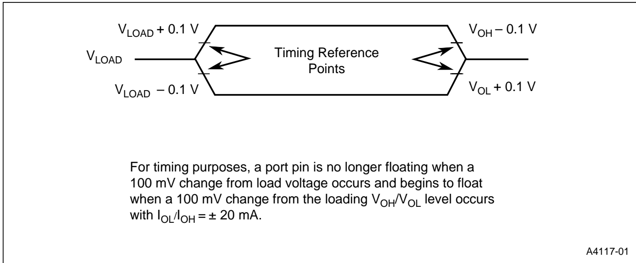
Figure 18. Float Waveforms
