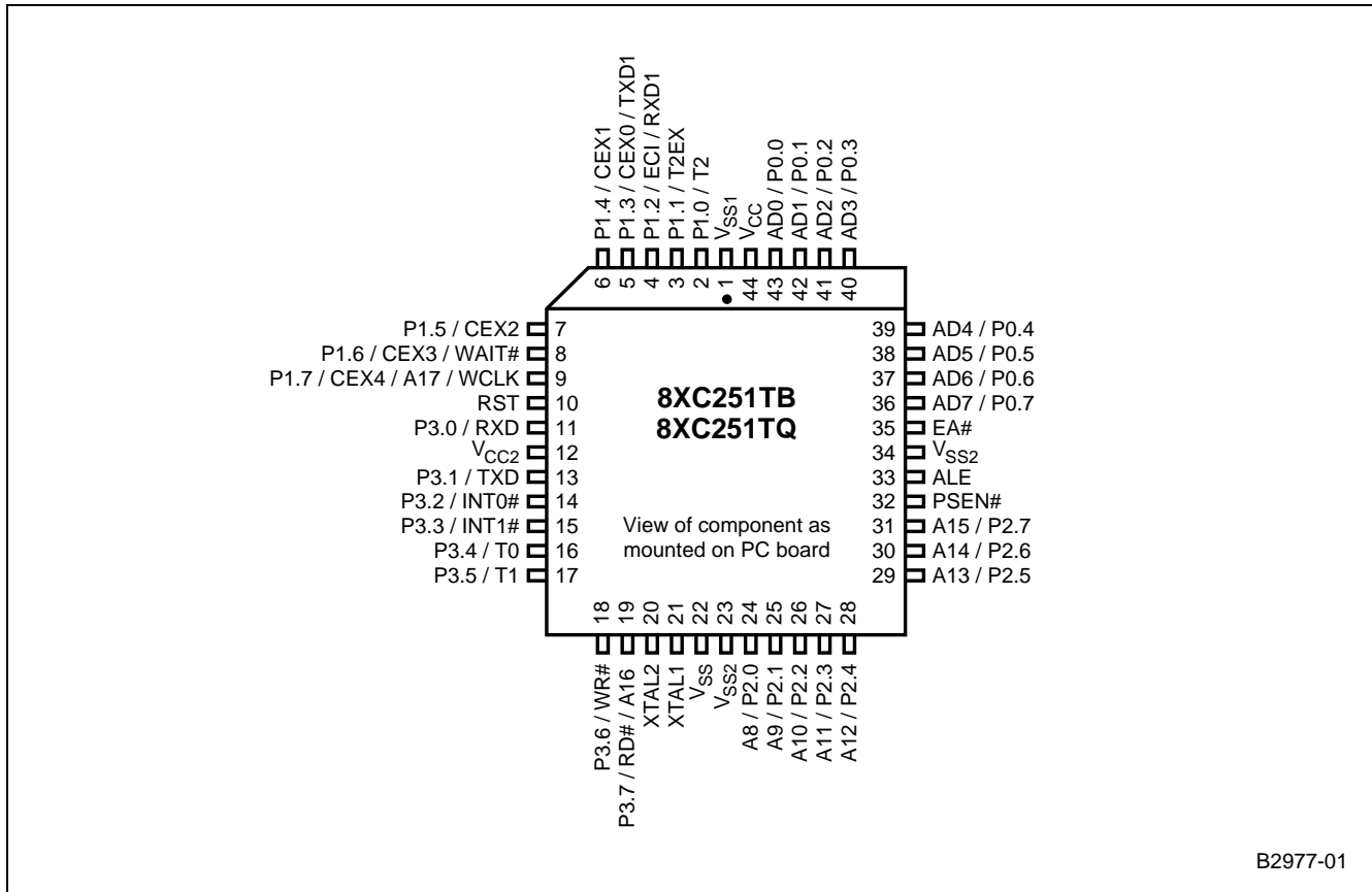
Figure 3. 8xC251TB/TQ 44-pin PLCC Package
