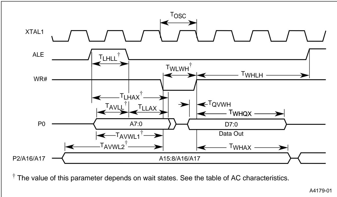
Figure 7. External Bus Cycle: Data Write (Nonpage Mode)
