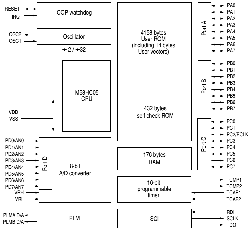
Figure A-1 MC68HC05B4 block diagram
