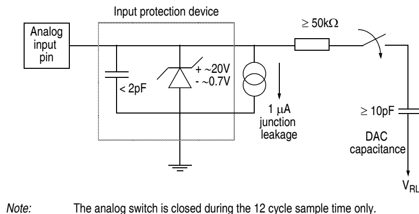
Figure 8-2 Electrical model of an A/D input pin
