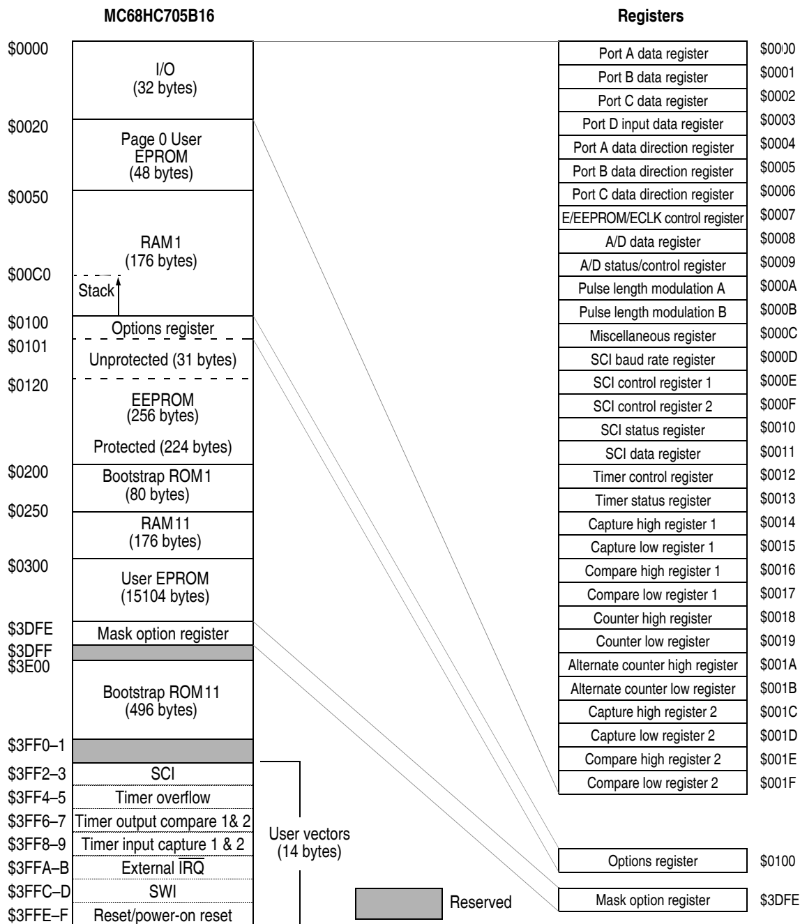
Figure E-2 Memory map of the MC68HC705B16
