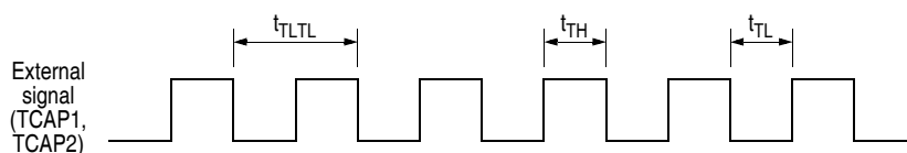
Figure H-10 Timer relationship
