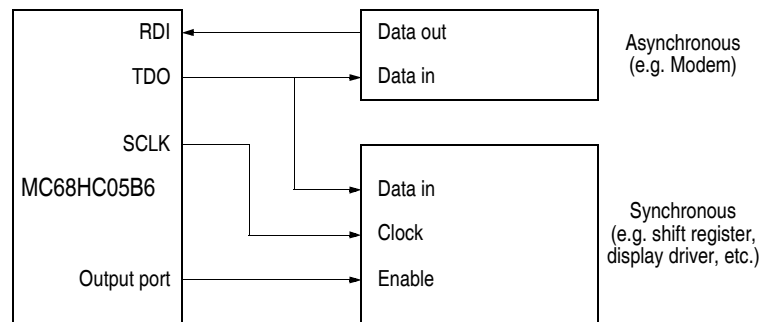
Figure 6-8 SCI example of synchronous and asynchronous transmission
