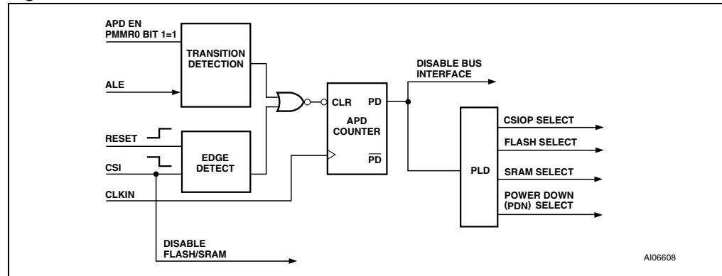
Figure 67. APD unit
