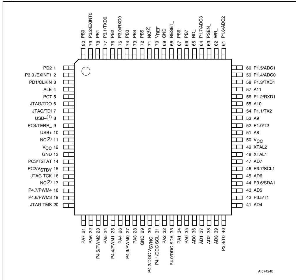
Figure 3. TQFP80 connections
