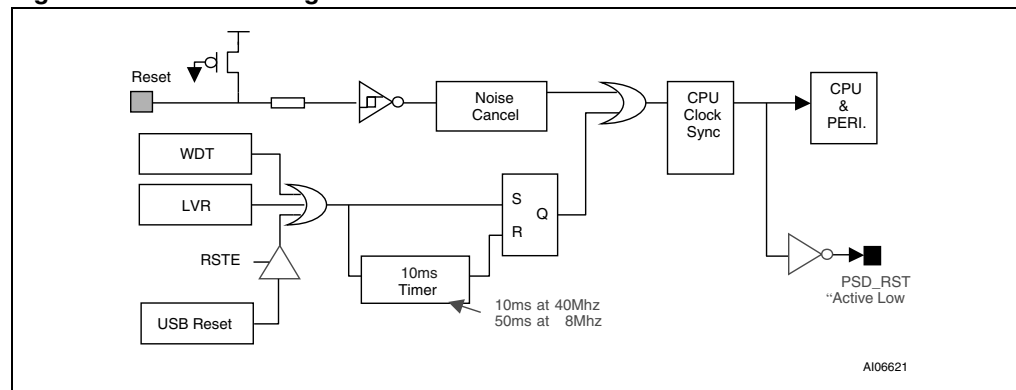
Figure 19. \overline{\text{RESET}} configuration
