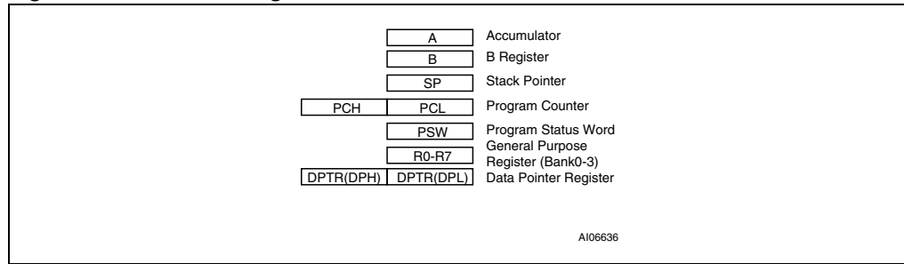
Figure 5. 8032 MCU registers
