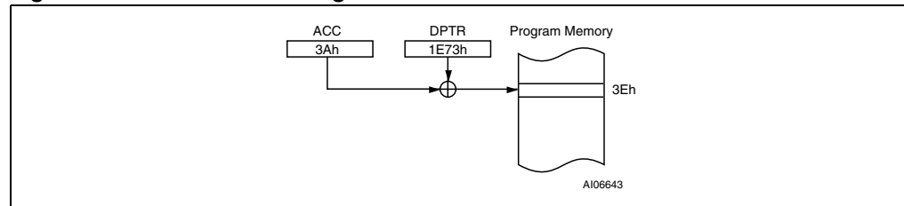
Figure 12. Indexed addressing
