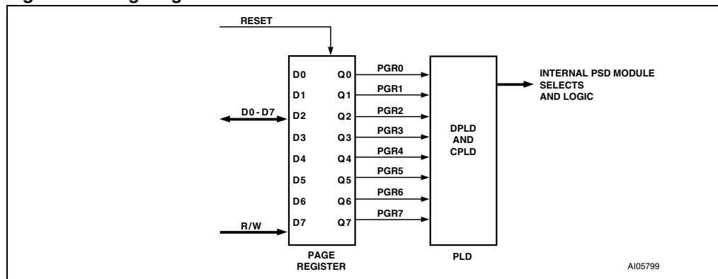
Figure 56. Page register
