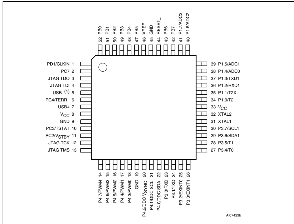
Figure 2. TQFP52 connections
