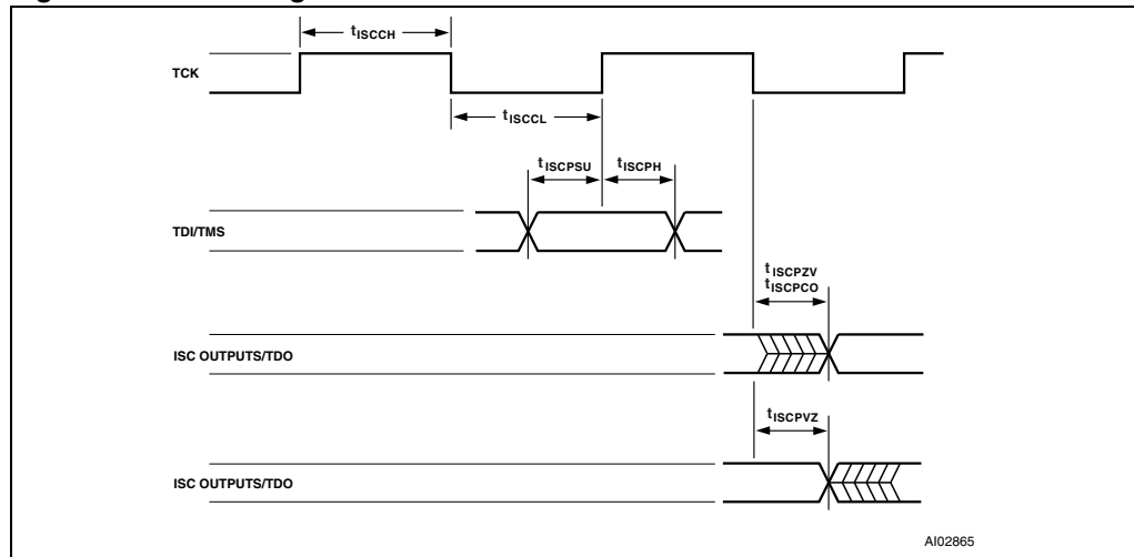
Figure 84. ISC timing
