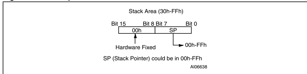
Figure 7. Stack pointer
