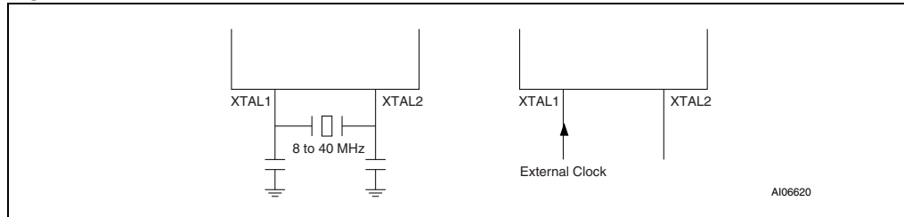
Figure 18. Oscillator
