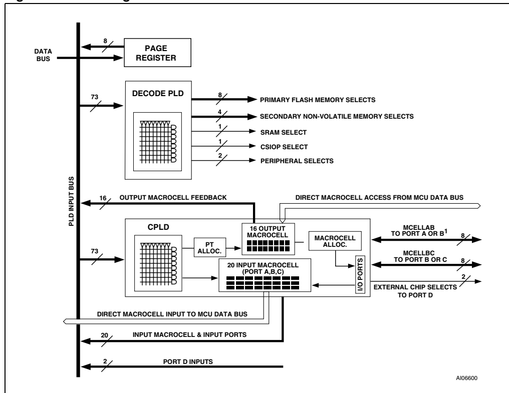
Figure 57. PLD diagram
