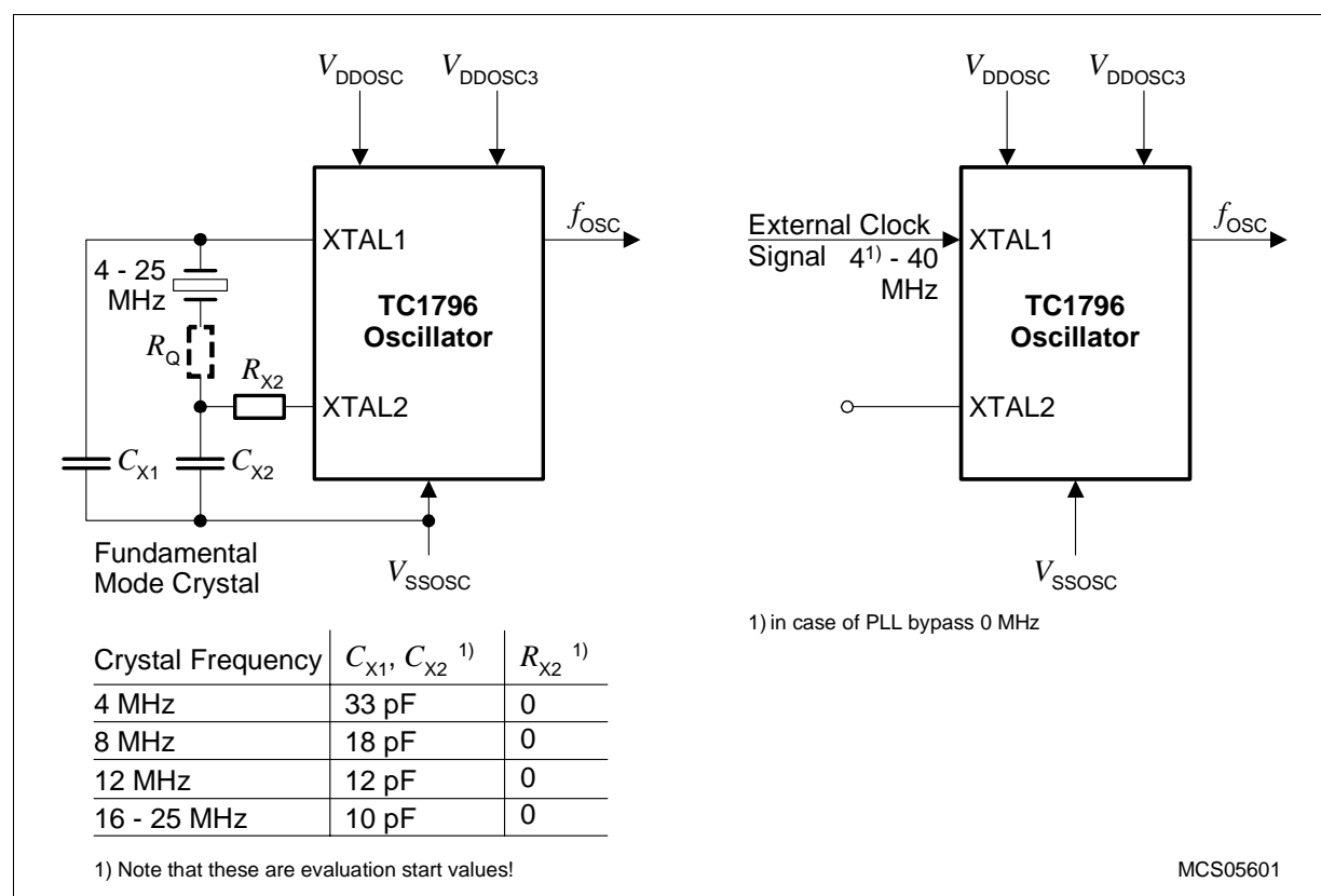
Figure 20 Oscillator Circuitries
