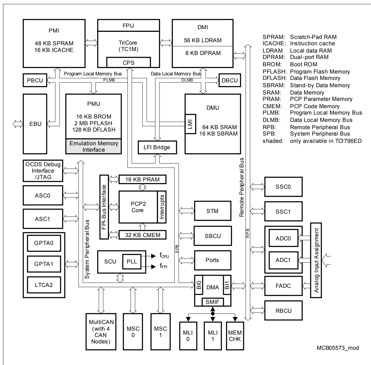
Figure 1 TC1796 Block Diagram
