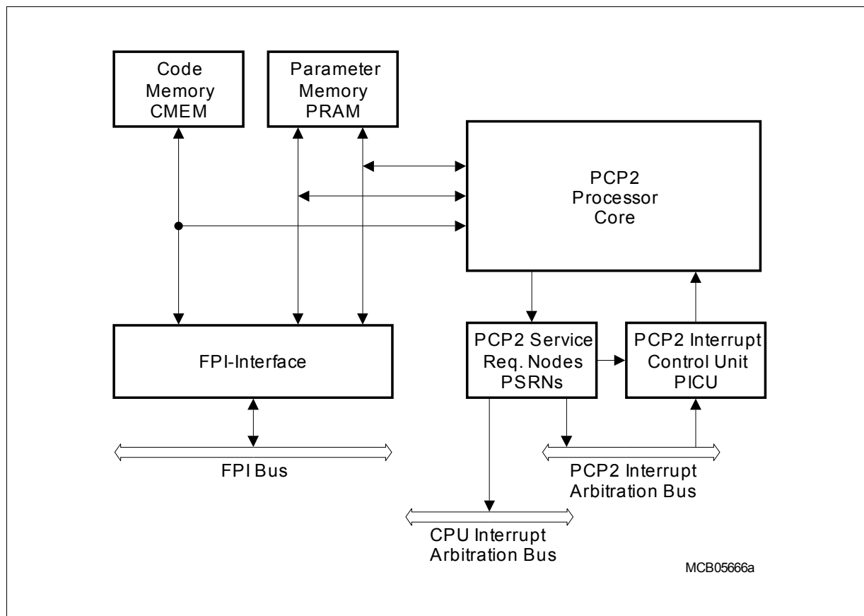
Figure 5 PCP2 Block Diagram
