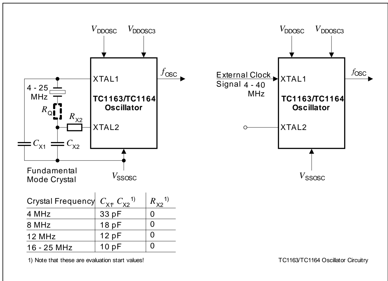
Figure 3-16 Oscillator Circuitries
