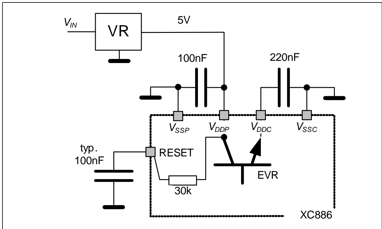
Figure 21 Reset Circuitry
