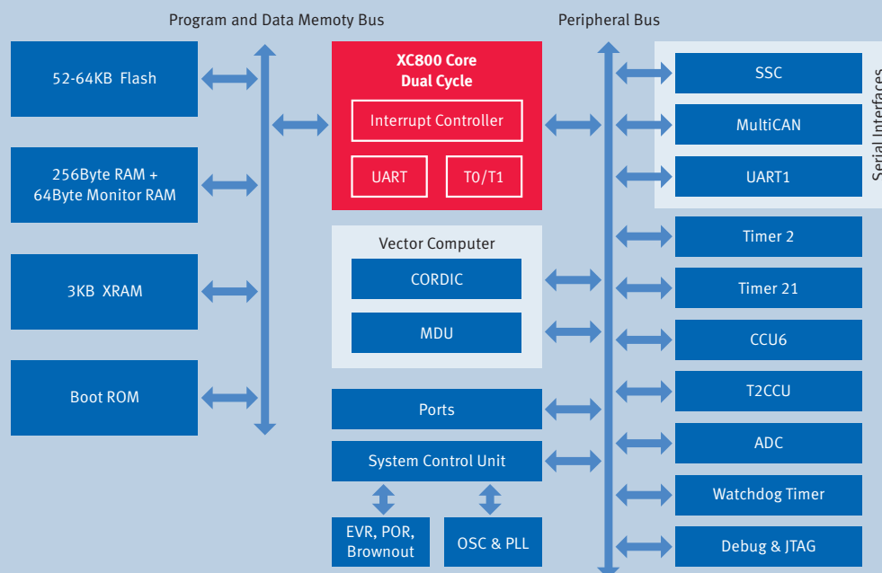
XC87x-Series Block Diagram
