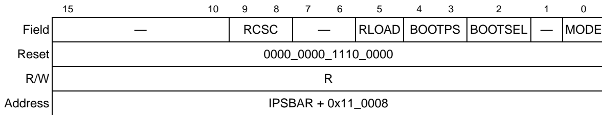
Figure 27-3. Reset Configuration Register (RCON)
