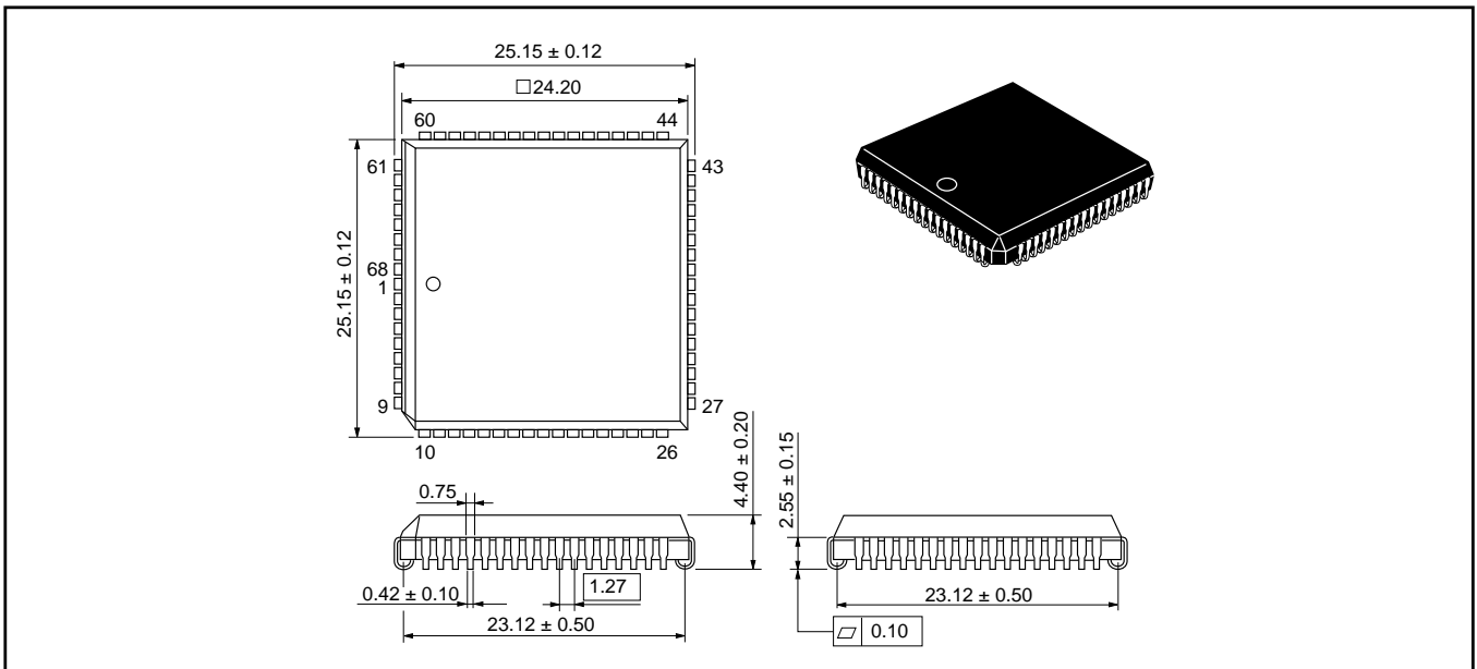
Figure E-4. Package Dimensions (CP-68)
