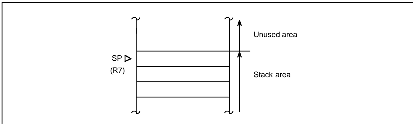
Figure 3-2. Stack Pointer
