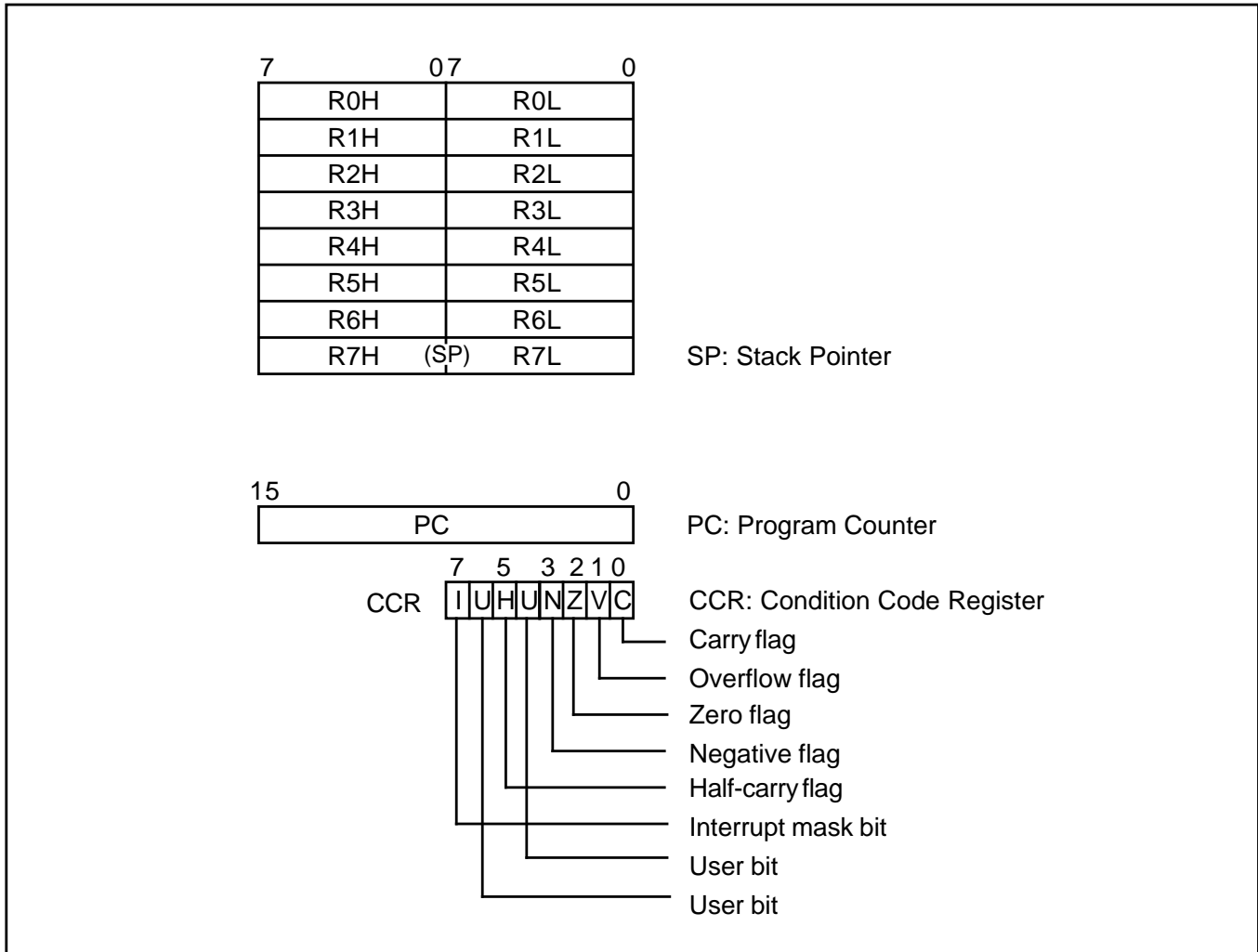
Figure 3-1. CPU Registers
