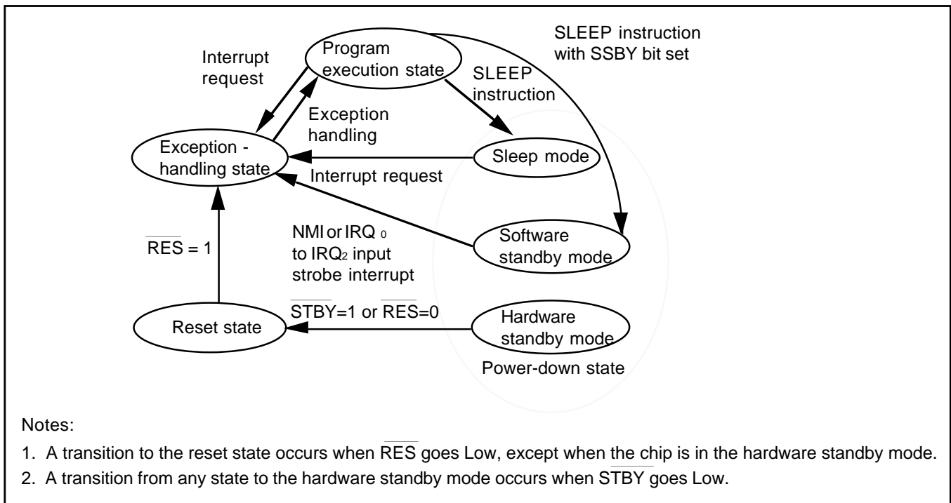
Figure 3-12. State Transitions
