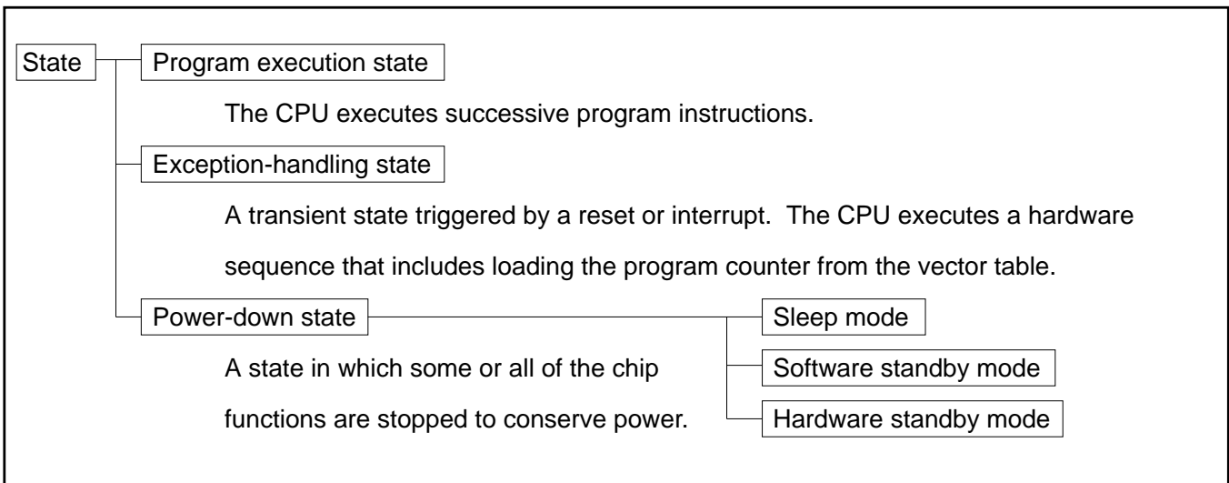
Figure 3-11. Operating States
