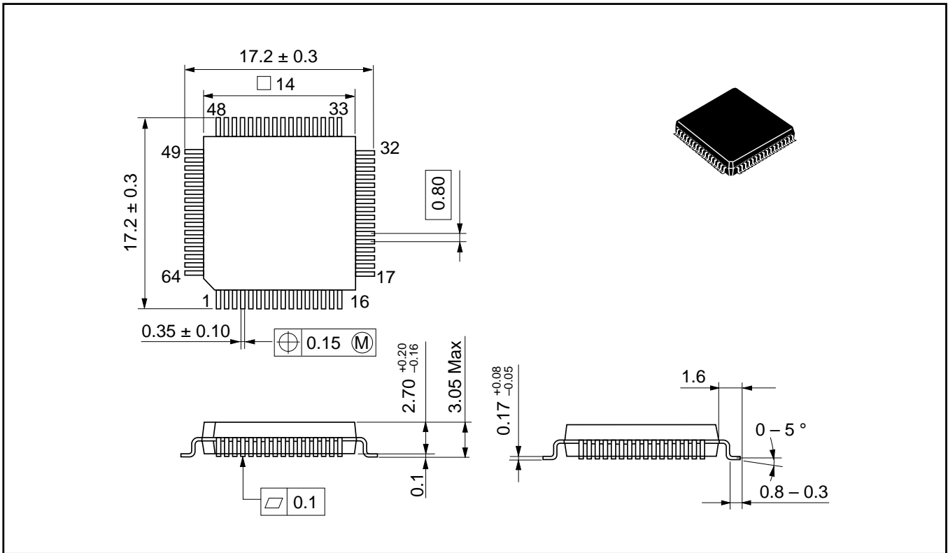
Figure E-3. Package Dimensions (FP-64A)
