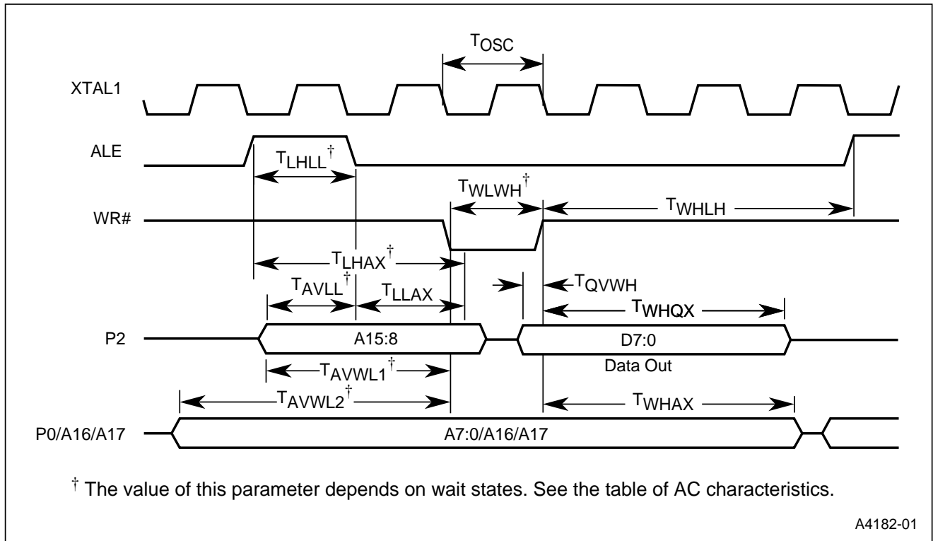
Figure 12. External Bus Cycle: Data Write (Page Mode)
