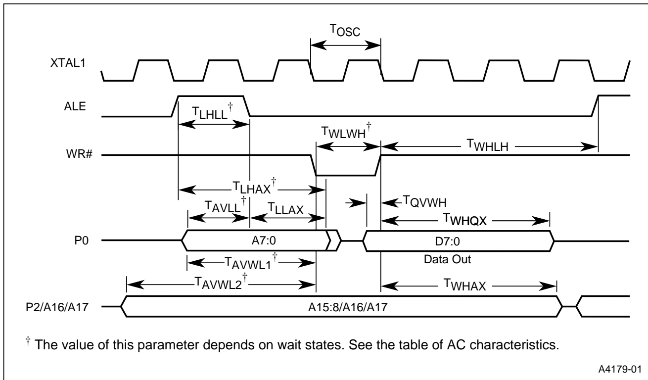
Figure 9. External Bus Cycle: Data Write (Nonpage Mode)
