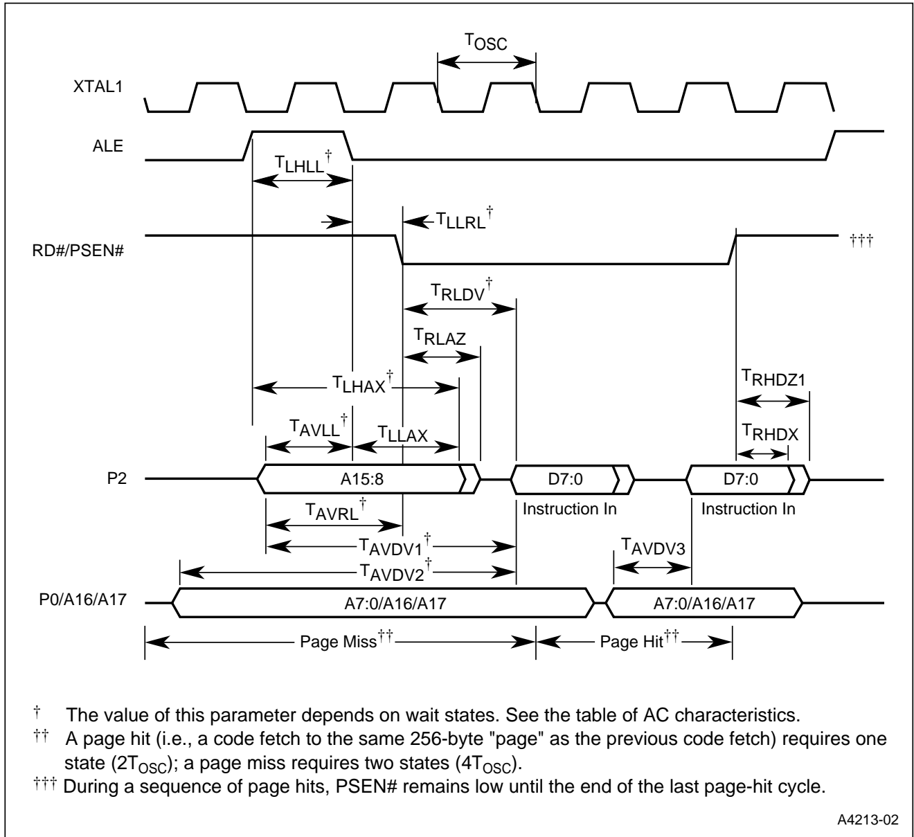
Figure 10. External Bus Cycle: Code Fetch (Page Mode)
