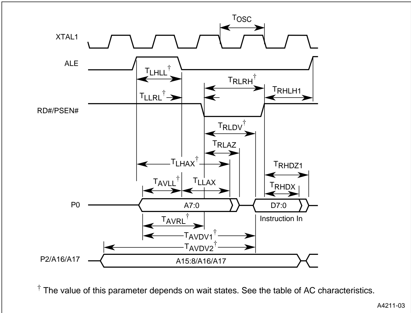
Figure 7. External Bus Cycle: Code Fetch (Nonpage Mode)
