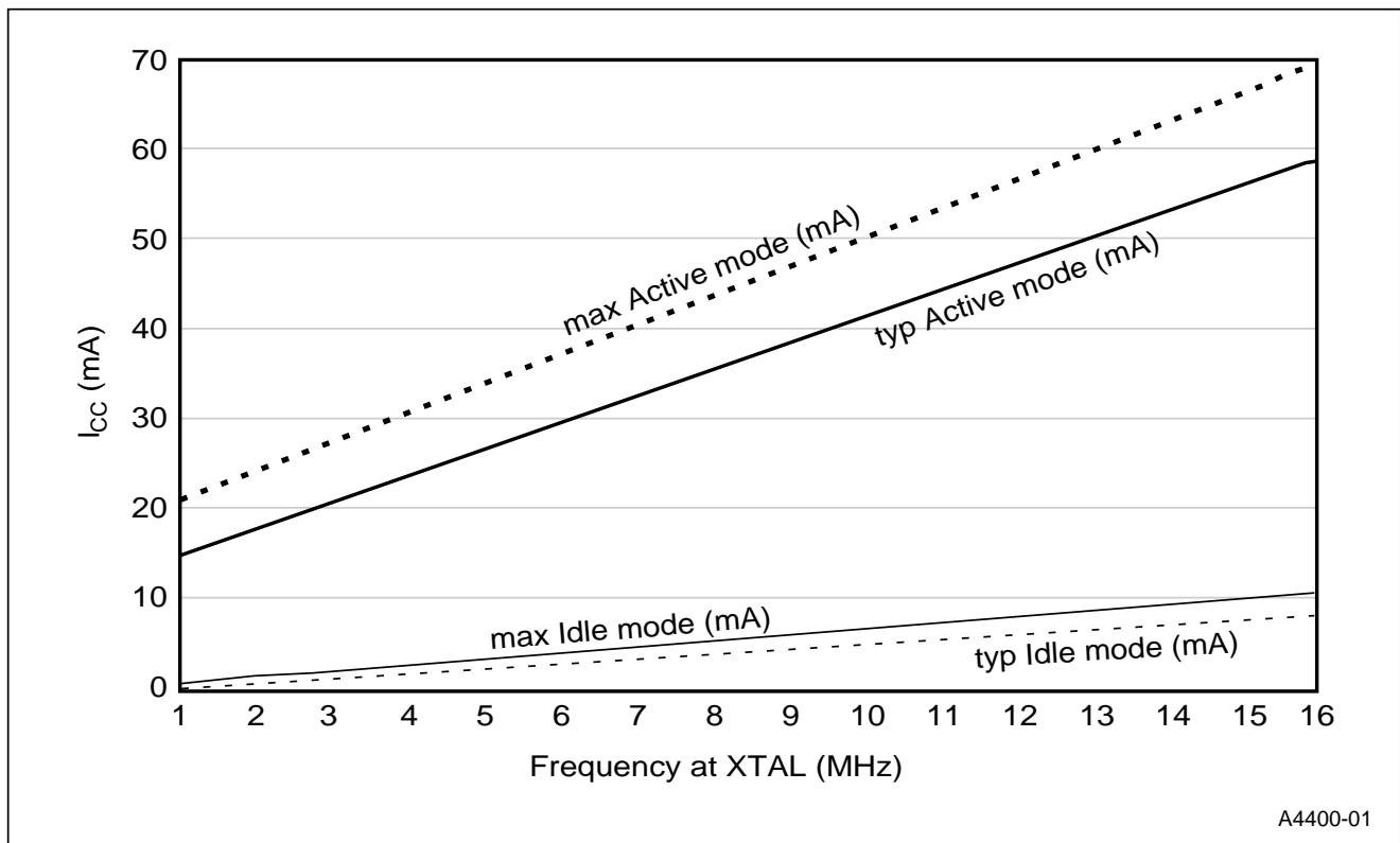
Figure 6. I_{CC} vs. Frequency (Mhz)
