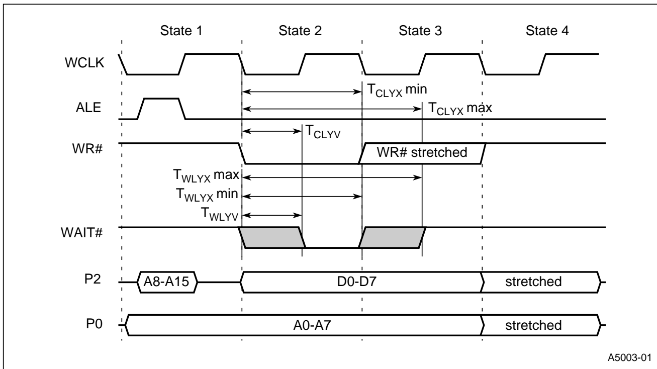
Figure 16. External Bus Cycle: Data Write (Page Mode)
