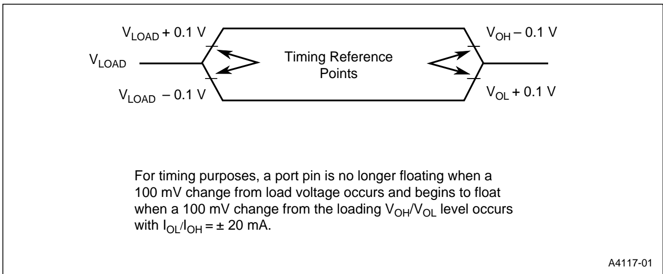
Figure 20. Float Waveforms
