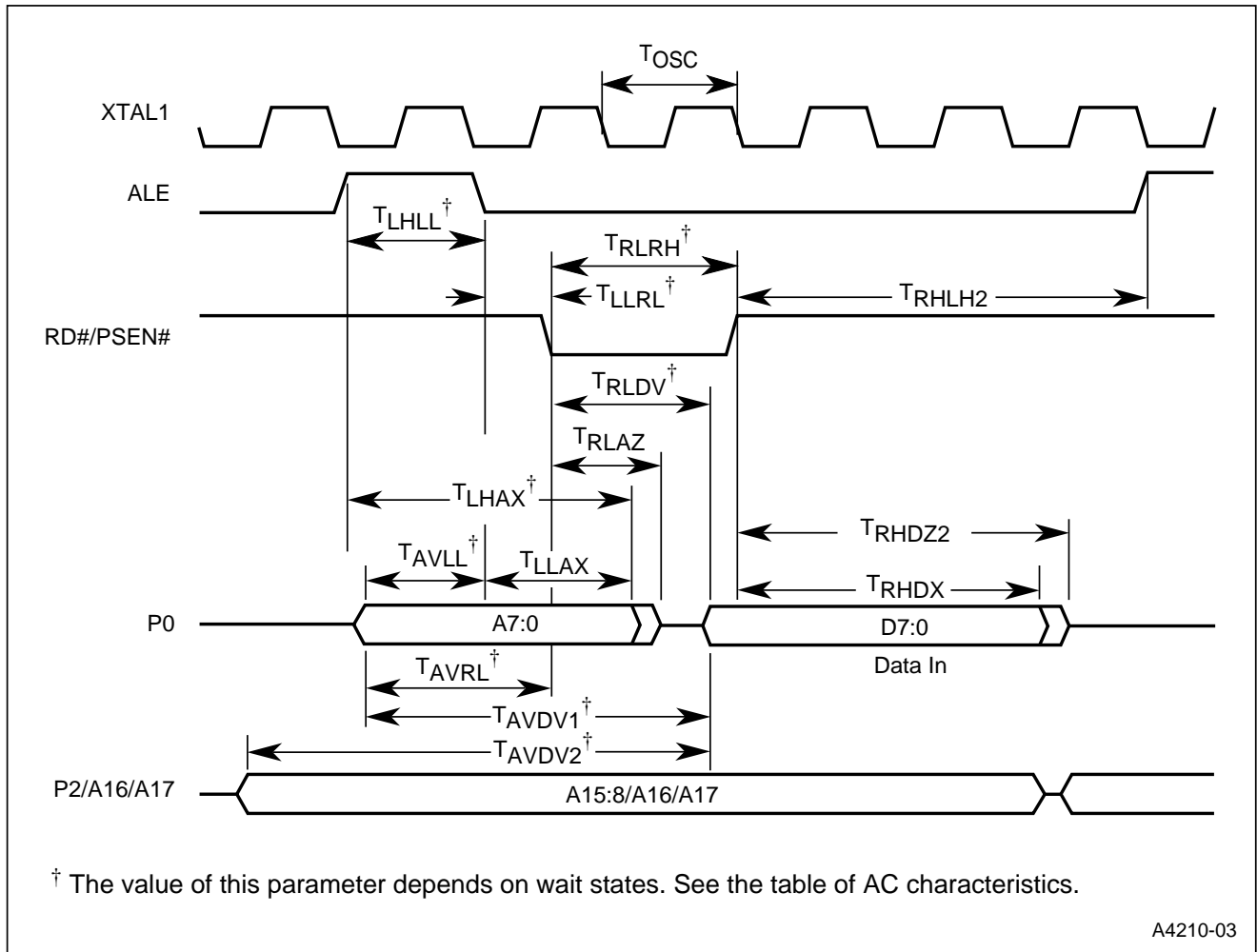
Figure 8. External Bus Cycle: Data Read (Nonpage Mode)
