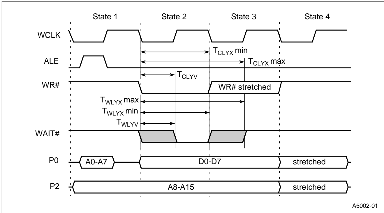
Figure 14. External Bus Cycle: Data Write (Nonpage Mode)
