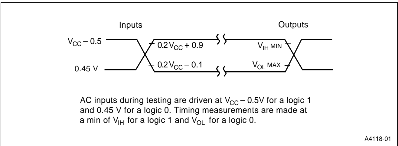
Figure 19. AC Testing Input, Output Waveforms
