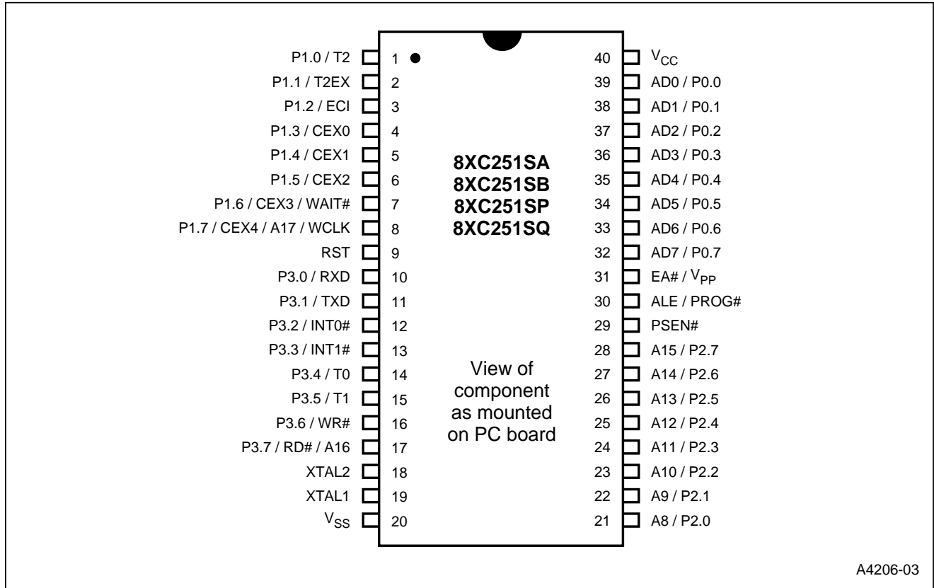
Figure 4. 8XC251SA/SB/SP/SQ 40-pin PDIP and Ceramic DIP Packages
