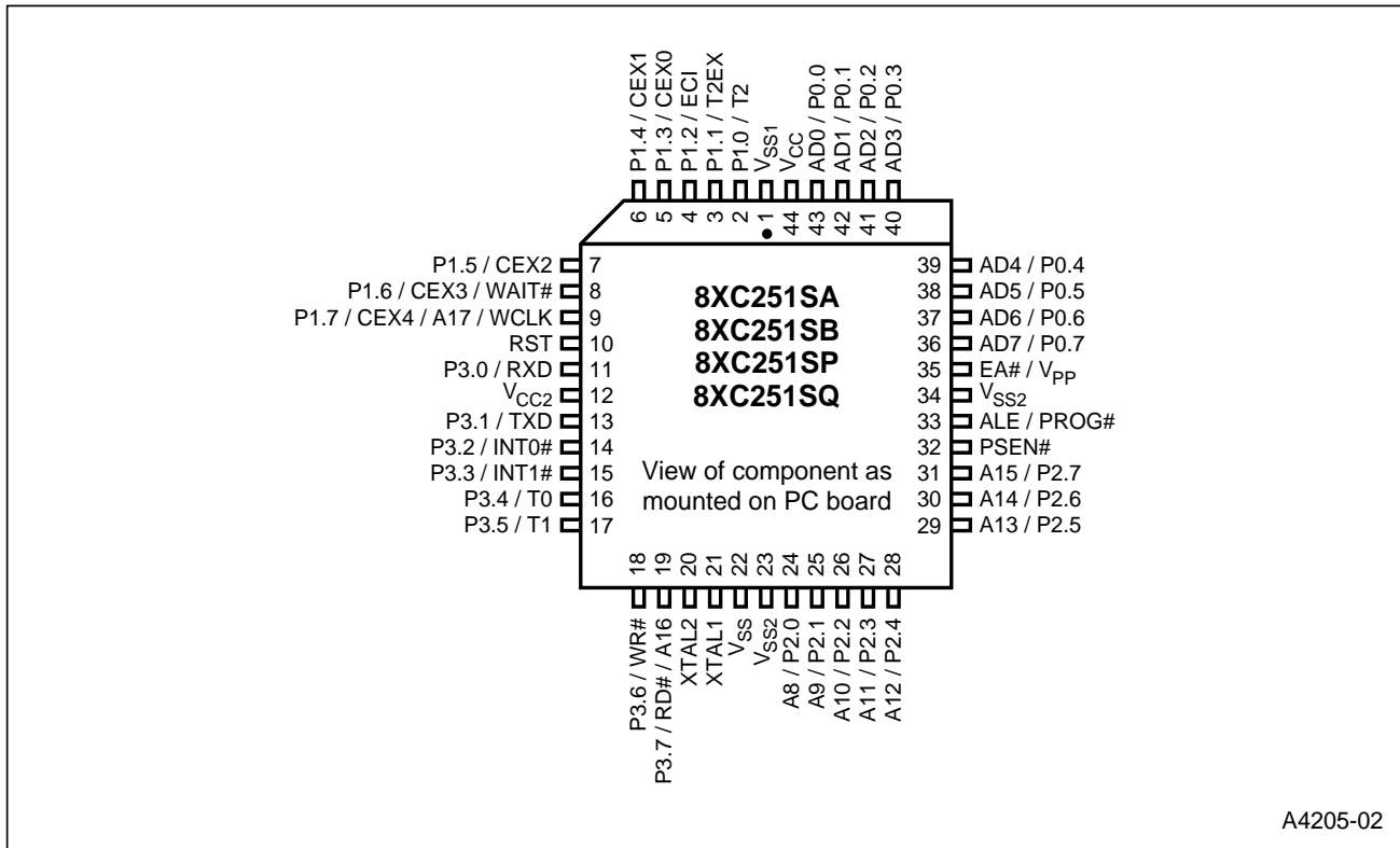
Figure 3. 8XC251SA/SB/SP/SQ 44-pin PLCC Package
