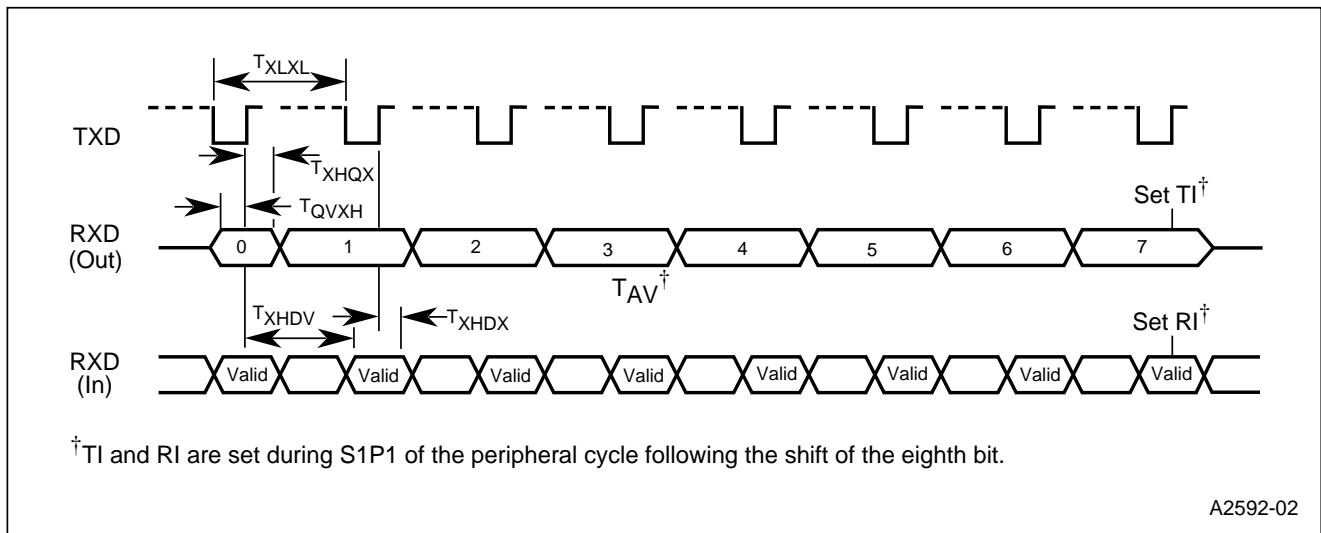
Figure 17. Serial Port Waveform — Shift Register Mode
