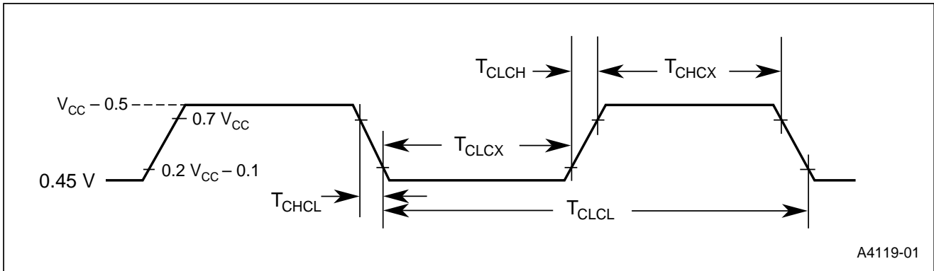
Figure 18. External Clock Drive Waveforms
