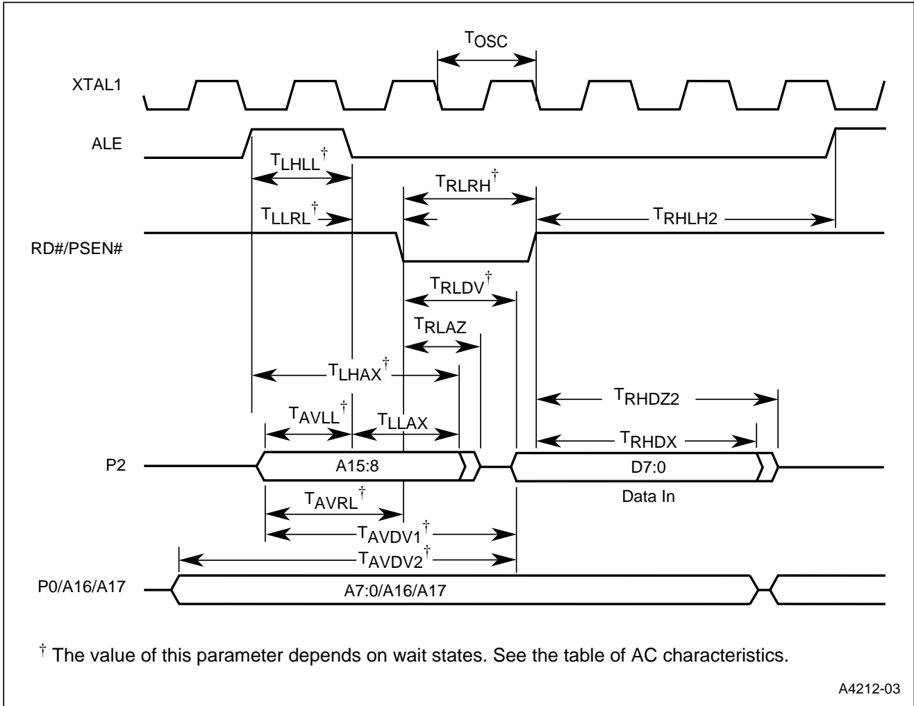
Figure 11. External Bus Cycle: Data Read (Page Mode)
