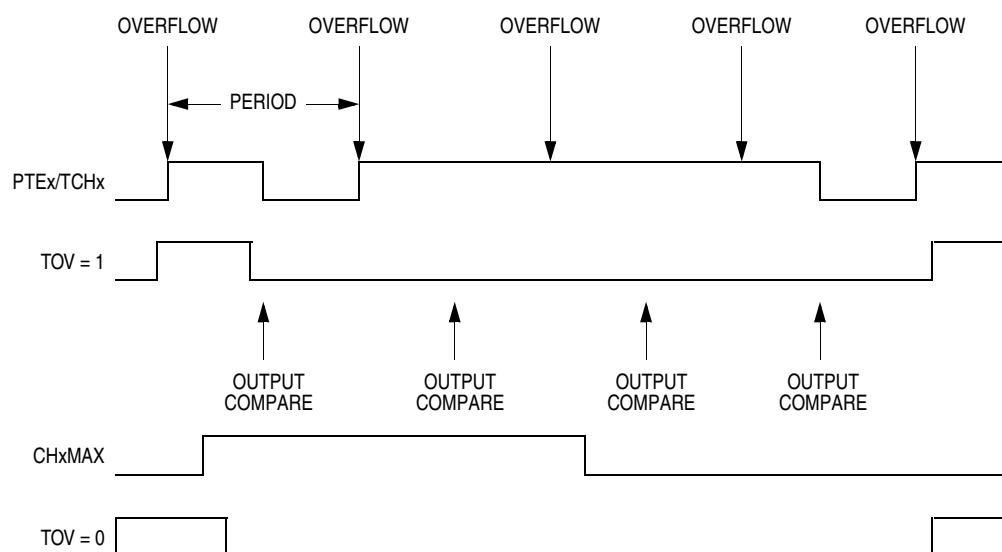
Figure 18-8. CHxMAX Latency
