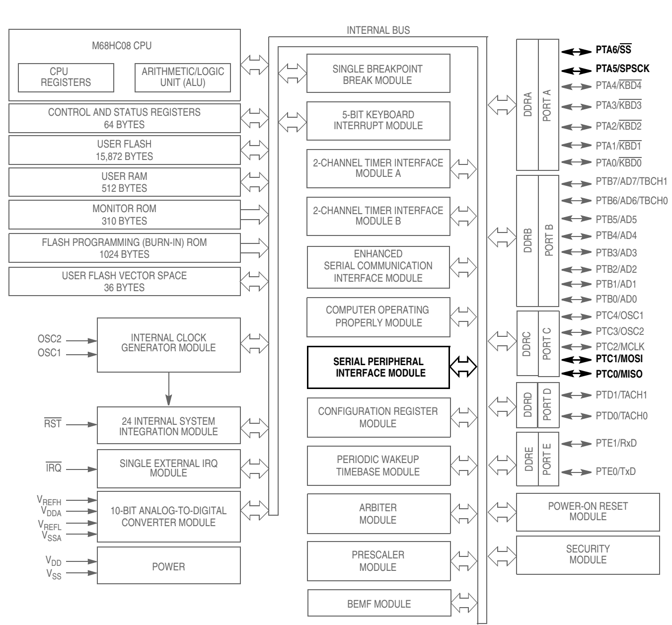
Figure 15-1. Block Diagram Highlighting SPI Block and Pins
