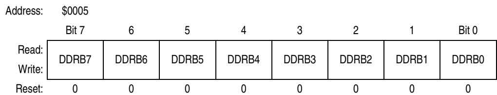
Figure 12-5. Data Direction Register B (DDRB)
