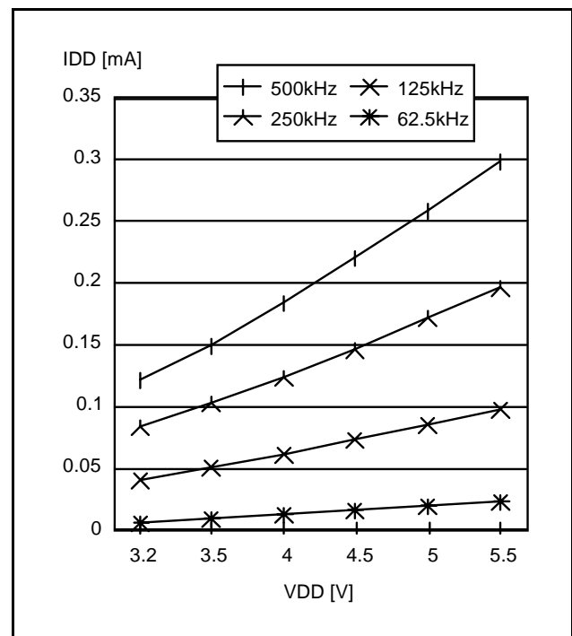
Figure 66. Typical I_{DD} in SLOW-WAIT vs. f_{CPU}
