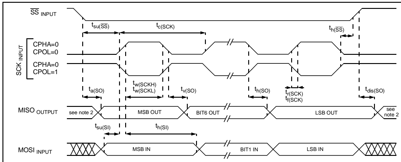
Figure 95. SPI Slave Timing Diagram with CPHA=0 3)
