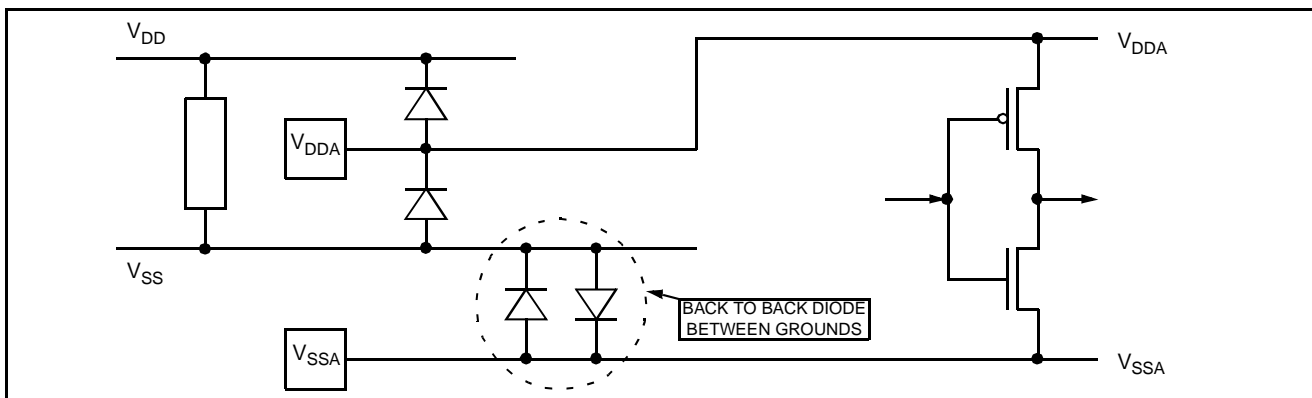
Figure 81. Multisupply Configuration
