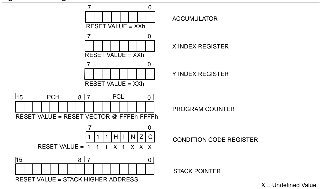
Figure 10. CPU Registers
