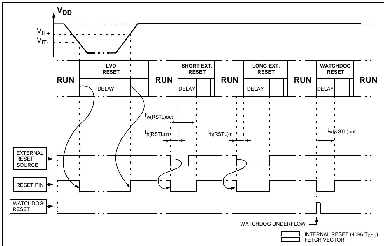
Figure 16. RESET Sequences
