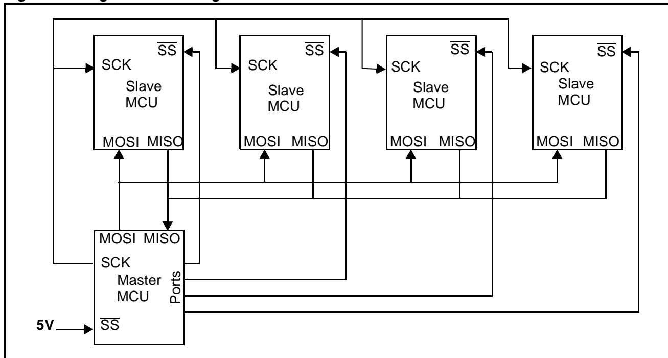
Figure 47. Single Master Configuration
