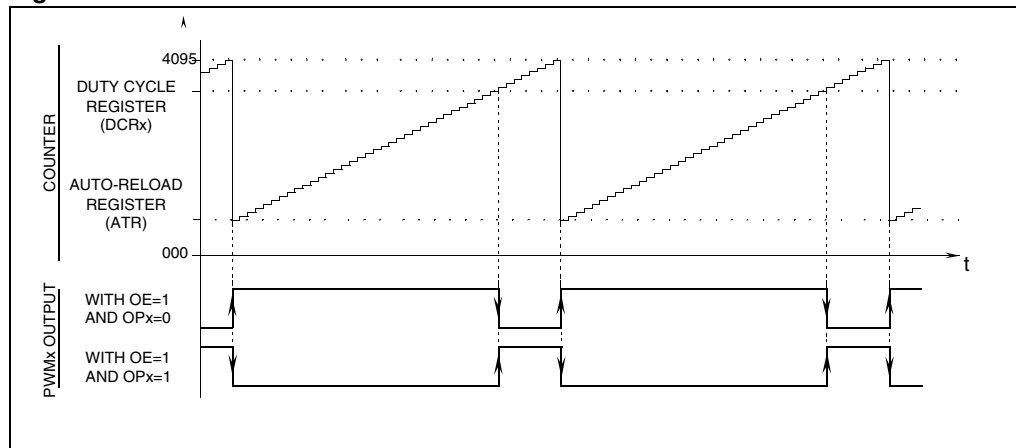
Figure 40. PWM function
