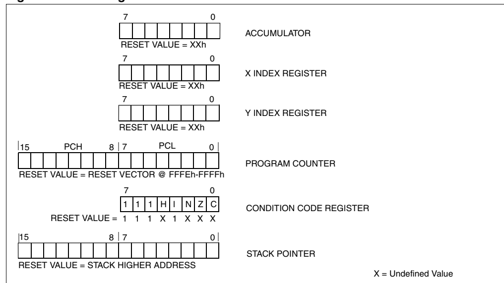
Figure 10. CPU registers
