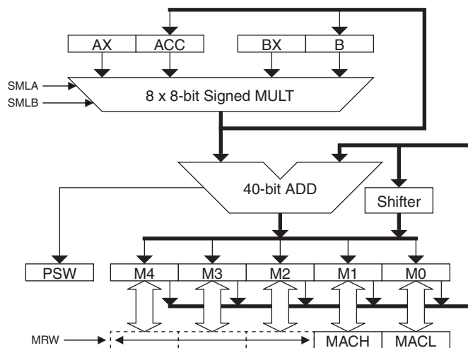
Figure 5-4. Multiply-Accumulate Unit
