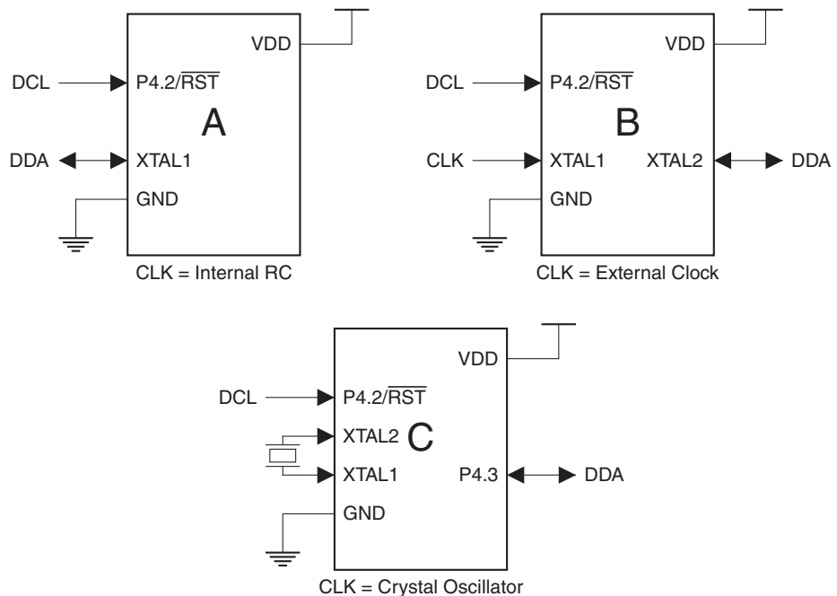
Figure 24-1. AT89LP6440 On-Chip Debug Connections
