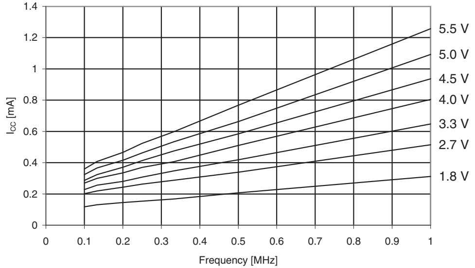
Figure 29-125. ATmega329A: Active Supply Current vs. Low Frequency (0.1 - 1.0 MHz)
