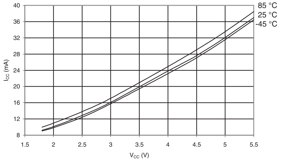
Figure 29-491. ATmega6490A: Active Supply Current vs. V_{CC} (32 kHz Watch Crystal)
