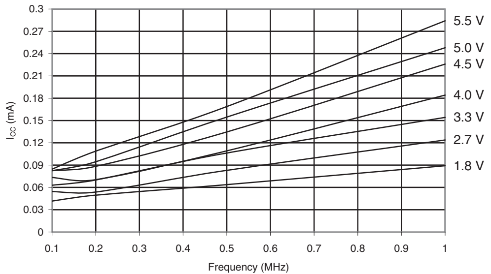
Figure 29-431. ATmega649P: Idle Supply Current vs. Low Frequency (0.1 - 1.0 MHz)
