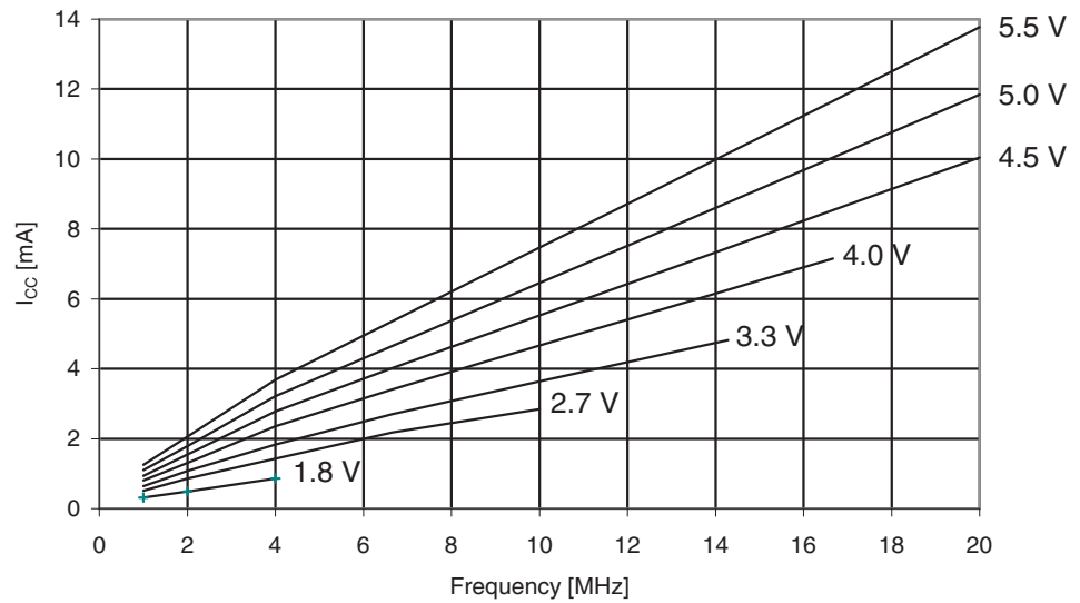
Figure 29-186. ATmega329PA: Active Supply Current vs. Frequency (1 - 20MHz)
