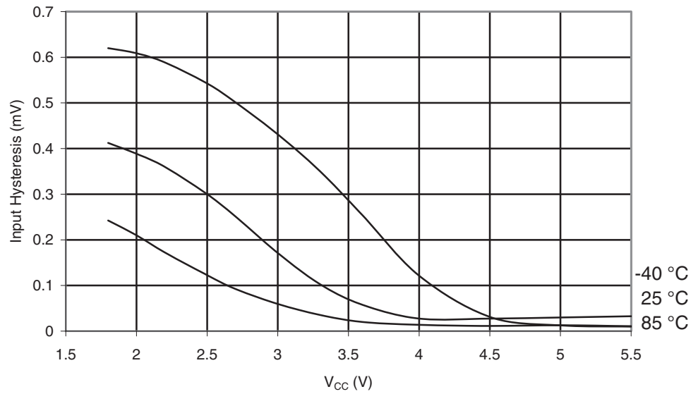
Figure 29-223. ATmega329PA: Reset Input Pin Hysteresis vs. V_{CC}
