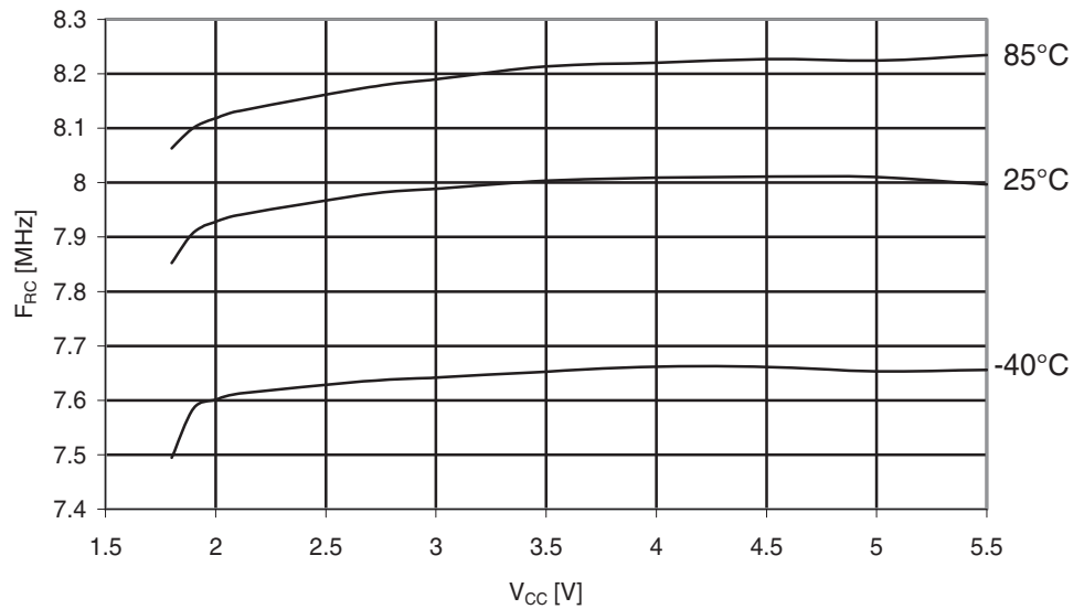
Figure 29-292. ATmega3290A: Calibrated 8 MHz RC Oscillator Frequency vs. V CC
