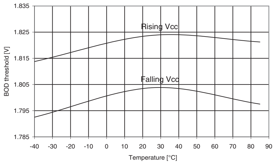
Figure 29-286. ATmega3290A: BOD Thresholds vs. Temperature (BOD Level is 1.8V)
