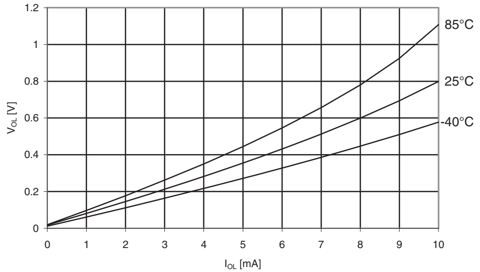
Figure 29-273. ATmega3290A. I/O Pin Output Voltage vs. Sink Current, Ports A, C, D, E, F, G ( V_{CC} = 2.7V )
