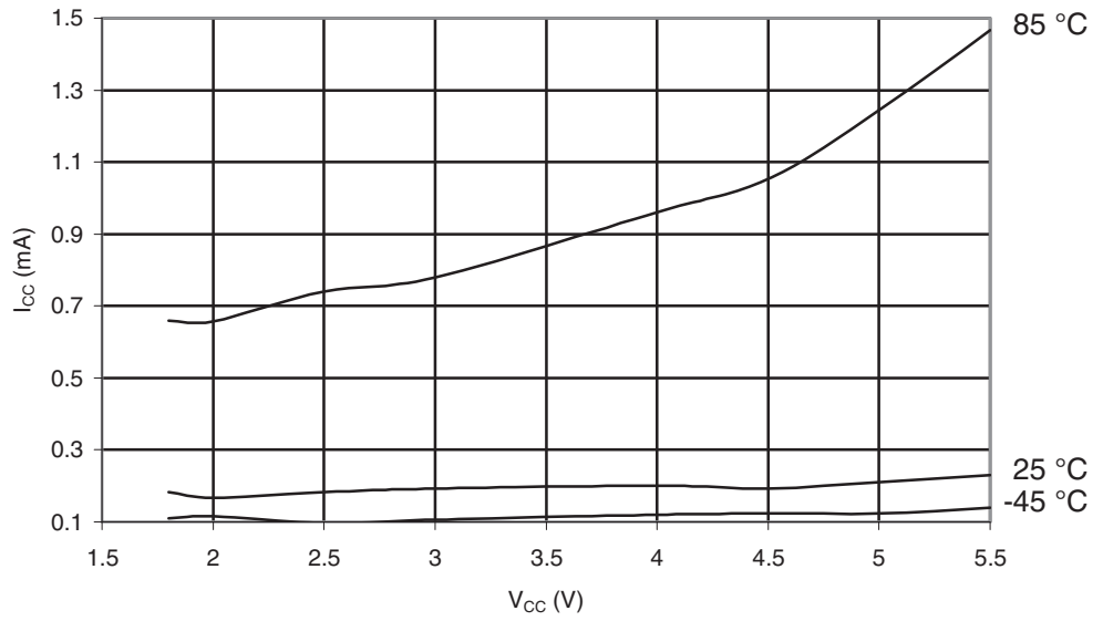
Figure 29-560. ATmega649A: Power-down Supply Current vs. V_{CC} (32 kHz Watch Crystal)
