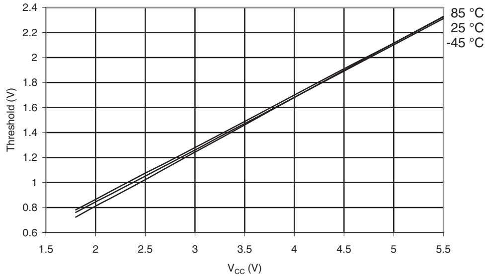
Figure 29-38. ATmega169A: Reset Input Threshold Voltage vs. V_{CC} ( V_{IL} , Reset Pin Read as "0")
