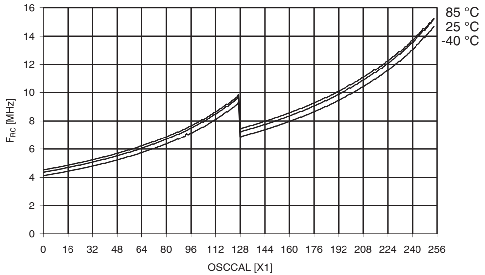
Figure 29-293. ATmega3290A: Calibrated 8 MHz RC Oscillator Frequency vs. Oscal Value
