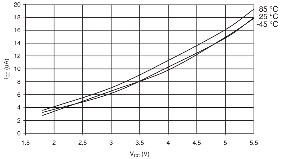
Figure 29-74. ATmega169PA: Power-down Supply Current vs. V_{CC} (Watchdog Timer Enabled)
