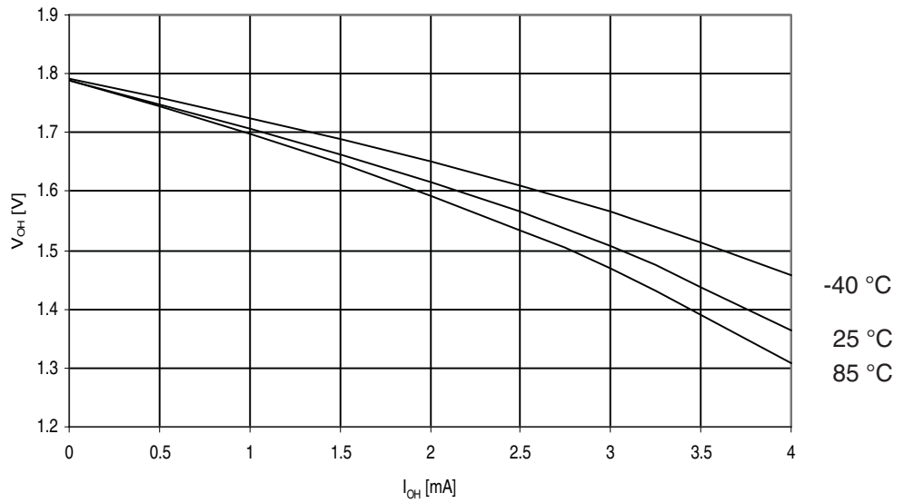
Figure 29-208. ATmega329PA: I/O Pin Output Voltage vs. Source Current, Ports A, C, D, E, F, G ( V_{CC} = 1.8V )
