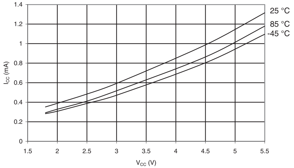
Figure 29-4. ATmega169A: Active Supply Current vs. V_{CC} (Internal RC Oscillator, 1 MHz)
