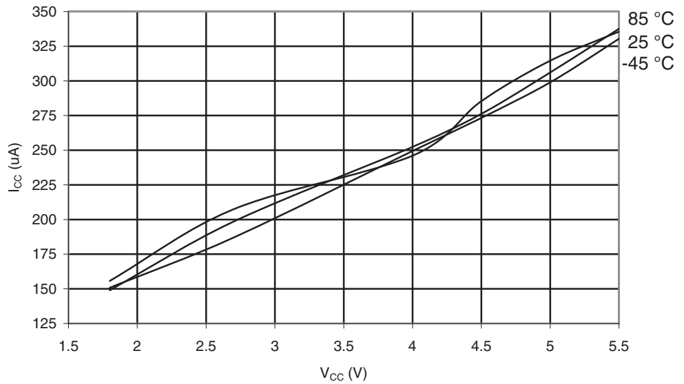
Figure 29-55. ATmega169A: Active Supply Current with ADC at 1 MHz vs. V_{CC}
