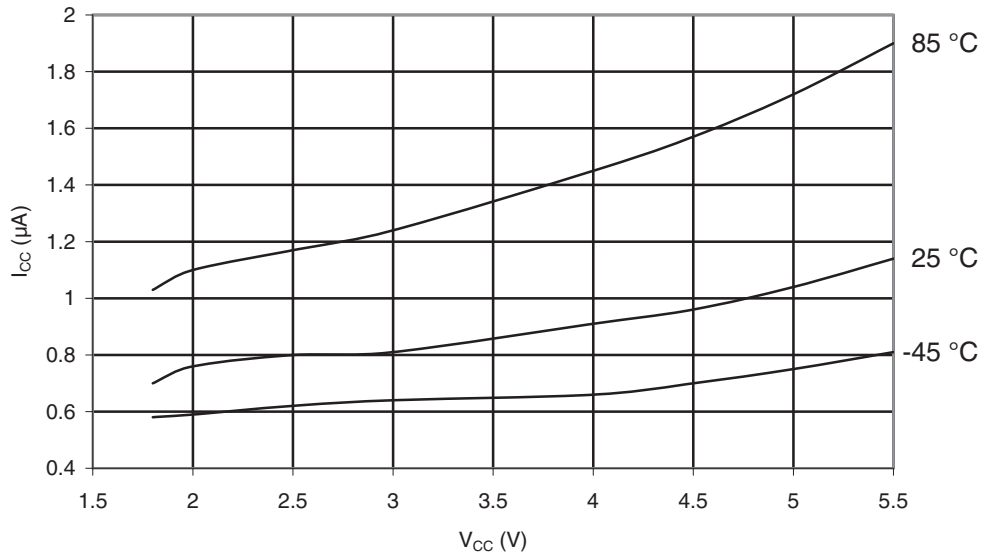
Figure 29-13. ATmega169A: Power-save Supply Current vs. V_{CC} (Watchdog Timer Disabled and 32 kHz Crystal Oscillator Running)
