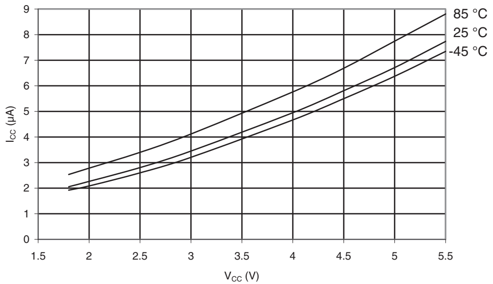
Figure 29-72. ATmega169PA: Idle Supply Current vs. V_{CC} (32 kHz Watch Crystal)
