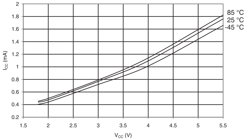
Figure 29-555. ATmega6490P: Idle Supply Current vs. V_{CC} (Internal RC Oscillator, 8 MHz)
