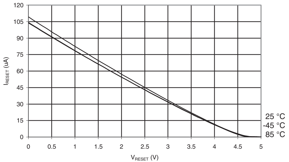
Figure 29-445. ATmega649P: Reset Pull-up Resistor Current vs. Reset Pin Voltage ( V_{CC} = 5V )
