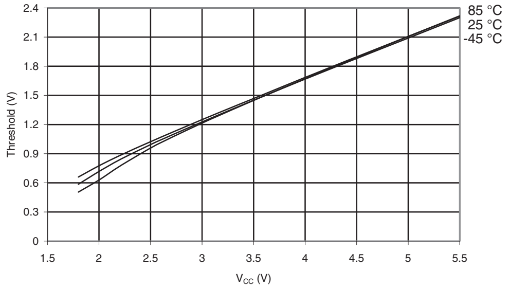
Figure 29-97. ATmega169PA. I/O Pin Input Threshold Voltage vs. V_{CC} ( V_{IL} , I/O Pin Read as "0")
