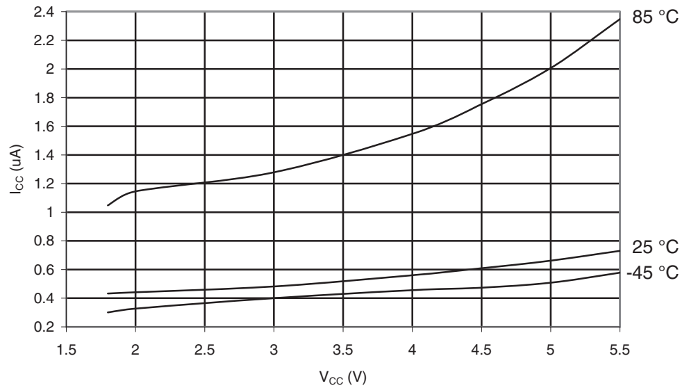
Figure 29-558. ATmega6490P: Power-down Supply Current vs. V_{CC} (Watchdog Timer Disabled)
