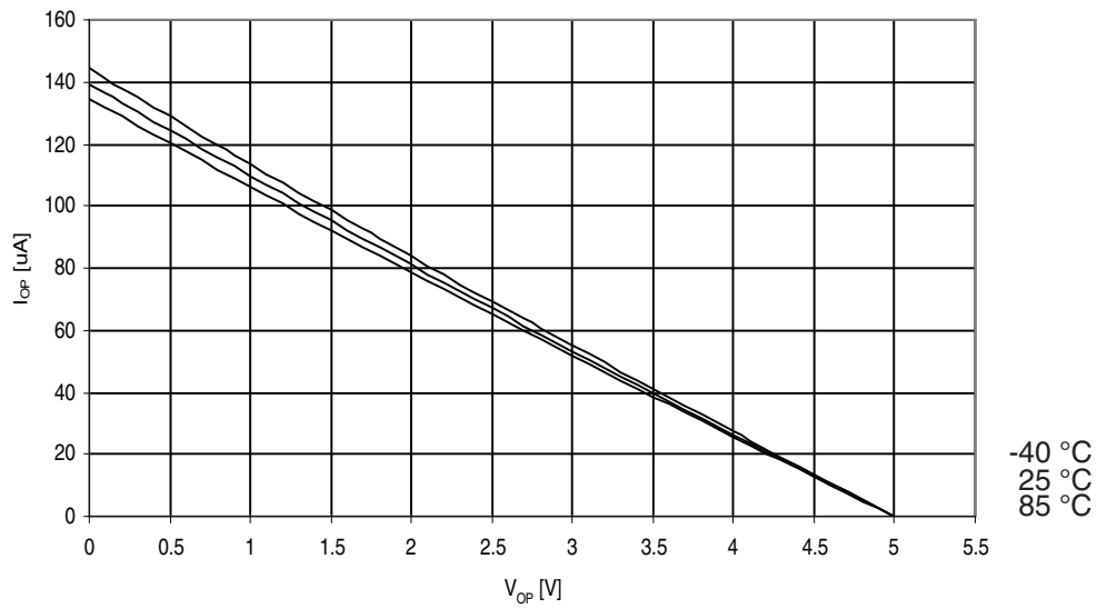
Figure 29-200. ATmega329PA: I/O Pin Pull-up Resistor Current vs. Input Voltage ( V_{CC} = 5V )
