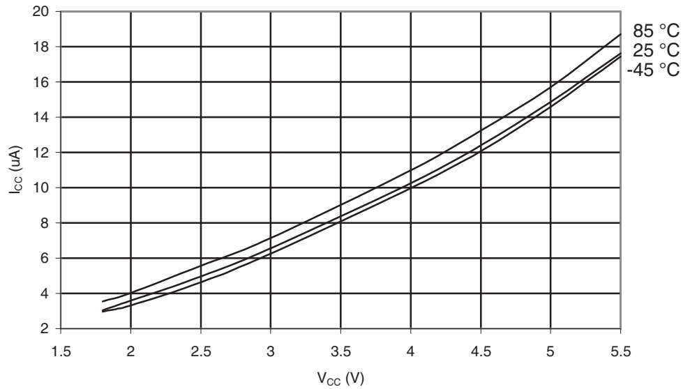
Figure 29-498. ATmega6490A: Power-down Supply Current vs. V_{CC} (Watchdog Timer Enabled)
