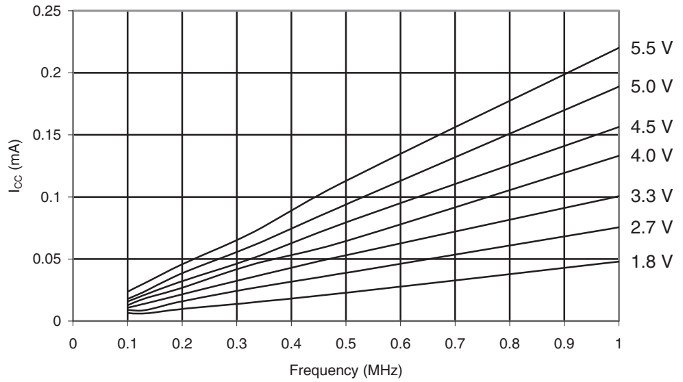
Figure 29-6. ATmega169A: Idle Supply Current vs.Low Frequency (0.1 - 1.0 MHz)
