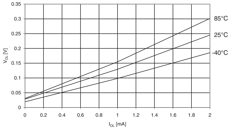
Figure 29-274. ATmega3290A: I/O Pin Output Voltage vs. Sink Current, Ports A, C, D, E, F, G ( V_{CC} = 1.8V )
