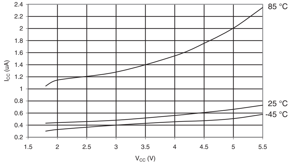
Figure 29-497. ATmega6490A: Power-down Supply Current vs. V_{CC} (Watchdog Timer Disabled)
