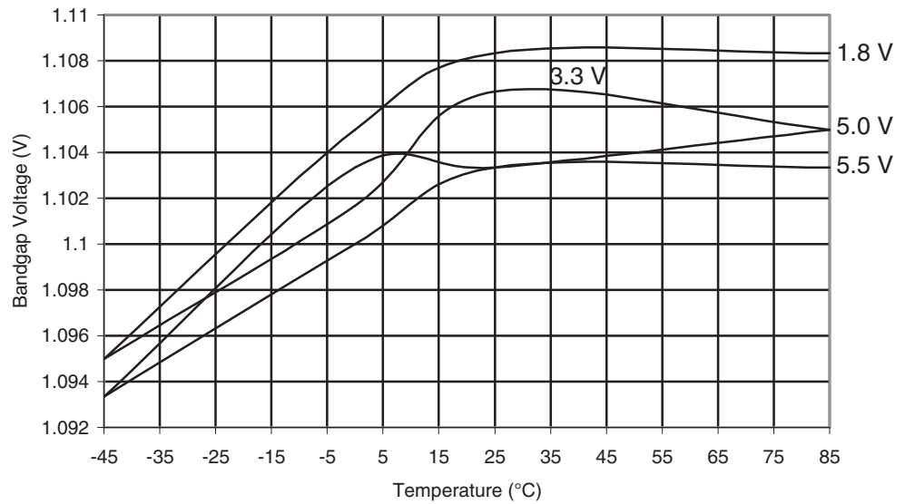
Figure 29-409. ATmega649A: Bandgap Voltage vs. Temperature
