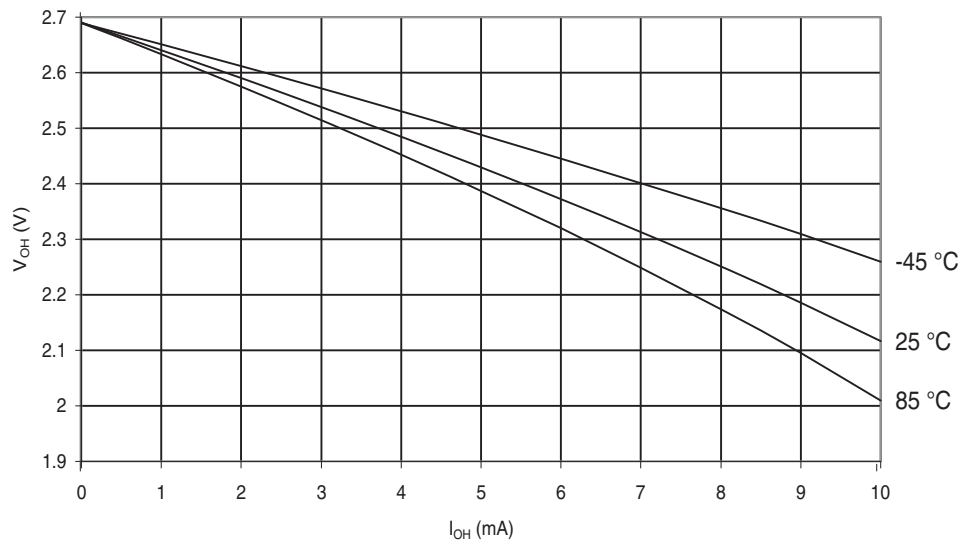
Figure 29-510. ATmega6490A: I/O Pin Output Voltage vs. Source Current, Ports A, C, D, E, F, G ( V_{CC} = 2.7V )
