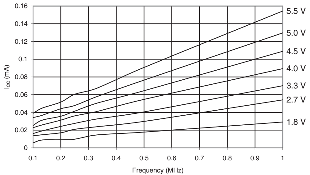
Figure 29-122. ATmega169PA: Reset Supply Current vs. V_{CC} (0.1 - 1.0 MHz, Excluding Current Through The Reset Pull-up)
