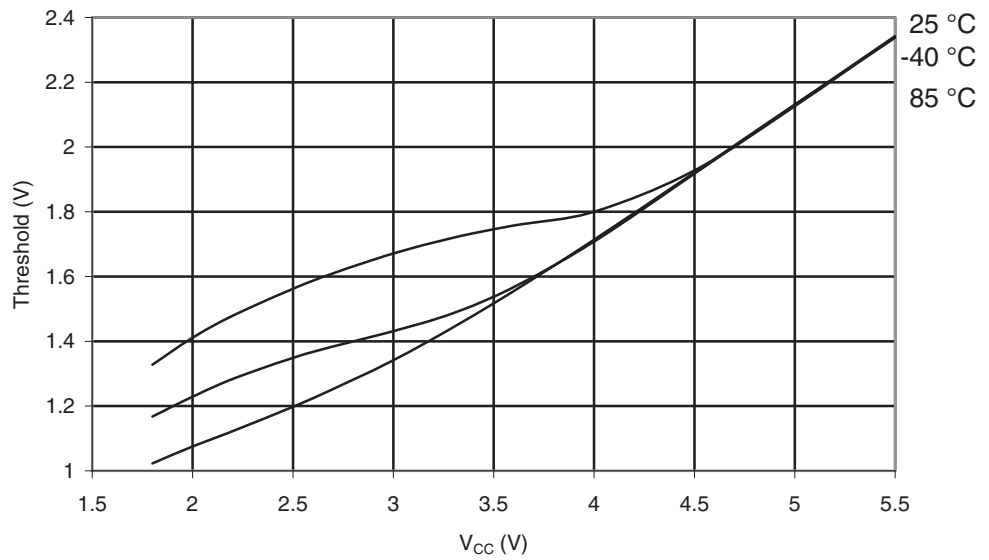
Figure 29-221. ATmega329PA: Reset Input Threshold Voltage vs. V_{CC} ( V_{IH} , Reset Pin Read as "1")
