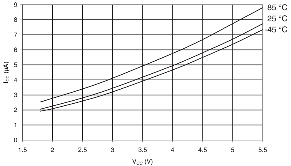
Figure 29-10. ATmega169A: Idle Supply Current vs. V_{CC} (32 kHz Watch Crystal)
