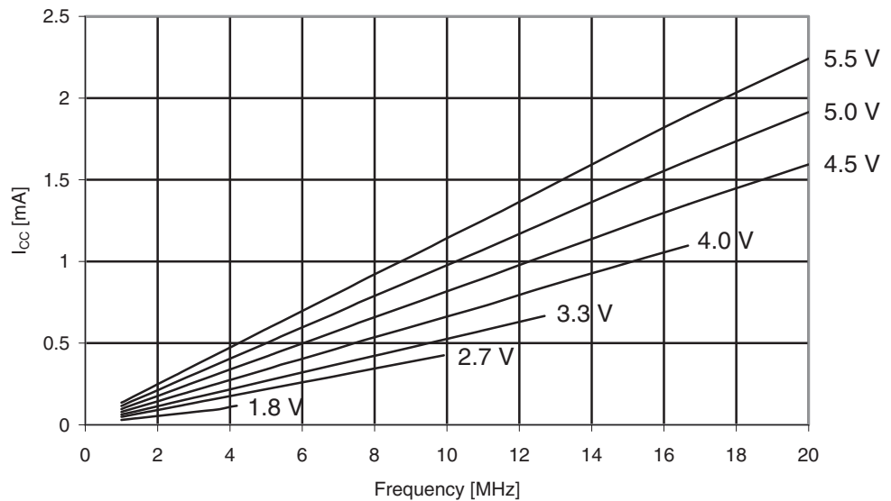
Figure 29-183. ATmega329A: Reset Supply Current vs. V_{CC} (1 - 20MHz, Excluding Current Through The Reset Pull-up)
