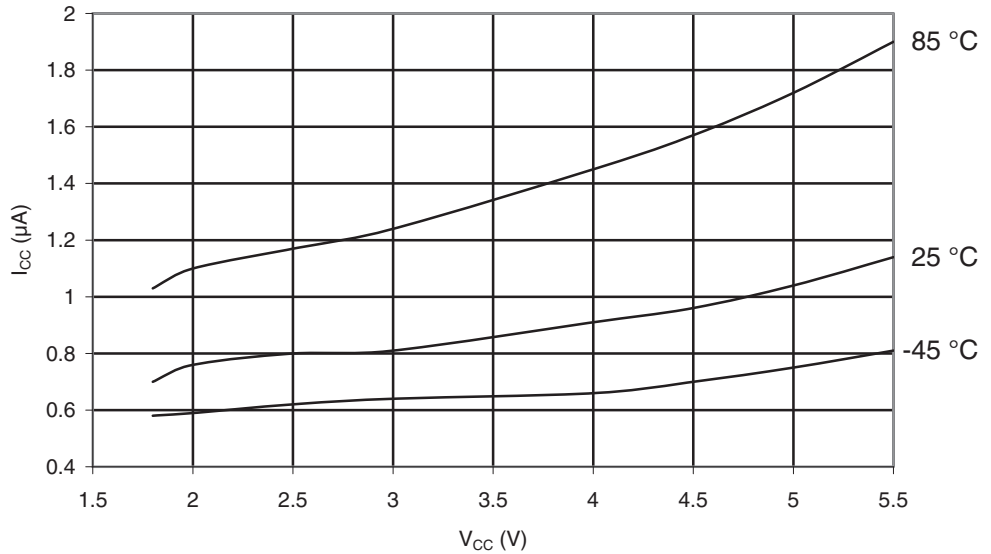
Figure 29-75. ATmega169PA: Power-save Supply Current vs. V_{CC} (Watchdog Timer Disabled)
