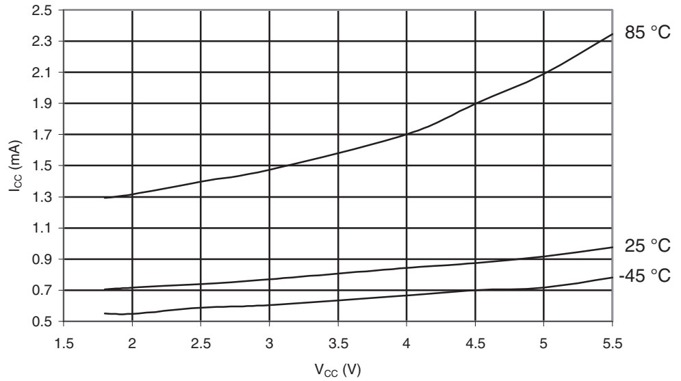
Figure 29-441. ATmega649P: Standby Supply Current vs. V_{CC} (Xtall and Resonator, Watchdog Timer Disabled)
