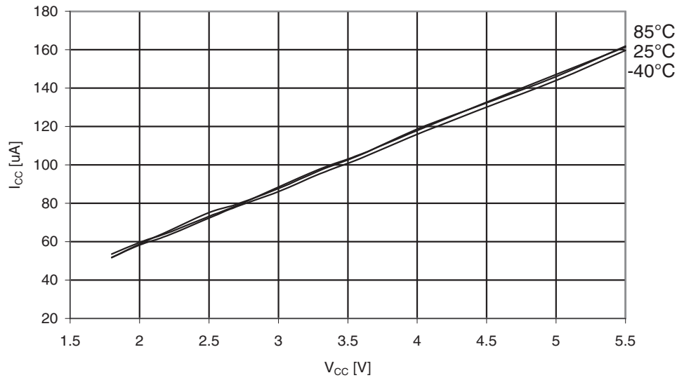
Figure 29-238. ATmega329PA: AREF External Reference Current vs. V_{CC}
