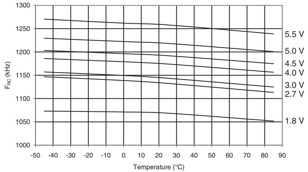
Figure 29-110. ATmega169PA: Watchdog Oscillator Frequency vs. Temperature
