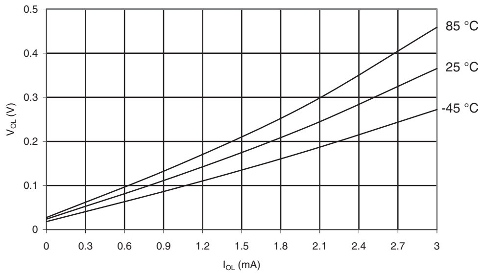
Figure 29-92. ATmega169PA: I/O Pin Output Voltage vs. Sink Current, Ports A, C, D, E, F, G ( V_{CC} = 1.8V )
