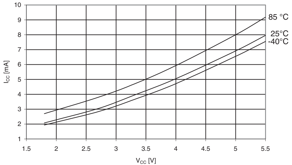
Figure 29-314. ATmega3290PA: Idle Supply Current vs. V_{CC} (32 kHz Watch Crystal)
