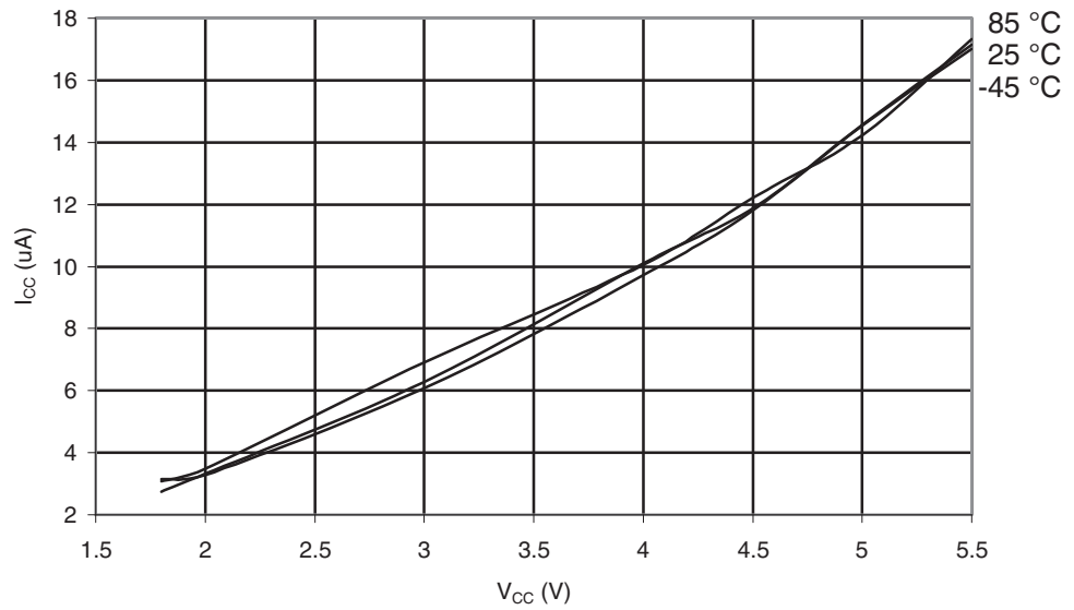
Figure 29-420. ATmega649A: Watchdog Timer Current vs. V_{CC}
