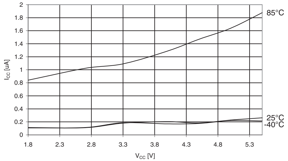
Figure 29-315. ATmega3290PA Power-down Supply Current vs. V_{CC} (Watchdog Timer Disabled)
