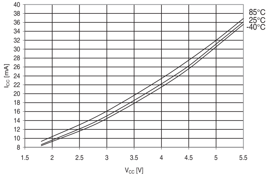
Figure 29-309. ATmega3290PA: Active Supply Current vs. V_{CC} (32 kHz Watch Crystal)
