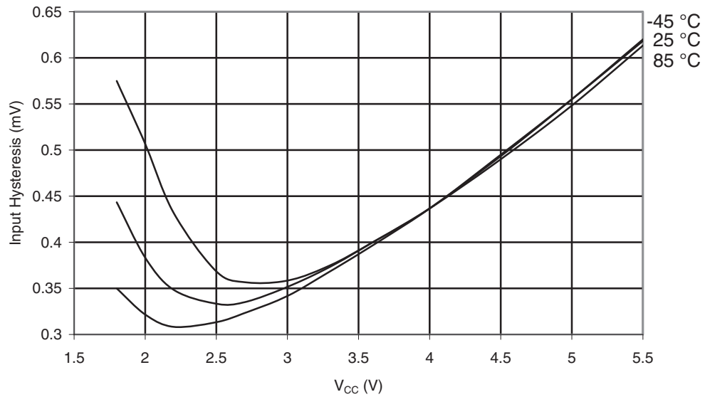
Figure 29-98. ATmega169PA: I/O Pin Input Hysteresis vs. V_{CC}
