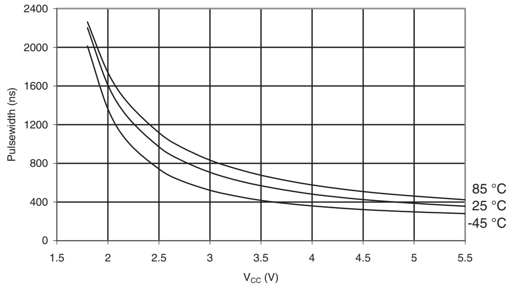
Figure 29-124. ATmega169PA: Minimum Reset Pulse Width vs. V_{CC}
