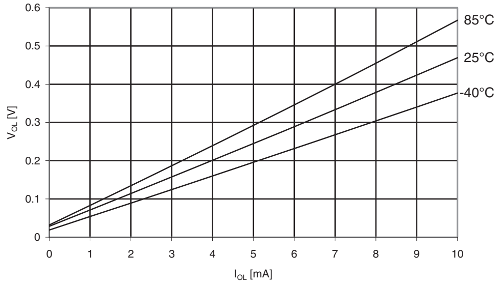
Figure 29-212. ATmega329PA: I/O Pin Output Voltage vs. Sink Current, Ports A, C, D, E, F, G ( V_{CC} = 5V )
