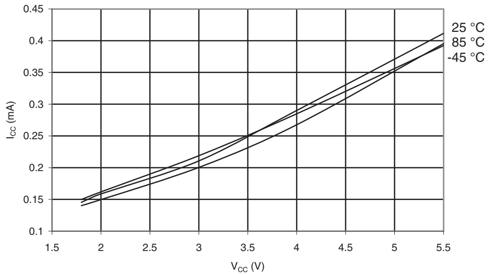
Figure 29-429. ATmega649P: Active Supply Current vs. V_{CC} (Internal RC Oscillator, 1 MHz)
