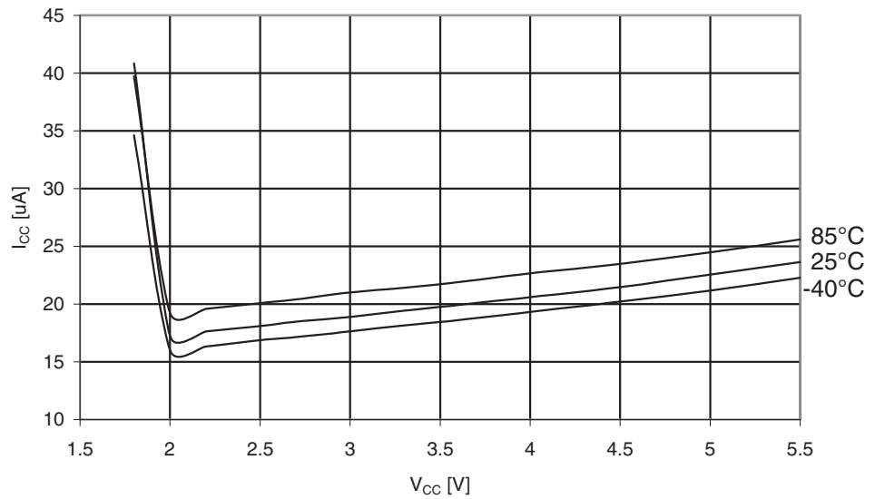
Figure 29-174. ATmega329A: Brownout Detector Current vs. V_{CC}
