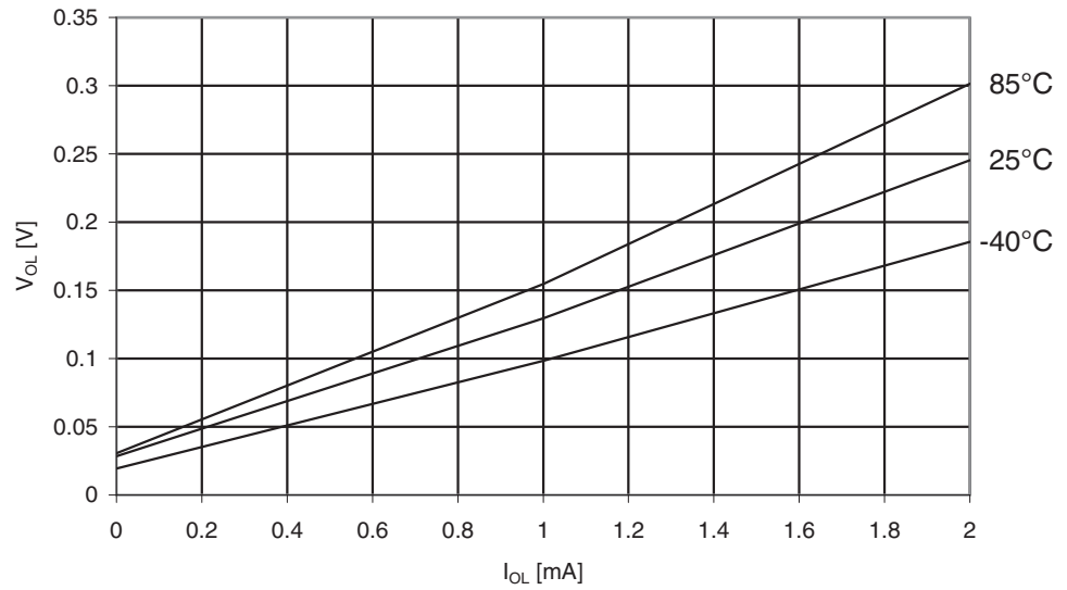
Figure 29-214. ATmega329PA: I/O Pin Output Voltage vs. Sink Current, Ports A, C, D, E, F, G ( V_{CC} = 1.8V )
