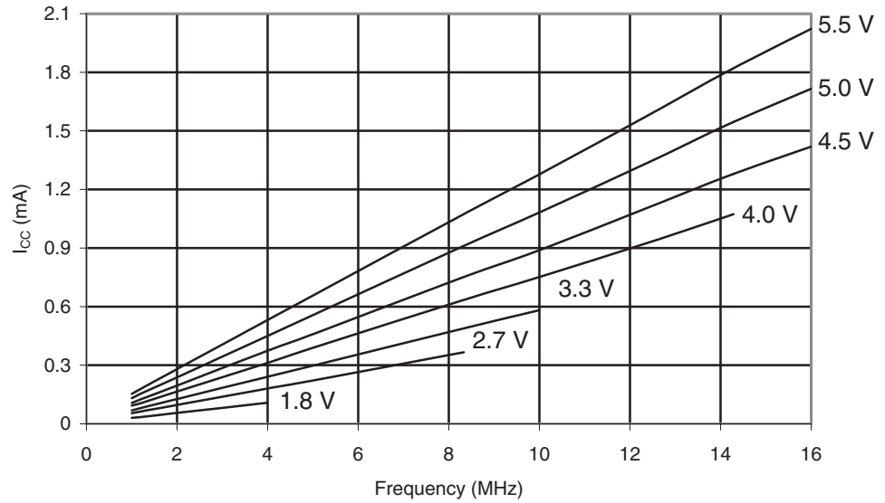
Figure 29-123. ATmega169PA: Reset Supply Current vs. V_{CC} (1 - 16 MHz, Excluding Current Through The Reset Pull-up)
