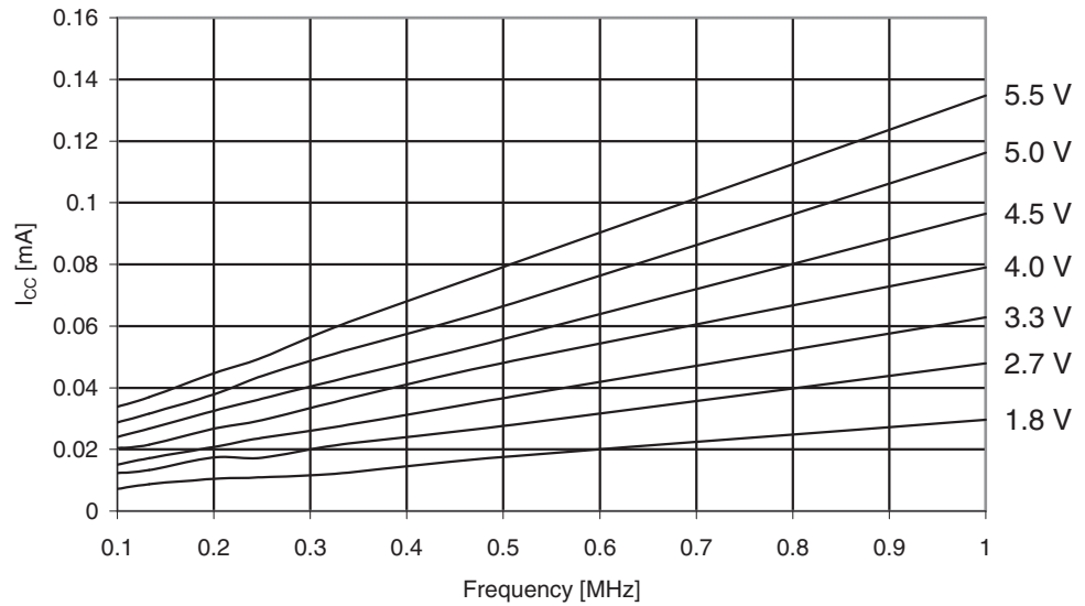
Figure 29-302. ATmega3290A: Reset Supply Current vs. V_{CC} (0.1 - 1.0 MHz, Excluding Current Through The Reset Pull-up)
