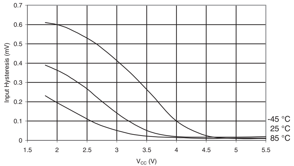
Figure 29-526. ATmega6490A: Reset Input Pin Hysteresis vs. V_{CC}
