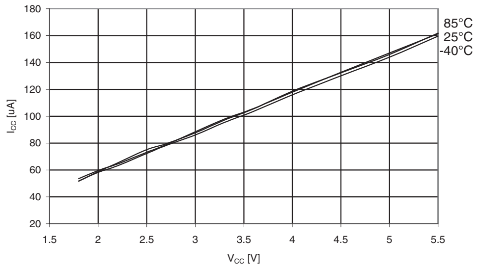
Figure 29-298. ATmega3290A: AREF External Reference Current vs. V_{CC}
