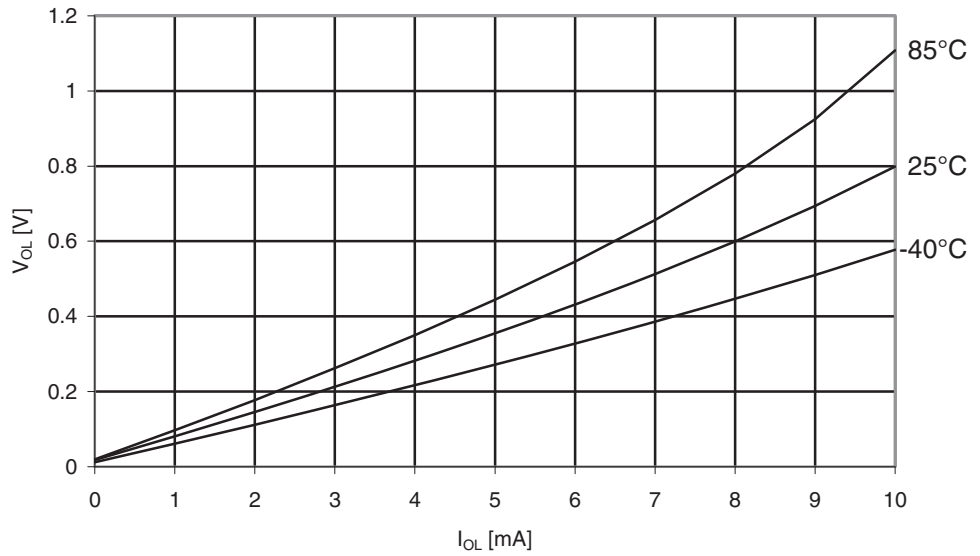
Figure 29-153. ATmega329A: I/O Pin Output Voltage vs. Sink Current, Ports A, C, D, E, F, G ( V_{CC} = 2.7V )
