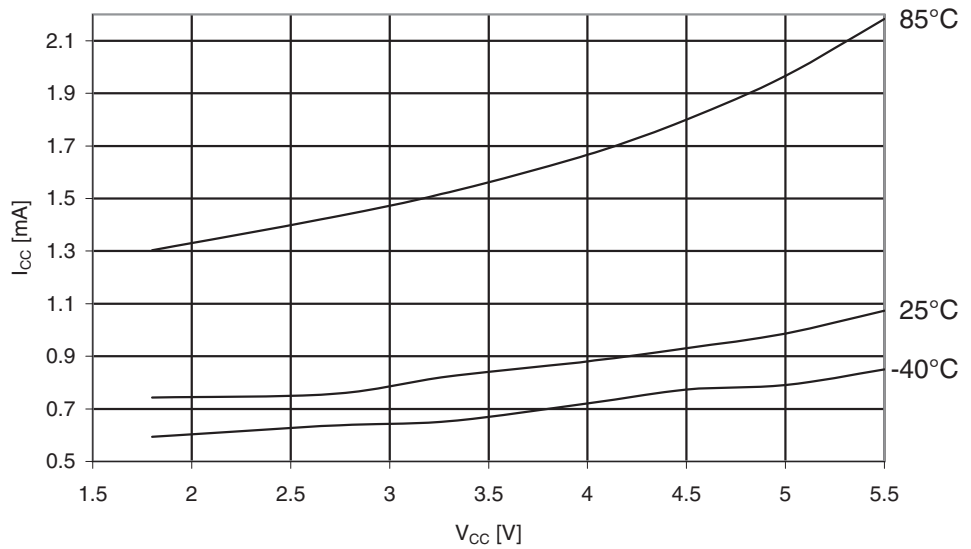
Figure 29-318. ATmega3290PA Standby Supply Current vs. V_{CC} (32 kHz Watch Crystal, Watchdog Timer Disabled)
