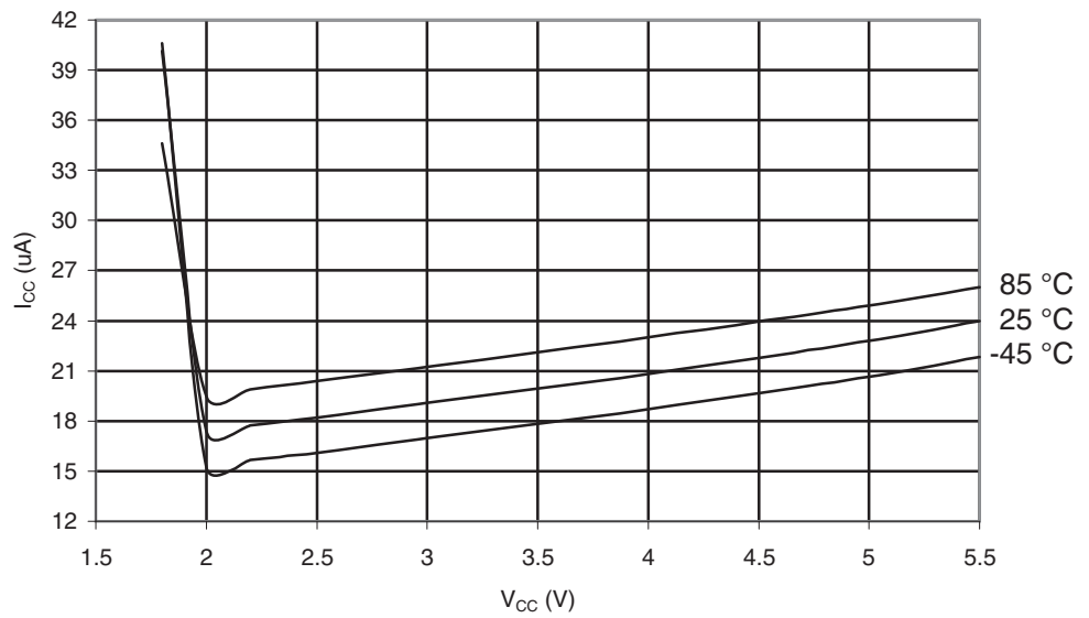
Figure 29-537. ATmega6490A: Brownout Detector Current vs. V_{CC}
