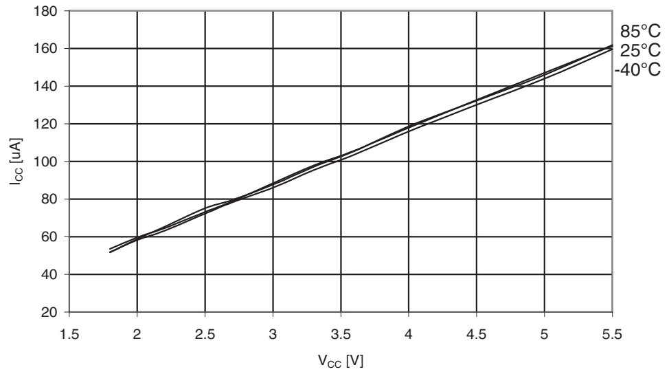
Figure 29-178. ATmega329A: AREF External Reference Current vs. V_{CC}
