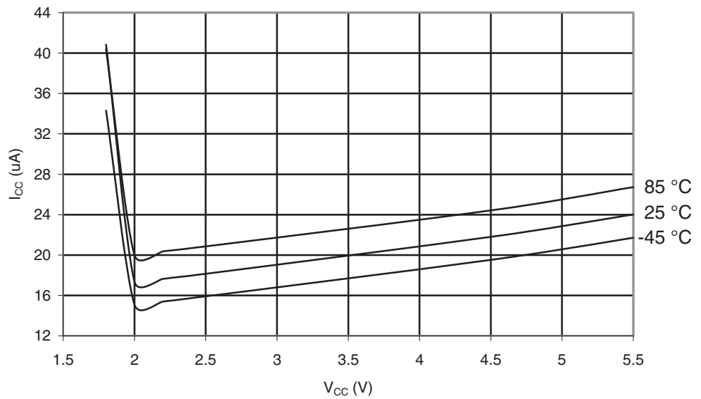
Figure 29-114. ATmega169PA: Brownout Detector Current vs. V_{CC}
