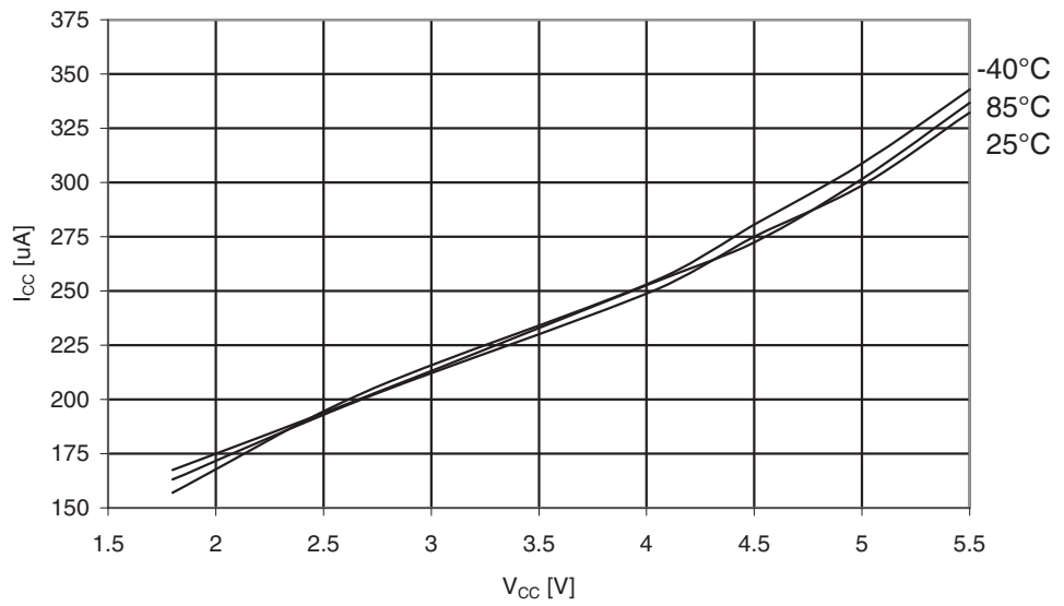
Figure 29-235. ATmega329PA: Active Supply Current with ADC at 50 kHz vs. V_{CC}
