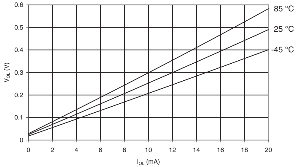
Figure 29-93. ATmega169PA: I/O Pin Output Voltage vs. Sink Current, Port B ( V_{CC} = 5V )
