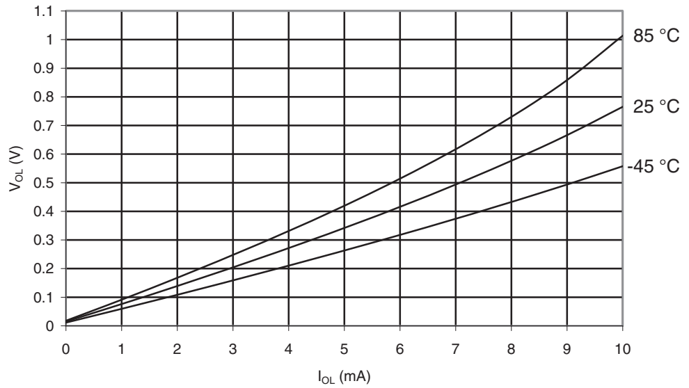
Figure 29-91. ATmega169PA. I/O Pin Output Voltage vs. Sink Current, Ports A, C, D, E, F, G ( V_{CC} = 2.7V )
