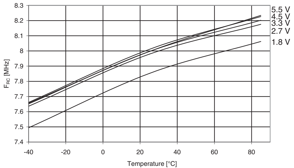
Figure 29-171. ATmega329A: Calibrated 8 MHz RC Oscillator Frequency vs. Temperature
