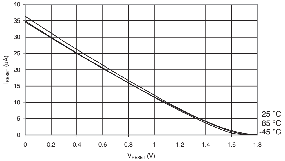
Figure 29-21. ATmega169A: Reset Pull-up Resistor Current vs. Reset Pin Voltage ( V_{CC} = 1.8V )
