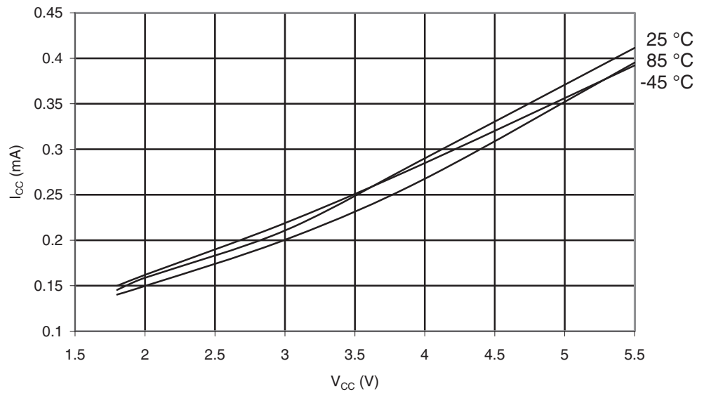
Figure 29-368. ATmega649A: Active Supply Current vs. V_{CC} (Internal RC Oscillator, 1 MHz)
