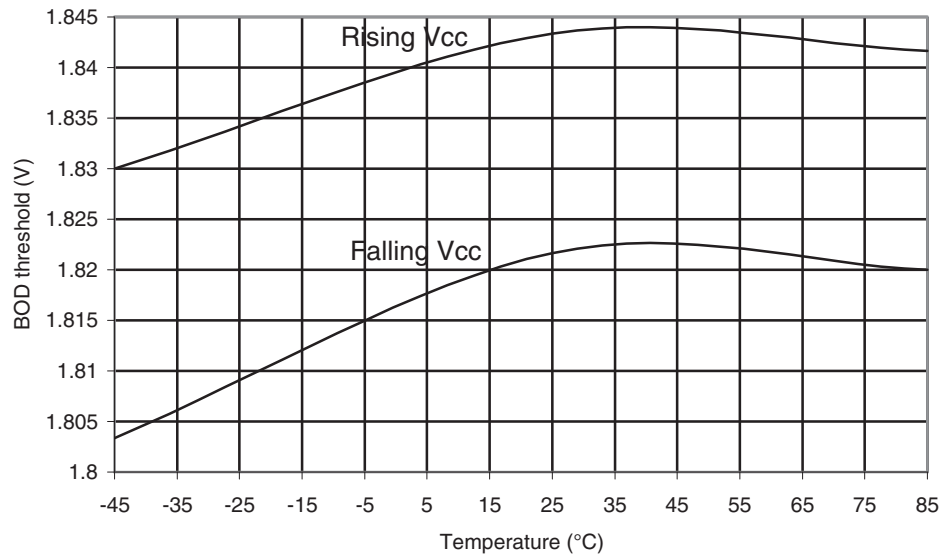
Figure 29-407. ATmega649A: BOD Thresholds vs. Temperature (BOD Level is 1.8V)
