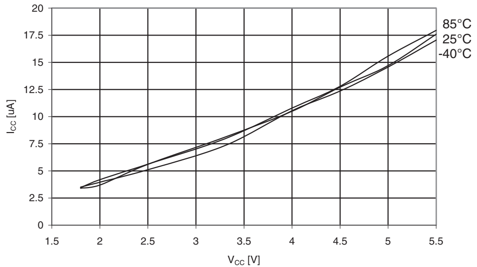
Figure 29-239. ATmega329PA: Watchdog Timer Current vs. V_{CC}
