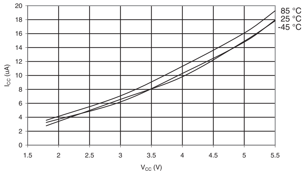
Figure 29-12. ATmega169A: Power-down Supply Current vs. V_{CC} (Watchdog Timer Enabled)
