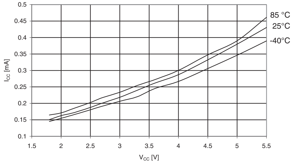
Figure 29-313. ATmega3290PA: Idle Supply Current vs. V_{CC} (Internal RC Oscillator, 1 MHz)
