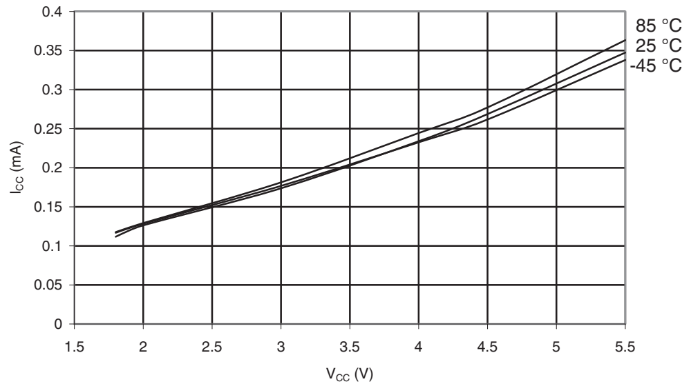
Figure 29-9. ATmega169A: Idle Supply Current vs. V_{CC} (Internal RC Oscillator, 1 MHz)
