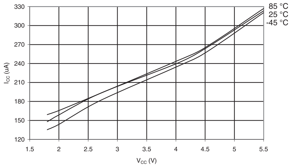
Figure 29-416. ATmega649A: Active Supply Current with ADC at 50 kHz vs. V_{CC}
