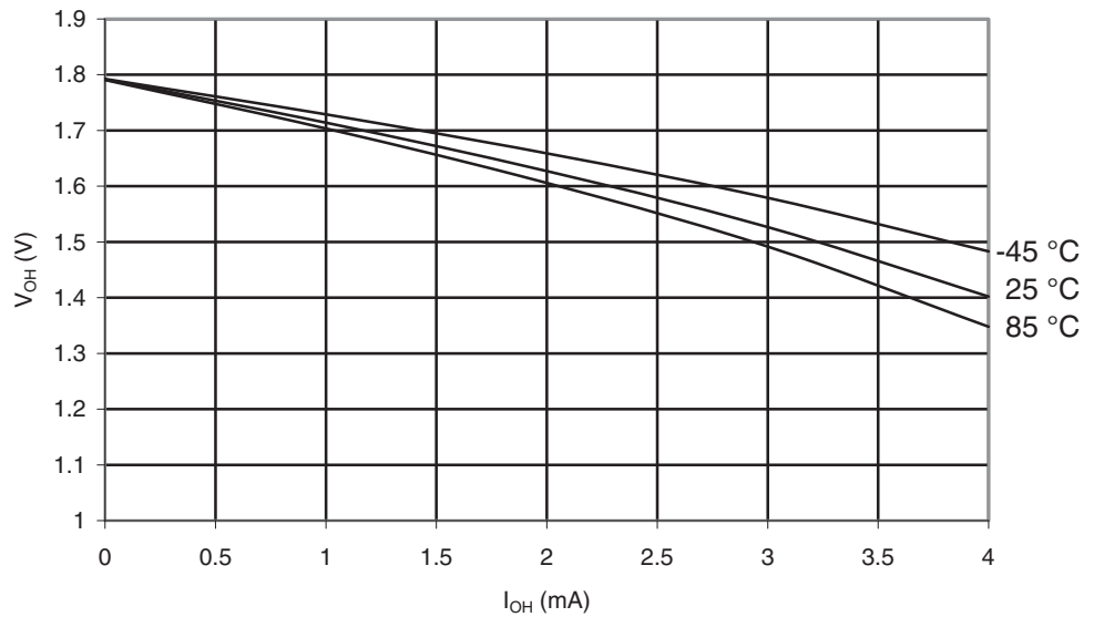
Figure 29-86. ATmega169PA: I/O Pin Output Voltage vs. Source Current, Ports A, C, D, E, F, G ( V_{CC} = 1.8V )
