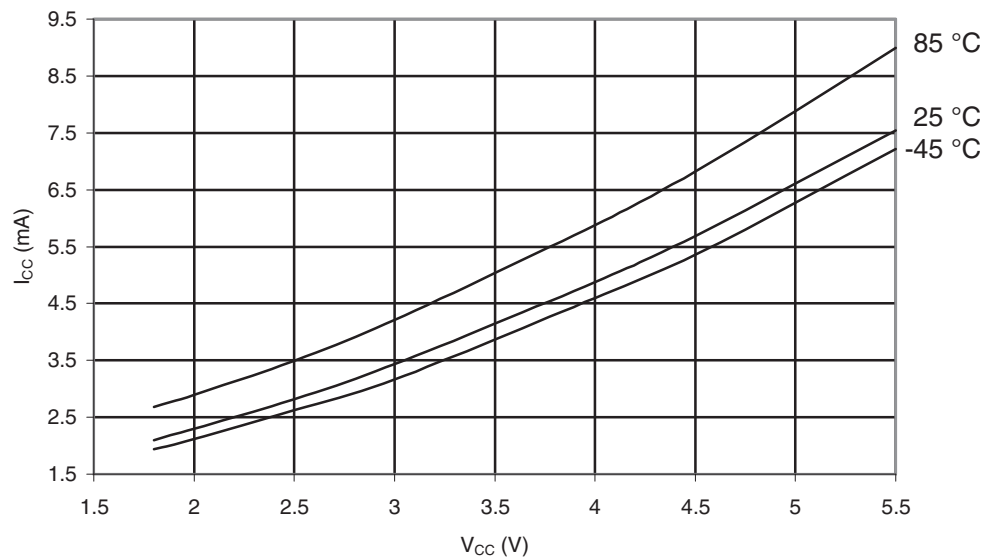
Figure 29-557. ATmega6490P: Idle Supply Current vs. V_{CC} (32 kHz Watch Crystal)
