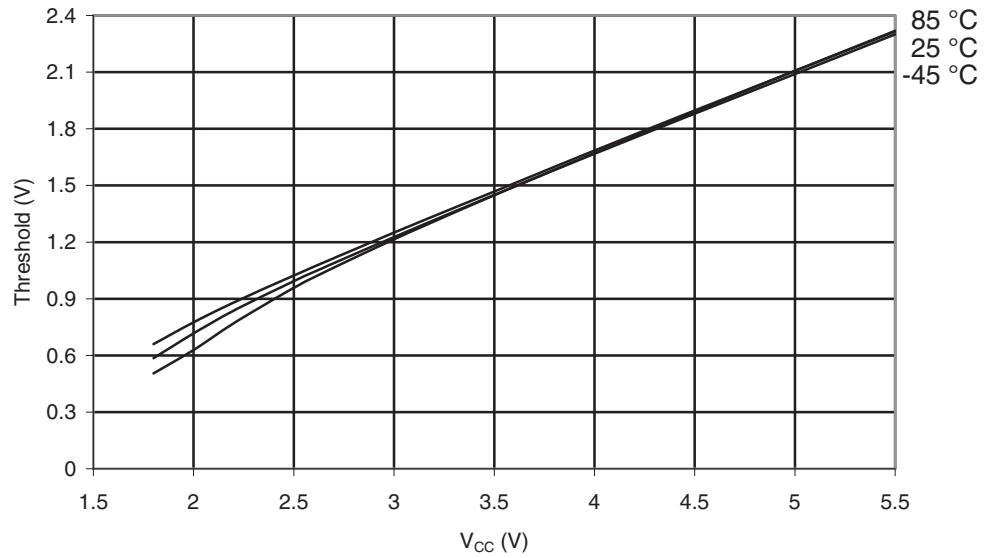
Figure 29-35. ATmega169A: I/O Pin Input Threshold Voltage vs. V_{CC} ( V_{IL} , I/O Pin Read as "0")
