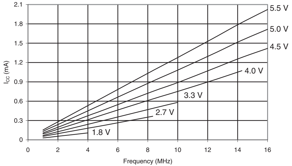
Figure 29-61. ATmega169A: Reset Supply Current vs. V_{CC} (1 - 16 MHz, Excluding Current Through The Reset Pull-up)
