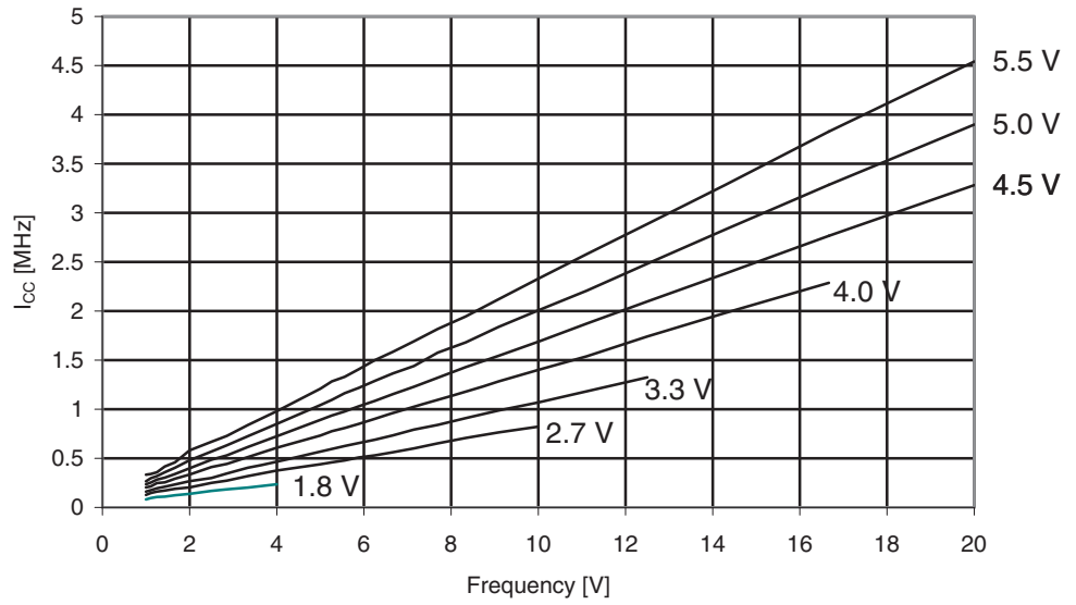
Figure 29-191. ATmega329PA: Idle Supply Current vs. Frequency (1 - 20MHz)
