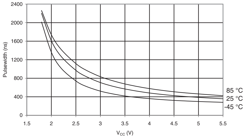
Figure 29-62. ATmega169A: Minimum Reset Pulse Width vs. V_{CC}
