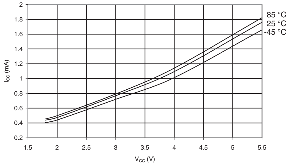
Figure 29-494. ATmega6490A: Idle Supply Current vs. V_{CC} (Internal RC Oscillator, 8 MHz)
