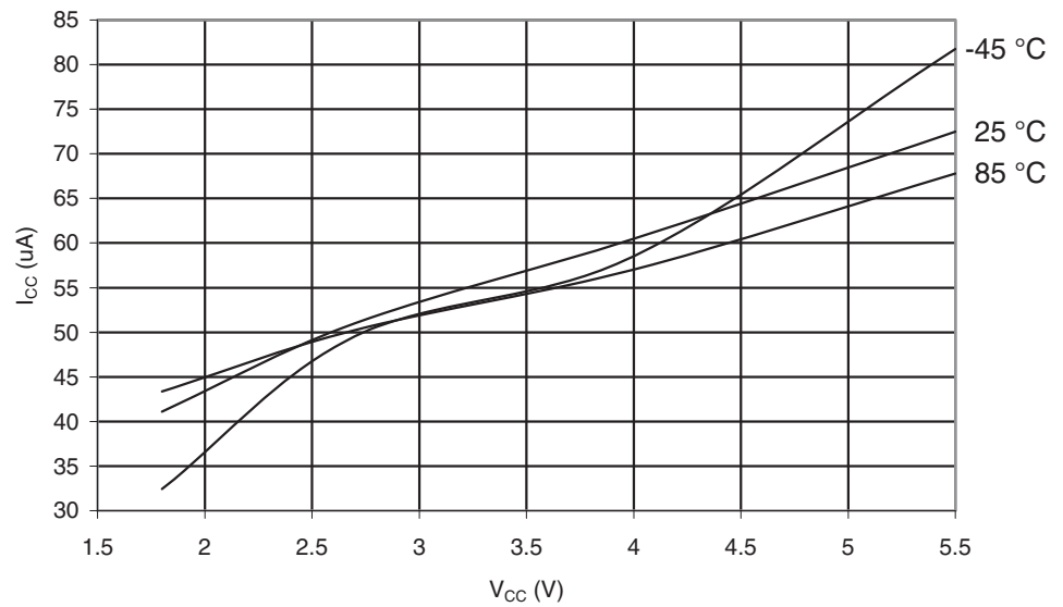
Figure 29-120. ATmega169PA: Analog Comparator Current vs. V_{CC}
