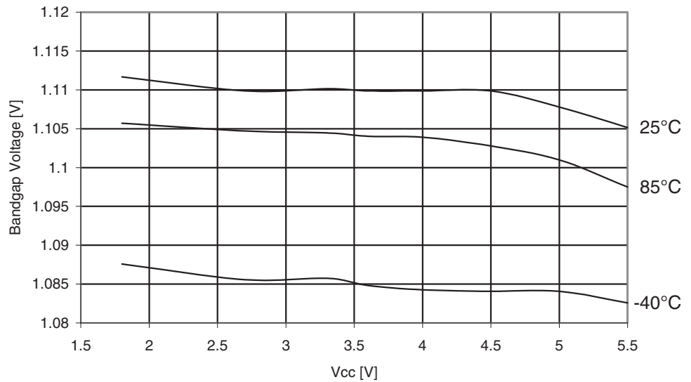
Figure 29-347. ATmega3290PA: Bandgap Voltage vs. V CC
