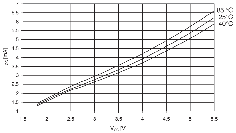
Figure 29-187. ATmega329PA: Active Supply Current vs. V_{CC} (Internal RC Oscillator, 8 MHz)
