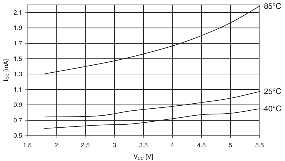
Figure 29-258. ATmega3290A: Standby Supply Current vs. V_{CC} (32 kHz Watch Crystal, Watchdog Timer Disabled)
