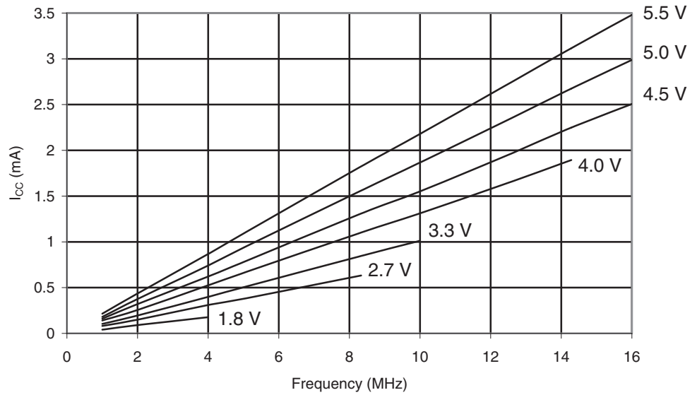
Figure 29-7. ATmega169A: Idle Supply Current vs. Frequency (1 - 16 MHz)
