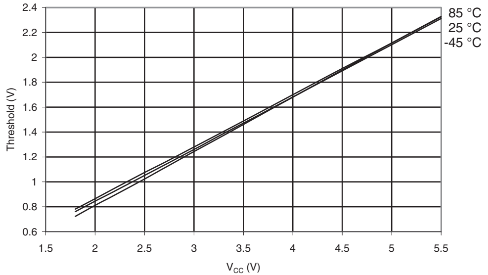
Figure 29-100. ATmega169PA: Reset Input Threshold Voltage vs. V_{CC} ( V_{IL} , Reset Pin Read as "0")
