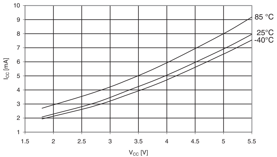
Figure 29-254. ATmega3290A: Idle Supply Current vs. V_{CC} (32 kHz Watch Crystal)
