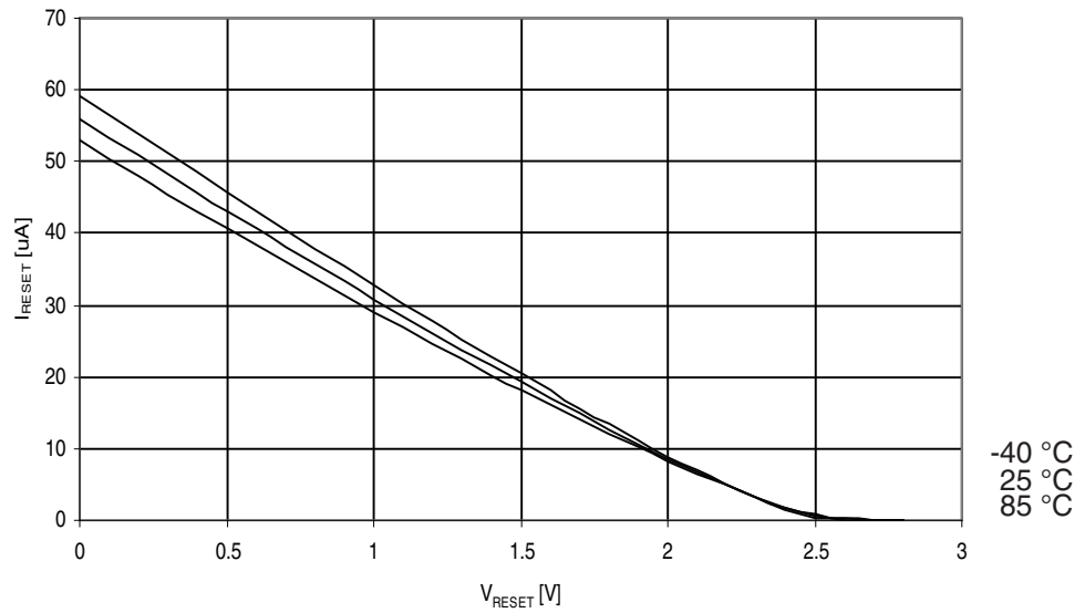
Figure 29-144. ATmega329A: Reset Pull-up Resistor Current vs. Reset Pin Voltage ( V_{CC} = 2.7V )
