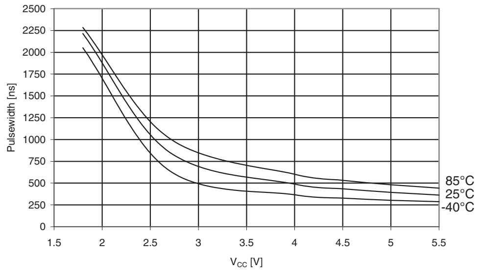
Figure 29-364. ATmega3290PA: Minimum Reset Pulse Width vs. V_{CC}
