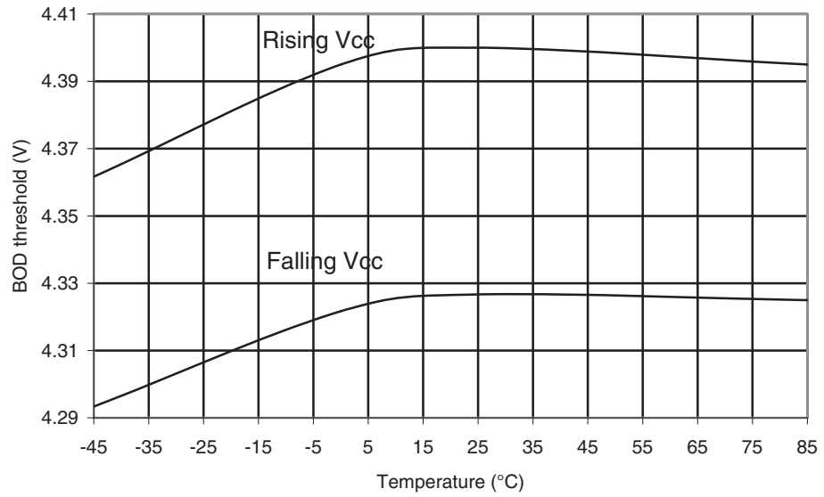
Figure 29-466. ATmega649P: BOD Thresholds vs. Temperature (BOD Level is 4.3V)
