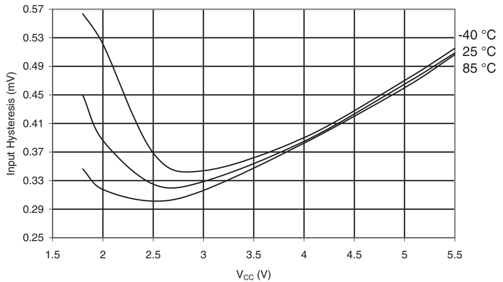
Figure 29-280. ATmega3290A: I/O Pin Input Hysteresis vs. V_{CC}
