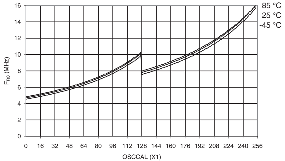
Figure 29-51. ATmega169A: Calibrated 8 MHz RC Oscillator Frequency vs. Oscal Value
