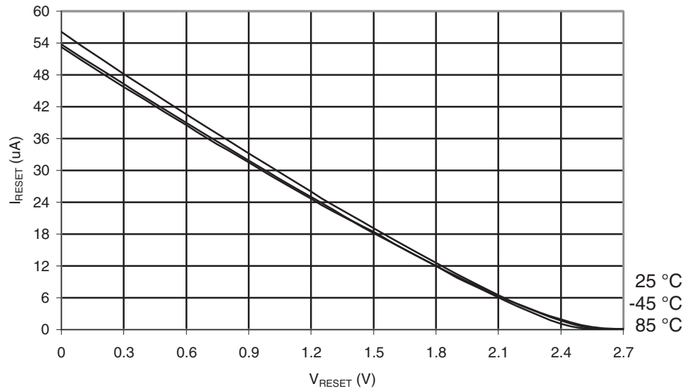
Figure 29-507. ATmega6490A: Reset Pull-up Resistor Current vs. Reset Pin Voltage ( V_{CC} = 2.7V )
