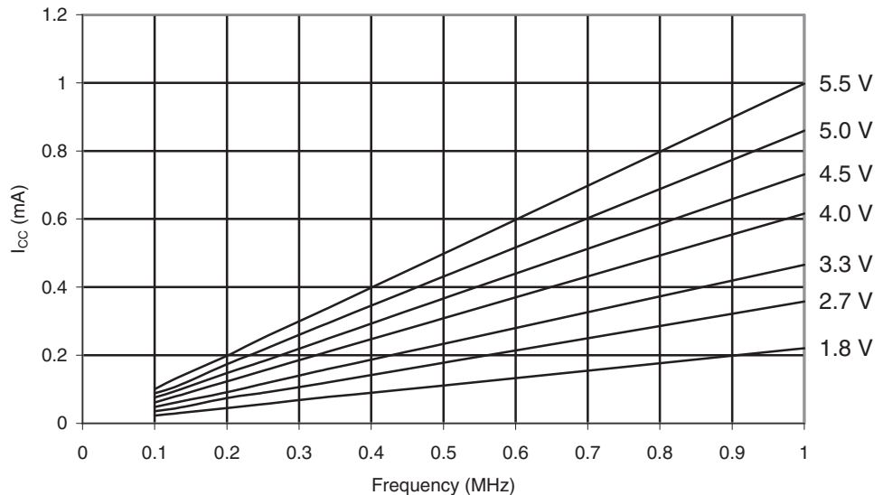
Figure 29-1. ATmega169A: Active Supply Current vs. Low Frequency (0.1 - 1.0 MHz)
