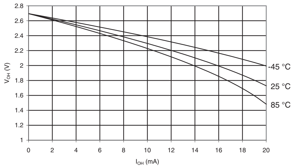
Figure 29-88. ATmega169PA: I/O Pin Output Voltage vs. Source Current, Port B ( V_{CC}=2.7V )
