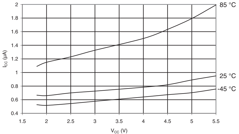
Figure 29-14. ATmega169A Standby Supply Current vs. V_{CC} (32 kHz Watch Crystal, Watchdog Timer Disabled)
