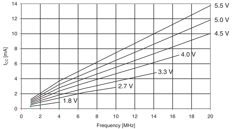
Figure 29-246. ATmega3290A: Active Supply Current vs. Frequency (1 - 20MHz)
