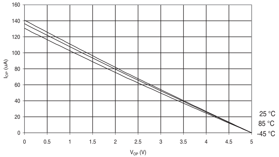
Figure 29-503. ATmega6490A: I/O Pin Pull-up Resistor Current vs. Input Voltage ( V_{CC} = 5V )
