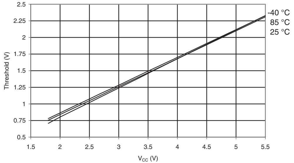
Figure 29-162. ATmega329A: Reset Input Threshold Voltage vs. V_{CC} ( V_{IL} , Reset Pin Read as "0")
