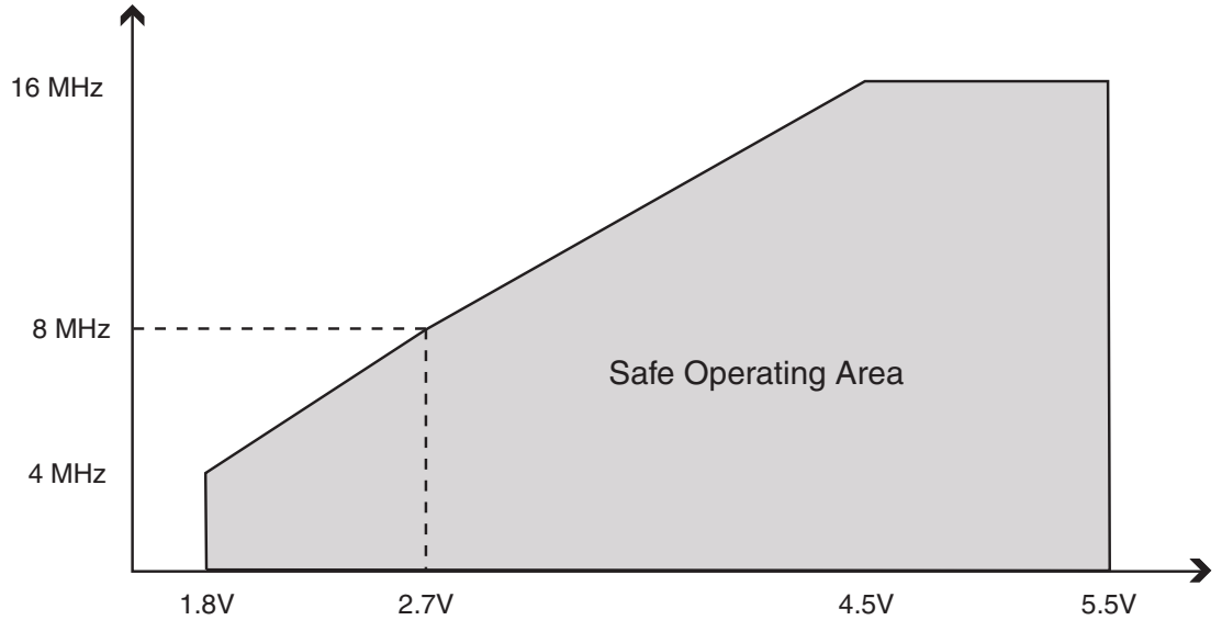
Figure 28-1. Maximum Frequency vs. V_{CC} , ATmega169A/169PA/ATmega649A/ATmega649P
