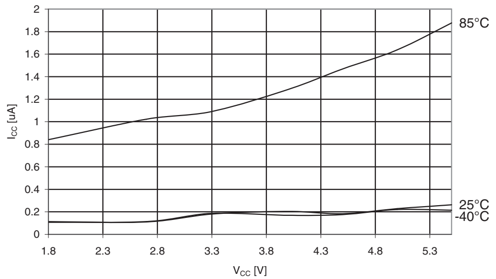
Figure 29-136. ATmega329A: Power-down Supply Current vs. V_{CC} (Watchdog Timer Enabled)
