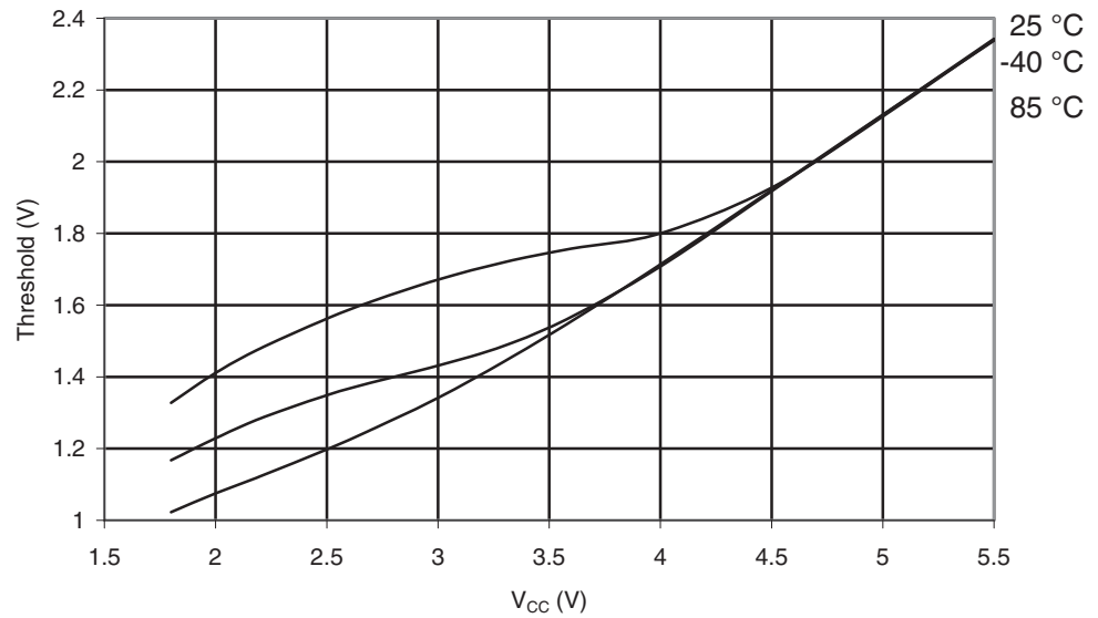
Figure 29-161. ATmega329A: Reset Input Threshold Voltage vs. V_{CC} ( V_{IH,Reset} , Reset Pin Read as "1")
