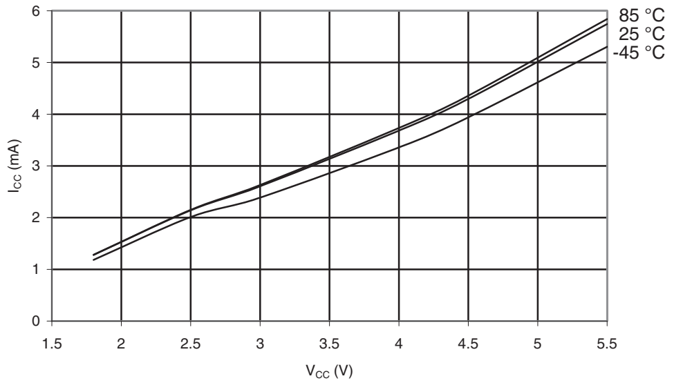
Figure 29-65. ATmega169PA: Active Supply Current vs. V_{CC} (Internal RC Oscillator, 8 MHz)
