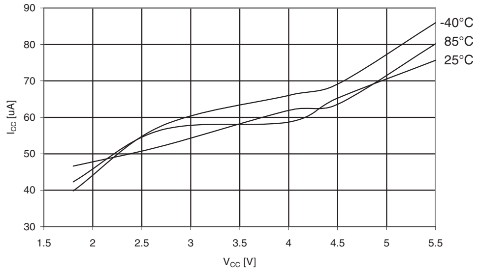
Figure 29-180. ATmega329A: Analog Comparator Current vs. V_{CC}
