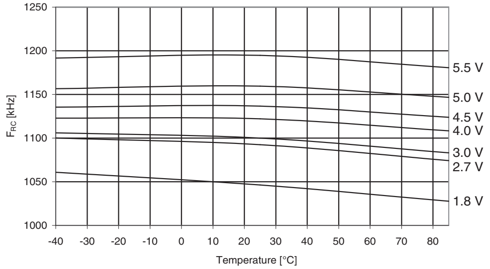
Figure 29-350. ATmega3290PA: Watchdog Oscillator Frequency vs. Temperature
