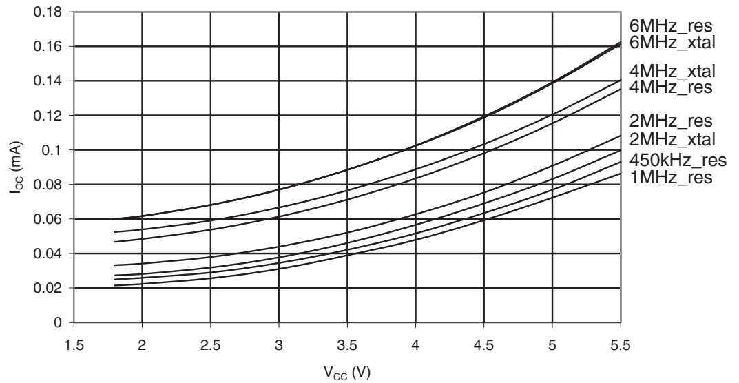
Figure 29-77. ATmega169PA: Standby Supply Current vs. V_{CC} (Xtall and Resonator, Watchdog Timer Disabled)
