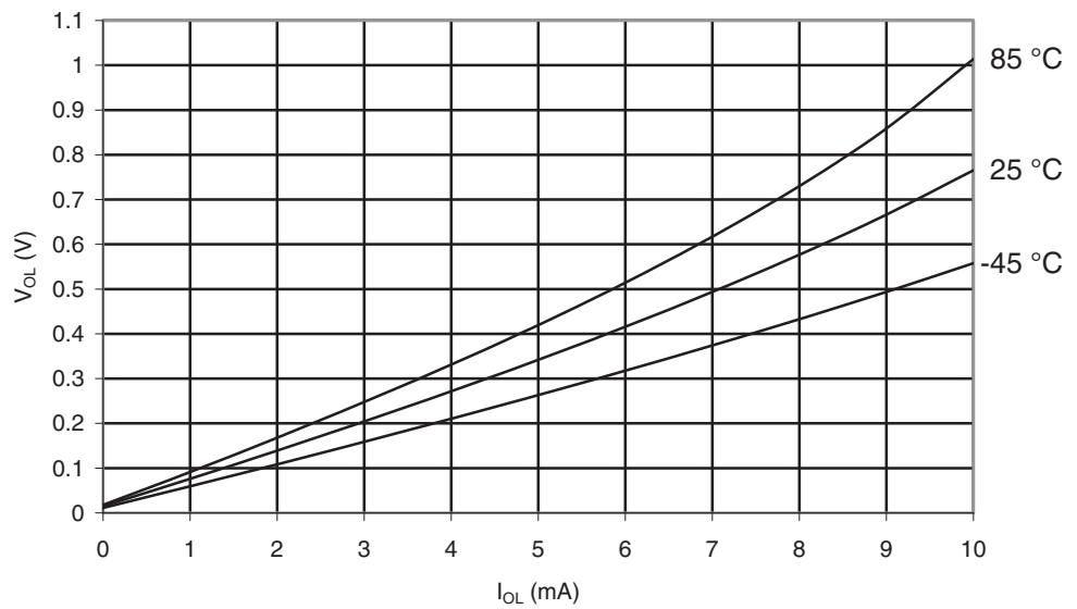
Figure 29-90. ATmega169PA: I/O Pin Output Voltage vs. Sink Current, Ports A, C, D, E, F, G ( V_{CC} = 5V )
