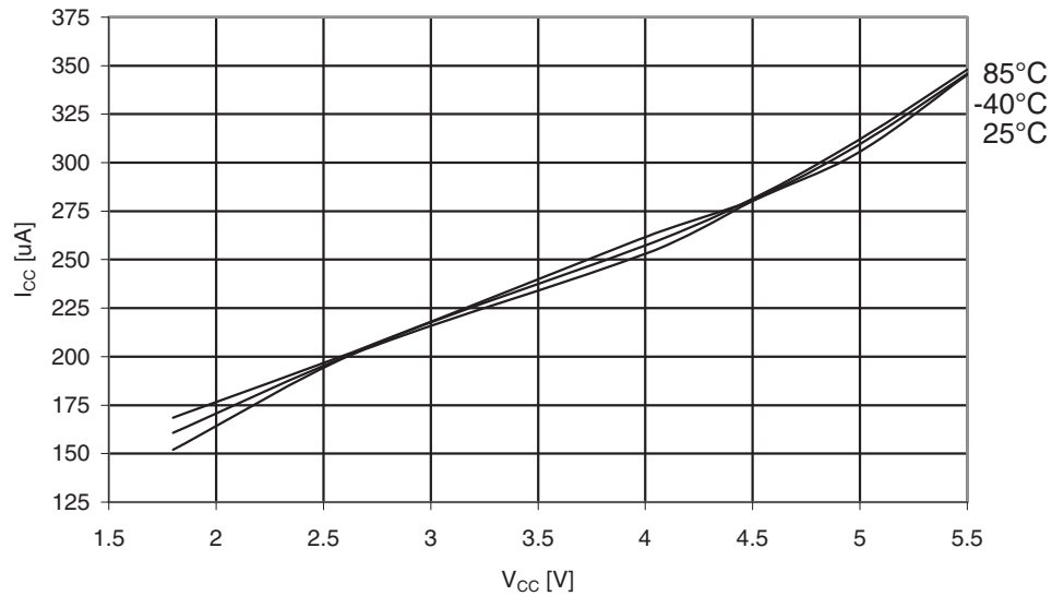
Figure 29-296. ATmega3290A: Active Supply Current with ADC at 200 kHz vs. V_{CC}
