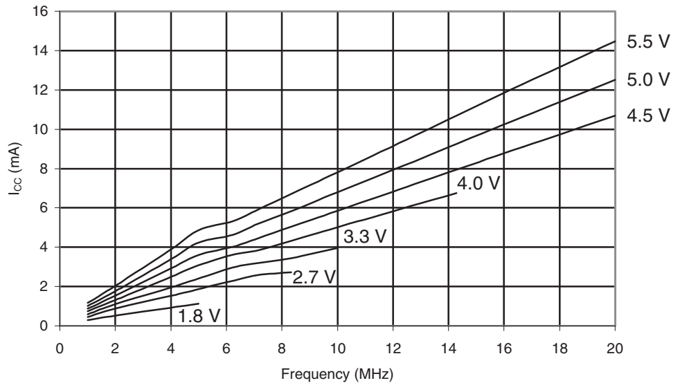
Figure 29-366. ATmega649A: Active Supply Current vs. Frequency (1 - 20 MHz)
