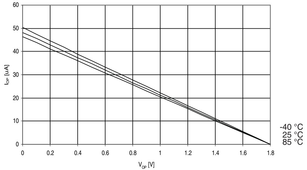
Figure 29-202. ATmega329PA: I/O Pin Pull-up Resistor Current vs. Input Voltage ( V_{CC} = 1.8V )
