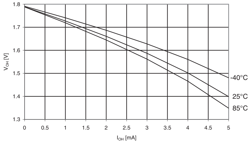
Figure 29-211. ATmega329PA: I/O Pin Output Voltage vs. Source Current, Port B ( V_{CC} = 1.8V )
