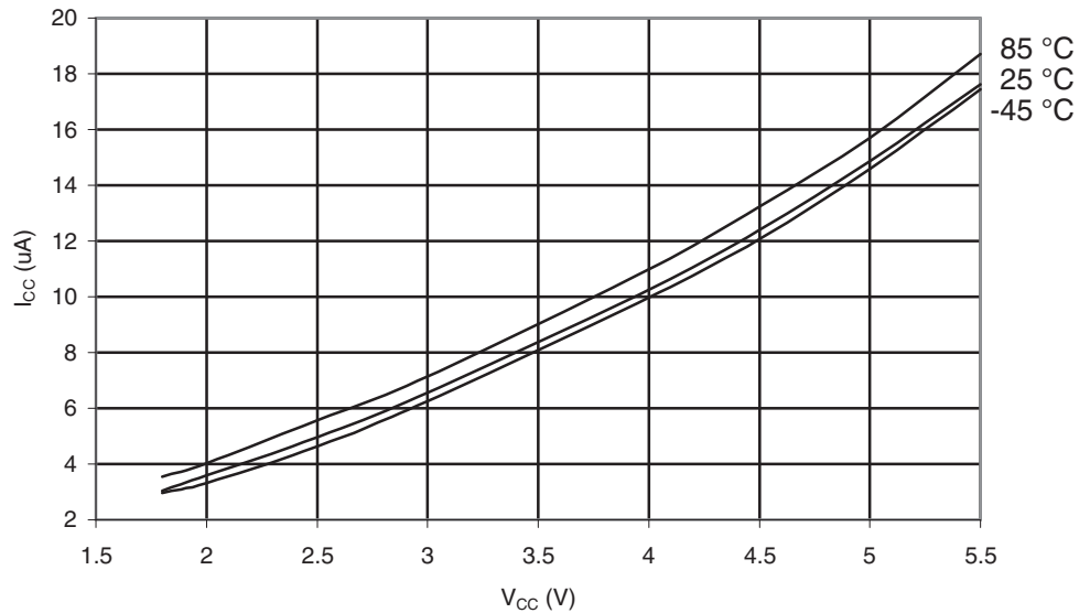
Figure 29-376. ATmega649A: Power-down Supply Current vs. V_{CC} (Watchdog Timer Enabled)
