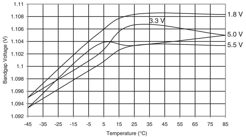
Figure 29-592. ATmega6490P: Bandgap Voltage vs. Temperature
