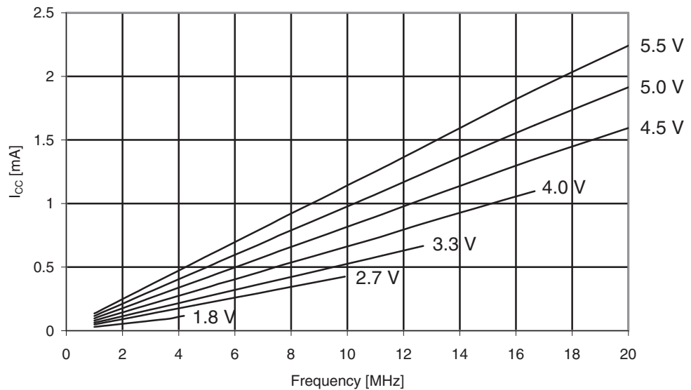
Figure 29-363. ATmega3290PA: Reset Supply Current vs. V_{CC} (1 - 20MHz, Excluding Current Through The Reset Pull-up)
