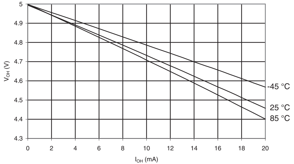
Figure 29-390. ATmega649A: I/O Pin Output Voltage vs. Source Current, Port B ( V_{CC} = 5V )
