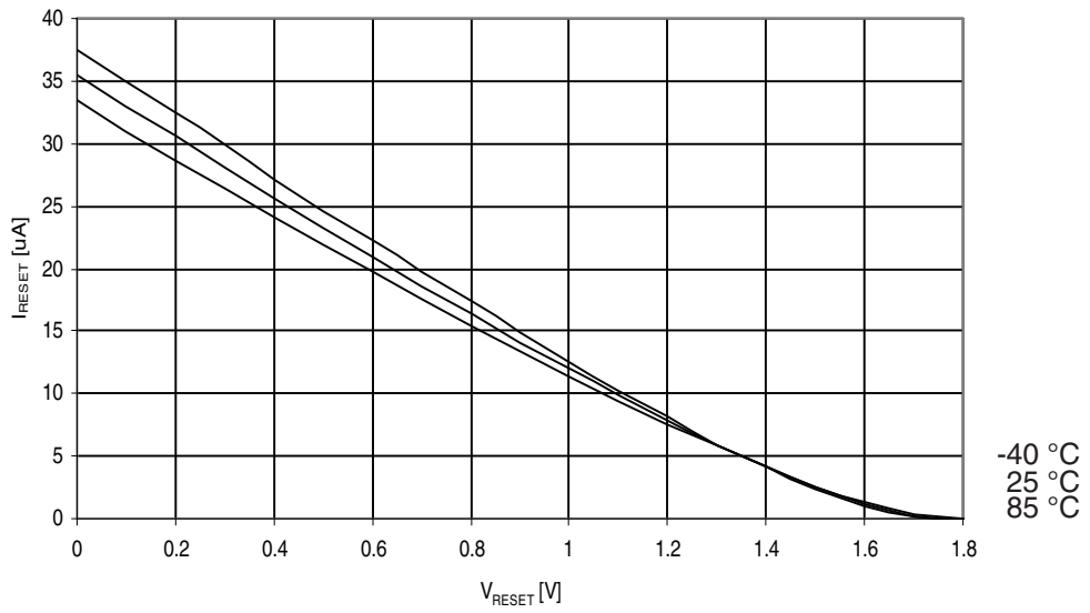
Figure 29-205. ATmega329PA: Reset Pull-up Resistor Current vs. Reset Pin Voltage ( V_{CC} = 1.8V )
