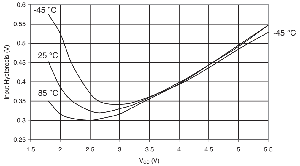
Figure 29-401. ATmega649A: I/O Pin Input Hysteresis vs. V_{CC}
