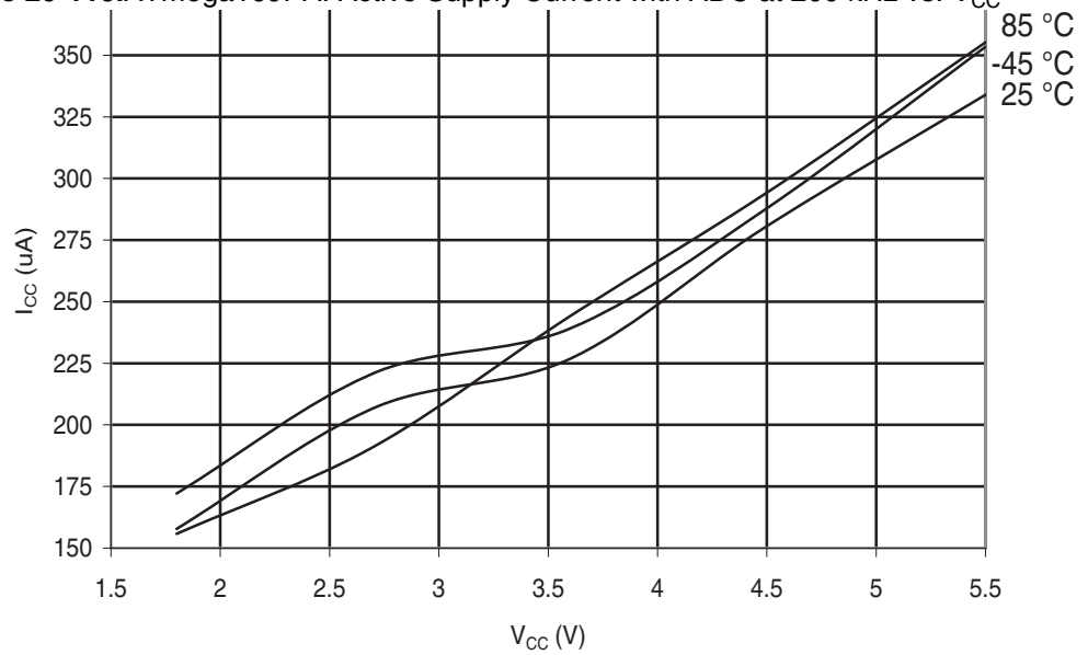
Figure 29-116. ATmega169PA: Active Supply Current with ADC at 200 kHz vs. V_{CC}
