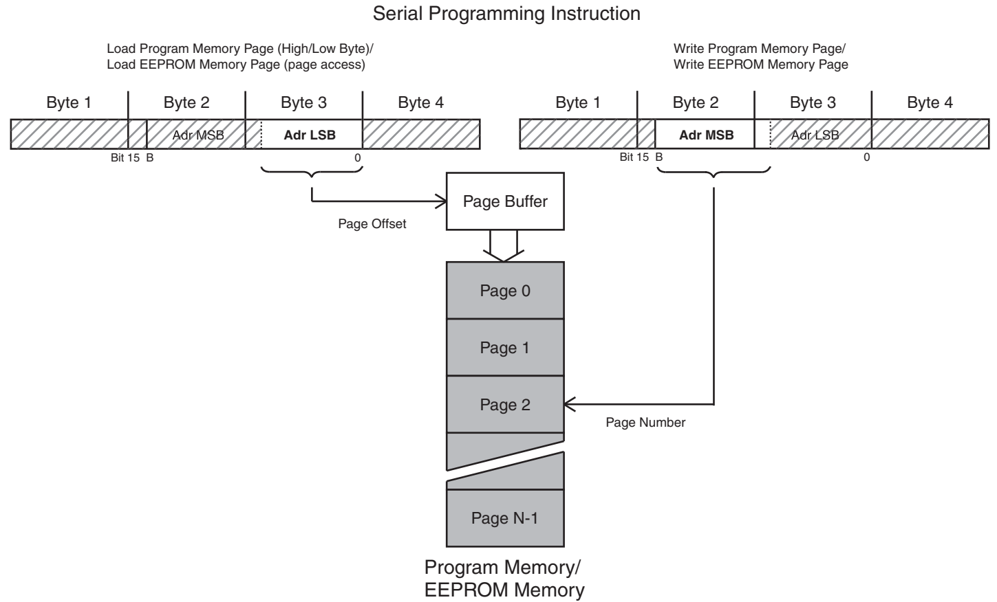
Figure 27-12. Serial Programming Instruction example
