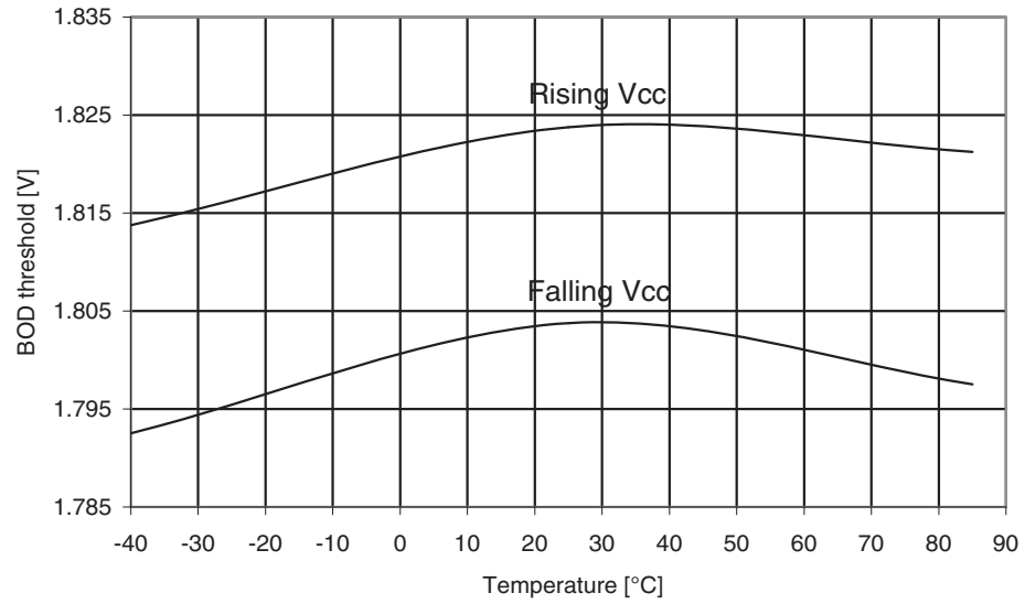
Figure 29-166. ATmega329A: BOD Thresholds vs. Temperature (BOD Level is 1.8V)
