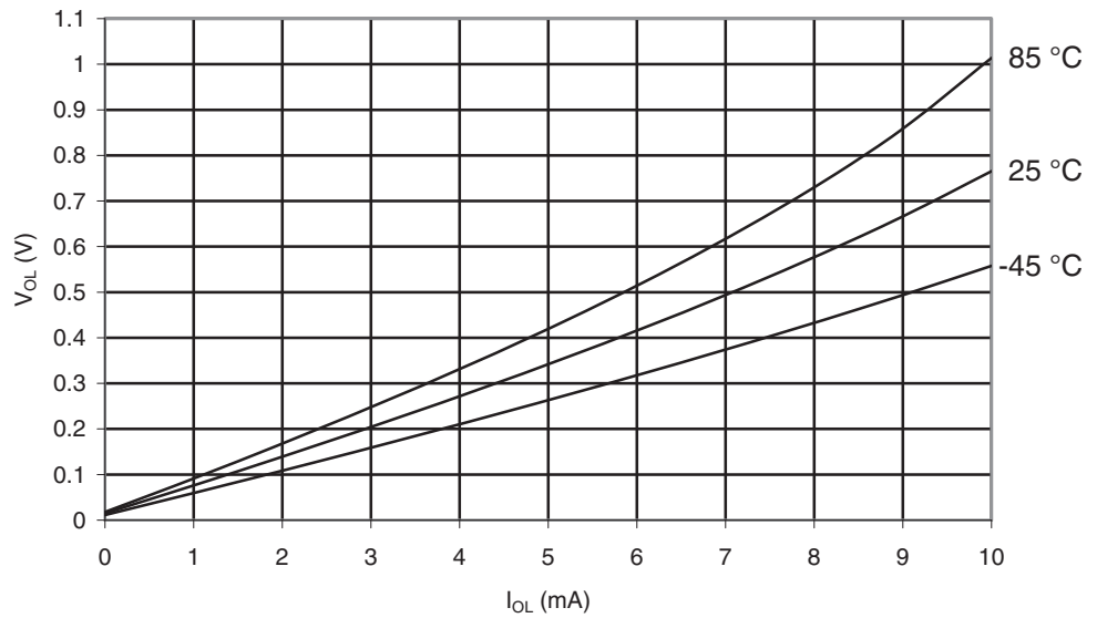
Figure 29-28. ATmega169A: I/O Pin Output Voltage vs. Sink Current, Ports A, C, D, E, F, G ( V_{CC} = 5V )
