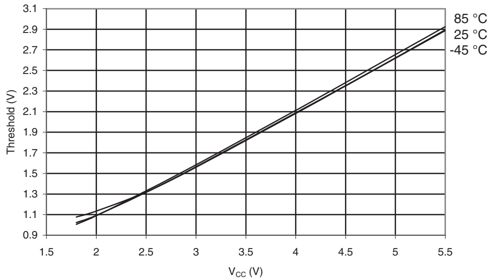
Figure 29-521. ATmega6490A: I/O Pin Input Threshold Voltage vs. V_{CC} ( V_{IH} , I/O Pin Read as "1")
