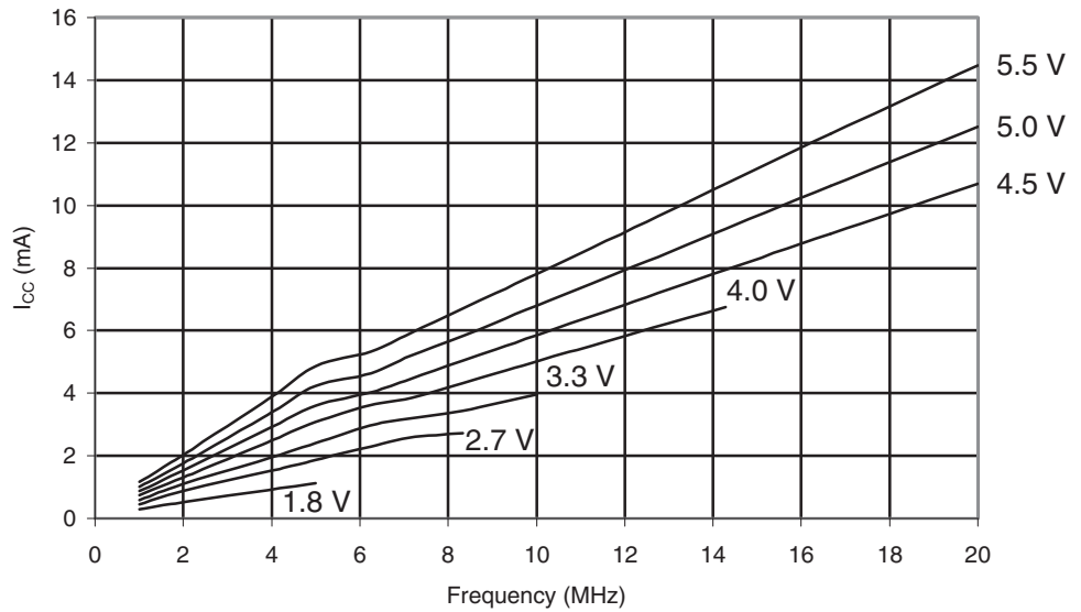
Figure 29-427. ATmega649P: Active Supply Current vs. Frequency (1 - 16 MHz)
