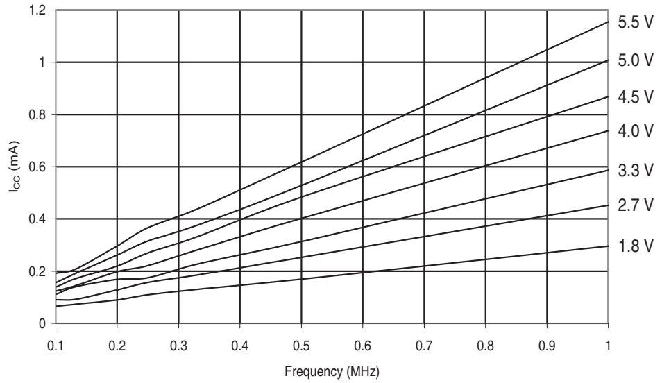
Figure 29-426. ATmega649P: Active Supply Current vs. Low Frequency (0.1 - 1.0 MHz)
