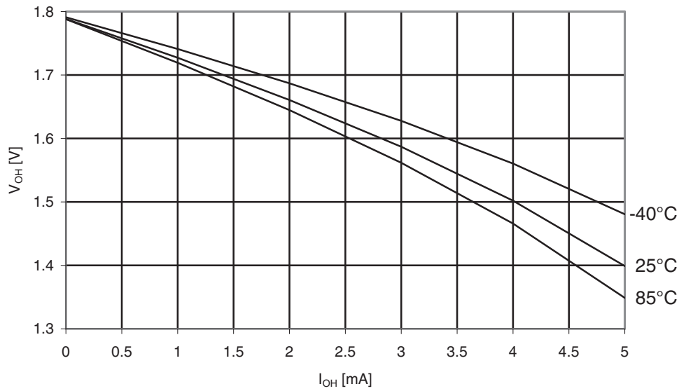
Figure 29-271. ATmega3290A: I/O Pin Output Voltage vs. Source Current, Port B ( V_{CC} = 1.8V )
