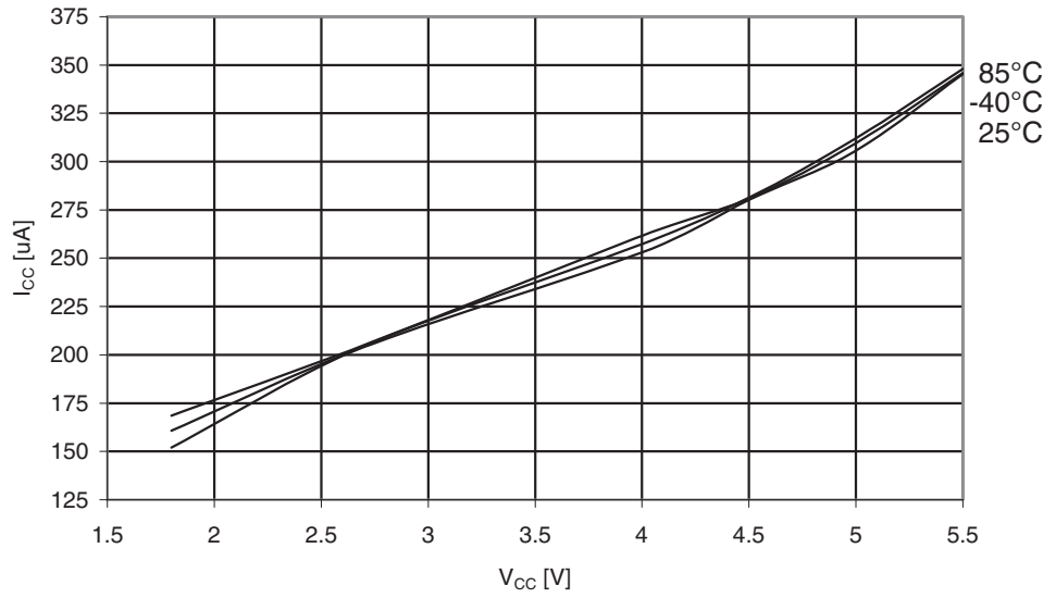
Figure 29-356. ATmega3290PA: Active Supply Current with ADC at 200 kHz vs. V_{CC}
