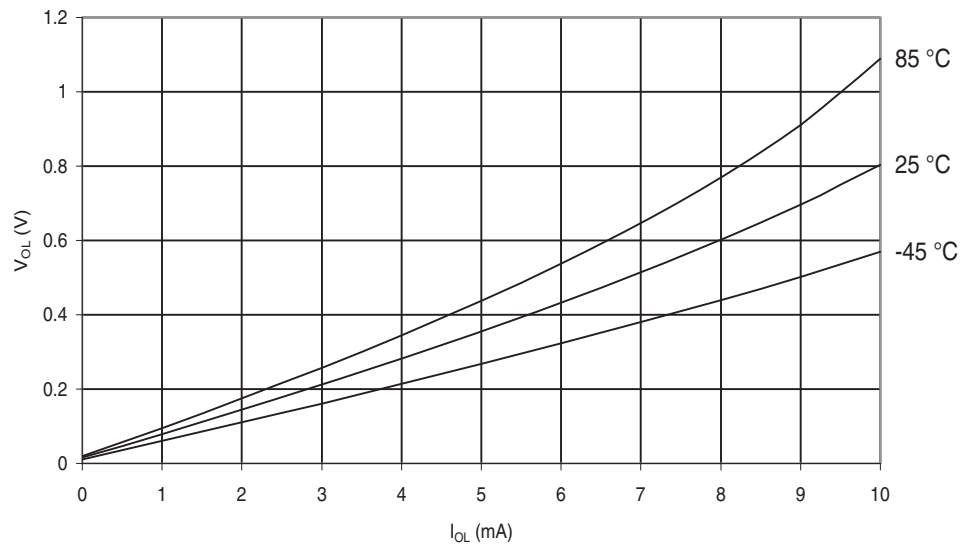
Figure 29-577. ATmega6490P: I/O Pin Output Voltage vs. Sink Current, Ports A, C, D, E, F, G ( V_{CC} = 2.7V )
