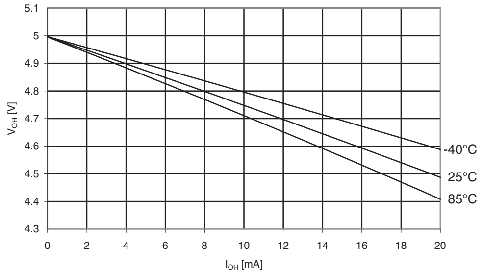
Figure 29-149. ATmega329A: I/O Pin Output Voltage vs. Source Current, Port B ( V_{CC} = 5V )
