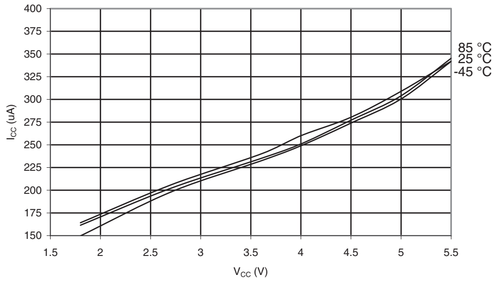
Figure 29-53. ATmega169A: Active Supply Current with ADC at 50 kHz vs. V_{CC}
