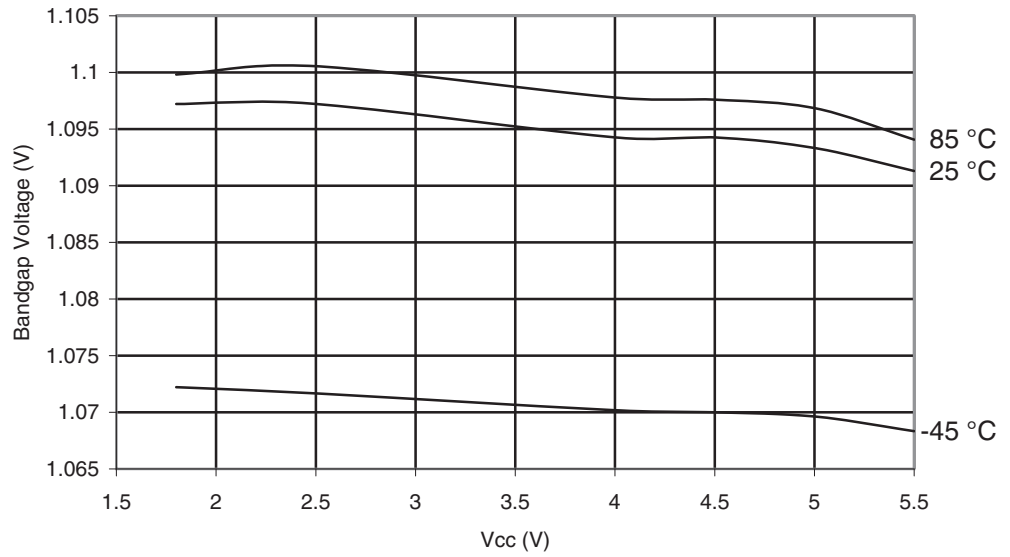
Figure 29-105. ATmega169PA: Bandgap Voltage vs. V_{CC}
