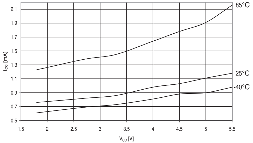
Figure 29-137. ATmega329A: Power-save Supply Current vs. V_{CC} (Watchdog Timer Disabled and 32 kHz Crystal Oscillator Running)
