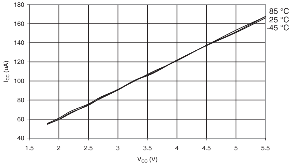
Figure 29-118. ATmega169PA: AREF External Reference Current vs. V_{CC}
