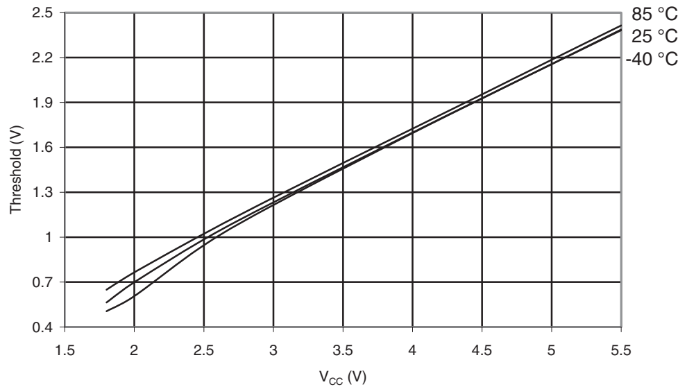
Figure 29-219. ATmega329PA: I/O Pin Input Threshold Voltage vs. V_{CC} ( V_{IL} , I/O Pin Read as "0")
