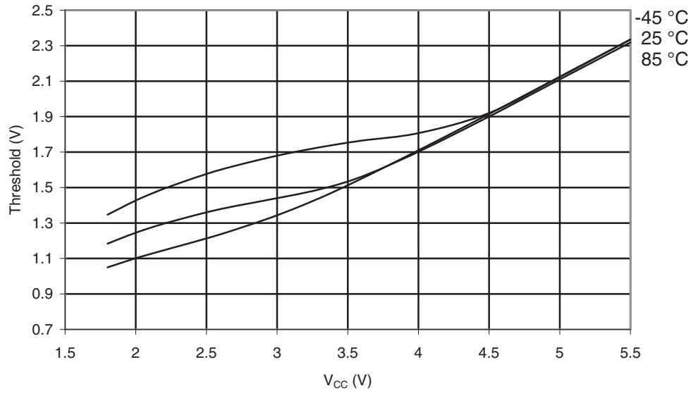
Figure 29-99. ATmega169PA: Reset Input Threshold Voltage vs. V_{CC} ( V_{IH} , Reset Pin Read as "1")
