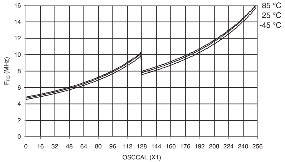
Figure 29-113. ATmega169PA: Calibrated 8 MHz RC Oscillator Frequency vs. Oscal Value
