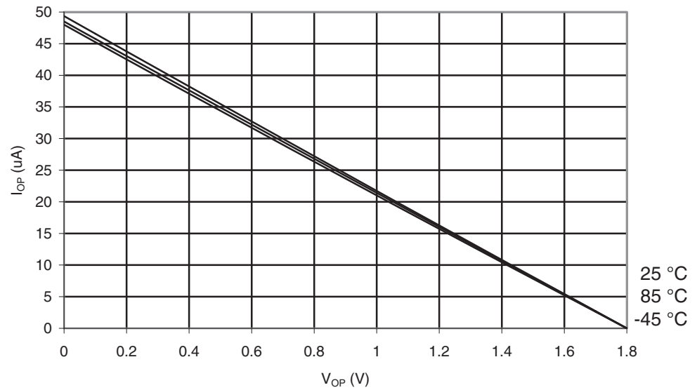
Figure 29-80. ATmega169PA: I/O Pin Pull-up Resistor Current vs. Input Voltage ( V_{CC} = 1.8V )
