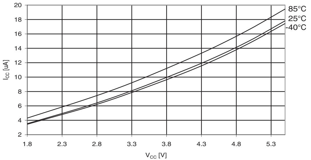
Figure 29-316. ATmega3290PA: Power-down Supply Current vs. V_{CC} (Watchdog Timer Enabled)
