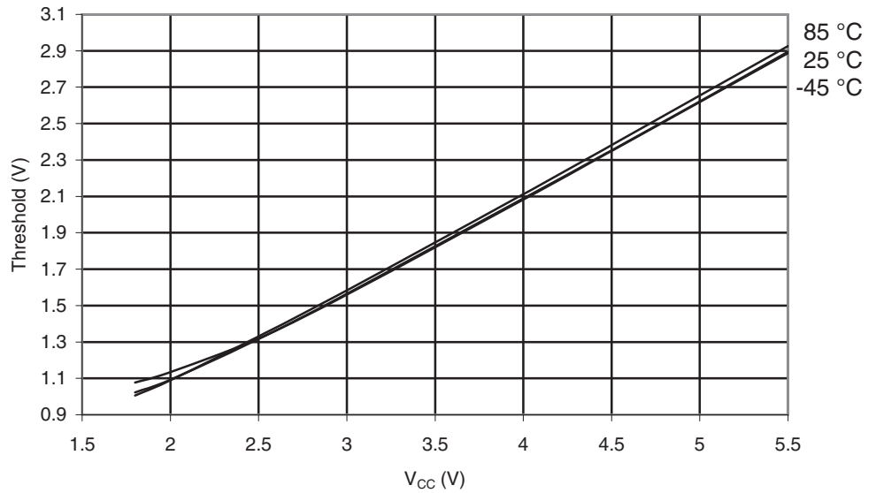
Figure 29-399. ATmega649A: I/O Pin Input Threshold Voltage vs. V_{CC} ( V_{IH} , I/O Pin Read as "1")
