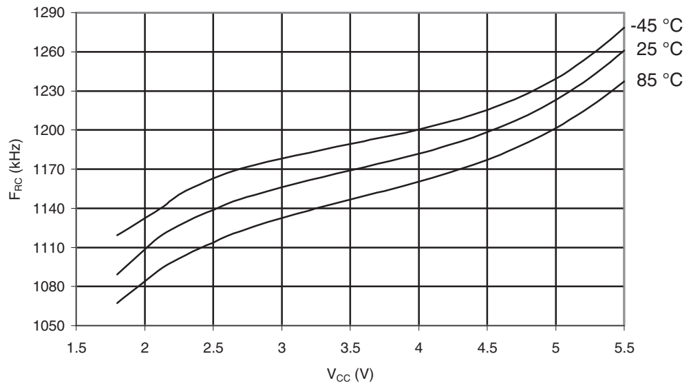
Figure 29-593. ATmega6490P: Watchdog Oscillator Frequency vs. V CC
