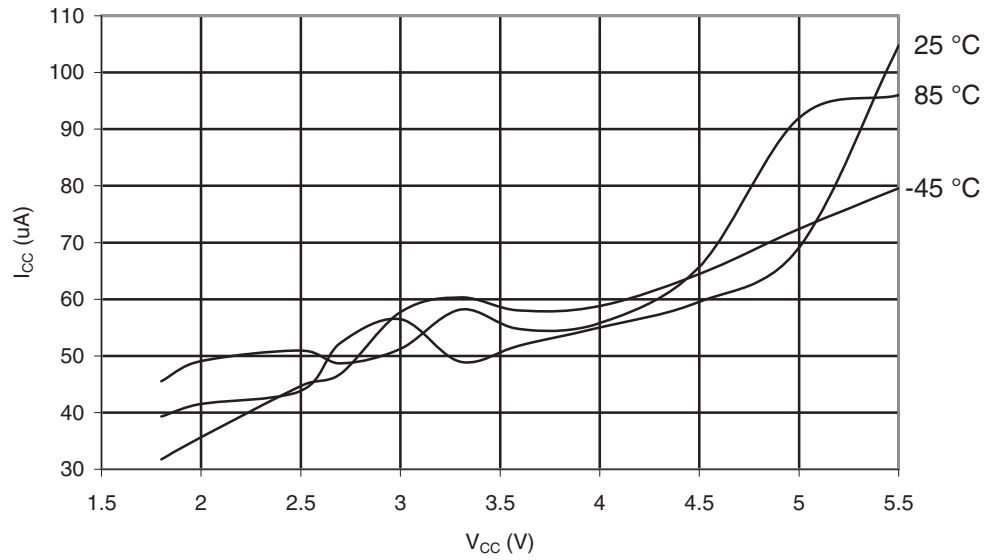
Figure 29-543. ATmega6490A: Analog Comparator Current vs. V_{CC}
