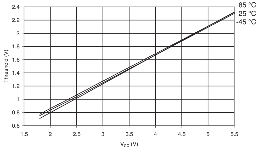
Figure 29-403. ATmega649A: Reset Input Threshold Voltage vs. V_{CC} ( V_{IL} , Reset Pin Read as "0")
