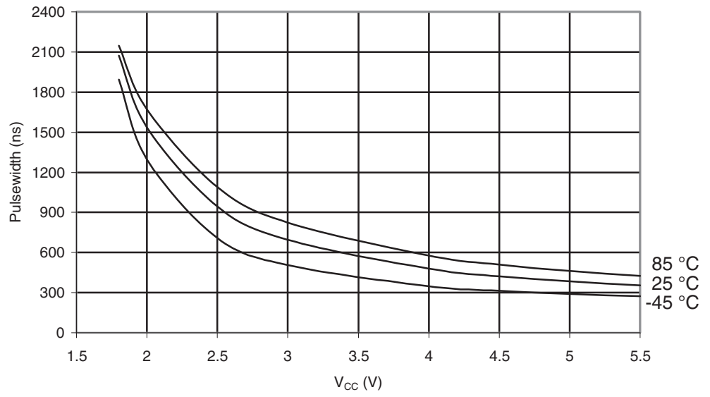
Figure 29-547. ATmega6490A: Minimum Reset Pulse Width vs. V_{CC}
