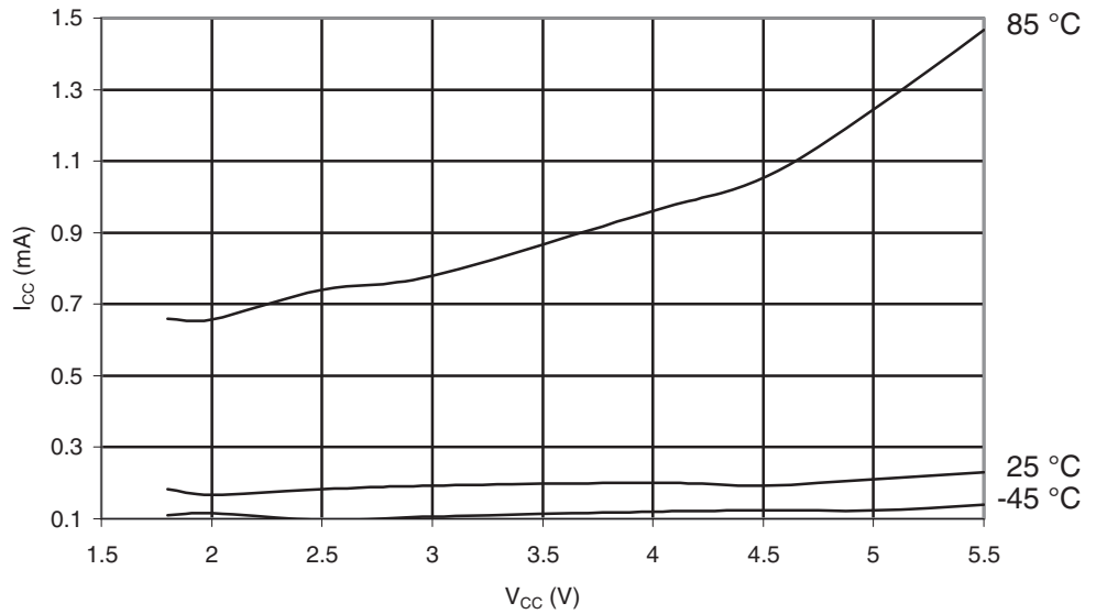
Figure 29-377. ATmega649A: Power-down Supply Current vs. V_{CC} (32 kHz Watch Crystal)
