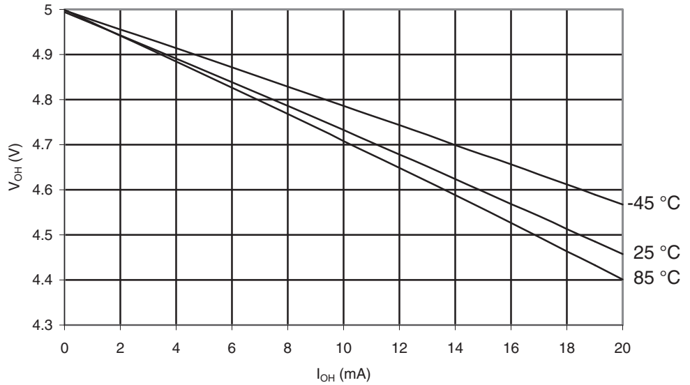
Figure 29-512. ATmega6490A: I/O Pin Output Voltage vs. Source Current, Port B ( V_{CC} = 5V )
