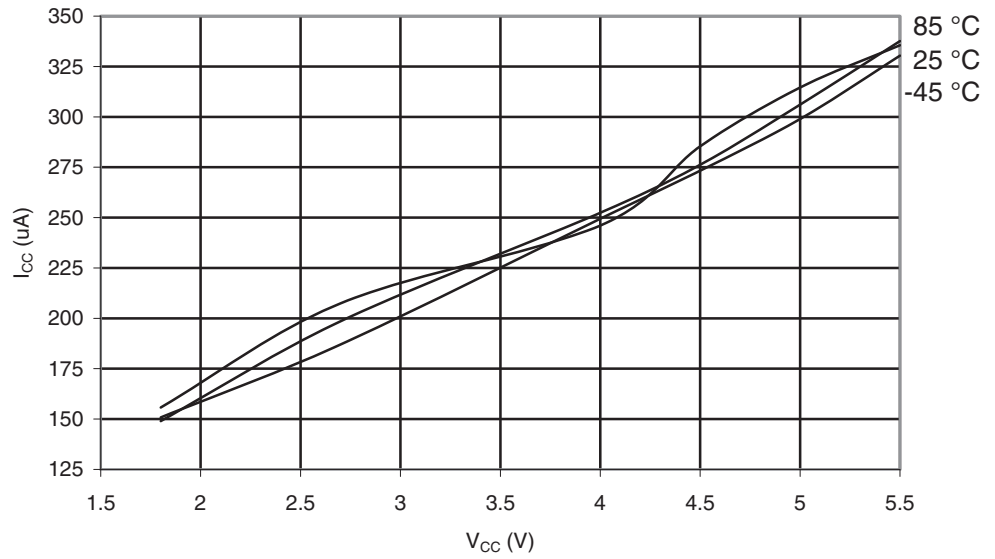
Figure 29-117. ATmega169PA: Active Supply Current with ADC at 1 MHz vs. V_{CC}
