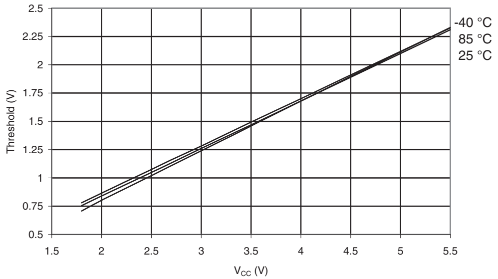
Figure 29-342. ATmega3290PA: Reset Input Threshold Voltage vs. V_{CC} ( V_{IL} , Reset Pin Read as "0")
