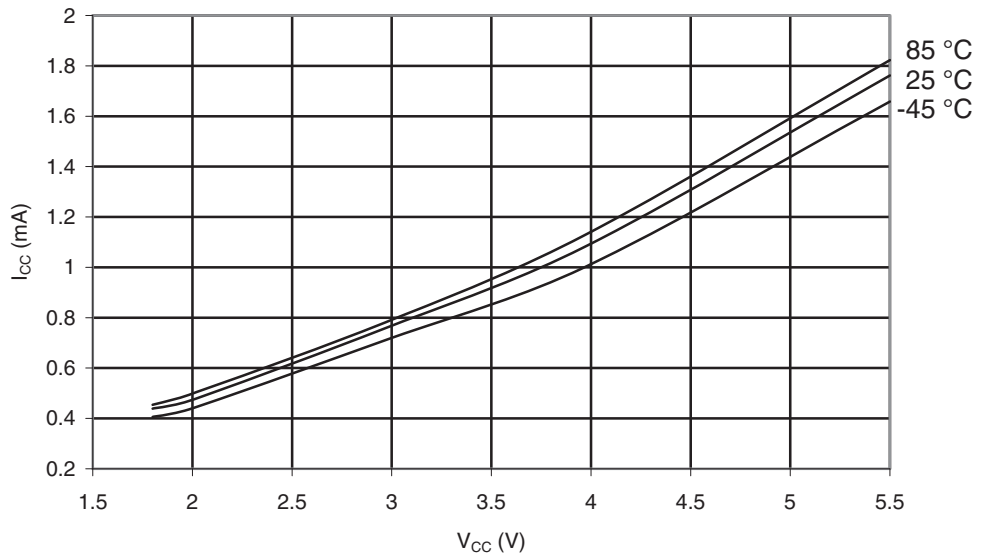
Figure 29-372. ATmega649A: Idle Supply Current vs. V_{CC} (Internal RC Oscillator, 8 MHz)
