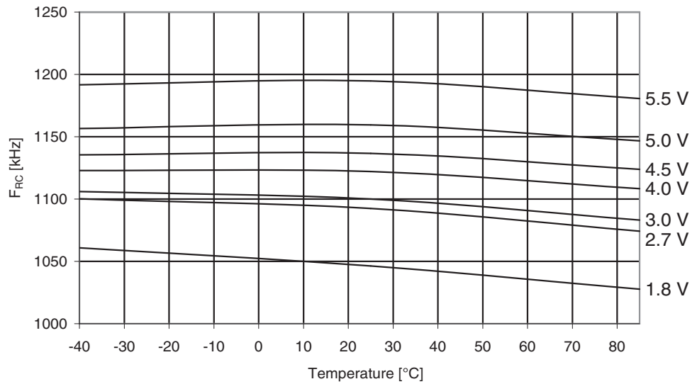
Figure 29-290. ATmega3290A: Watchdog Oscillator Frequency vs. Temperature
