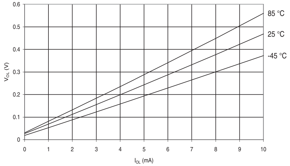
Figure 29-394. ATmega649A: I/O Pin Output Voltage vs. Sink Current, Ports A, C, D, E, F, G ( V_{CC} = 2.7V )
