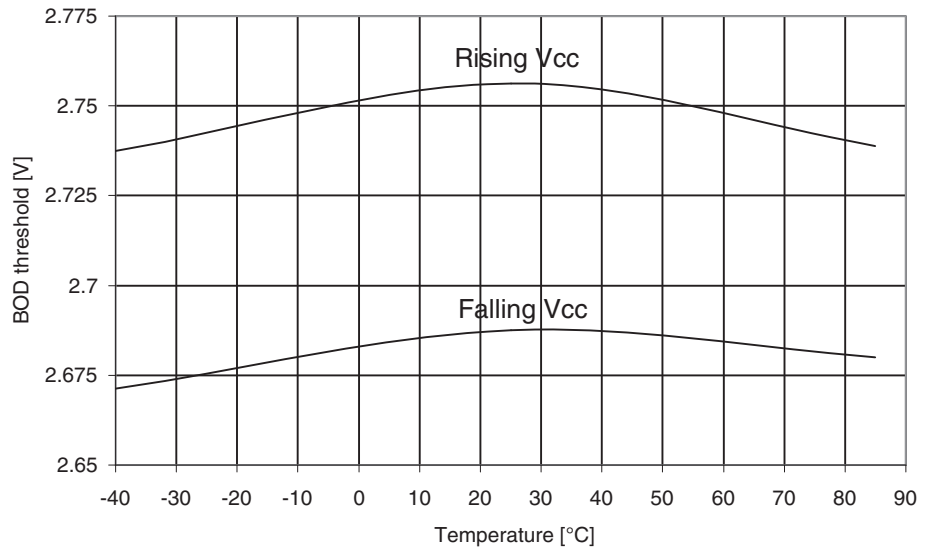
Figure 29-345. ATmega3290PA: BOD Thresholds vs. Temperature (BOD Level is 2.7V)
