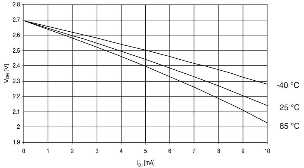
Figure 29-267. ATmega3290A: I/O Pin Output Voltage vs. Source Current, Ports A, C, D, E, F, G ( V_{CC} = 2.7V )
