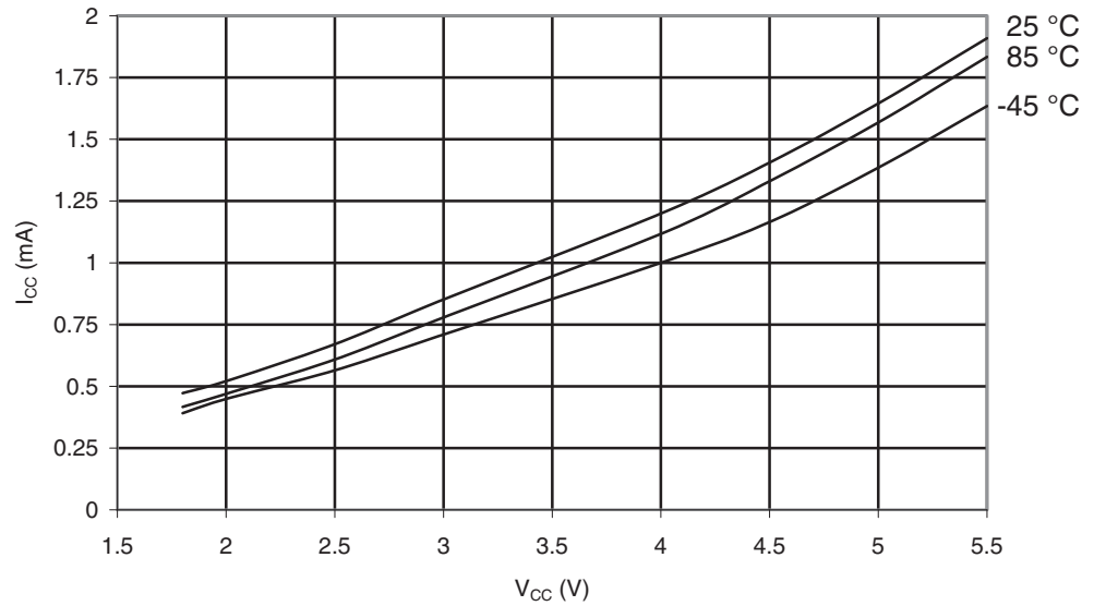
Figure 29-8. ATmega169A: Idle Supply Current vs. V_{CC} (Internal RC Oscillator, 8 MHz)
