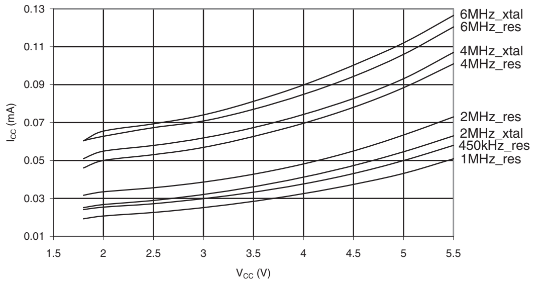
Figure 29-319. ATmega3290PA: Standby Supply Current vs. V_{CC} (Xtall and Resonator, Watchdog Timer Disabled)
