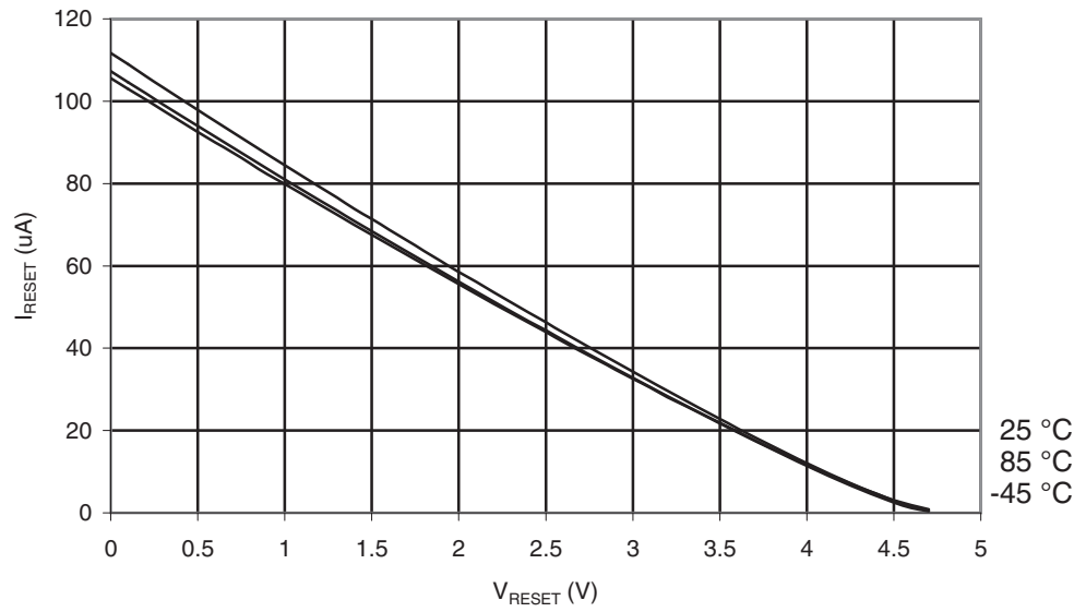
Figure 29-19. ATmega169A: Reset Pull-up Resistor Current vs. Reset Pin Voltage ( V_{CC} = 5V )
