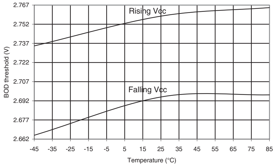
Figure 29-103. ATmega169PA: BOD Thresholds vs. Temperature (BOD Level is 2.7V)
