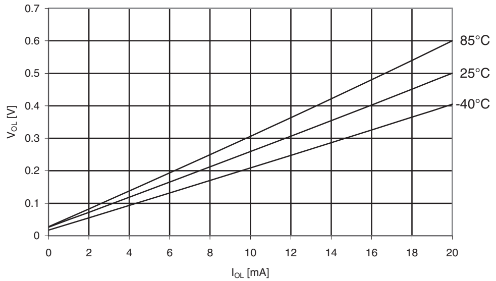
Figure 29-275. ATmega3290A: I/O Pin Output Voltage vs. Sink Current, Port B ( V_{CC} = 5V )
