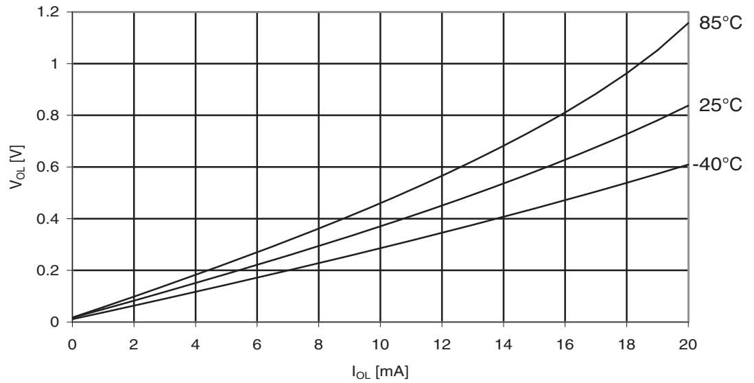
Figure 29-156. ATmega329A: I/O Pin Output Voltage vs. Sink Current, Port B ( V_{CC} = 2.7V )
