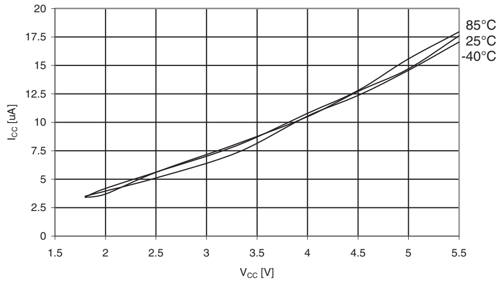
Figure 29-359. ATmega3290PA: Watchdog Timer Current vs. V_{CC}
