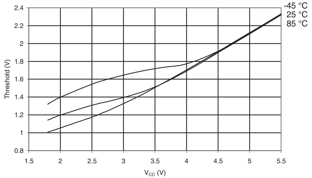
Figure 29-524. ATmega6490A: Reset Input Threshold Voltage vs. V_{CC} ( V_{IH,Reset} Pin Read as "1")
