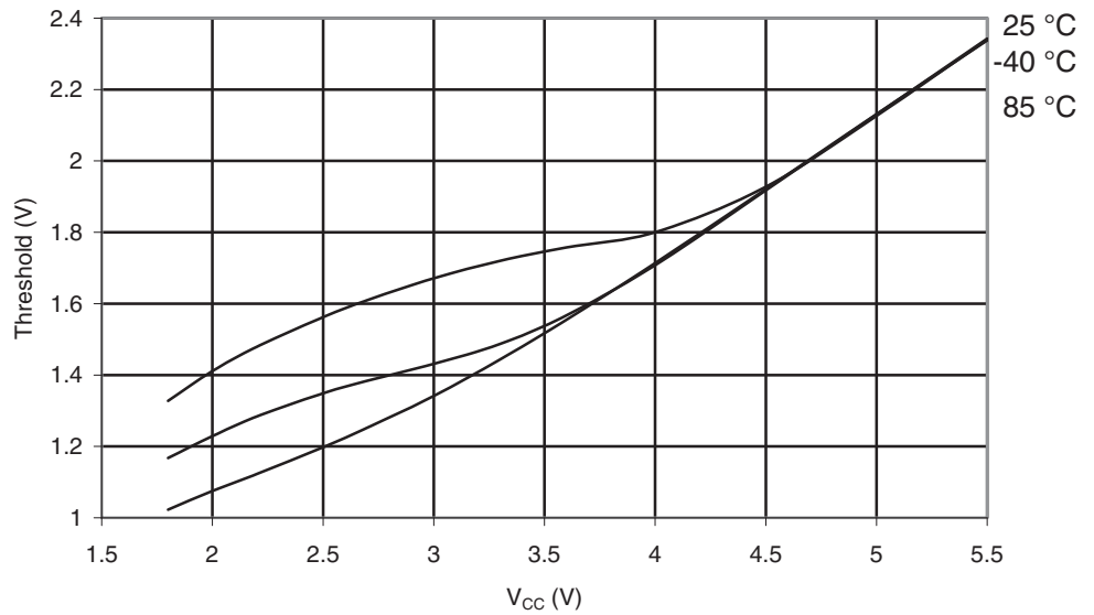
Figure 29-341. ATmega3290PA: Reset Input Threshold Voltage vs. V_{CC} ( V_{IH,Reset} Pin Read as "1")
