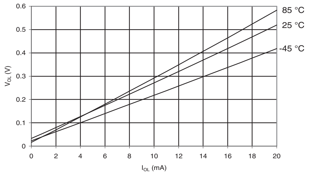
Figure 29-579. ATmega6490P: I/O Pin Output Voltage vs. Sink Current, Port B ( V_{CC} = 5V )
