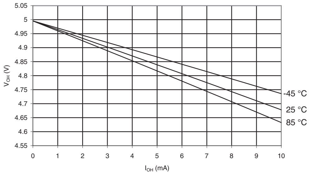
Figure 29-22. ATmega169A: I/O Pin Output Voltage vs. Source Current, Ports A, C, D, E, F, G ( V_{CC} = 5V )
