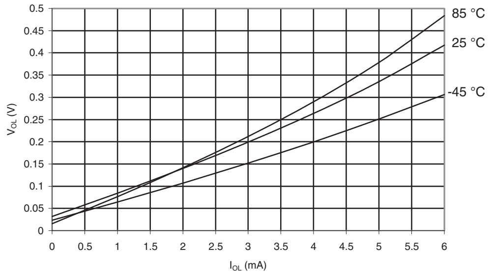
Figure 29-581. ATmega6490P: I/O Pin Output Voltage vs. Sink Current, Port B ( V_{CC} = 1.8V )
