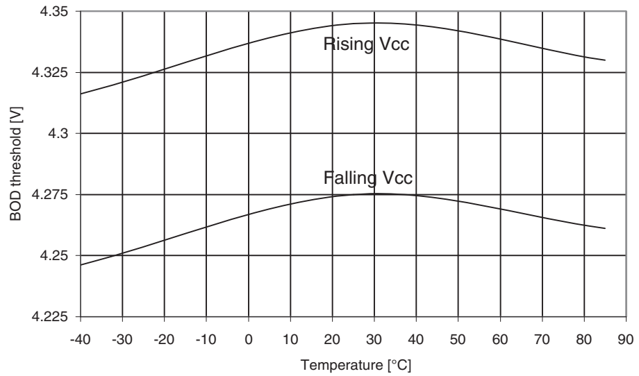
Figure 29-224. ATmega329PA: BOD Thresholds vs. Temperature (BOD Level is 4.3V)
