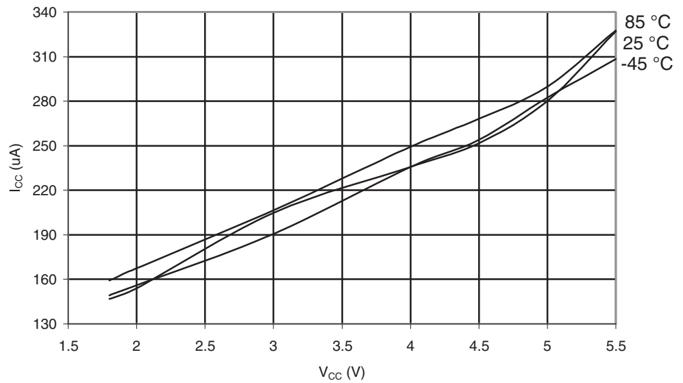
Figure 29-418. ATmega649A: Active Supply Current with ADC at 1 MHz vs. V_{CC}
