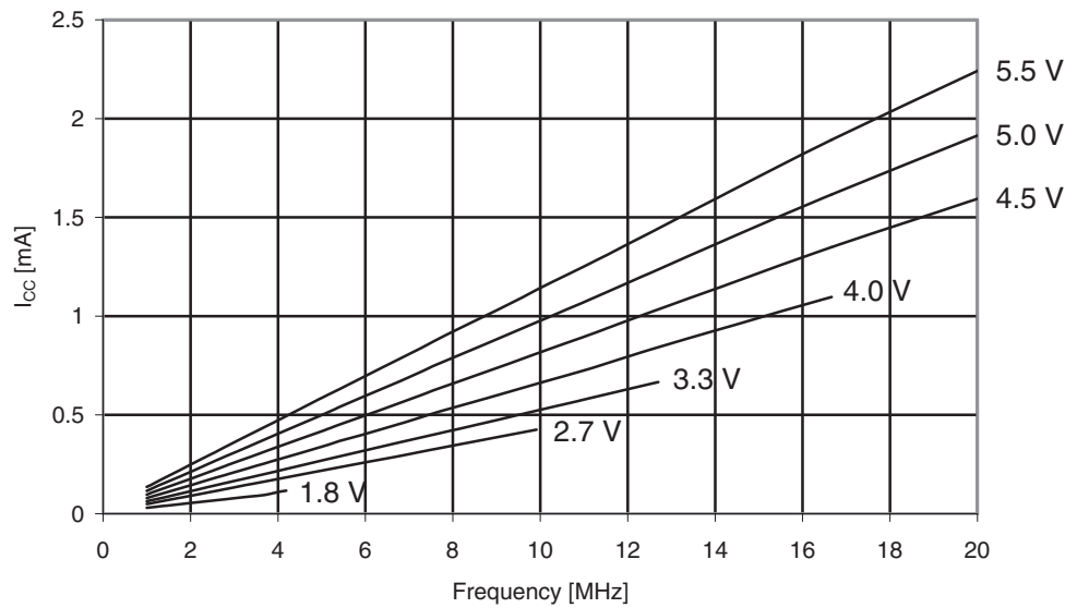
Figure 29-243. ATmega329PA: Reset Supply Current vs. V_{CC} (1 - 20MHz, Excluding Current Through The Reset Pull-up)
