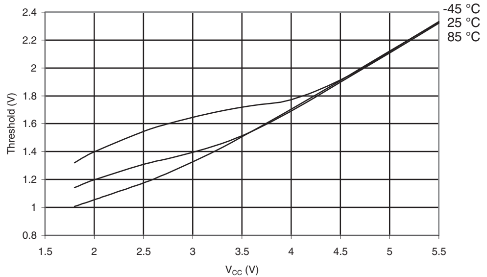
Figure 29-463. ATmega649P: Reset Input Threshold Voltage vs. V_{CC} ( V_{IH} , Reset Pin Read as "1")
