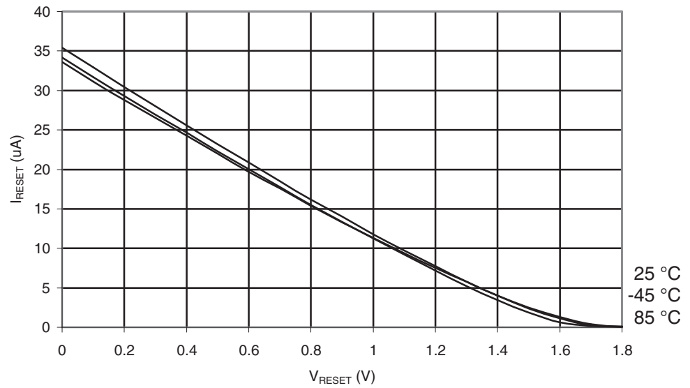
Figure 29-386. ATmega649A: Reset Pull-up Resistor Current vs. Reset Pin Voltage ( V_{CC} = 1.8V )
