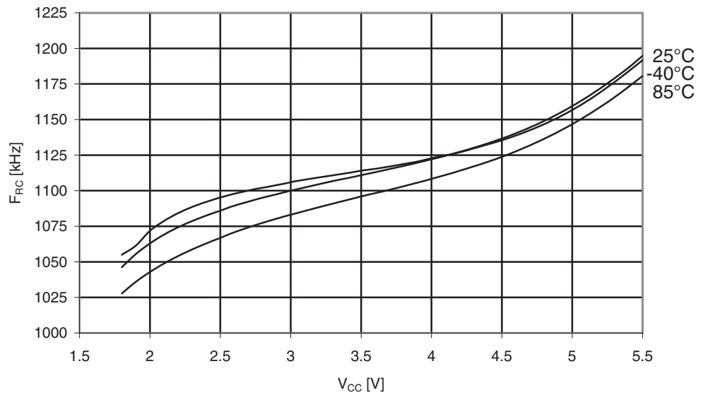
Figure 29-289. ATmega3290A: Watchdog Oscillator Frequency vs. V_{CC}
