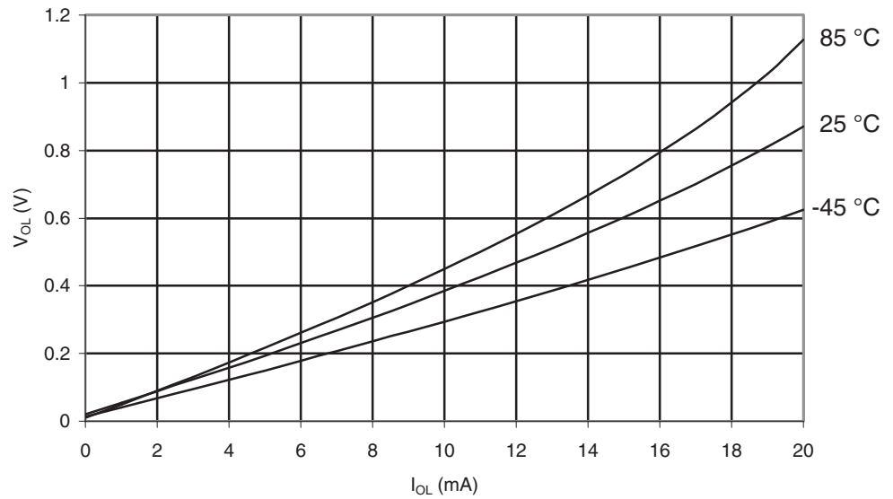
Figure 29-580. ATmega6490P: I/O Pin Output Voltage vs. Sink Current, Port B ( V_{CC} = 2.7V_9 )
