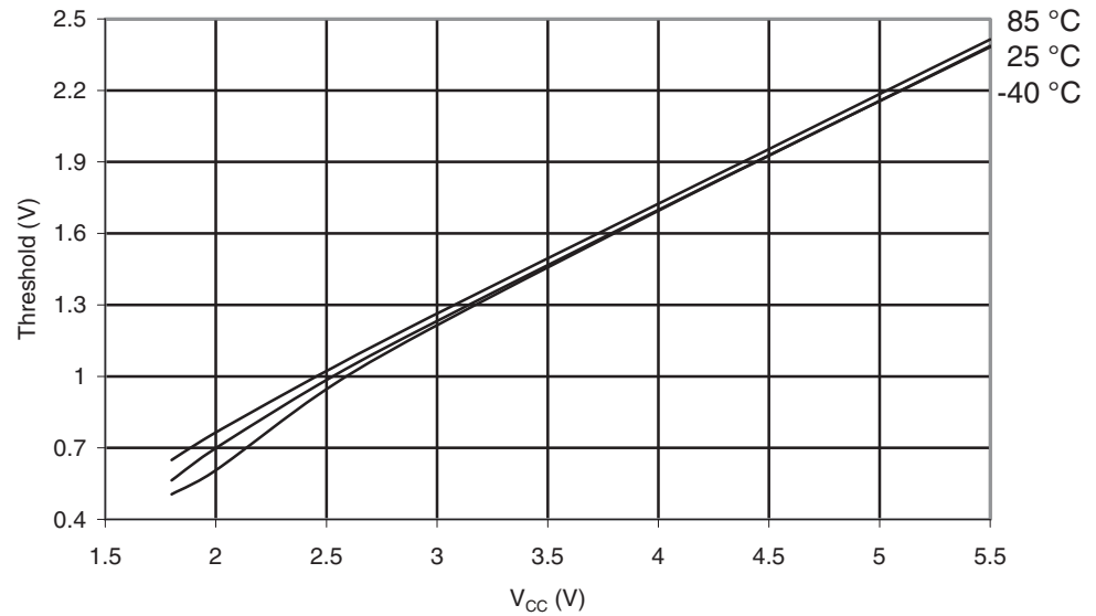
Figure 29-339. ATmega3290PA: I/O Pin Input Threshold Voltage vs. V_{CC} ( V_{IL} , I/O Pin Read as "0")
