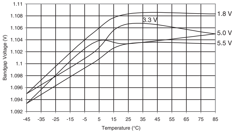
Figure 29-531. ATmega6490A: Bandgap Voltage vs. Temperature
