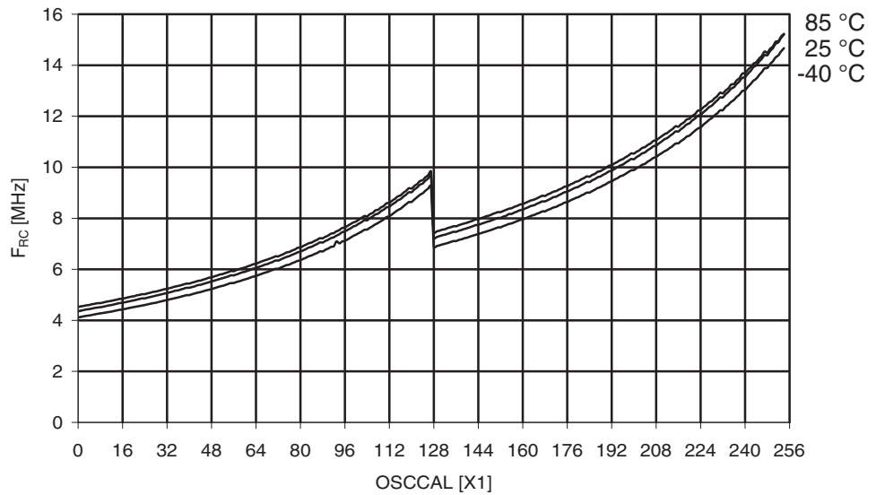
Figure 29-353. ATmega3290PA: Calibrated 8 MHz RC Oscillator Frequency vs. OSCAL Value
