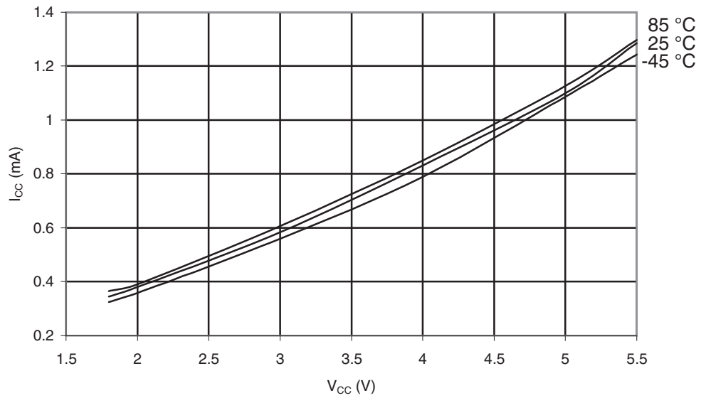
Figure 29-373. ATmega649A: Idle Supply Current vs. V_{CC} (Internal RC Oscillator, 1 MHz)
