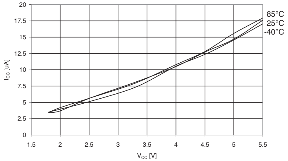
Figure 29-299. ATmega3290A: Watchdog Timer Current vs. V_{CC}
