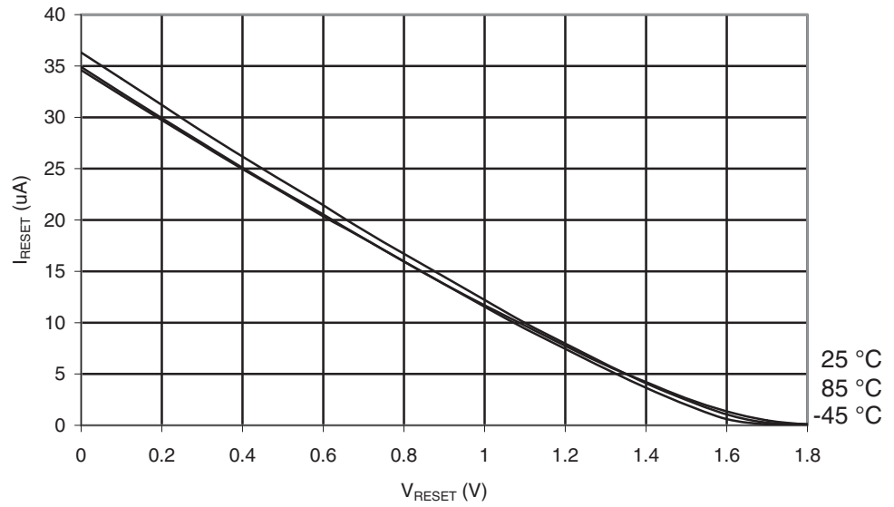
Figure 29-83. ATmega169PA: Reset Pull-up Resistor Current vs. Reset Pin Voltage ( V_{CC} = 1.8V )
