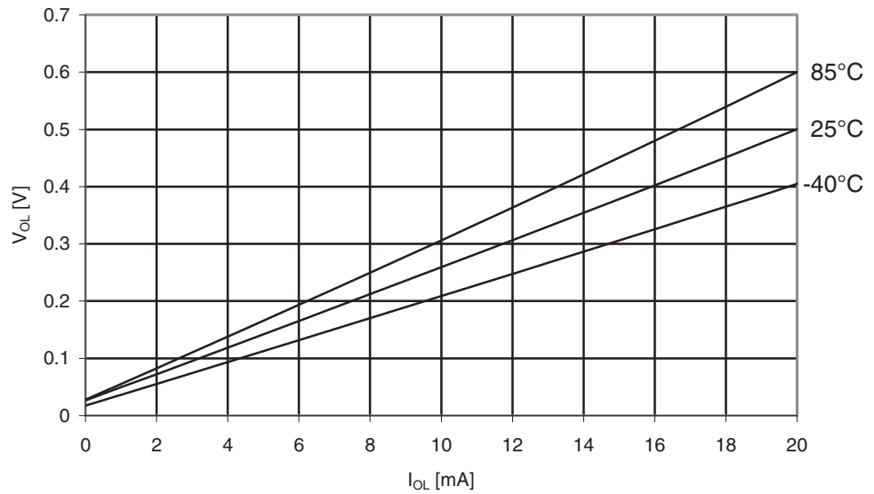
Figure 29-335. ATmega3290PA: I/O Pin Output Voltage vs. Sink Current, Port B ( V_{CC} = 5V )
