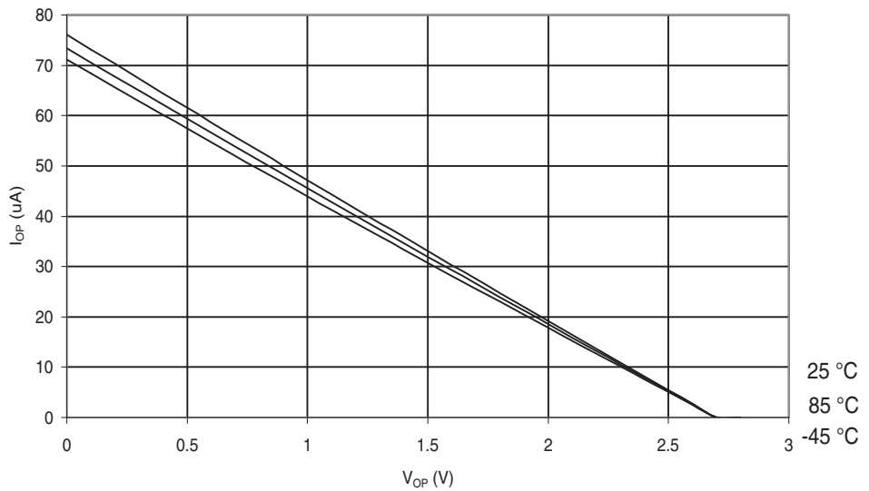
Figure 29-565. ATmega6490P: I/O Pin Pull-up Resistor Current vs. Input Voltage ( V_{CC} = 2.7V )
