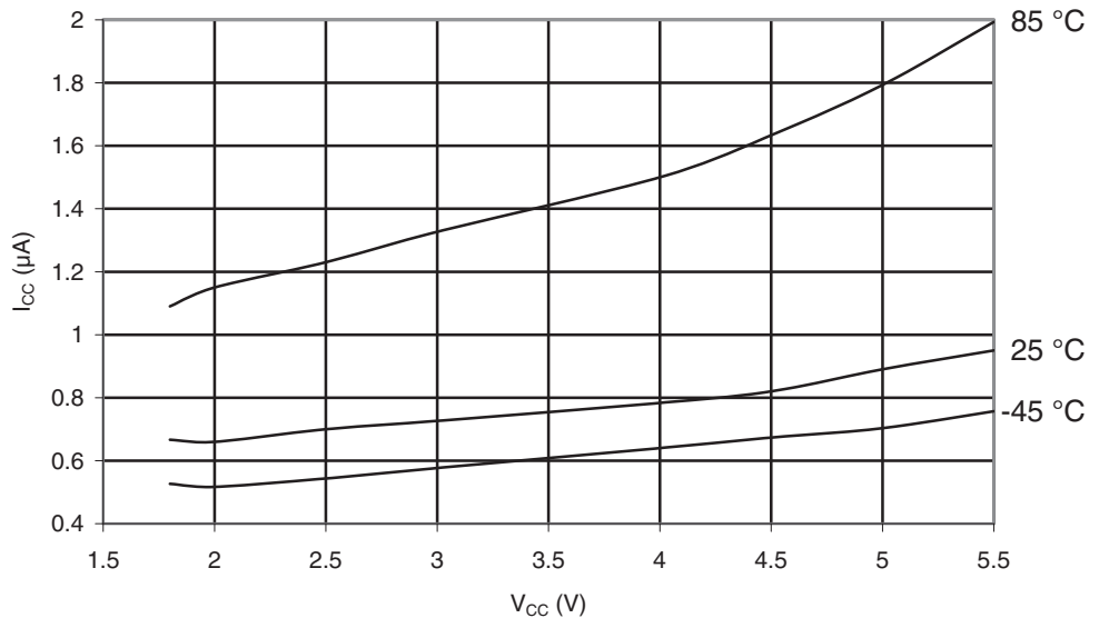
Figure 29-76. ATmega169PA: Standby Supply Current vs. V_{CC} (32 kHz Watch Crystal, Watchdog Timer Disabled)
