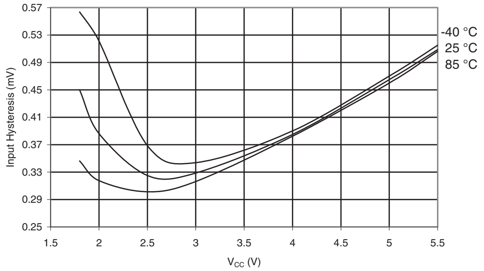
Figure 29-340. ATmega3290PA: I/O Pin Input Hysteresis vs. V_{CC}
