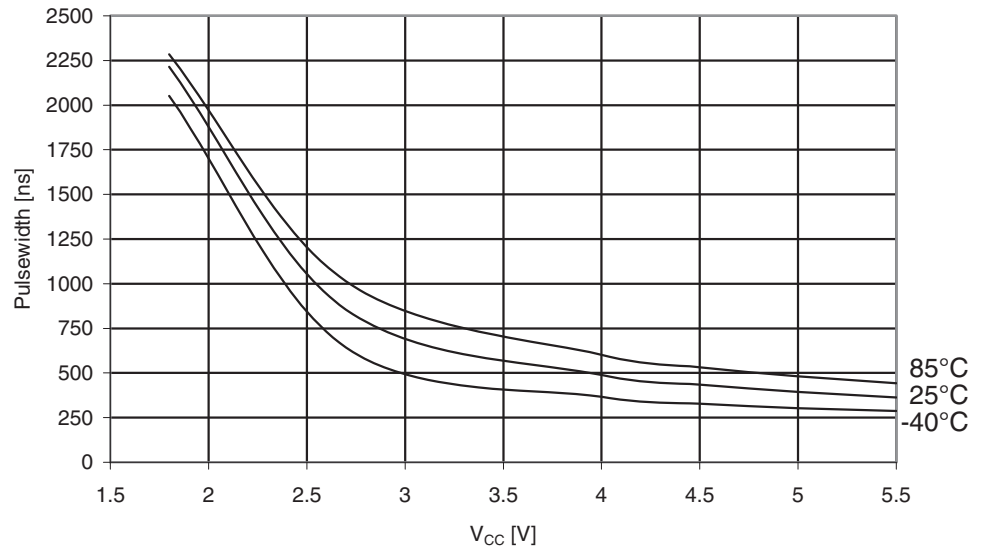
Figure 29-184. ATmega329A: Minimum Reset Pulse Width vs. V_{CC}
