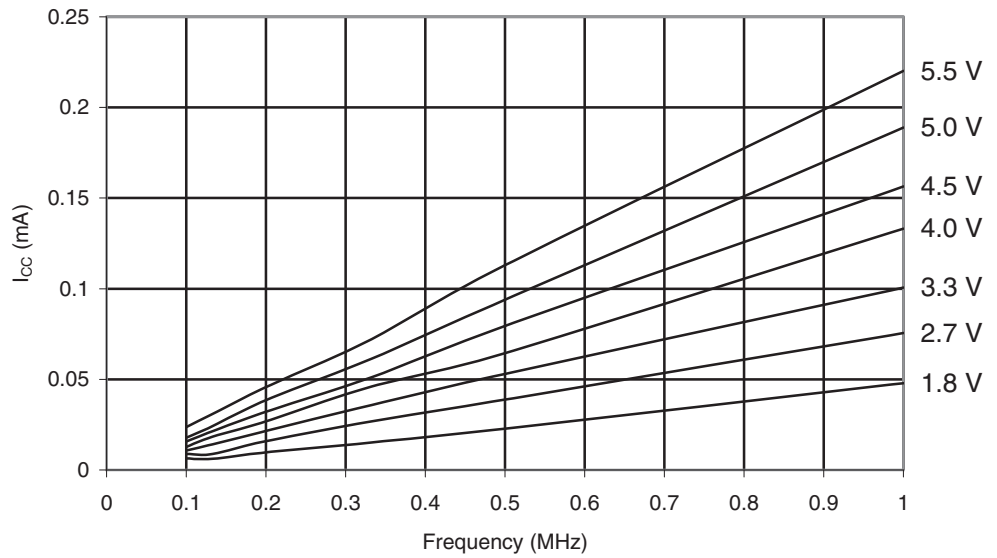
Figure 29-68. ATmega169PA: Idle Supply Current vs. Frequency (0.1 - 1.0 MHz)
