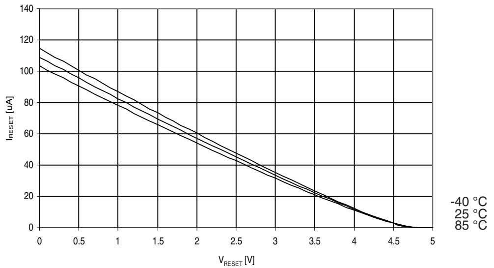
Figure 29-203. ATmega329PA: Reset Pull-up Resistor Current vs. Reset Pin Voltage ( V_{CC} = 5V )
