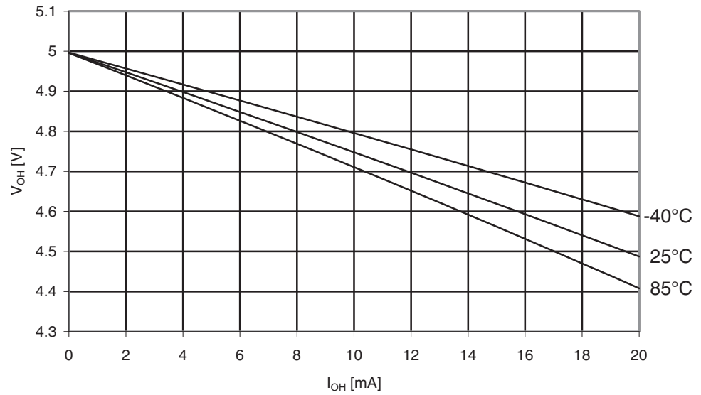
Figure 29-269. ATmega3290A: I/O Pin Output Voltage vs. Source Current, Port B ( V_{CC} = 5V )
