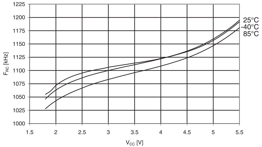
Figure 29-349. ATmega3290PA: Watchdog Oscillator Frequency vs. V_{CC}
