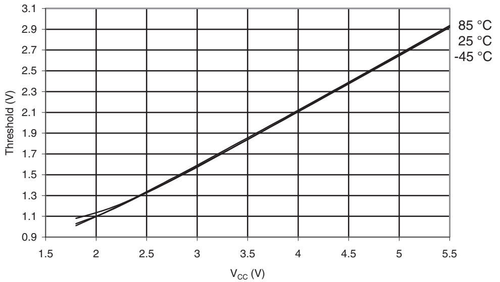
Figure 29-96. ATmega169PA: I/O Pin Input Threshold Voltage vs. V_{CC} ( V_{IH} , I/O Pin Read as "1")
