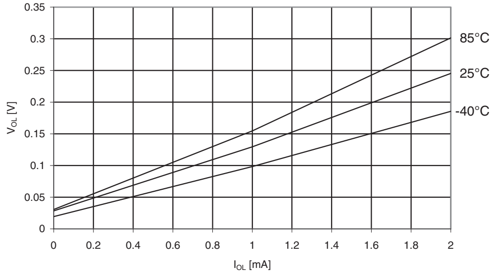
Figure 29-154. ATmega329A: I/O Pin Output Voltage vs. Sink Current, Ports A, C, D, E, F, G ( V_{CC} = 1.8V )
