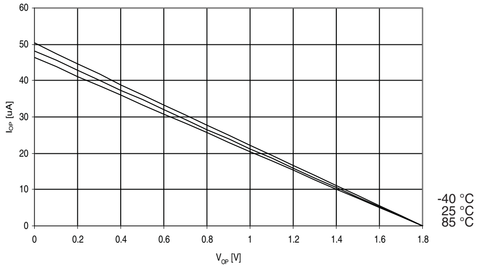
Figure 29-322. ATmega3290PA: I/O Pin Pull-up Resistor Current vs. Input Voltage ( V_{CC} = 1.8V )
