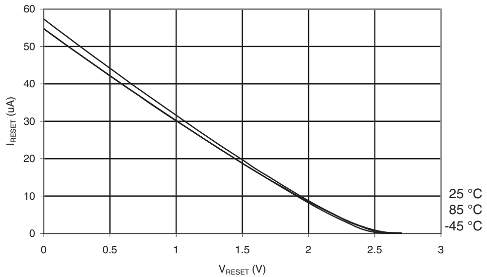
Figure 29-82. ATmega169PA: Reset Pull-up Resistor Current vs. Reset Pin Voltage ( V_{CC} = 2.7V )
