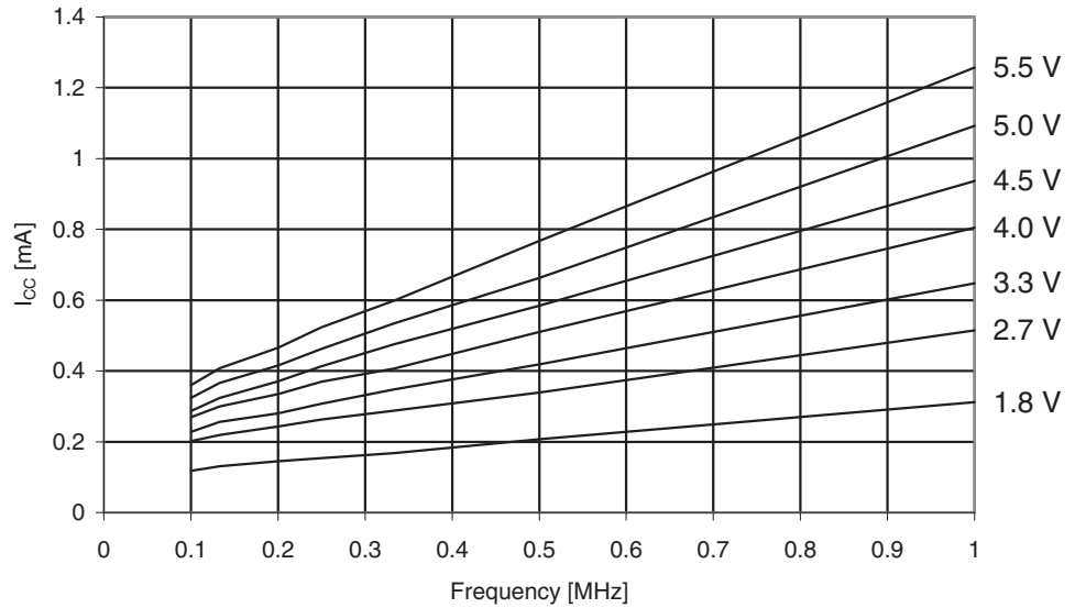
Figure 29-185. ATmega329PA: Active Supply Current vs. Low Frequency (0.1 - 1.0 MHz)
