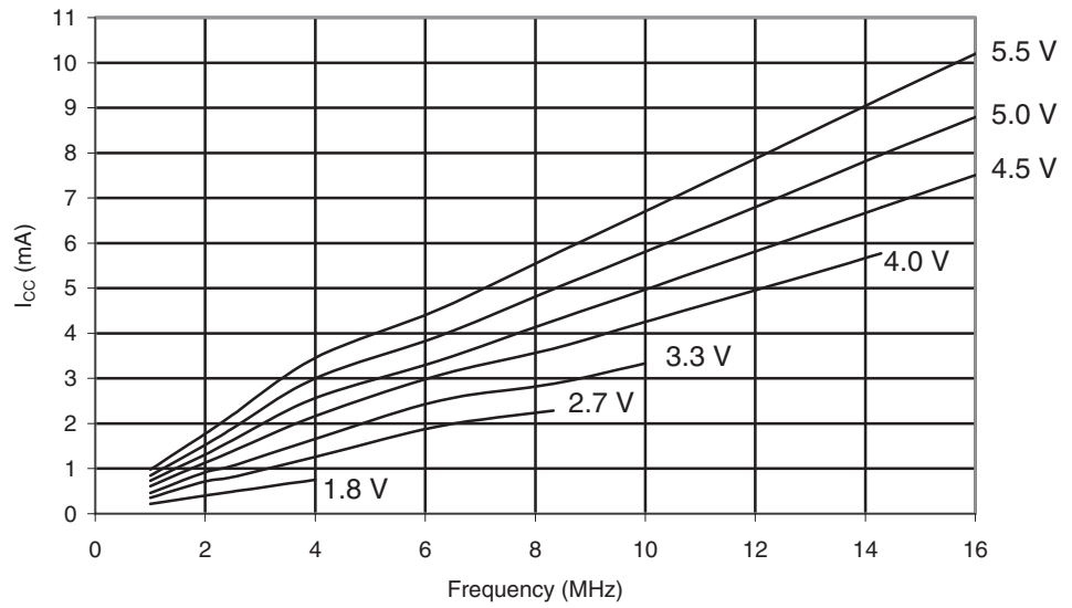
Figure 29-2. ATmega169A: Active Supply Current vs. Frequency (1 - 16 MHz)
