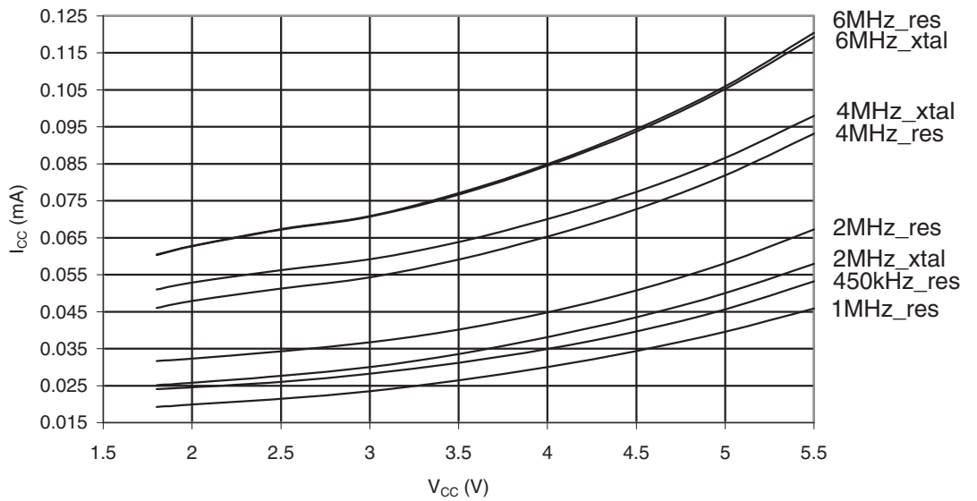
Figure 29-502. ATmega6490A: Standby Supply Current vs. V_{CC} (Xtall and Resonator, Watchdog Timer Disabled)
