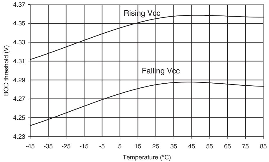
Figure 29-102. ATmega169PA: BOD Thresholds vs. Temperature (BOD Level is 4.3V)
