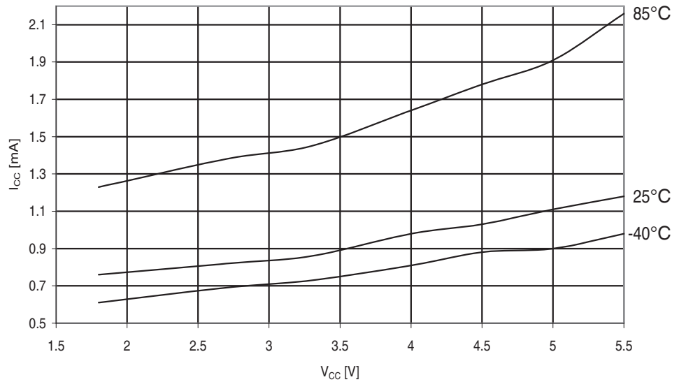
Figure 29-257. ATmega3290A: Power-save Supply Current vs. V_{CC} (Watchdog Timer Disabled and 32 kHz Crystal Oscillator Running)
