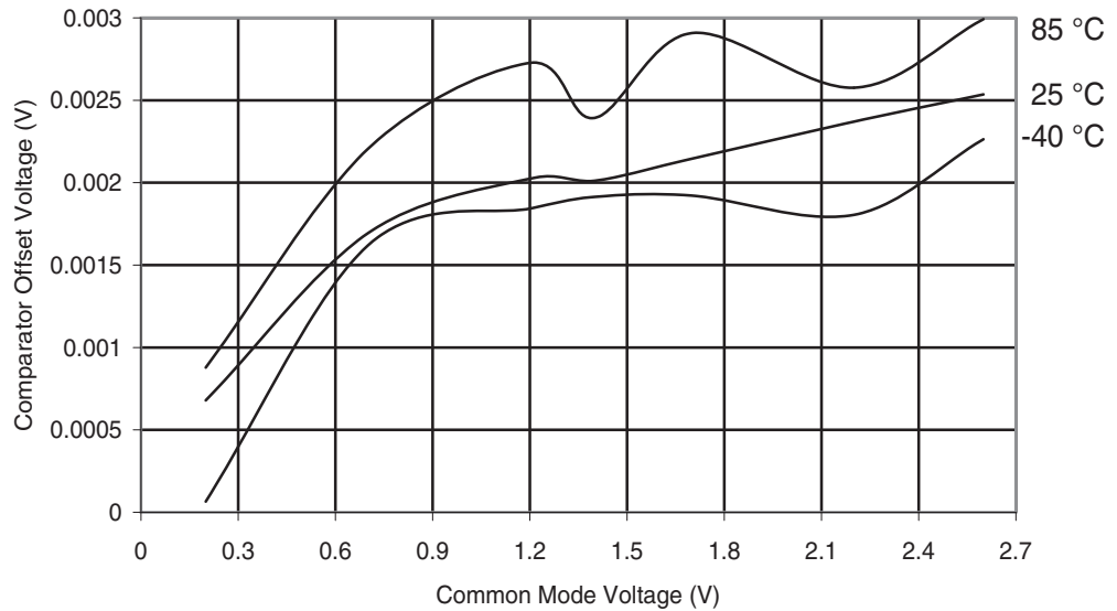
Figure 29-108. ATmega169PA: Analog Comparator Offset Voltage vs. Common Mode Voltage ( V_{CC} = 2.7V )
