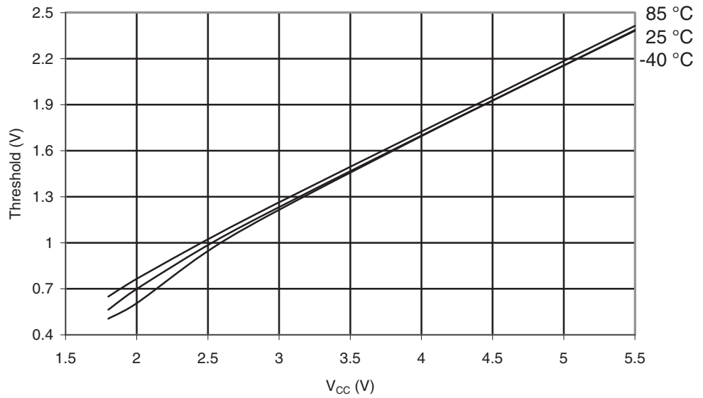
Figure 29-279. ATmega3290A: I/O Pin Input Threshold Voltage vs. V_{CC} ( V_{IL} , I/O Pin Read as "0")
