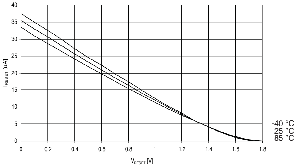
Figure 29-325. ATmega3290PA: Reset Pull-up Resistor Current vs. Reset Pin Voltage ( V_{CC} = 1.8V )
