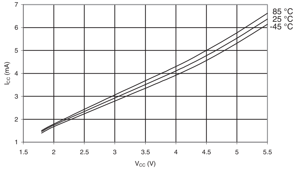
Figure 29-367. ATmega649A: Active Supply Current vs. V_{CC} (Internal RC Oscillator, 8 MHz)
