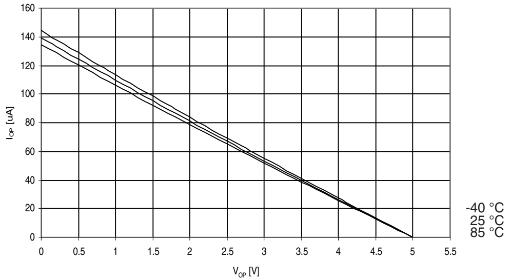
Figure 29-260. ATmega3290A: I/O Pin Pull-up Resistor Current vs. Input Voltage ( V_{CC} = 5V )
