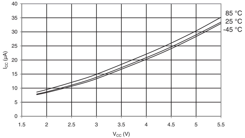
Figure 29-5. ATmega169A: Active Supply Current vs. V_{CC} (32 kHz Watch Crystal)
