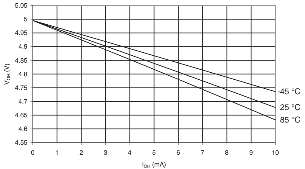
Figure 29-84. ATmega169PA: I/O Pin Output Voltage vs. Source Current, Ports A, C, D, E, F, G ( V_{CC} = 5V )
