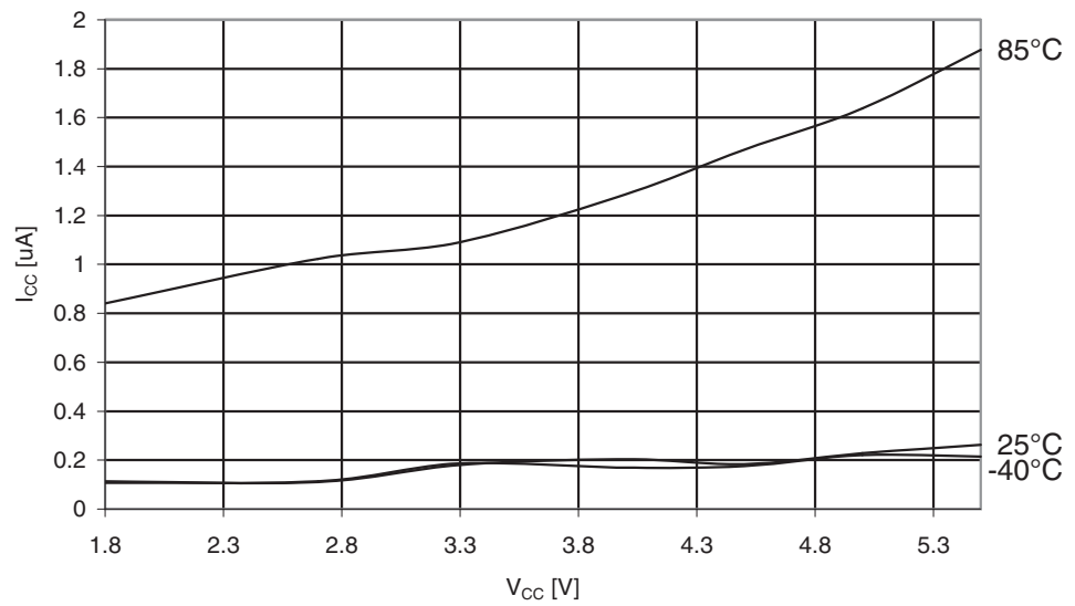
Figure 29-196. ATmega329PA: Power-down Supply Current vs. V_{CC} (Watchdog Timer Enabled)
