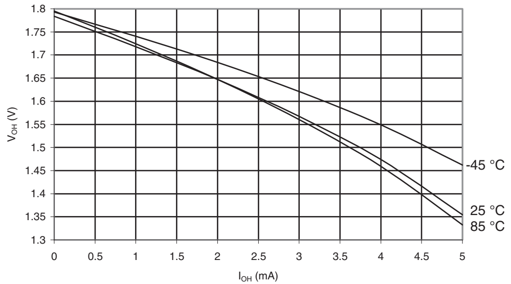
Figure 29-514. ATmega6490A: I/O Pin Output Voltage vs. Source Current, Port B ( V_{CC} = 1.8V )
