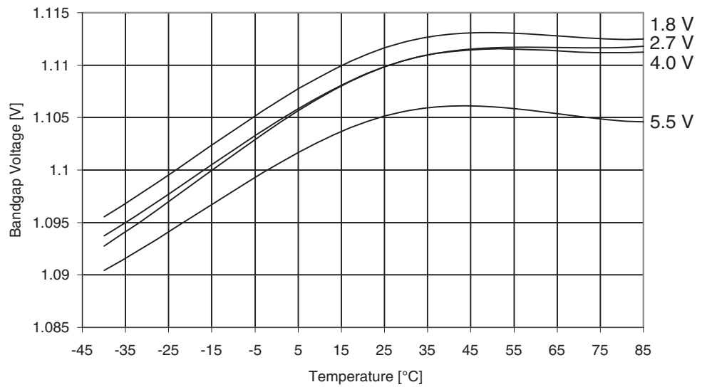
Figure 29-288. ATmega3290A: Bandgap Voltage vs. Temperature
