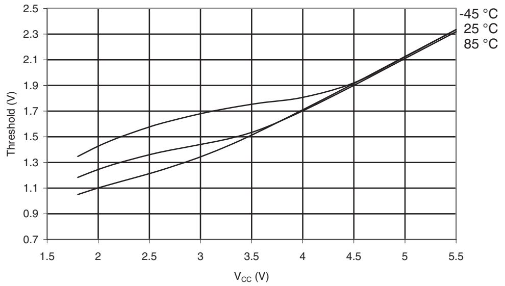
Figure 29-37. ATmega169A: Reset Input Threshold Voltage vs. V_{CC} ( V_{IH} , Reset Pin Read as "1")
