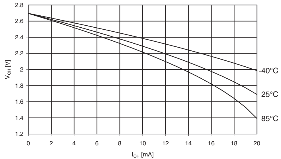
Figure 29-270. ATmega3290A: I/O Pin Output Voltage vs. Source Current, Port B ( V_{CC} = 2.7V )
