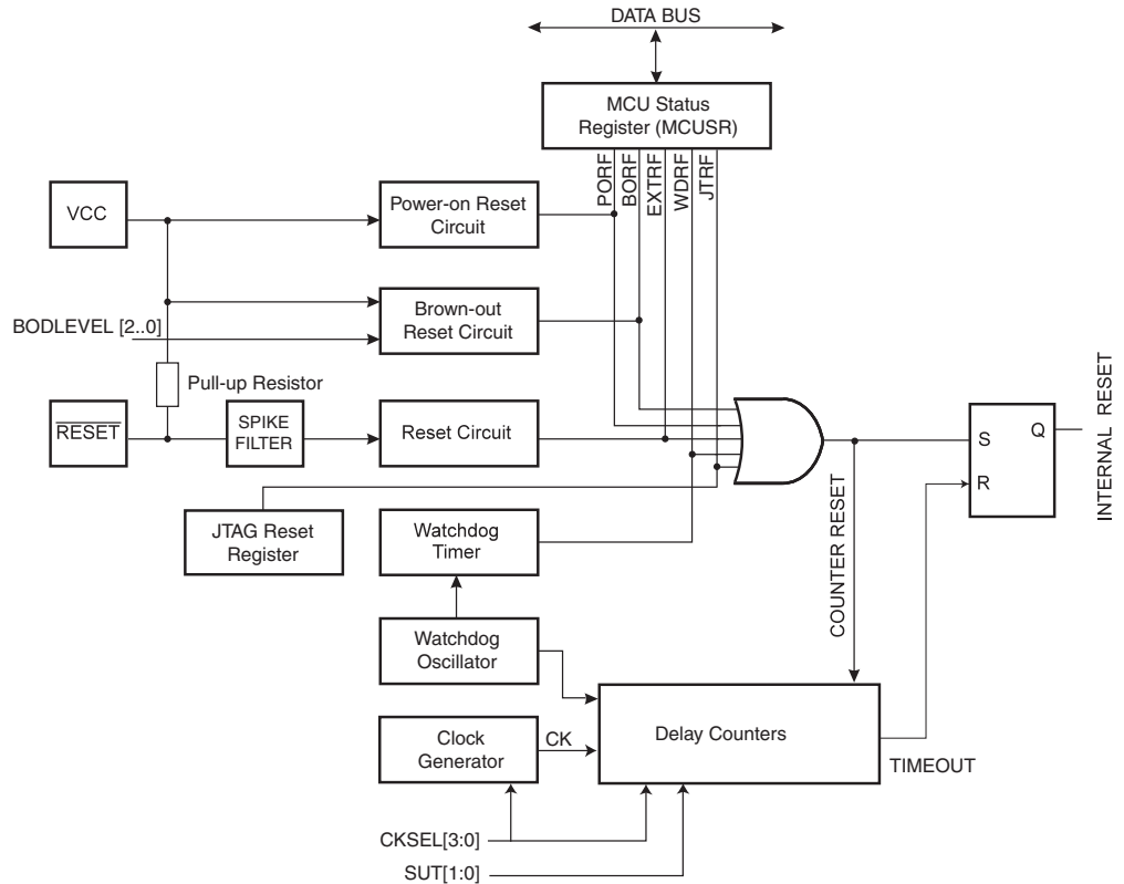
Figure 10-1. Reset Logic
