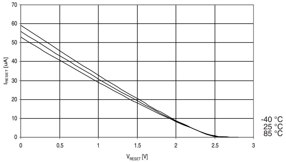
Figure 29-264. ATmega3290A: Reset Pull-up Resistor Current vs. Reset Pin Voltage ( V_{CC} = 2.7V )
