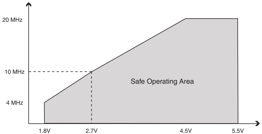
Figure 28-2. Maximum Frequency vs. V_{CC} (0 - 20 MHz) ATmega329A/ATmega329PA/ATmega3290A/ATmega3290PA/ATmega6490A/ ATmega6490P
