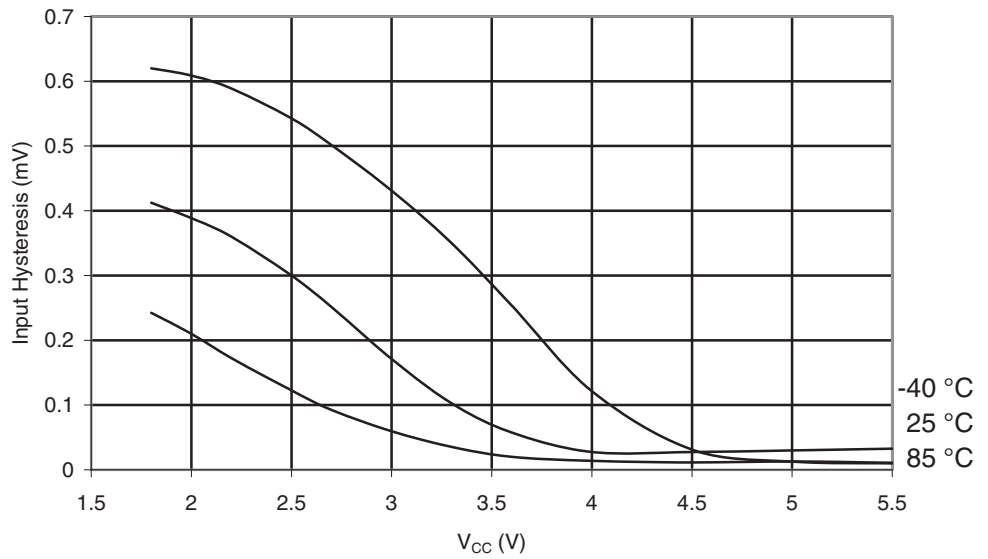
Figure 29-343. ATmega3290PA: Reset Input Pin Hysteresis vs. V_{CC}
