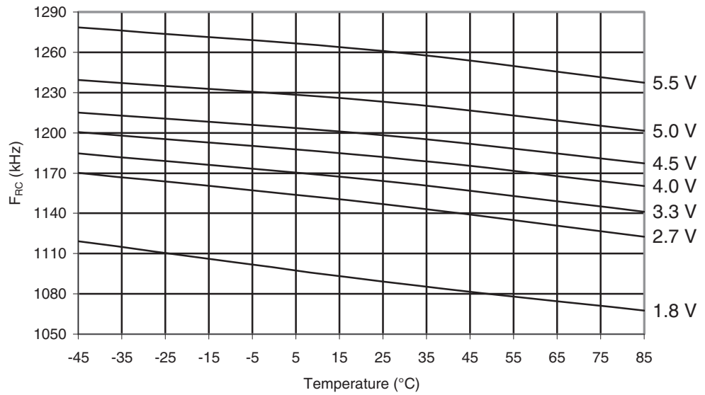
Figure 29-472. ATmega649P: Watchdog Oscillator Frequency vs. Temperature
