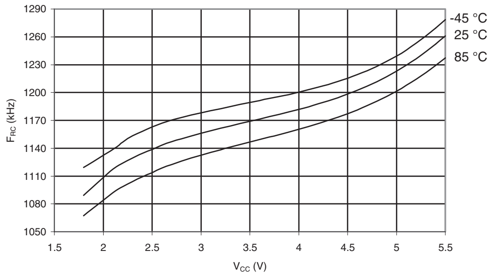
Figure 29-532. ATmega6490A: Watchdog Oscillator Frequency vs. V_{CC}
