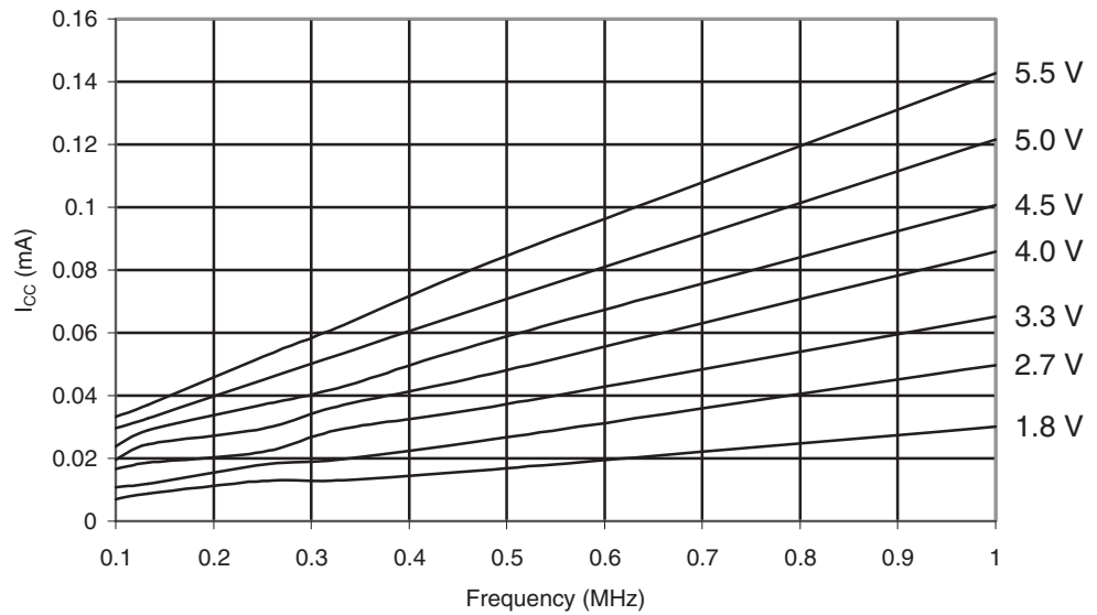
Figure 29-545. ATmega6490A: Reset Supply Current vs. V_{CC} (0.1 - 1.0 MHz, Excluding Current Through The Reset Pull-up)
