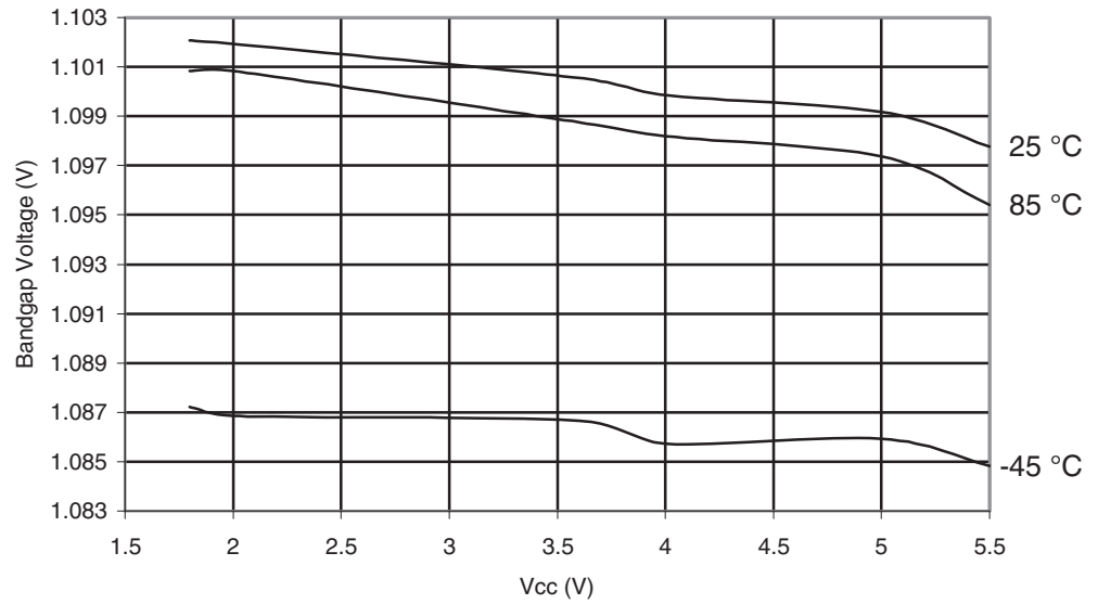
Figure 29-408. ATmega649A: Bandgap Voltage vs. V CC
