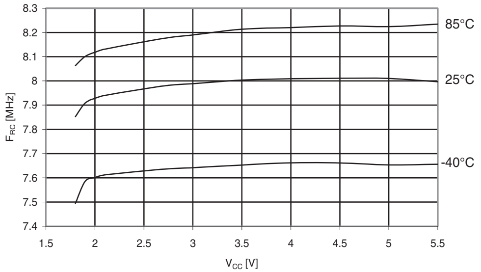
Figure 29-172. ATmega329A: Calibrated 8 MHz RC Oscillator Frequency vs. V_{CC}
