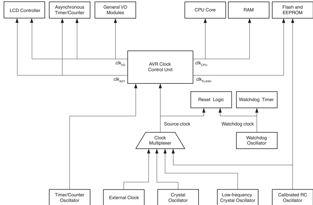
Figure 8-1. Clock Distribution
