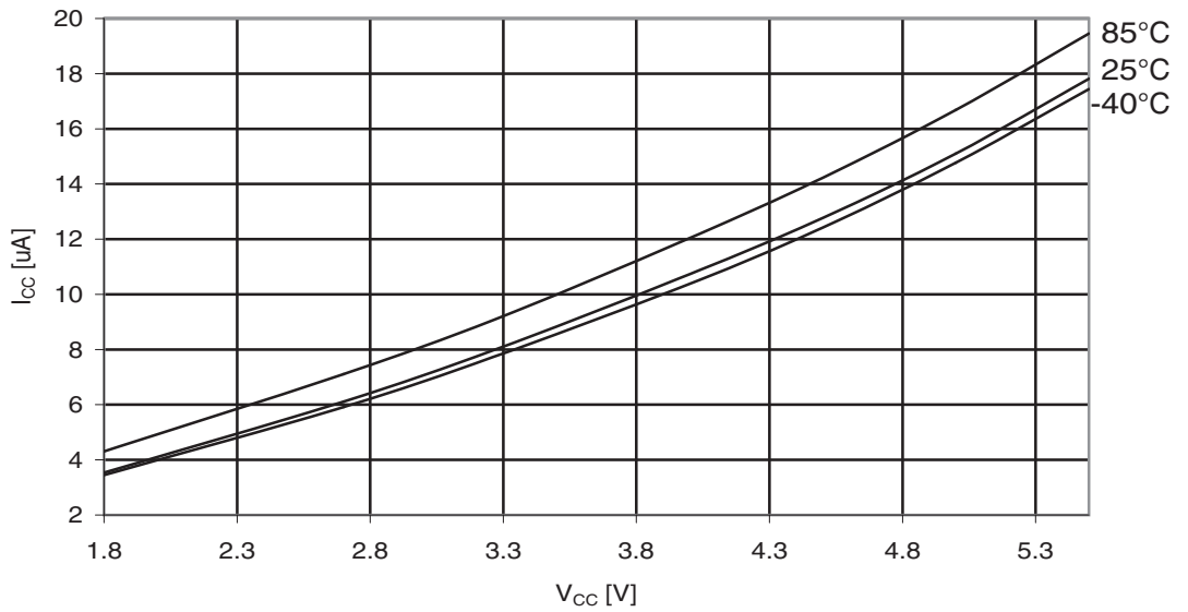
Figure 29-256. ATmega3290A: Power-down Supply Current vs. V_{CC} (Watchdog Timer Enabled)
