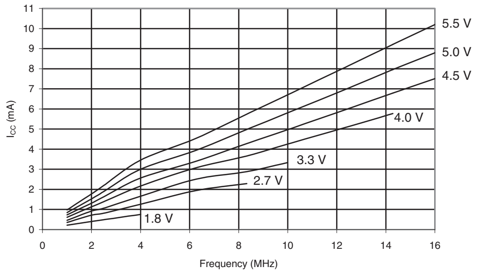
Figure 29-64. ATmega169PA: Active Supply Current vs. Frequency (1 - 16 MHz)
