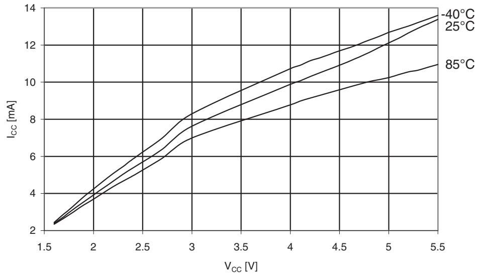
Figure 29-181. ATmega329A: Programming Current vs. V_{CC}
