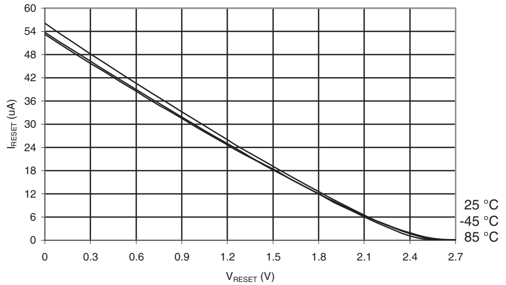
Figure 29-446. ATmega649P: Reset Pull-up Resistor Current vs. Reset Pin Voltage ( V_{CC} = 2.7V )
