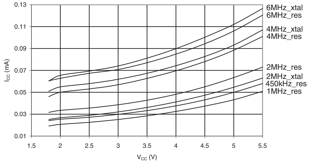
Figure 29-259. ATmega3290A: Standby Supply Current vs. V_{CC} (Xtall and Resonator, Watchdog Timer Disabled)
