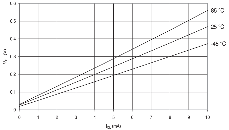
Figure 29-455. ATmega649P: I/O Pin Output Voltage vs. Sink Current, Ports A, C, D, E, F, G ( V_{CC} = 2.7V )
