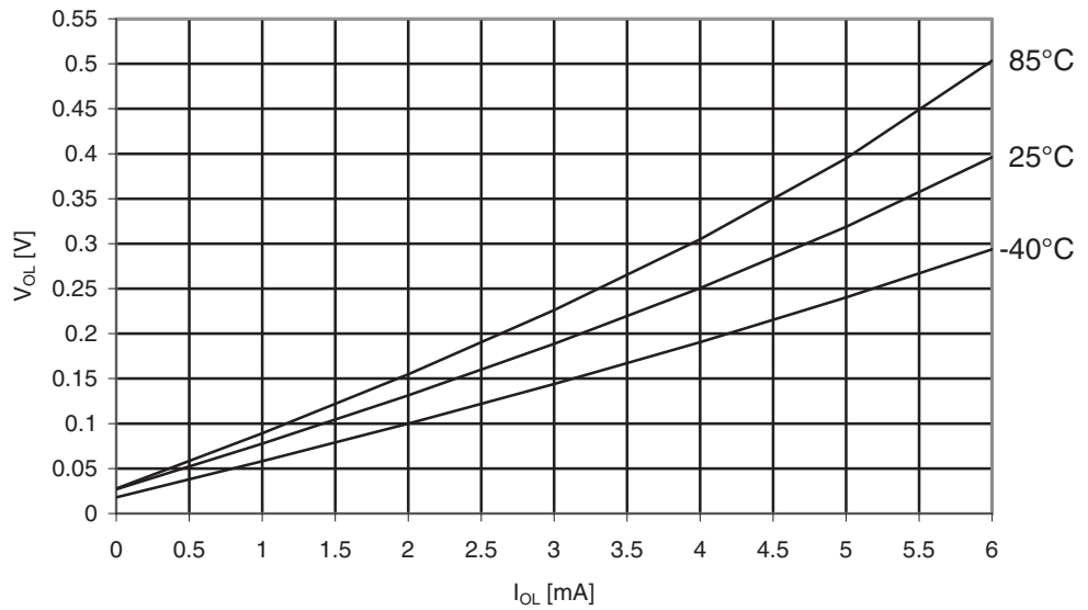
Figure 29-337. ATmega3290PA: I/O Pin Output Voltage vs. Sink Current, Port B ( V_{CC} = 1.8V )
