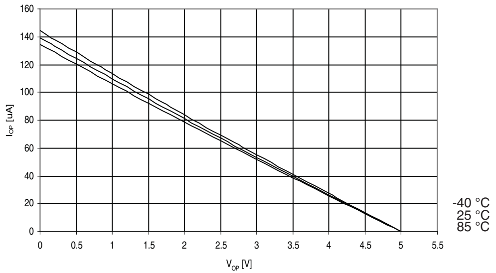
Figure 29-140. ATmega329A: I/O Pin Pull-up Resistor Current vs. Input Voltage ( V_{CC} = 5V )
