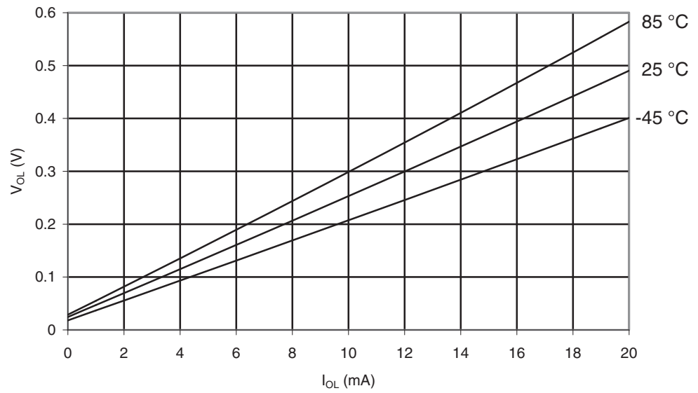
Figure 29-31. ATmega169A: I/O Pin Output Voltage vs. Sink Current, Port B ( V_{CC} = 5V )
