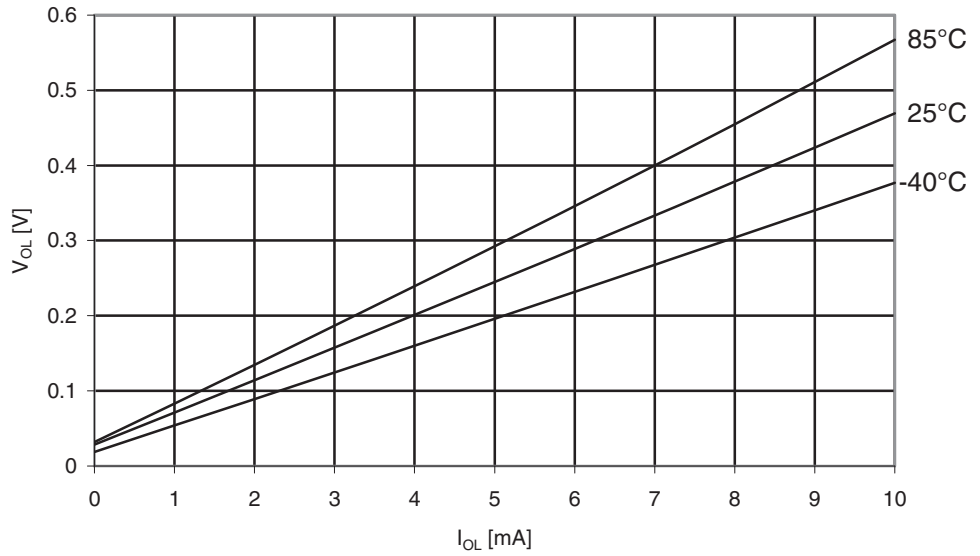
Figure 29-152. ATmega329A: I/O Pin Output Voltage vs. Sink Current, Ports A, C, D, E, F, G ( V_{CC} = 5V )
