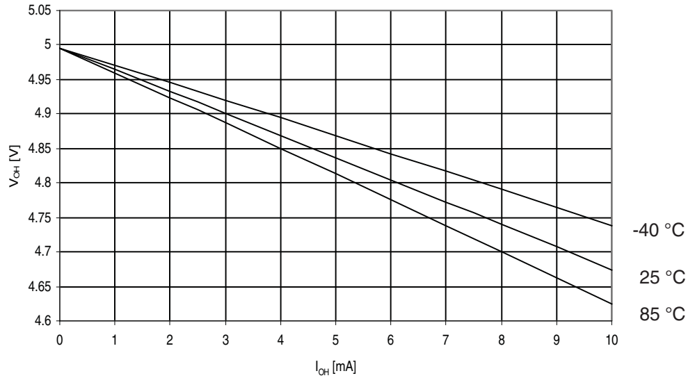
Figure 29-326. ATmega3290PA: I/O Pin Output Voltage vs. Source Current, Ports A, C, D, E, F, G ( V_{CC} = 5V )
