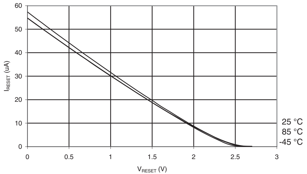
Figure 29-20. ATmega169A: Reset Pull-up Resistor Current vs. Reset Pin Voltage ( V_{CC} = 2.7V )
