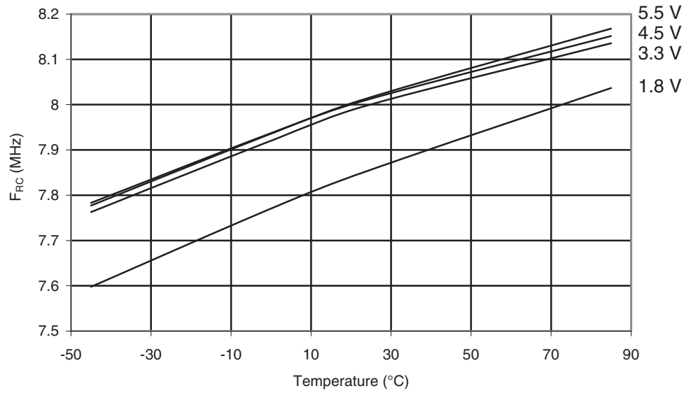
Figure 29-49. ATmega169A: Calibrated 8 MHz RC Oscillator Frequency vs. Temperature
