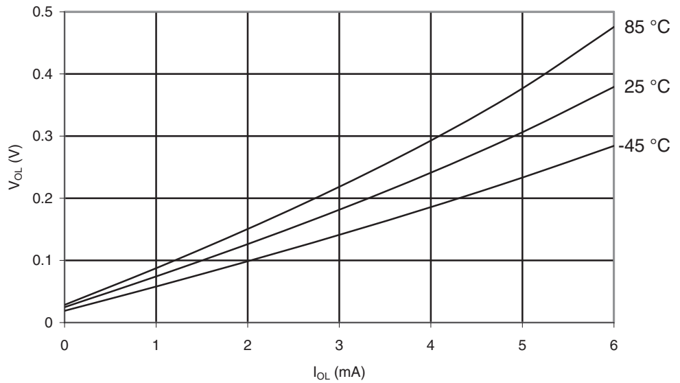
Figure 29-33. ATmega169A: I/O Pin Output Voltage vs. Sink Current, Port B ( V_{CC} = 1.8V )
