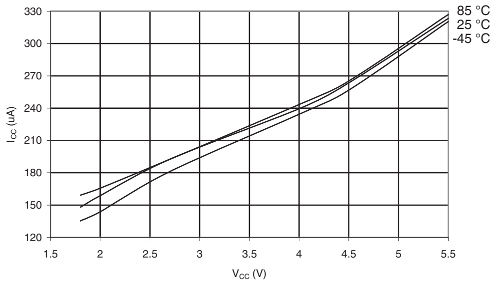
Figure 29-538. ATmega6490A: Active Supply Current with ADC at 50 kHz vs. V_{CC}
