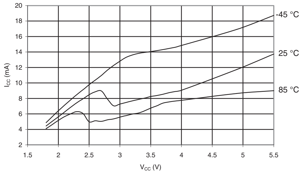
Figure 29-544. ATmega6490A: Programming Current vs. V_{CC}
