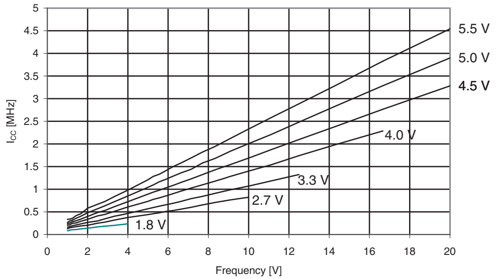
Figure 29-131. ATmega329A: Idle Supply Current vs. Frequency (1 - 20MHz)
