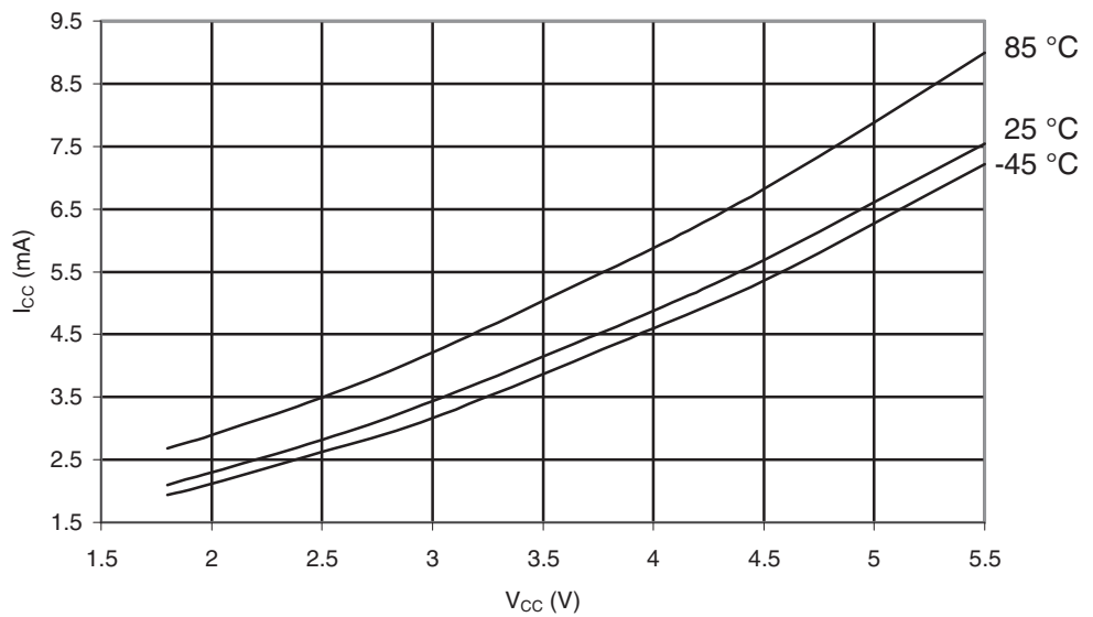
Figure 29-496. ATmega6490A: Idle Supply Current vs. V_{CC} (32 kHz Watch Crystal)
