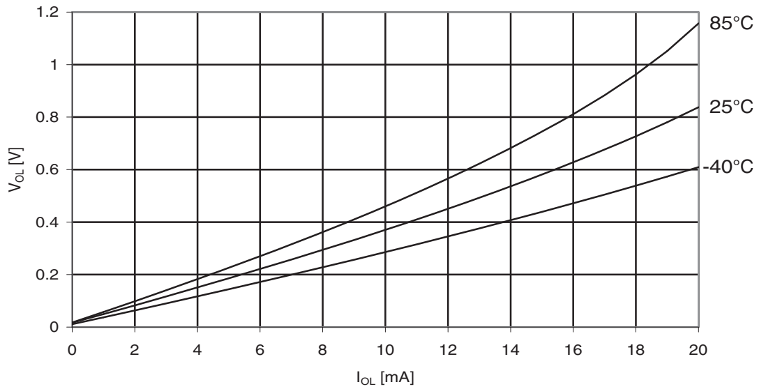
Figure 29-216. ATmega329PA: I/O Pin Output Voltage vs. Sink Current, Port B ( V_{CC} = 2.7V )
