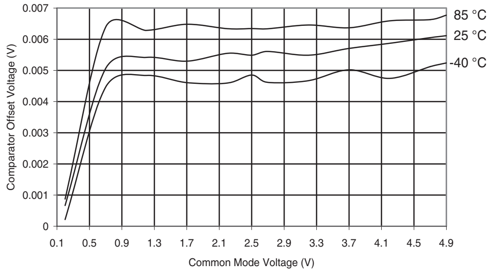
Figure 29-107. ATmega169PA: Analog Comparator Offset Voltage vs. Common Mode Voltage ( V_{CC} = 5V )
