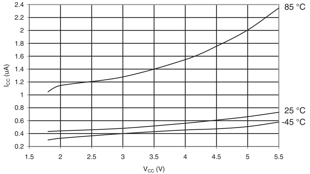
Figure 29-375. ATmega649A: Power-down Supply Current vs. V_{CC} (Watchdog Timer Disabled)
