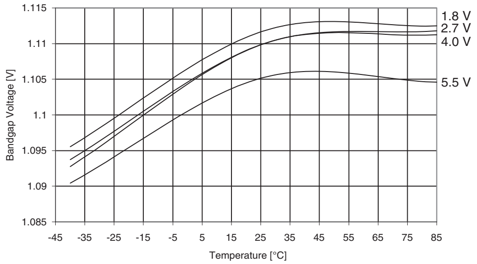
Figure 29-168. ATmega329A: Bandgap Voltage vs. Temperature
