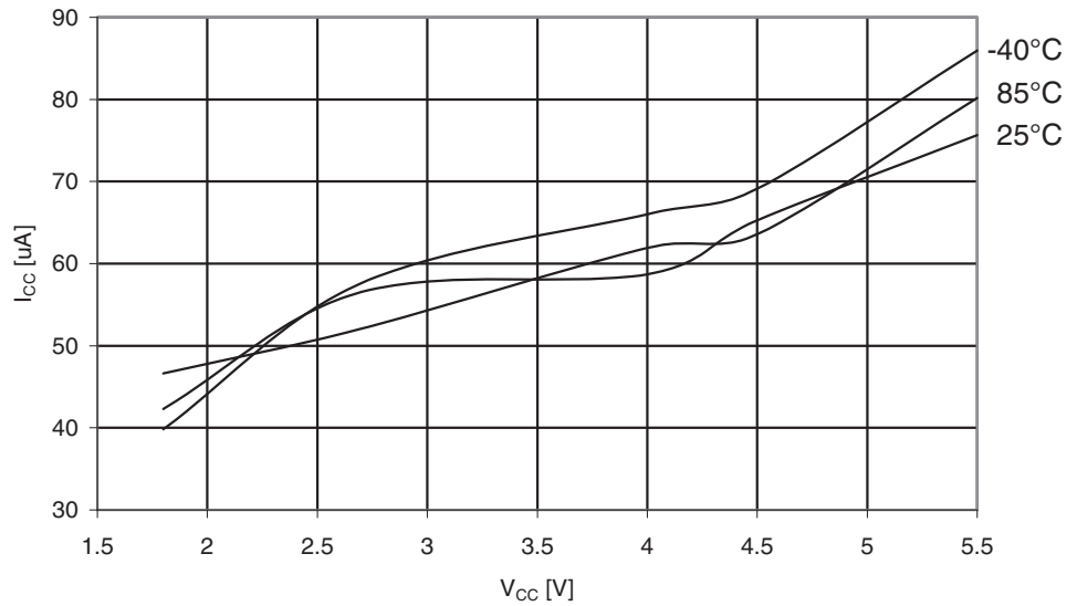
Figure 29-300. ATmega3290A: Analog Comparator Current vs. V_{CC}
