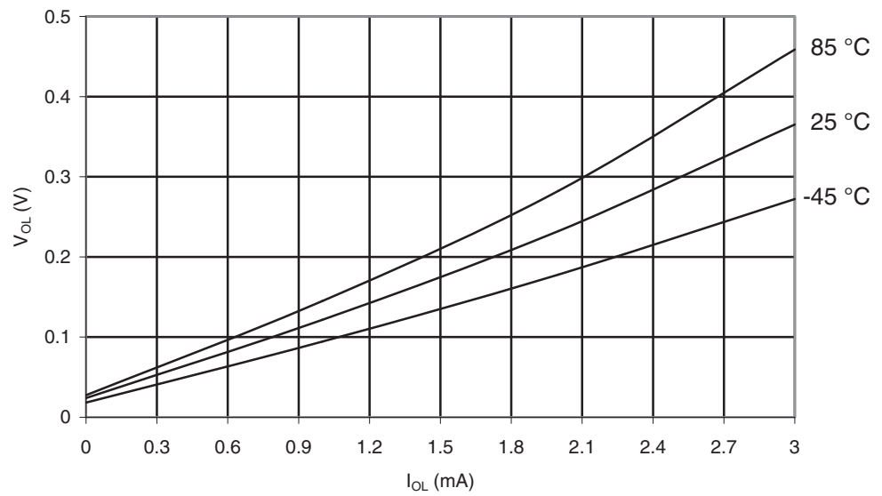
Figure 29-30. ATmega169A: I/O Pin Output Voltage vs. Sink Current, Ports A, C, D, E, F, G ( V_{CC} = 1.8V )
