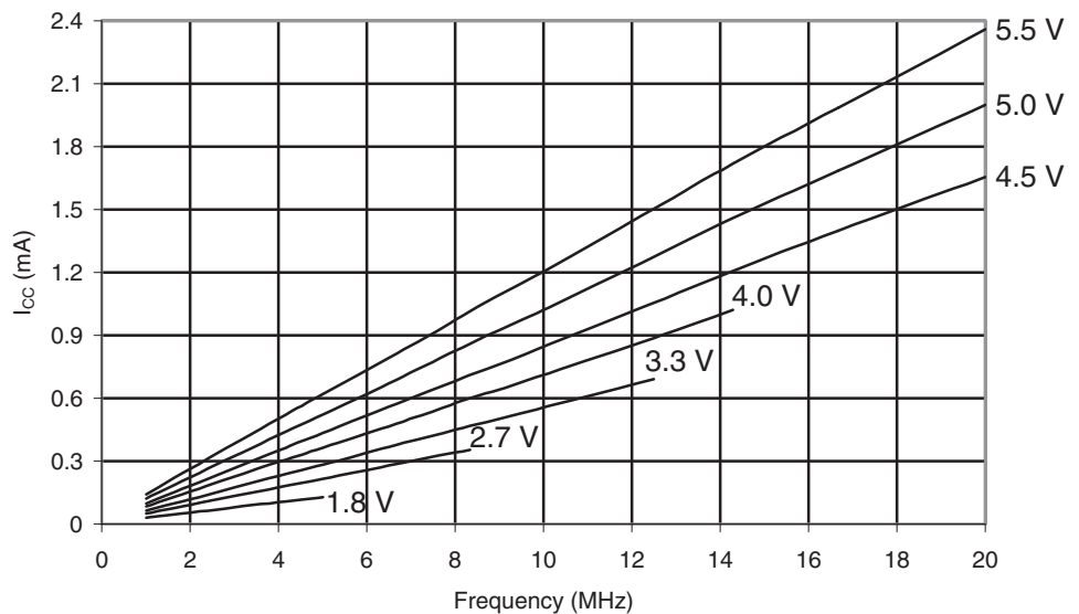
Figure 29-607. ATmega6490P: Reset Supply Current vs. V_{CC} (1 - 16 MHz, Excluding Current Through The Reset Pull-up)
