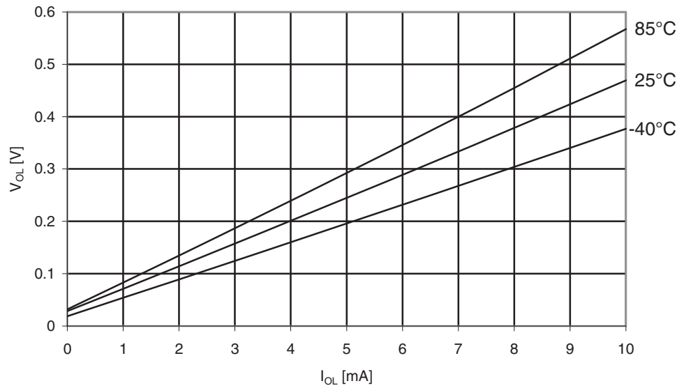
Figure 29-272. ATmega3290A: I/O Pin Output Voltage vs. Sink Current, Ports A, C, D, E, F, G ( V_{CC} = 5V )
