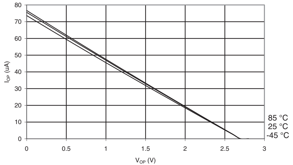
Figure 29-79. ATmega169PA: I/O Pin Pull-up Resistor Current vs. Input Voltage ( V_{CC} = 2.7V )
