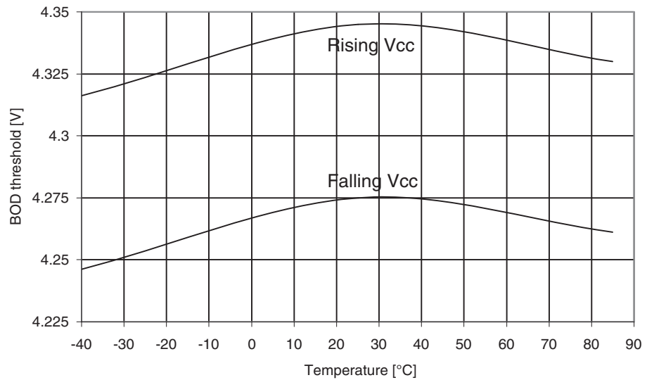
Figure 29-284. ATmega3290A: BOD Thresholds vs. Temperature (BOD Level is 4.3V)
