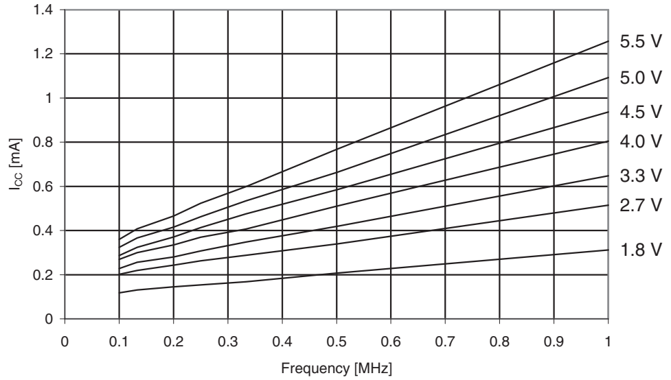
Figure 29-245. ATmega3290A: Active Supply Current vs. Low Frequency (0.1 - 1.0 MHz)
