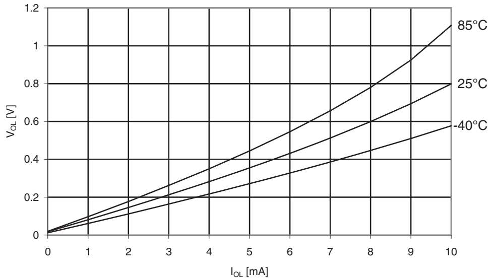
Figure 29-333. ATmega3290PA. I/O Pin Output Voltage vs. Sink Current, Ports A, C, D, E, F, G ( V_{CC} = 2.7V )
