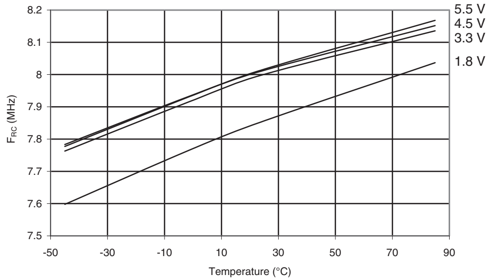
Figure 29-111. ATmega169PA: Calibrated 8 MHz RC Oscillator Frequency vs. Temperature
