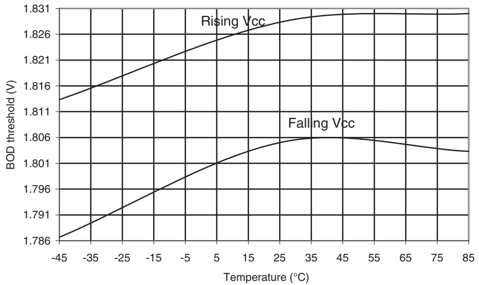
Figure 29-104. ATmega169PA: BOD Thresholds vs. Temperature (BOD Level is 1.8V)
