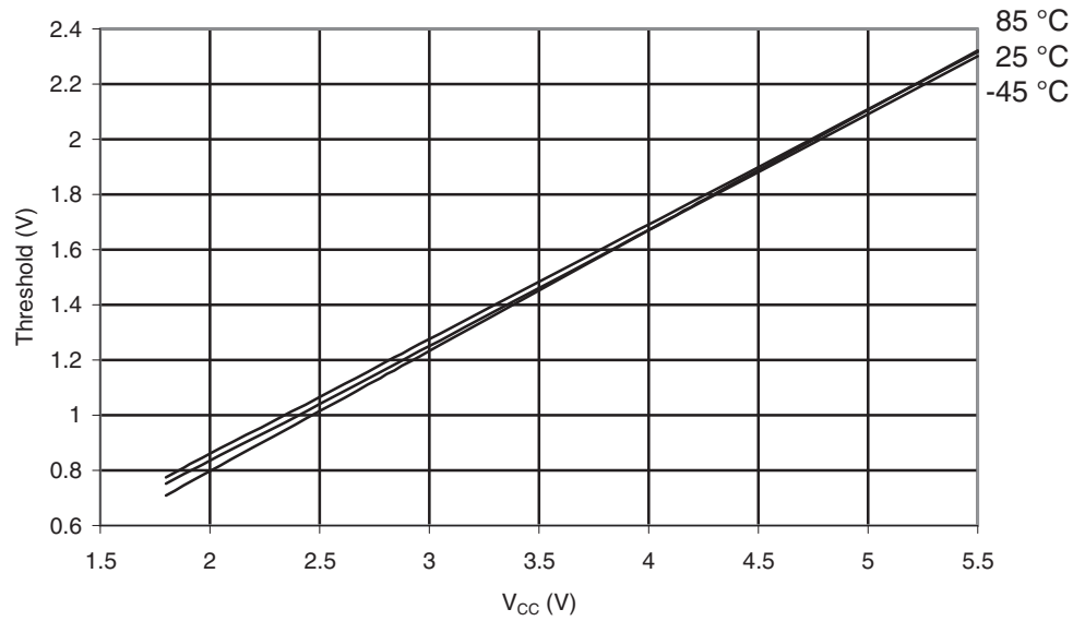
Figure 29-464. ATmega649P: Reset Input Threshold Voltage vs. V_{CC} ( V_{IL} , Reset Pin Read as "0")
