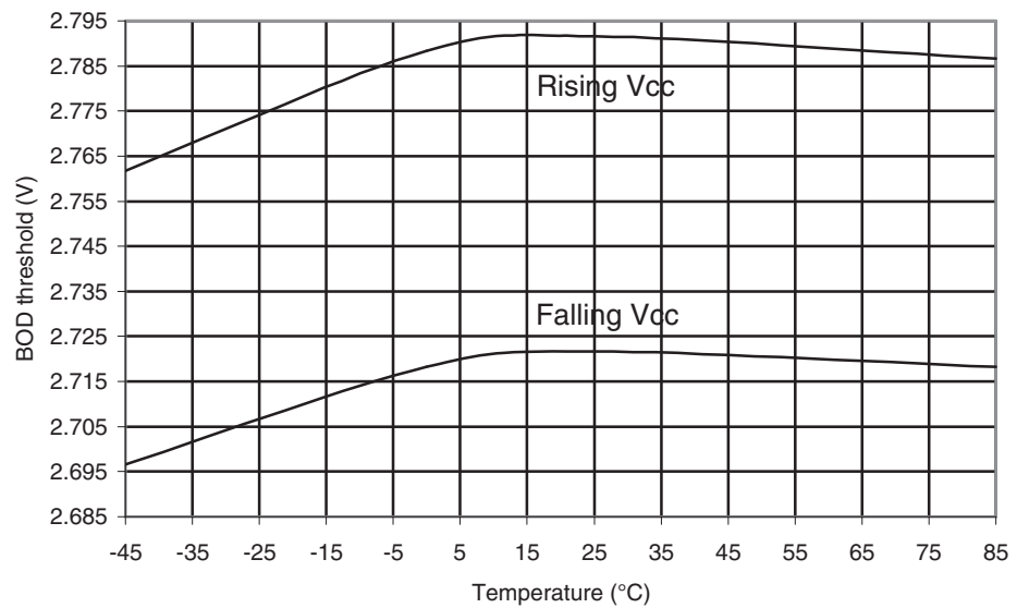
Figure 29-406. ATmega649A: BOD Thresholds vs. Temperature (BOD Level is 2.7V)
