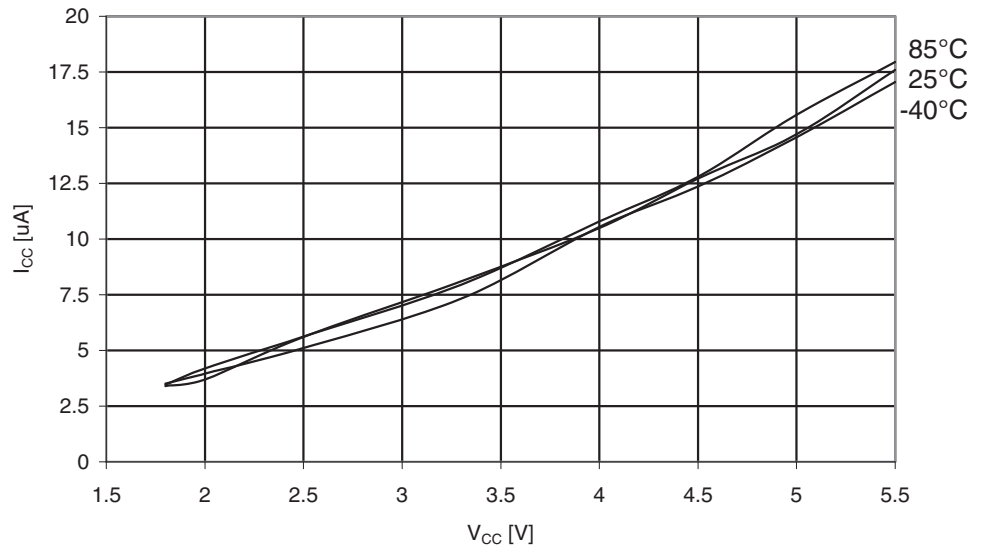
Figure 29-179. ATmega329A: Watchdog Timer Current vs. V_{CC}
