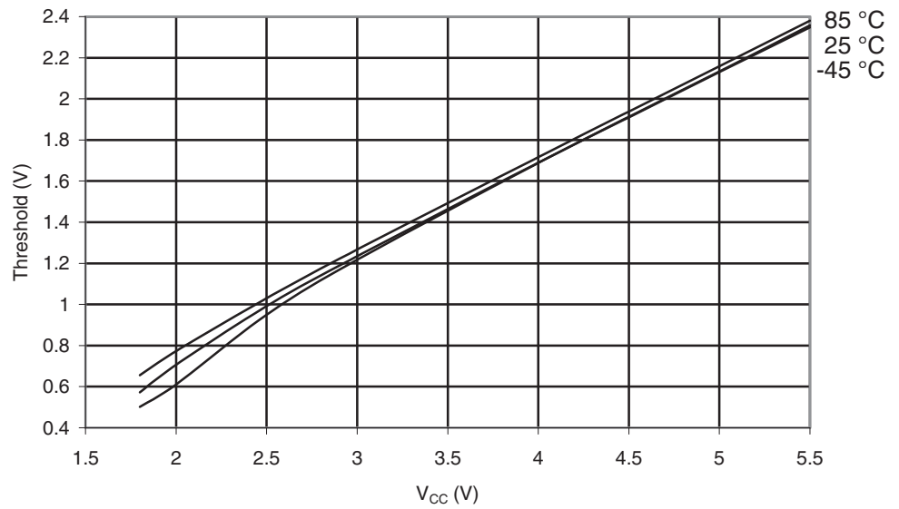
Figure 29-461. ATmega649P: I/O Pin Input Threshold Voltage vs. V_{CC} ( V_{IL} , I/O Pin Read as "0")
