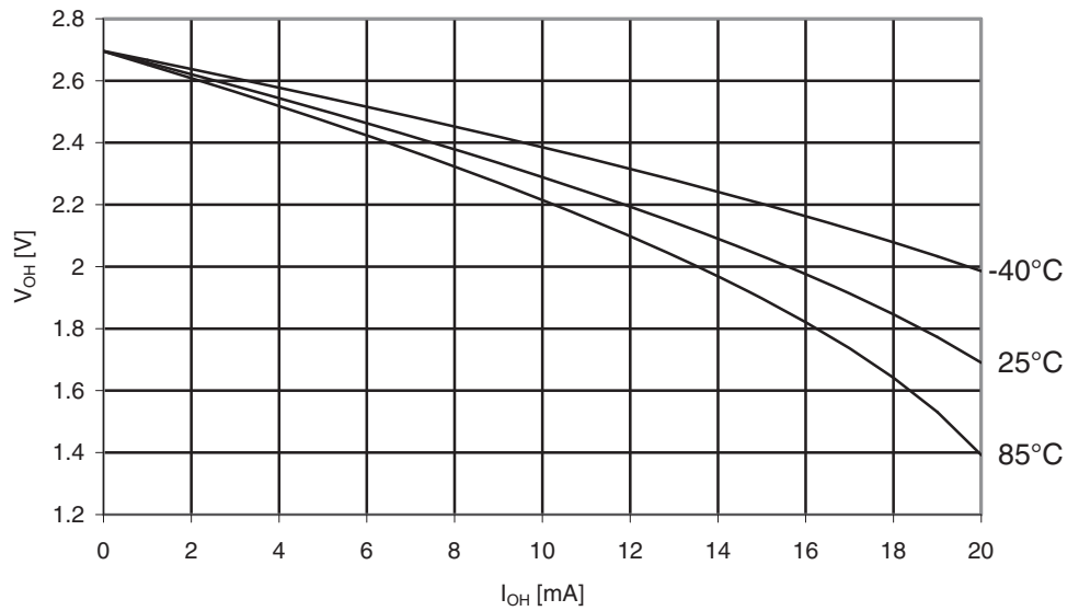
Figure 29-150. ATmega329A: I/O Pin Output Voltage vs. Source Current, Port B ( V_{CC} = 2.7V )
