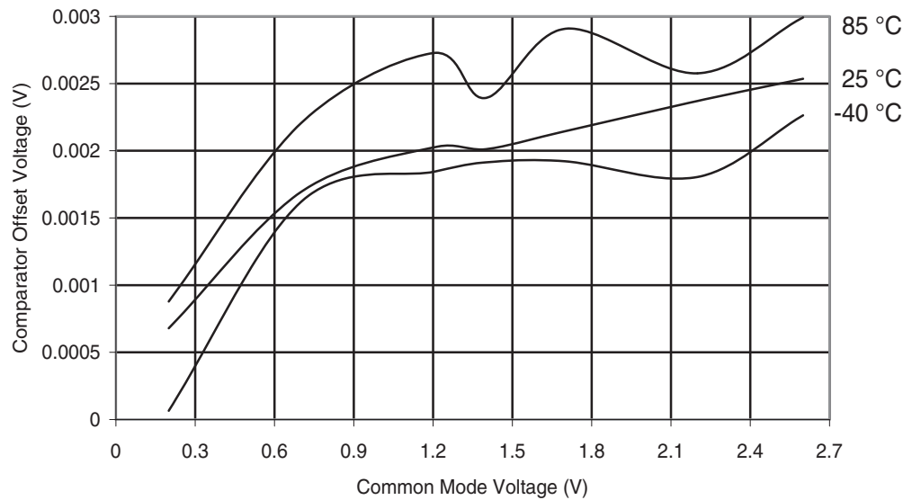
Figure 29-46. ATmega169A: Analog Comparator Offset Voltage vs. Common Mode Voltage ( V_{CC} = 2.7V )
