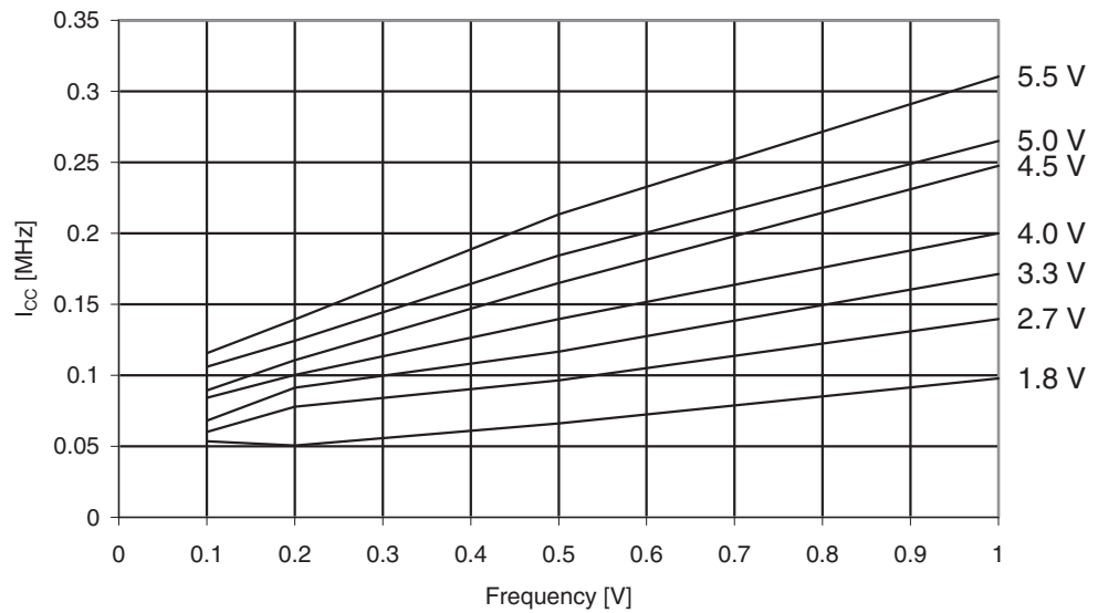
Figure 29-310. ATmega3290PA: Idle Supply Current vs. Low Frequency (0.1 - 1.0 MHz)
