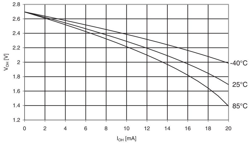
Figure 29-210. ATmega329PA: I/O Pin Output Voltage vs. Source Current, Port B ( V_{CC} = 2.7V )
