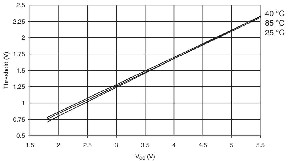
Figure 29-282. ATmega3290A: Reset Input Threshold Voltage vs. V_{CC} ( V_{IL} , Reset Pin Read as "0")
