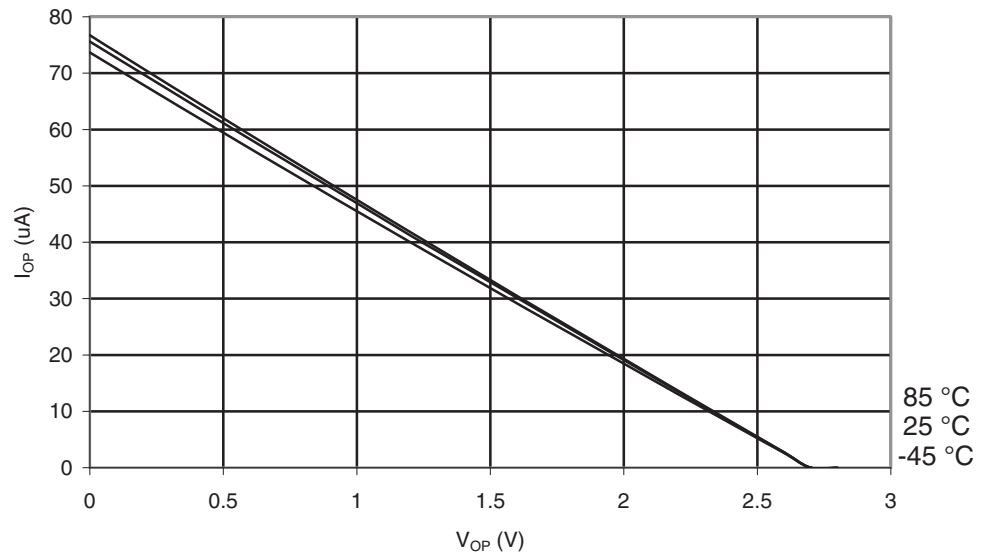
Figure 29-17. ATmega169A: I/O Pin Pull-up Resistor Current vs. Input Voltage ( V_{CC} = 2.7V )
