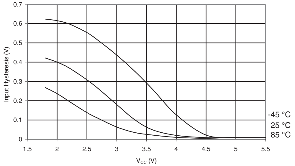
Figure 29-39. ATmega169A: Reset Input Pin Hysteresis vs. V_{CC}
