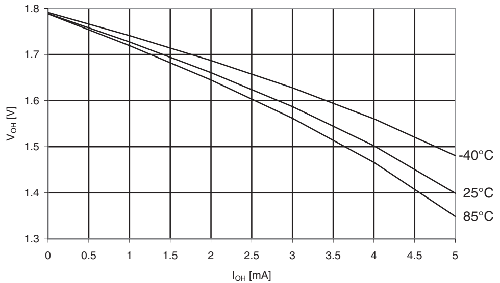
Figure 29-151. ATmega329A: I/O Pin Output Voltage vs. Source Current, Port B ( V_{CC} = 1.8V )
