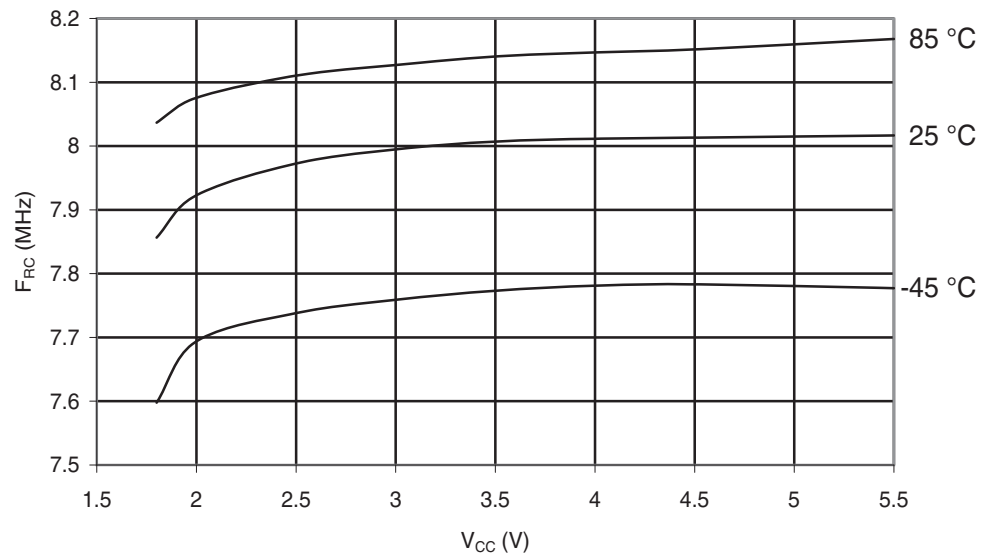
Figure 29-50. ATmega169A: Calibrated 8 MHz RC Oscillator Frequency vs. V_{CC}
