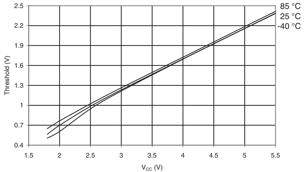
Figure 29-159. ATmega329A: I/O Pin Input Threshold Voltage vs. V_{CC} ( V_{IL} , I/O Pin Read as "0")
