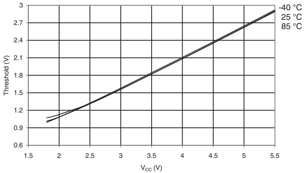
Figure 29-218. ATmega329PA: I/O Pin Input Threshold Voltage vs. V_{CC} ( V_{IH} , I/O Pin Read as "1")
