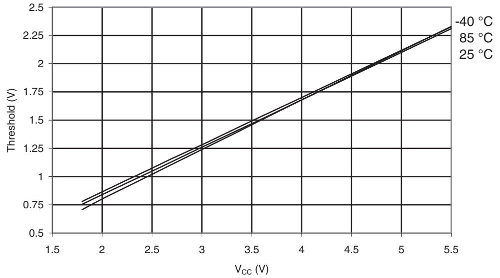
Figure 29-222. ATmega329PA: Reset Input Threshold Voltage vs. V_{CC} ( V_{IL} , Reset Pin Read as "0")
