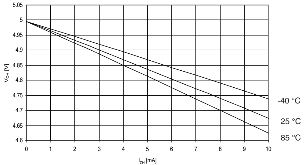
Figure 29-266. ATmega3290A: I/O Pin Output Voltage vs. Source Current, Ports A, C, D, E, F, G ( V_{CC} = 5V )
