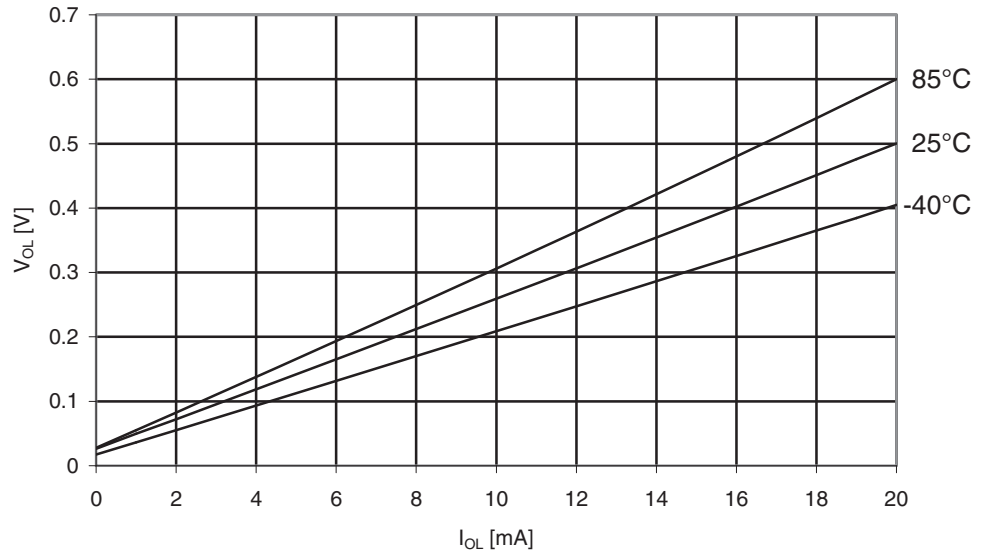
Figure 29-155. ATmega329A: I/O Pin Output Voltage vs. Sink Current, Port B ( V_{CC} = 5V )
