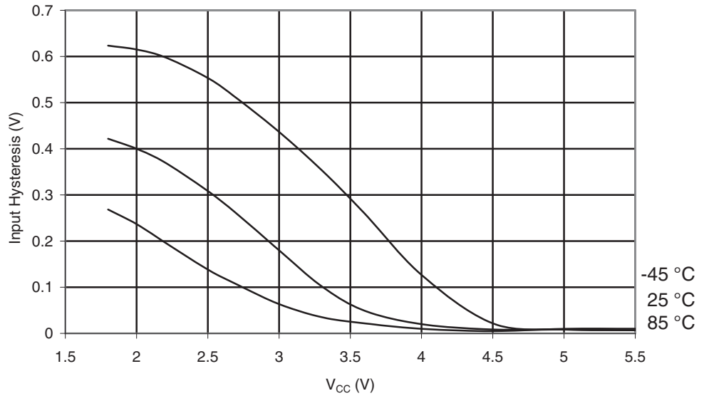
Figure 29-101. ATmega169PA: Reset Input Pin Hysteresis vs. V_{CC}
