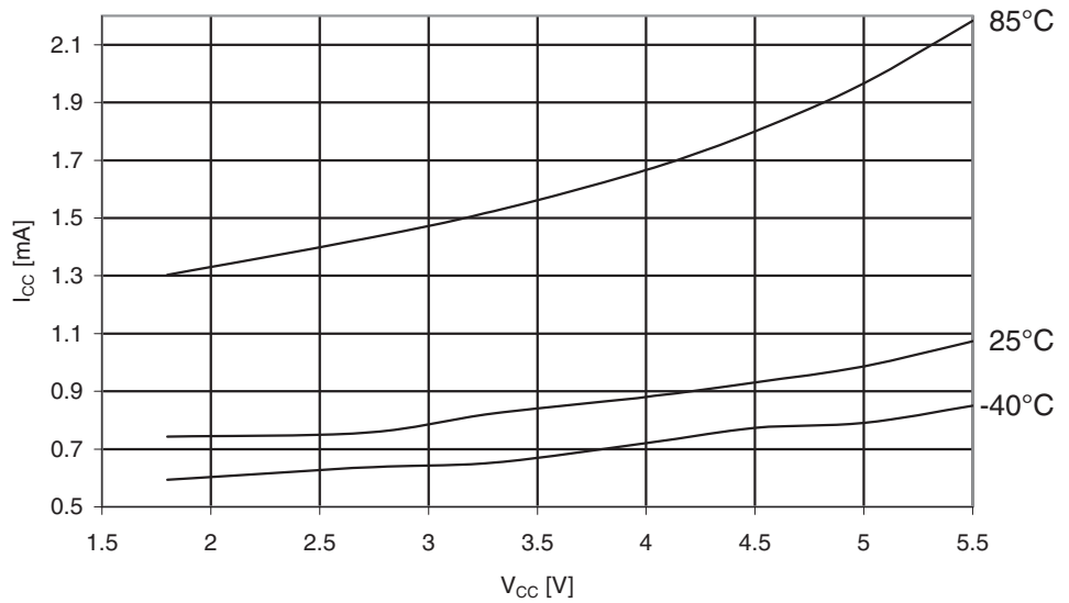
Figure 29-198. ATmega329PA Standby Supply Current vs. V_{CC} (32 kHz Watch Crystal, Watchdog Timer Disabled)
