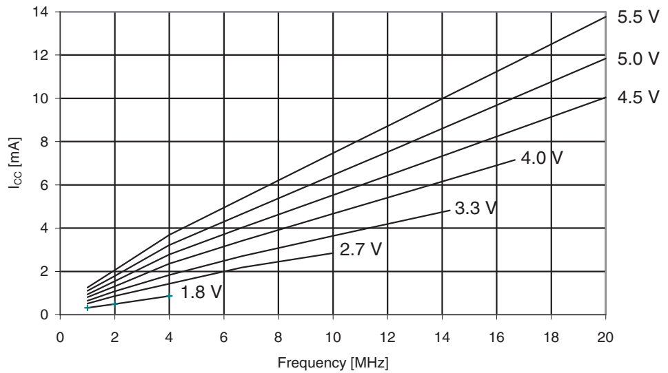
Figure 29-306. ATmega3290PA: Active Supply Current vs. Frequency (1 - 20MHz)
