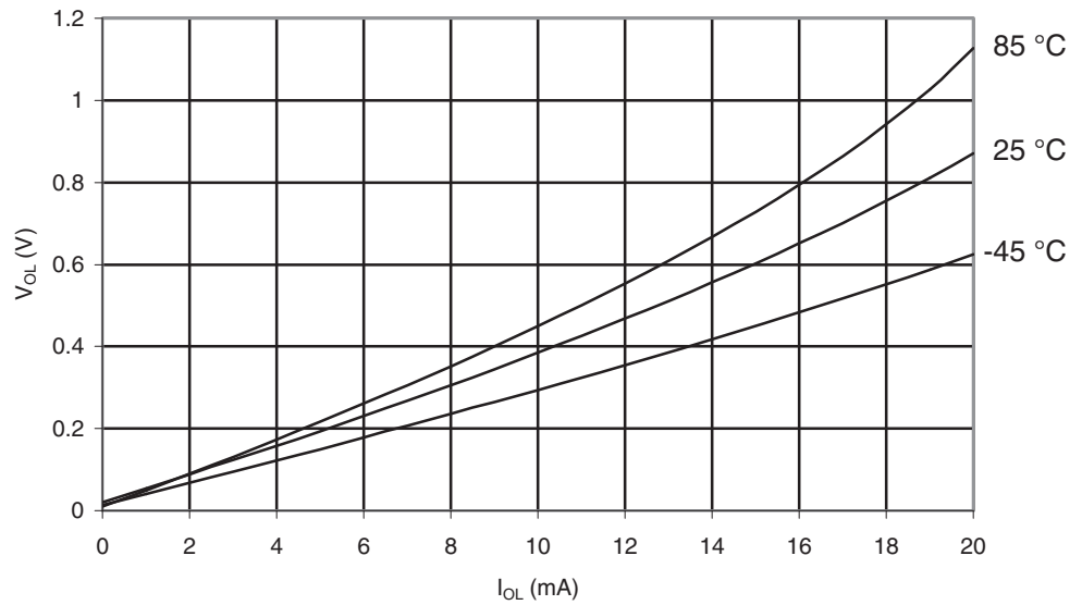
Figure 29-519. ATmega6490A: I/O Pin Output Voltage vs. Sink Current, Port B ( V_{CC} = 2.7V_9 )
