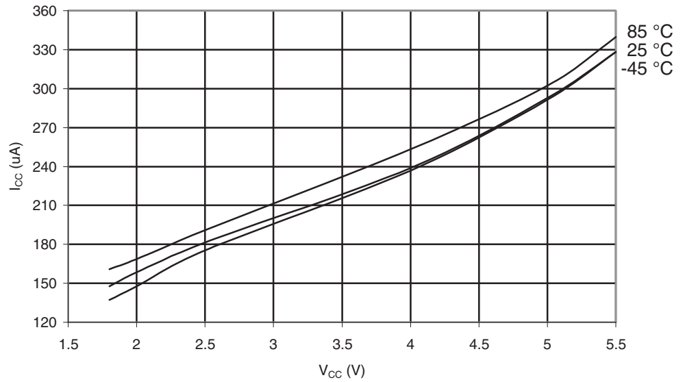
Figure 29-539. ATmega6490A: Active Supply Current with ADC at 200 kHz vs. V_{CC}
