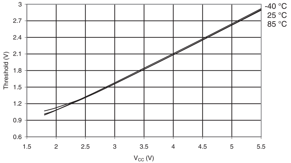
Figure 29-158. ATmega329A: I/O Pin Input Threshold Voltage vs. V_{CC} ( V_{IH} , I/O Pin Read as "1")
