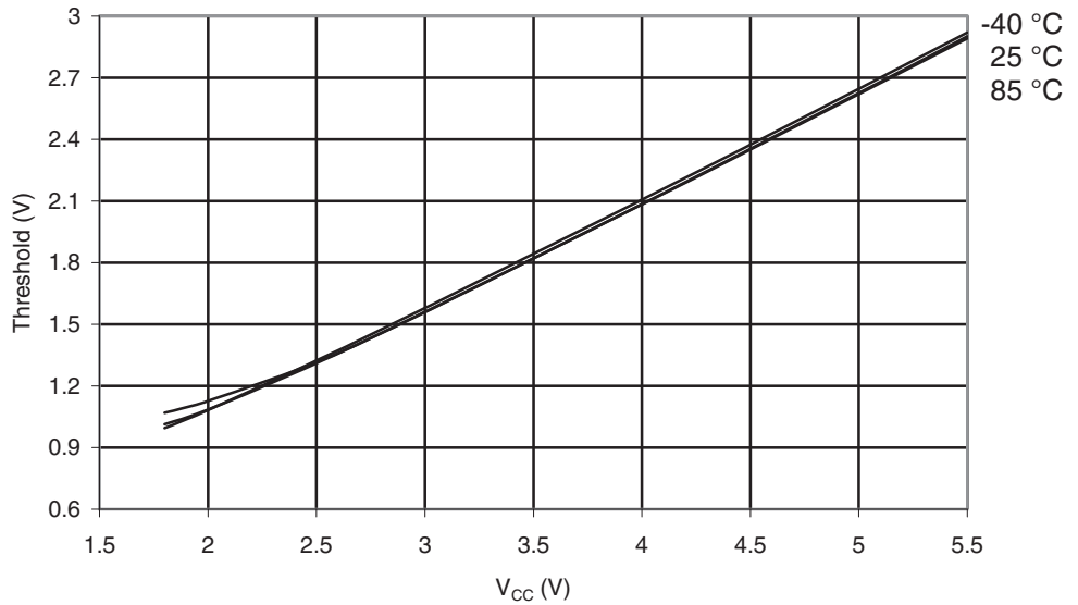
Figure 29-278. ATmega3290A: I/O Pin Input Threshold Voltage vs. V_{CC} ( V_{IH} , I/O Pin Read as "1")
