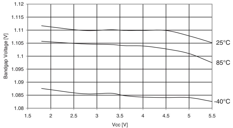
Figure 29-167. ATmega329A: Bandgap Voltage vs. V CC
