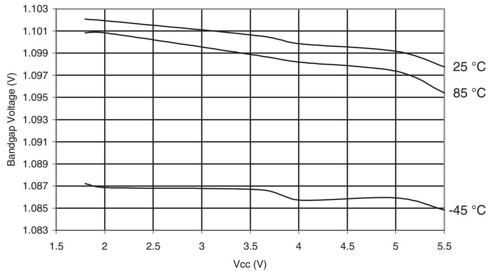
Figure 29-530. ATmega6490A: Bandgap Voltage vs. V CC
