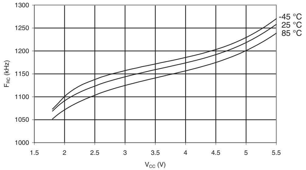
Figure 29-109. ATmega169PA: Watchdog Oscillator Frequency vs. V_{CC}
