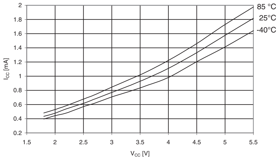
Figure 29-132. ATmega329A: Idle Supply Current vs. V_{CC} (Internal RC Oscillator, 8 MHz)
