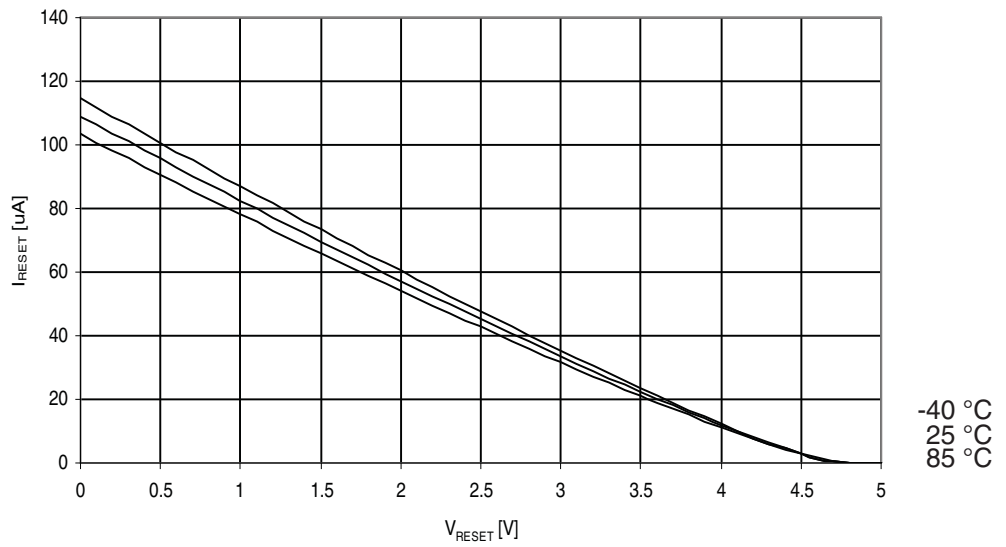
Figure 29-143. ATmega329A: Reset Pull-up Resistor Current vs. Reset Pin Voltage ( V_{CC} = 5V )
