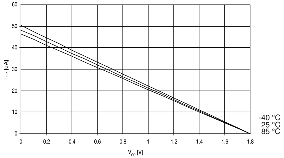
Figure 29-142. ATmega329A: I/O Pin Pull-up Resistor Current vs. Input Voltage ( V_{CC} = 1.8V )
