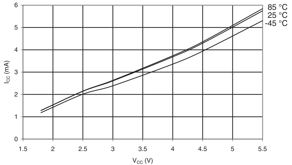
Figure 29-3. ATmega169A: Active Supply Current vs. V_{CC} (Internal RC Oscillator, 8 MHz)
