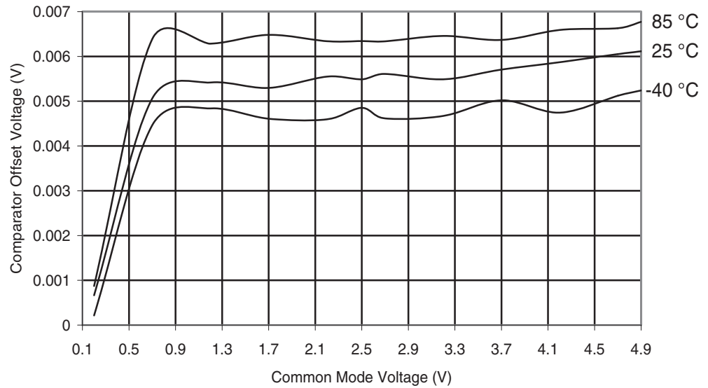
Figure 29-45. ATmega169A: Analog Comparator Offset Voltage vs. Common Mode Voltage ( V_{CC} = 5V )
