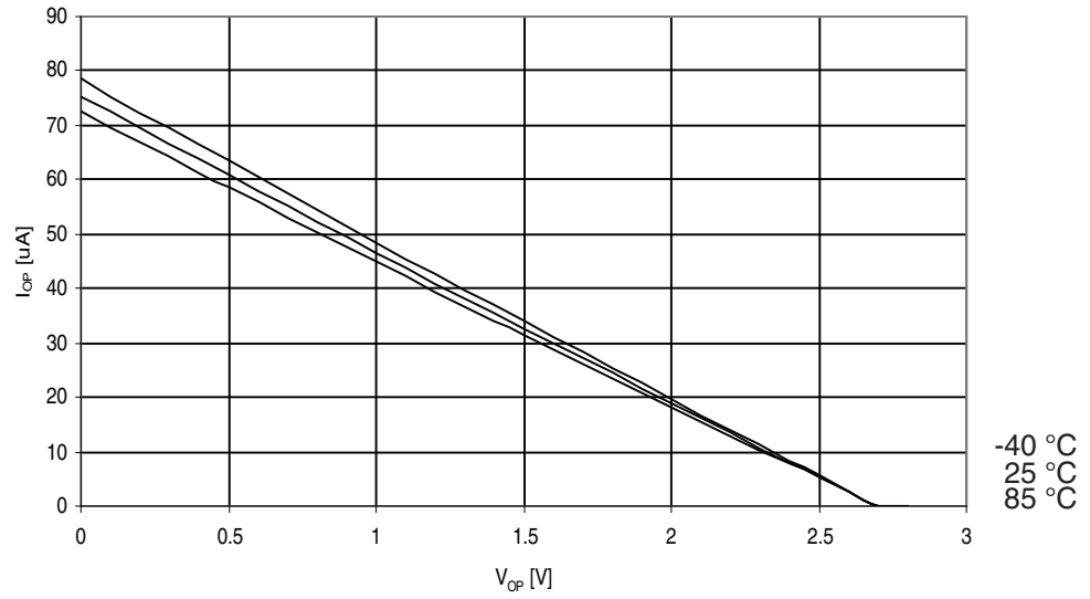
Figure 29-261. ATmega3290A: I/O Pin Pull-up Resistor Current vs. Input Voltage ( V_{CC} = 2.7V )
