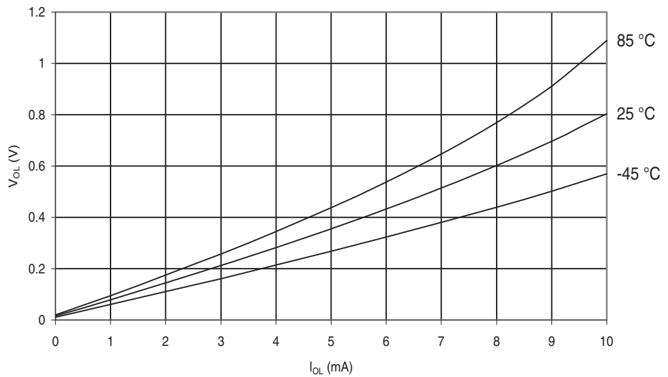
Figure 29-516. ATmega6490A: I/O Pin Output Voltage vs. Sink Current, Ports A, C, D, E, F, G ( V_{CC} = 2.7V )
