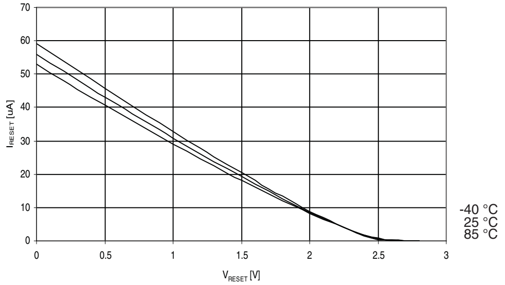
Figure 29-324. ATmega3290PA: Reset Pull-up Resistor Current vs. Reset Pin Voltage ( V_{CC} = 2.7V )
