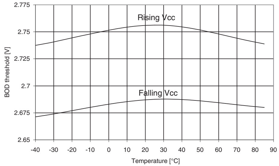
Figure 29-285. ATmega3290A: BOD Thresholds vs. Temperature (BOD Level is 2.7V)
