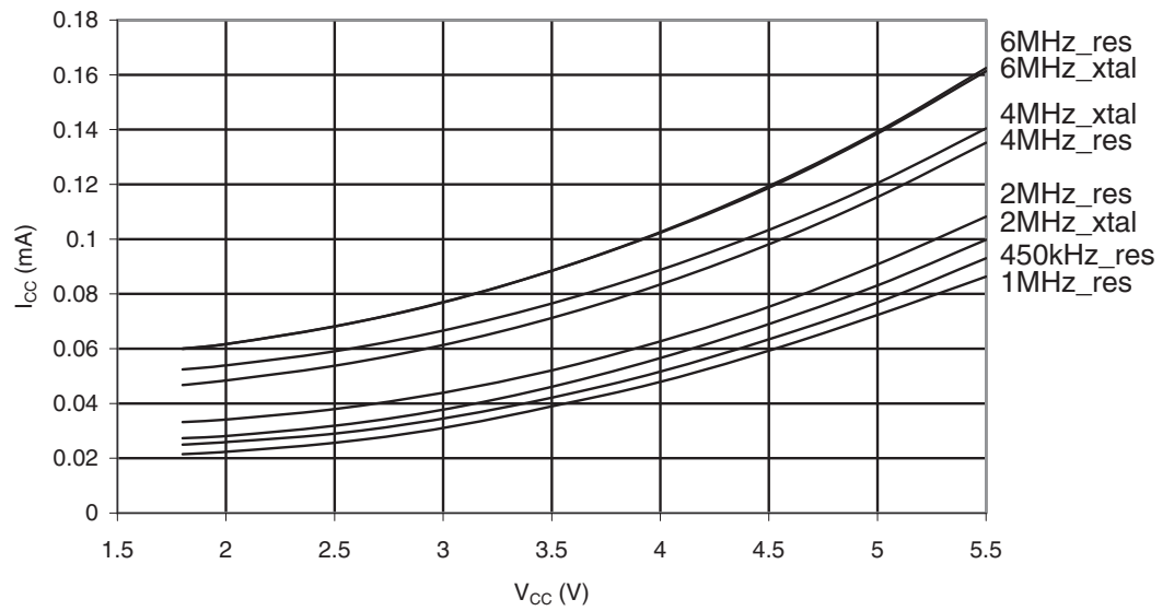
Figure 29-15. ATmega169A: Standby Supply Current vs. V_{CC} (Xtall and Resonator, Watchdog Timer Disabled)
