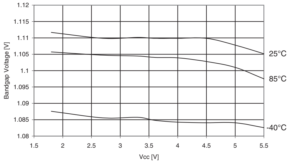
Figure 29-227. ATmega329PA: Bandgap Voltage vs. V CC
