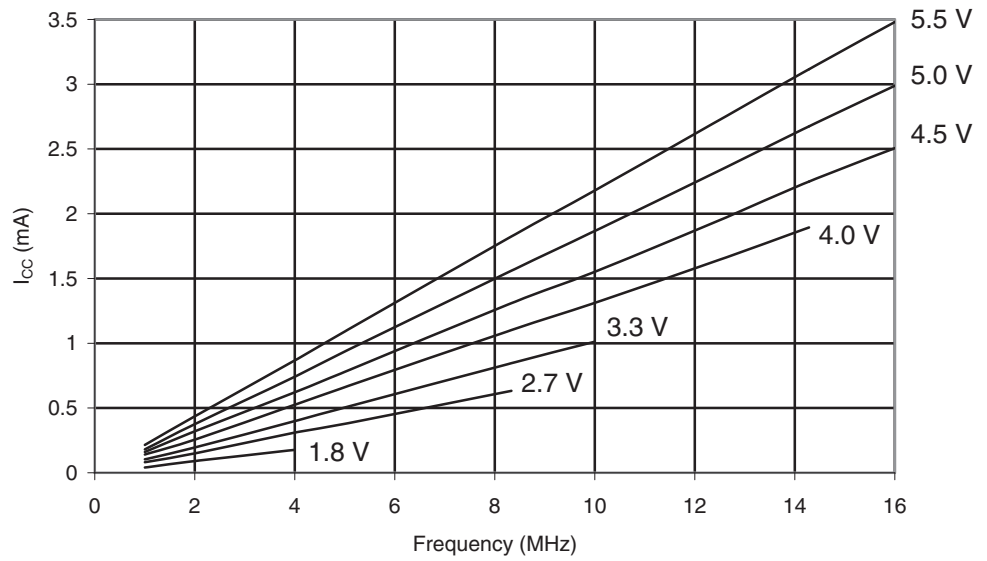
Figure 29-69. ATmega169PA: Idle Supply Current vs. Frequency (1 - 16 MHz)
