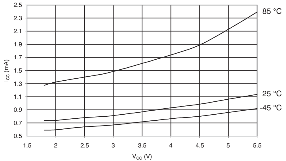
Figure 29-378. ATmega649A: Power-save Supply Current vs. V_{CC} (Watchdog Timer Disabled and 32 kHz Crystal Oscillator Running)
