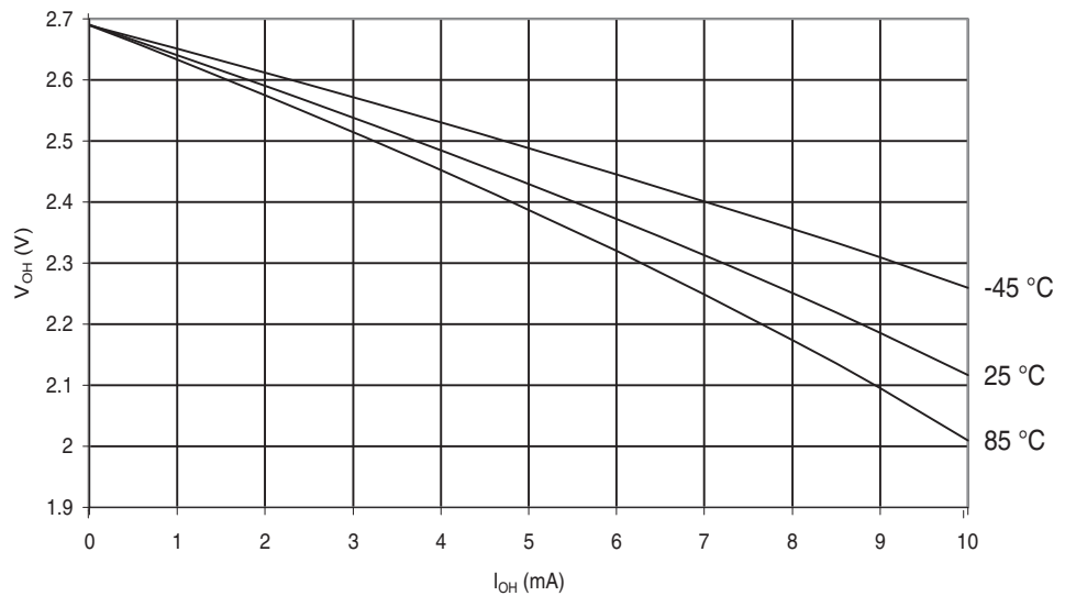
Figure 29-449. ATmega649P: I/O Pin Output Voltage vs. Source Current, Ports A, C, D, E, F, G ( V_{CC} = 2.7V )
