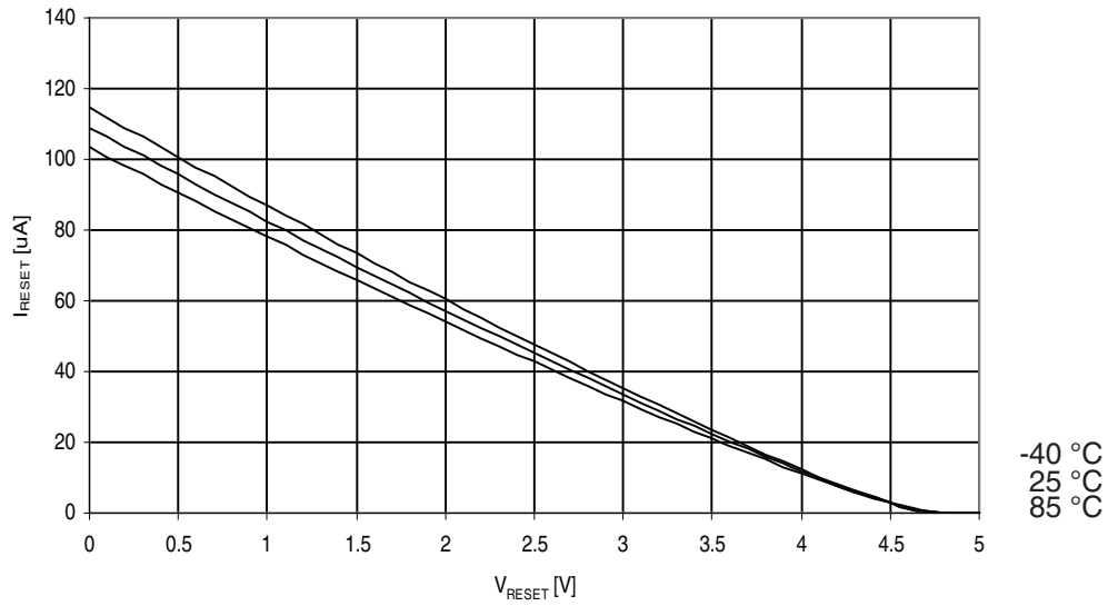
Figure 29-263. ATmega3290A: Reset Pull-up Resistor Current vs. Reset Pin Voltage ( V_{CC} = 5V )
