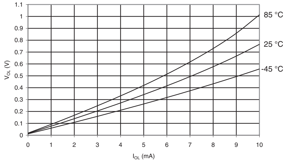
Figure 29-29. ATmega169A. I/O Pin Output Voltage vs. Sink Current, Ports A, C, D, E, F, G ( V_{CC} = 2.7V )
