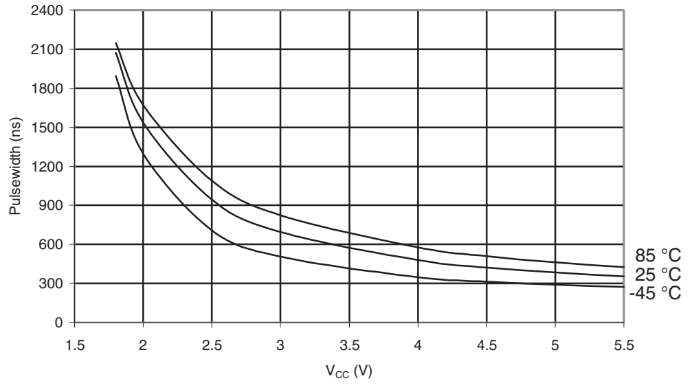
Figure 29-608. ATmega6490P: Minimum Reset Pulse Width vs. V_{CC}
