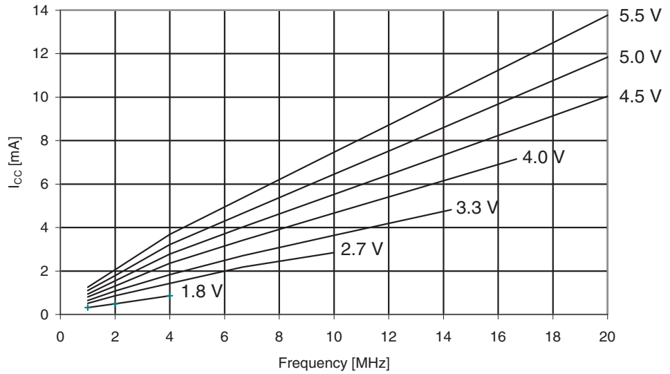
Figure 29-126. ATmega329A: Active Supply Current vs. Frequency (1 - 20MHz)
