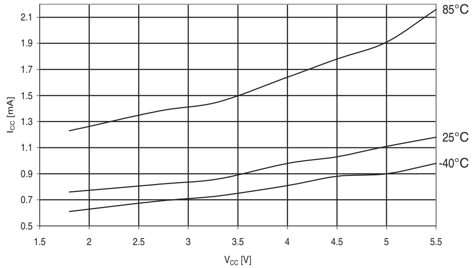
Figure 29-317. ATmega3290PA: Power-save Supply Current vs. V_{CC} (Watchdog Timer Disabled and 32 kHz Crystal Oscillator Running)
