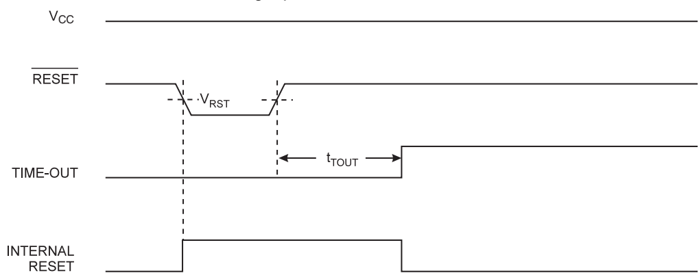
Figure 10-4. External Reset During Operation
