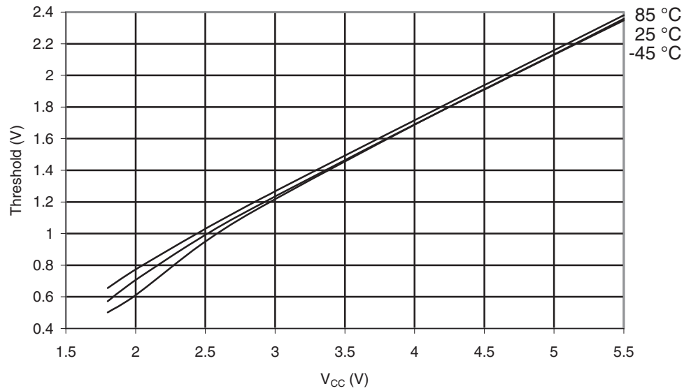
Figure 29-522. ATmega6490A: I/O Pin Input Threshold Voltage vs. V_{CC} ( V_{IL} , I/O Pin Read as "0")
