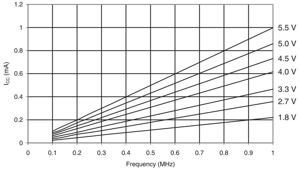
Figure 29-63. ATmega169PA: Active Supply Current vs. Frequency (0.1 - 1.0 MHz)
