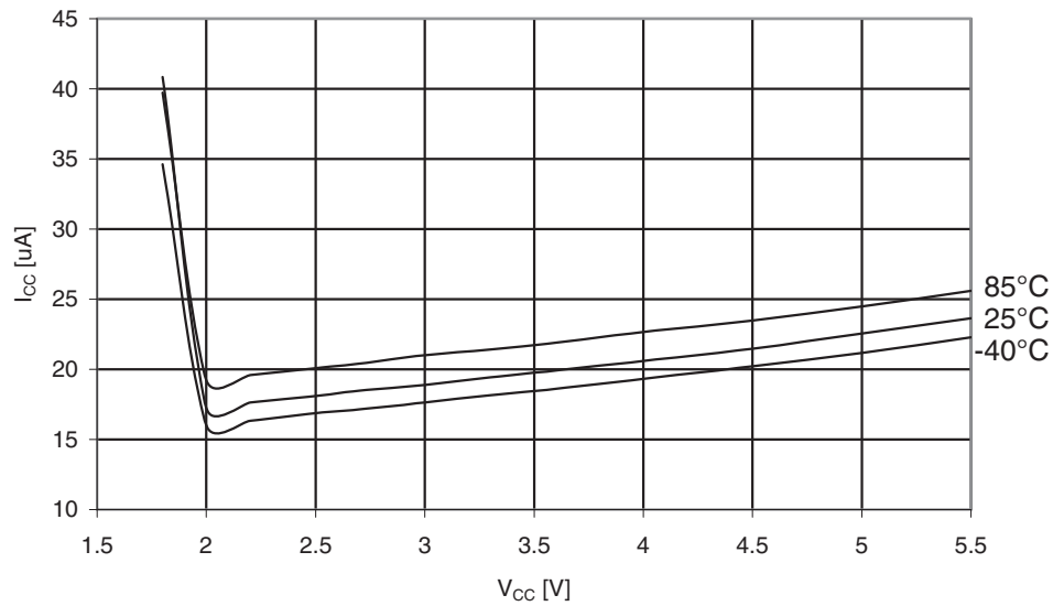
Figure 29-294. ATmega3290A: Brownout Detector Current vs. V_{CC}
