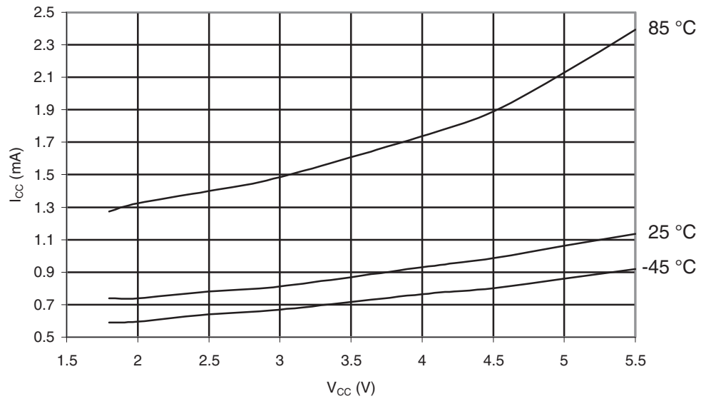
Figure 29-500. ATmega6490A: Power-save Supply Current vs. V_{CC} (Watchdog Timer Disabled and 32 kHz Crystal Oscillator Running)
