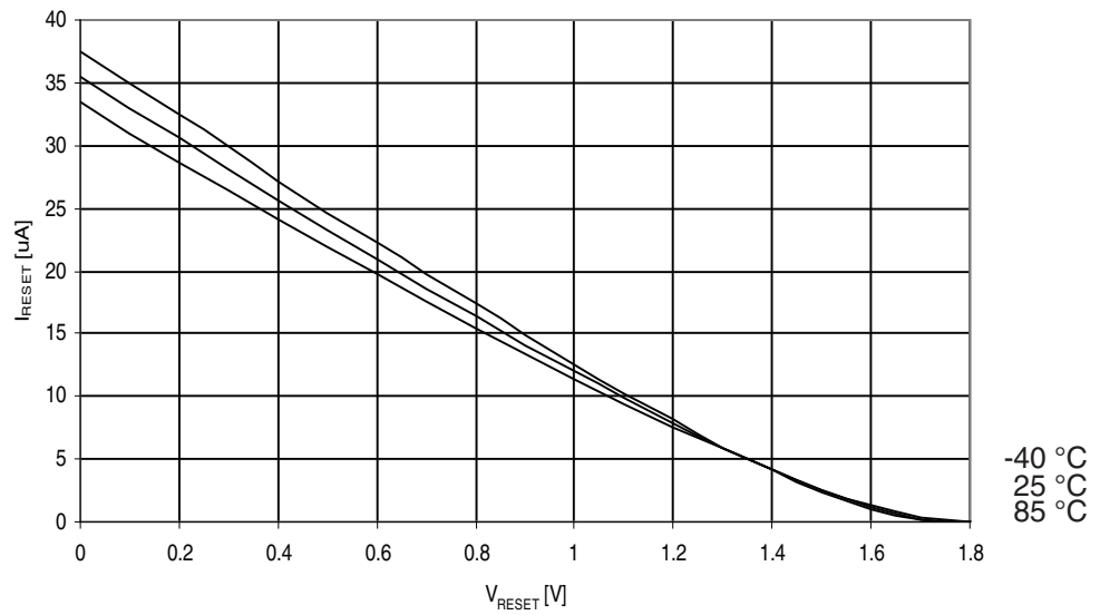
Figure 29-145. ATmega329A: Reset Pull-up Resistor Current vs. Reset Pin Voltage ( V_{CC} = 1.8V )
