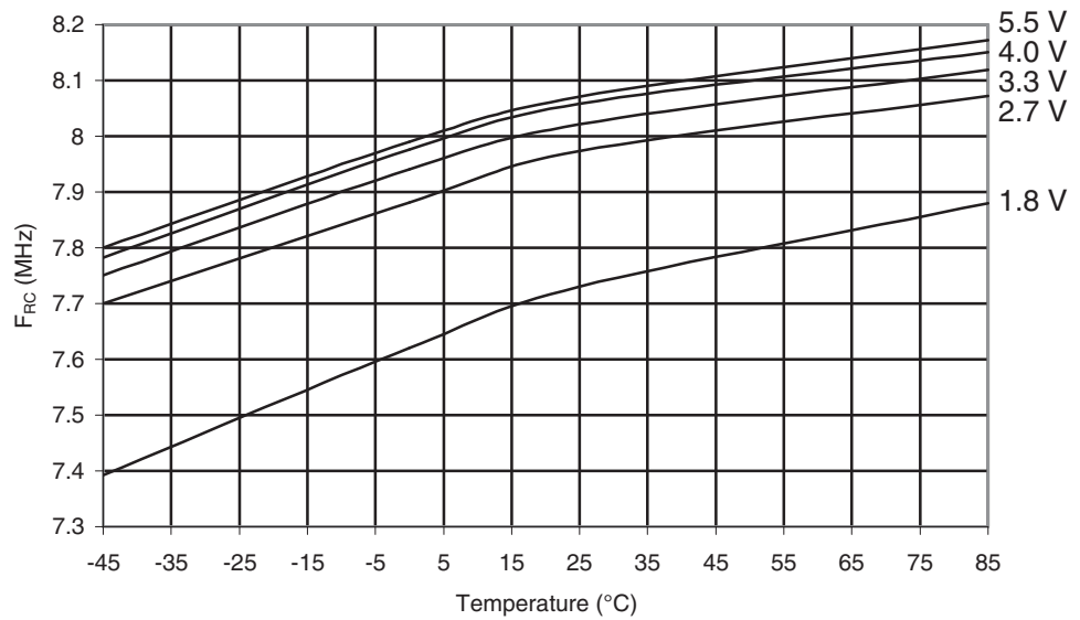
Figure 29-412. ATmega649A: Calibrated 8 MHz RC Oscillator Frequency vs. Temperature
