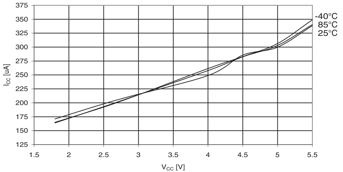
Figure 29-357. ATmega3290PA: Active Supply Current with ADC at 1 MHz vs. V_{CC}
