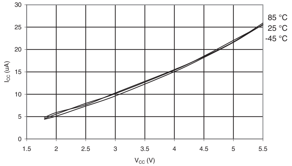
Figure 29-119. ATmega169PA: Watchdog Timer Current vs. V_{CC}
