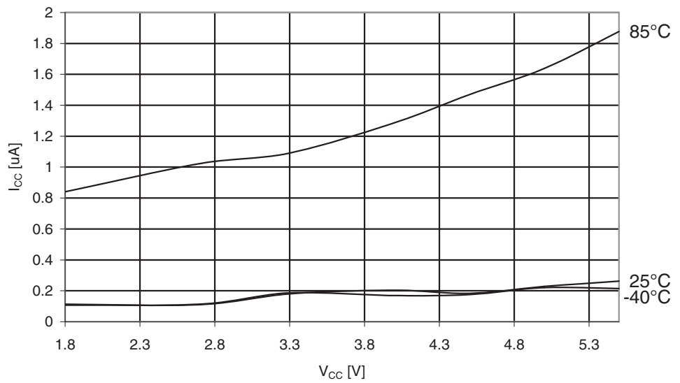
Figure 29-256. ATmega3290A: Power-down Supply Current vs. V_{CC} (Watchdog Timer Enabled)
