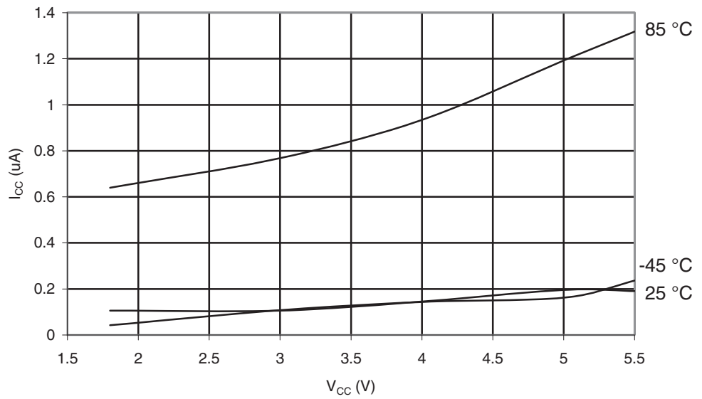
Figure 29-73. ATmega169PA: Power-down Supply Current vs. V_{CC} (Watchdog Timer Disabled)
