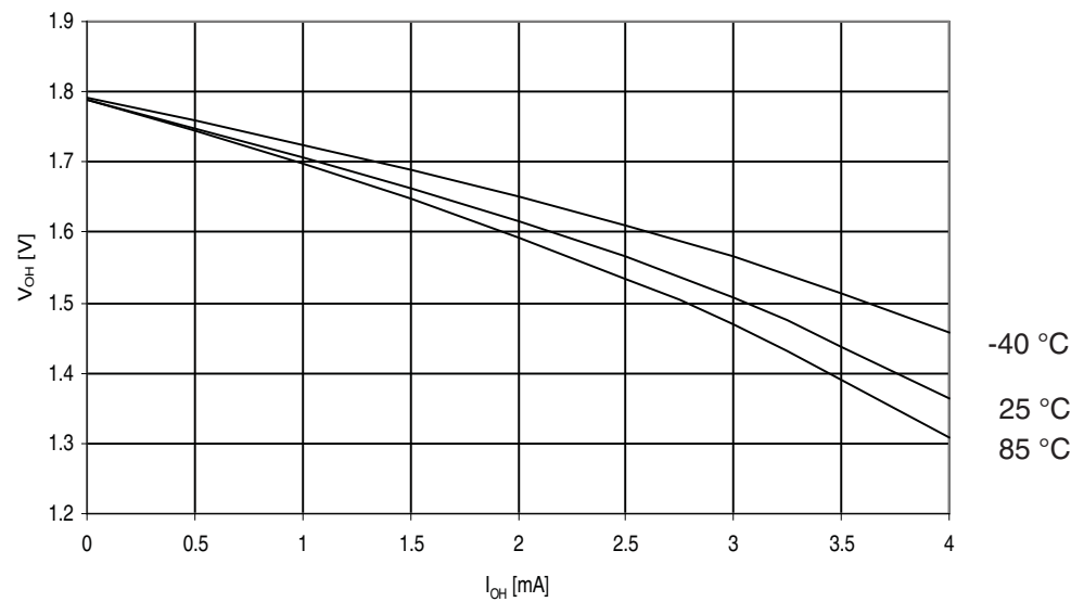
Figure 29-268. ATmega3290A: I/O Pin Output Voltage vs. Source Current, Ports A, C, D, E, F, G ( V_{CC} = 1.8V )
