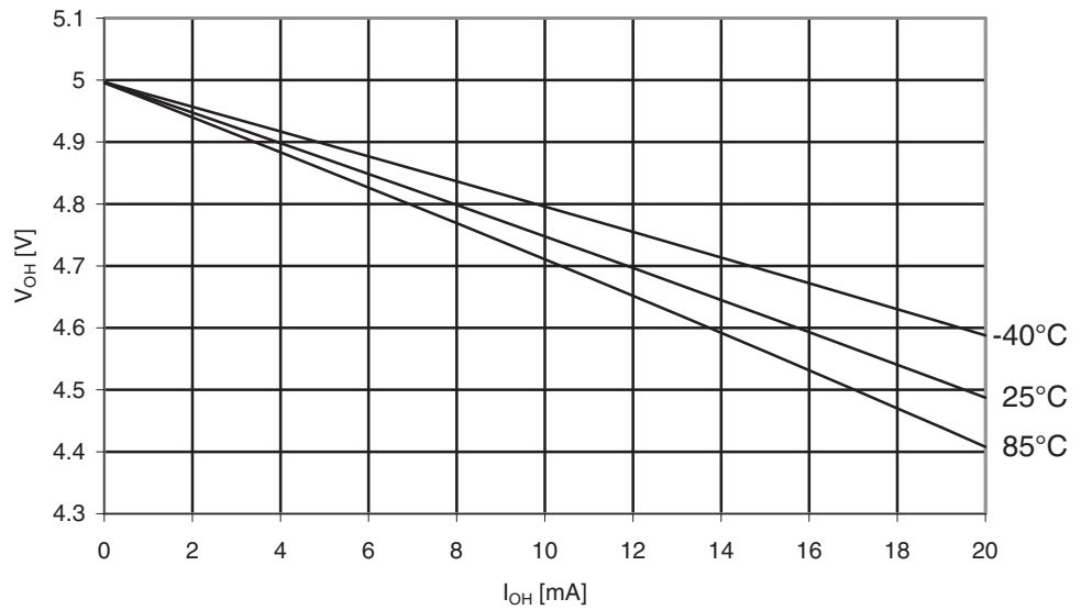
Figure 29-329. ATmega3290PA: I/O Pin Output Voltage vs. Source Current, Port B ( V_{CC} = 5V )
