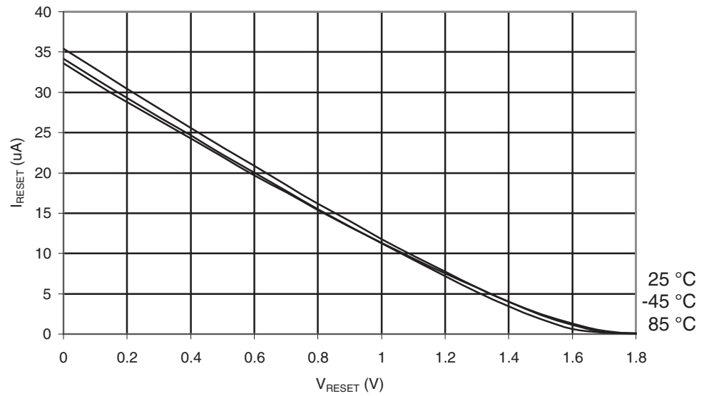
Figure 29-569. ATmega6490P: Reset Pull-up Resistor Current vs. Reset Pin Voltage ( V_{CC} = 1.8V )
