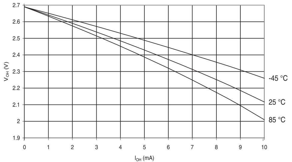
Figure 29-388. ATmega649A: I/O Pin Output Voltage vs. Source Current, Ports A, C, D, E, F, G ( V_{CC} = 2.7V )
