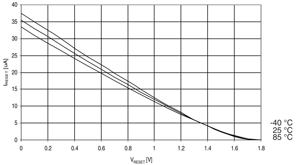
Figure 29-265. ATmega3290A: Reset Pull-up Resistor Current vs. Reset Pin Voltage ( V_{CC} = 1.8V )
