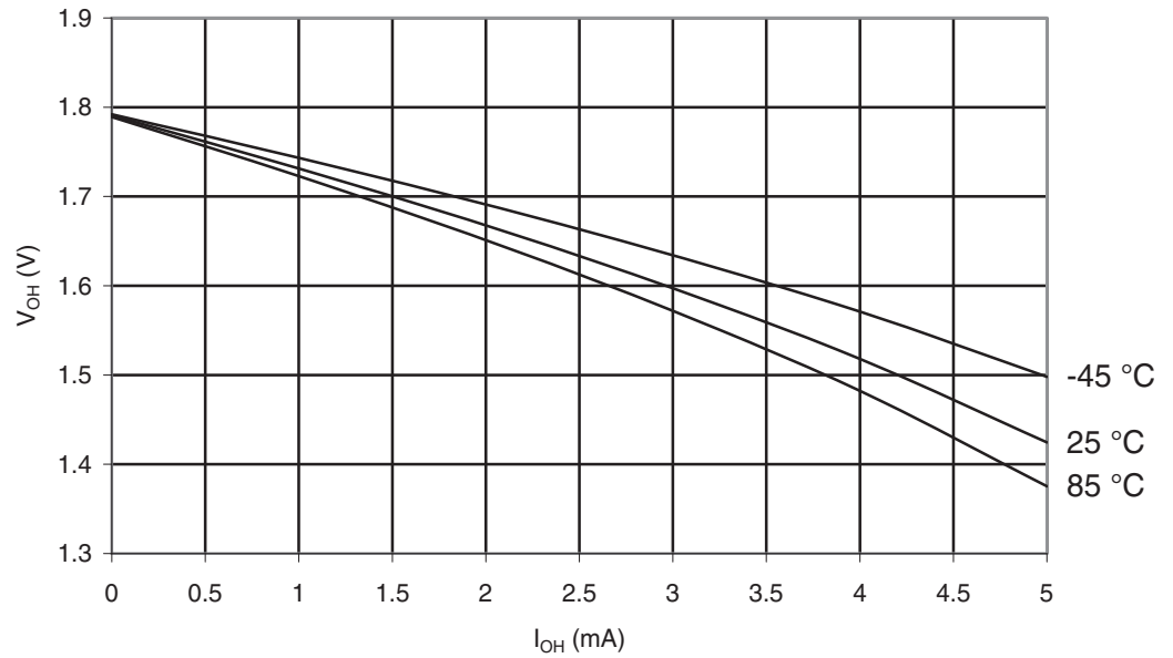
Figure 29-89. ATmega169PA: I/O Pin Output Voltage vs. Source Current, Port B ( V_{CC} = 1.8V )
