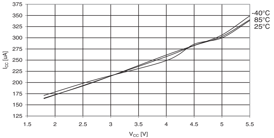
Figure 29-237. ATmega329PA: Active Supply Current with ADC at 1 MHz vs. V_{CC}
