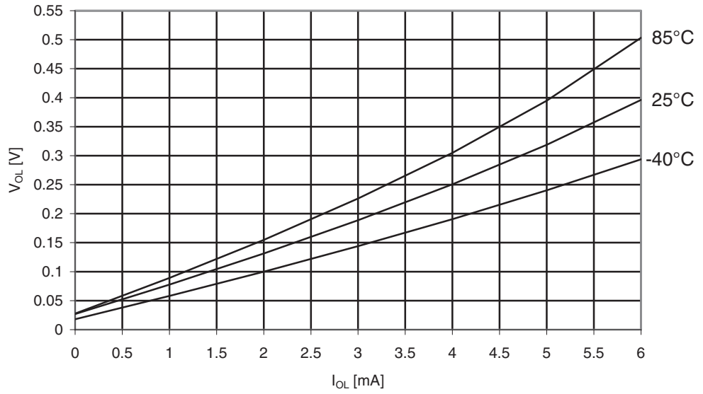
Figure 29-277. ATmega3290A: I/O Pin Output Voltage vs. Sink Current, Port B ( V_{CC} = 1.8V )
