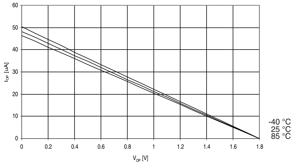
Figure 29-262. ATmega3290A: I/O Pin Pull-up Resistor Current vs. Input Voltage ( V_{CC} = 1.8V )
