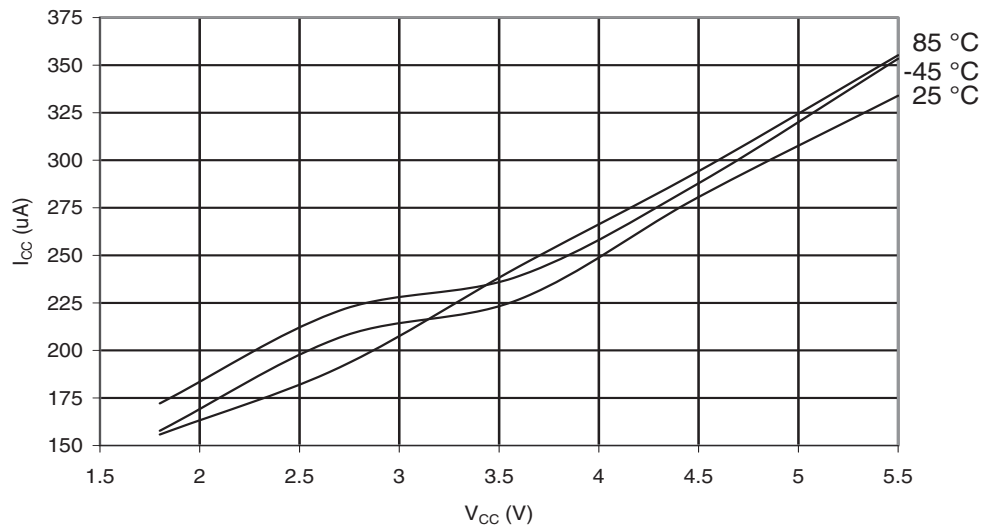
Figure 29-54. ATmega169A: Active Supply Current with ADC at 200 kHz vs. V_{CC}
