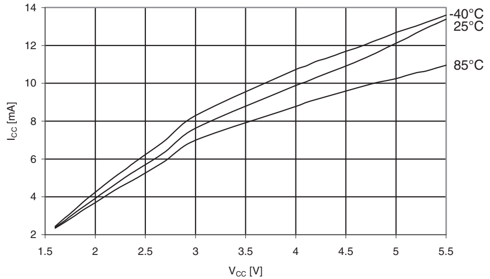
Figure 29-301. ATmega3290A: Programming Current vs. V_{CC}
