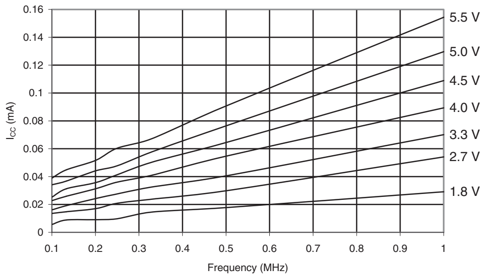
Figure 29-60. ATmega169A: Reset Supply Current vs. V_{CC} (0.1 - 1.0 MHz, Excluding Current Through The Reset Pull-up)
