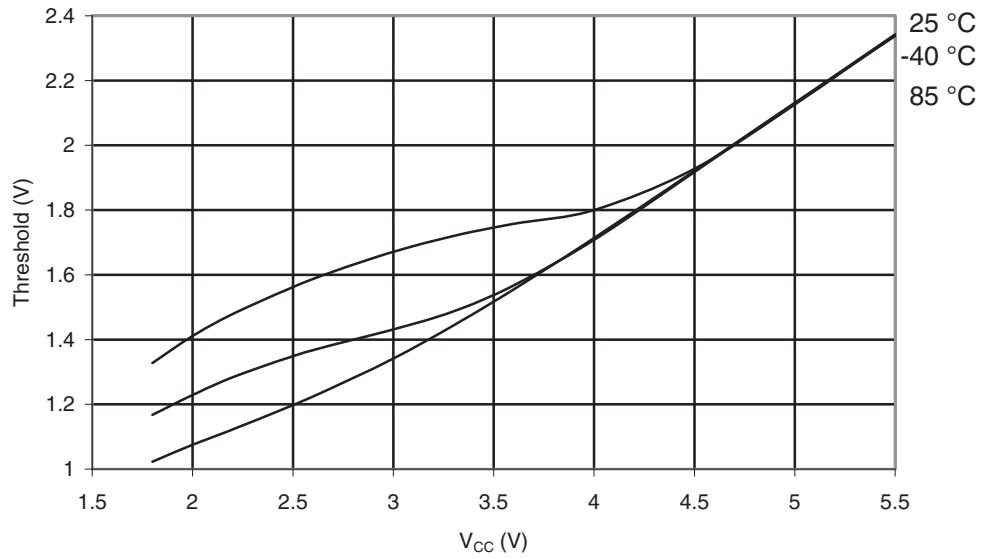
Figure 29-281. ATmega3290A: Reset Input Threshold Voltage vs. V_{CC} ( V_{IH} , Reset Pin Read as "1")
