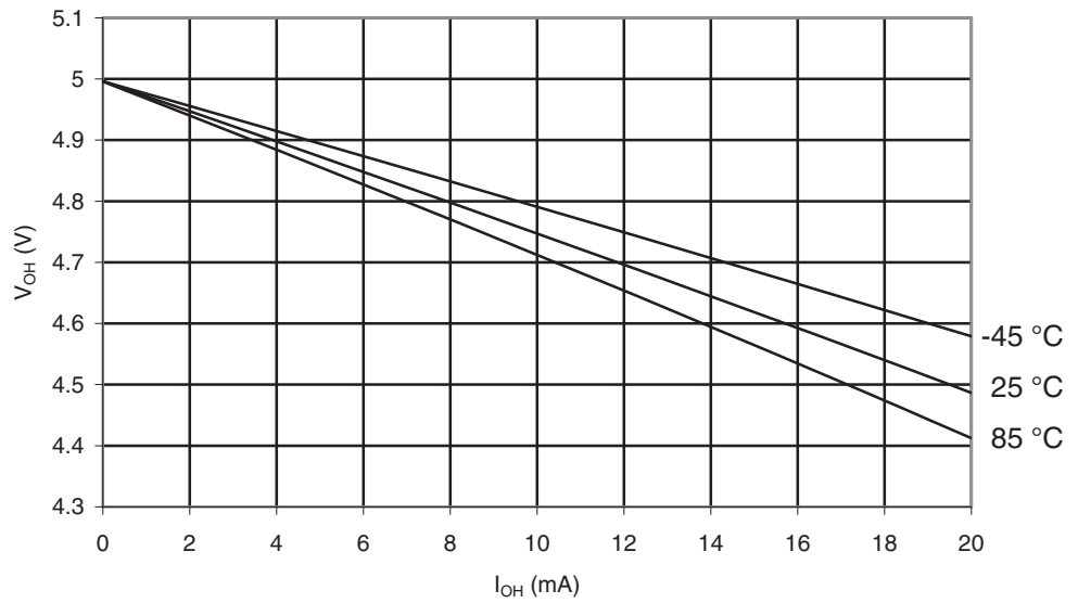
Figure 29-25. ATmega169A: I/O Pin Output Voltage vs. Source Current, Port B ( V_{CC} = 5V )
