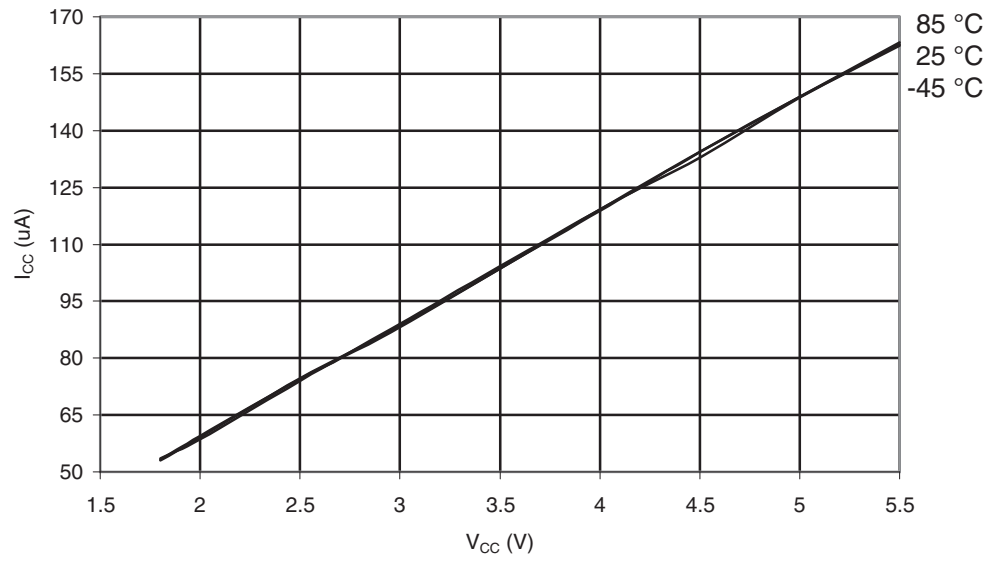
Figure 29-419. ATmega649A: AREF External Reference Current vs. V_{CC}
