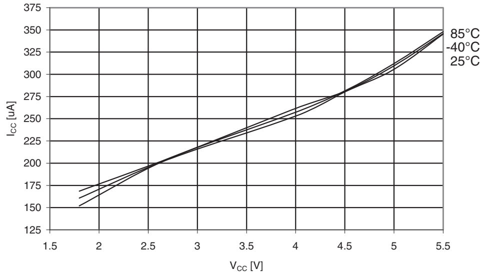
Figure 29-176. ATmega329A: Active Supply Current with ADC at 200 kHz vs. V_{CC}
