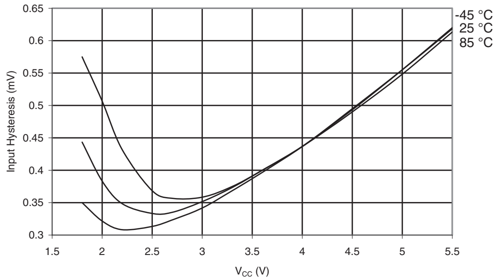
Figure 29-36. ATmega169A: I/O Pin Input Hysteresis vs. V_{CC}
