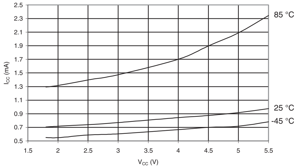
Figure 29-502. ATmega6490A: Standby Supply Current vs. V_{CC} (Xtall and Resonator, Watchdog Timer Disabled)
