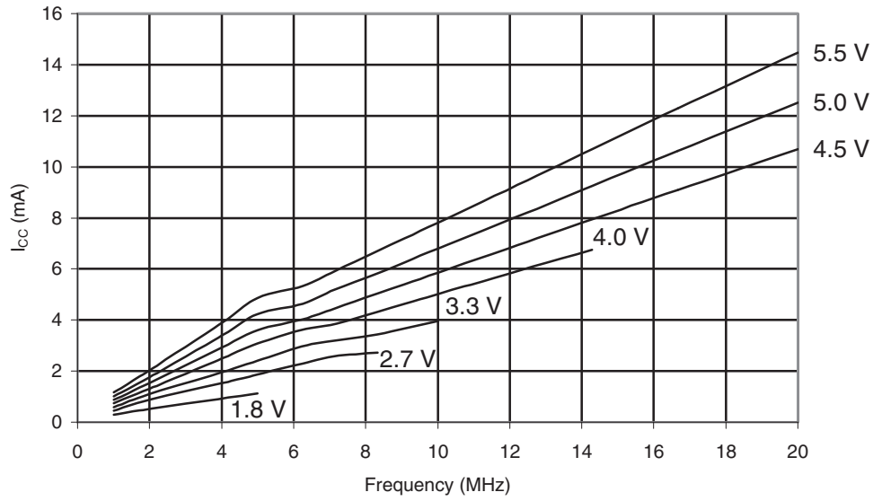
Figure 29-432. ATmega649P: Idle Supply Current vs. Frequency (1 - 16 MHz)
