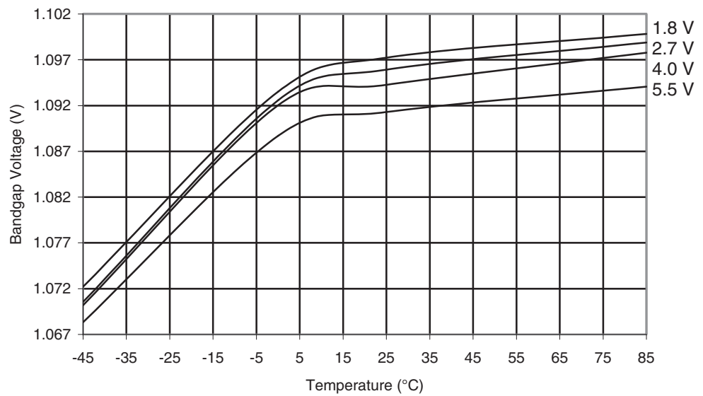
Figure 29-44. ATmega169A: Bandgap Voltage vs. Temperature
