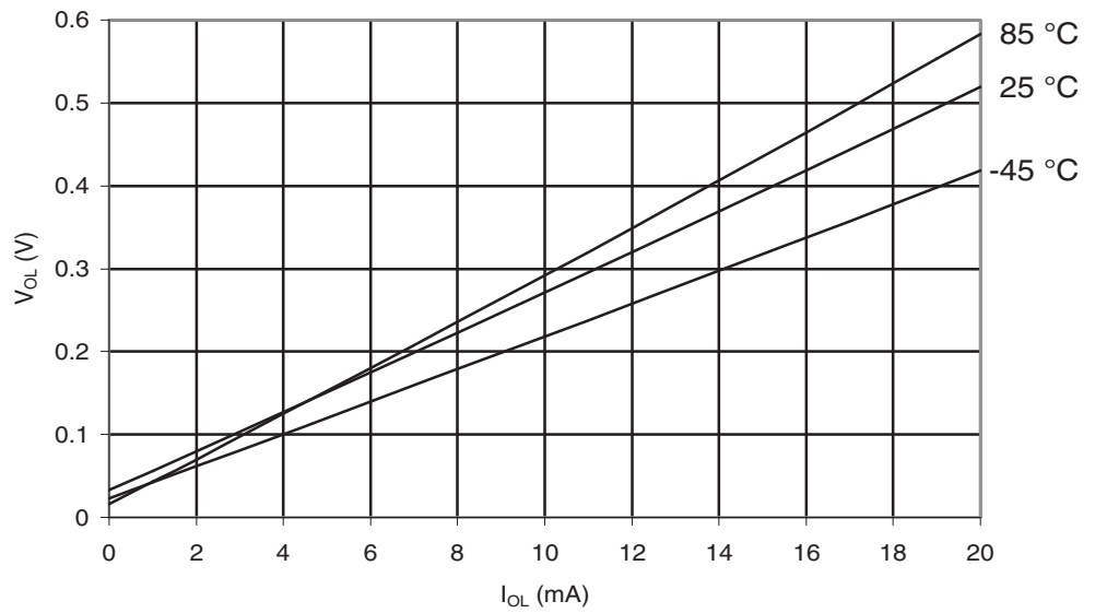
Figure 29-518. ATmega6490A: I/O Pin Output Voltage vs. Sink Current, Port B ( V_{CC} = 5V )
