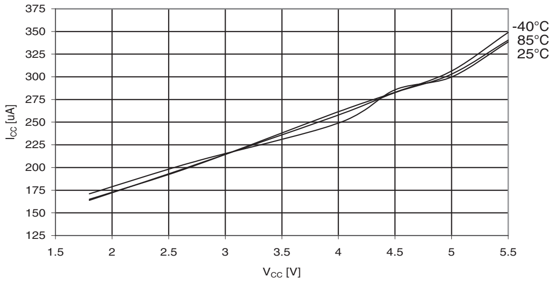
Figure 29-297. ATmega3290A: Active Supply Current with ADC at 1 MHz vs. V_{CC}
