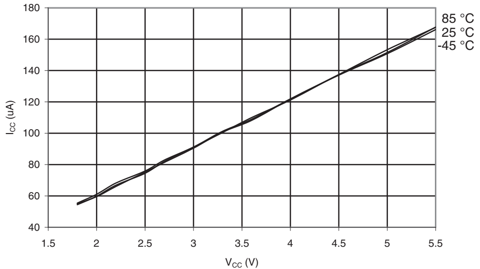
Figure 29-56. ATmega169A: AREF External Reference Current vs. V_{CC}
