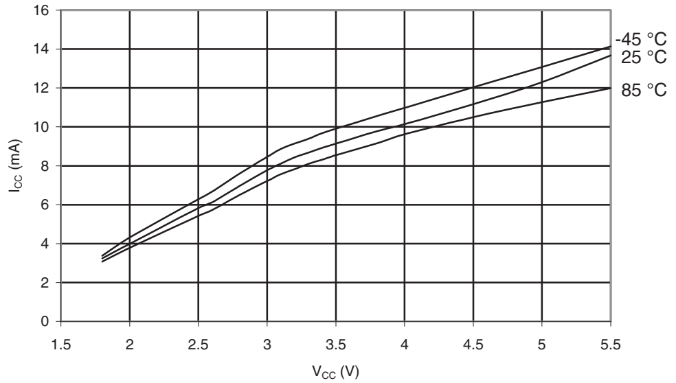
Figure 29-121. ATmega169PA: Programming Current vs. V_{CC}
