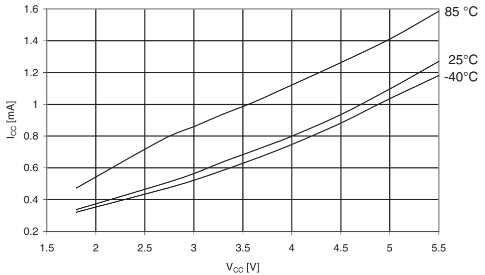
Figure 29-308. ATmega3290PA: Active Supply Current vs. V_{CC} (Internal RC Oscillator, 1 MHz)
