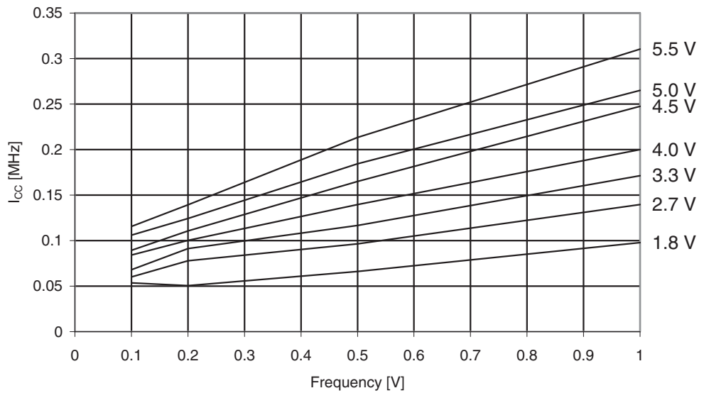
Figure 29-190. ATmega329PA: Idle Supply Current vs. Low Frequency (0.1 - 1.0 MHz)
