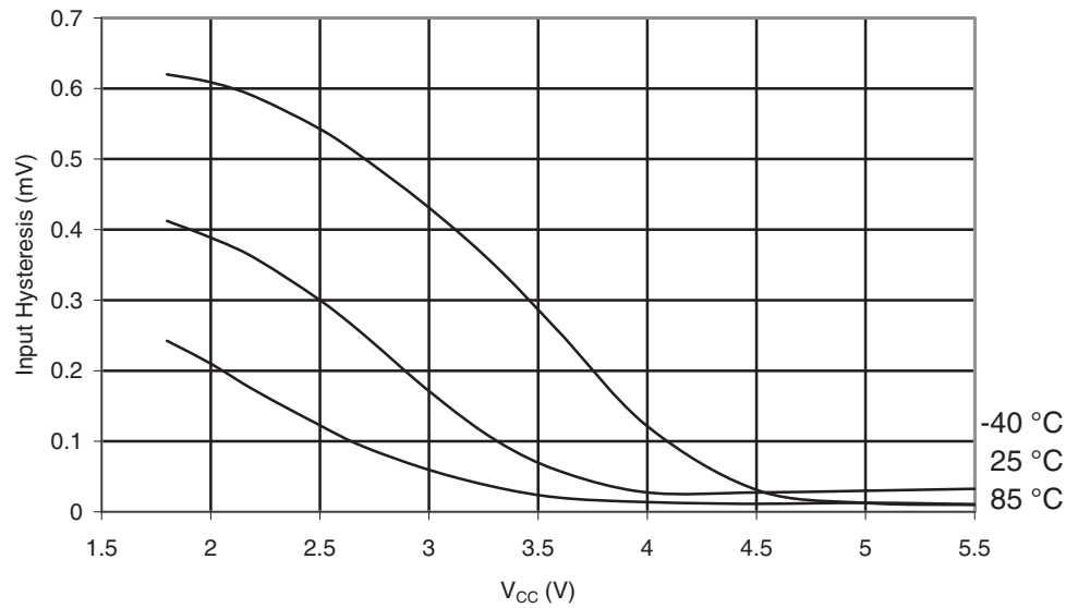
Figure 29-283. ATmega3290A: Reset Input Pin Hysteresis vs. V_{CC}
