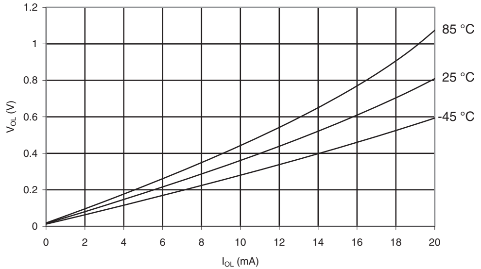
Figure 29-94. ATmega169PA: I/O Pin Output Voltage vs. Sink Current, Port B ( V_{CC} = 2.7V9 )
