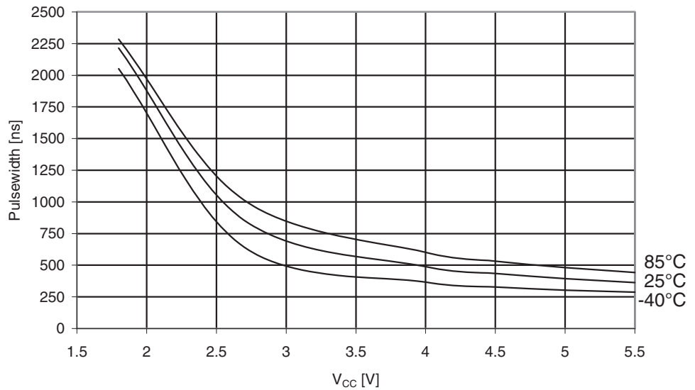
Figure 29-304. ATmega3290A: Minimum Reset Pulse Width vs. V_{CC}
