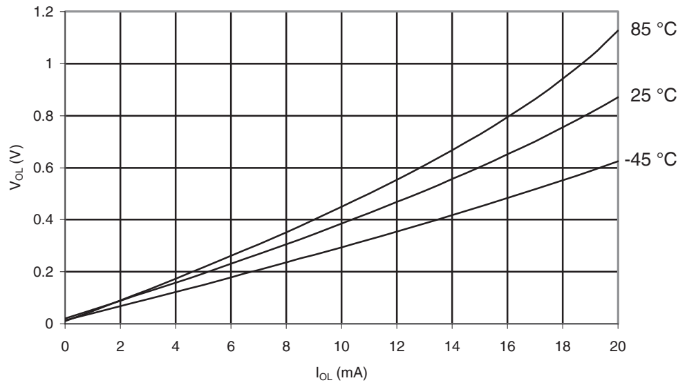
Figure 29-397. ATmega649A: I/O Pin Output Voltage vs. Sink Current, Port B ( V_{CC} = 2.7V_9 )
