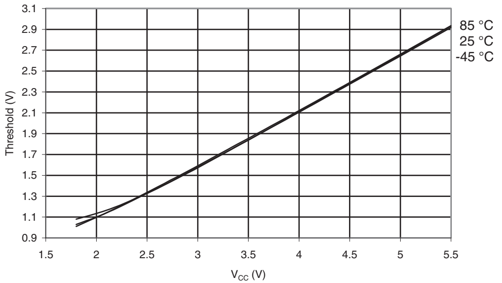
Figure 29-34. ATmega169A: I/O Pin Input Threshold Voltage vs. V_{CC} ( V_{IH} , I/O Pin Read as “1”)
