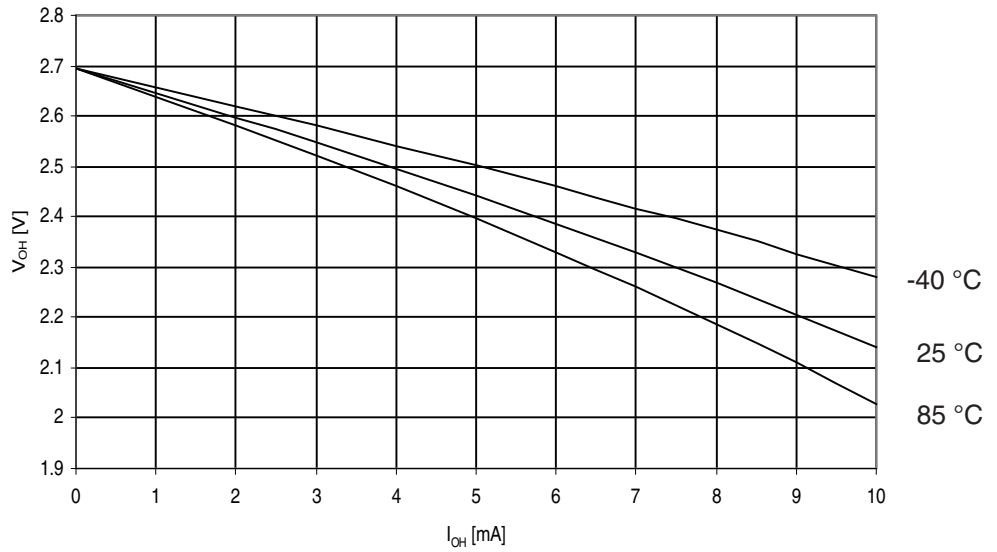
Figure 29-207. ATmega329PA: I/O Pin Output Voltage vs. Source Current, Ports A, C, D, E, F, G ( V_{CC} = 2.7V )
