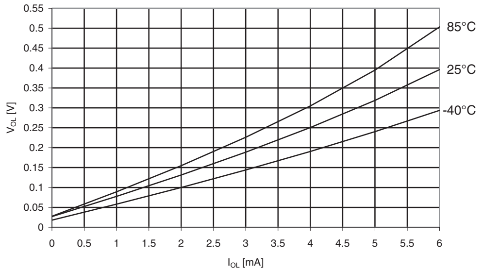
Figure 29-157. ATmega329A: I/O Pin Output Voltage vs. Sink Current, Port B ( V_{CC} = 1.8V )
