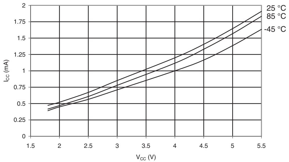
Figure 29-70. ATmega169PA: Idle Supply Current vs. V_{CC} (Internal RC Oscillator, 8 MHz)
