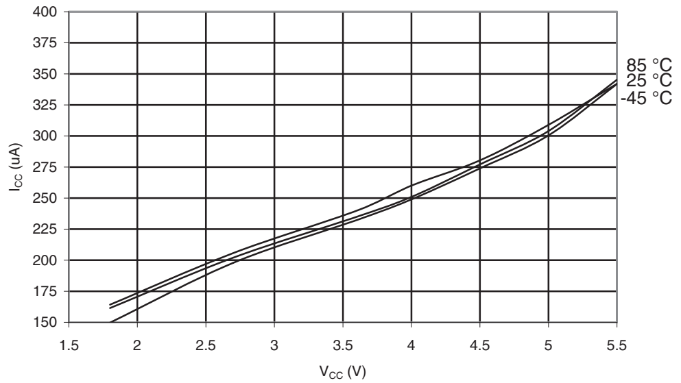
Figure 29-115. ATmega169PA: Active Supply Current with ADC at 50 kHz vs. V_{CC}
