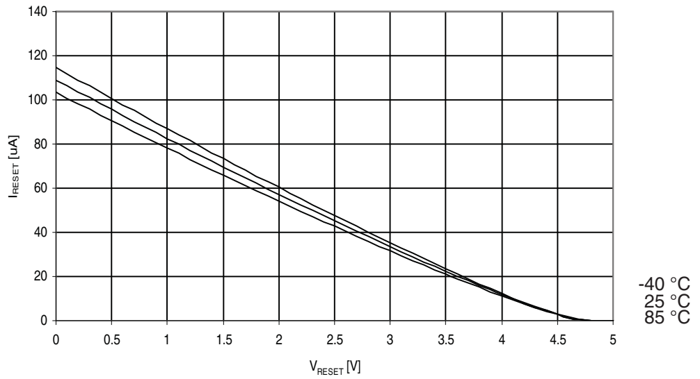
Figure 29-323. ATmega3290PA: Reset Pull-up Resistor Current vs. Reset Pin Voltage ( V_{CC} = 5V )
