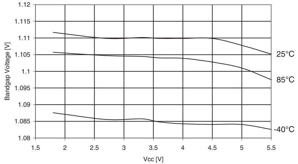
Figure 29-287. ATmega3290A: Bandgap Voltage vs. V_{CC}
