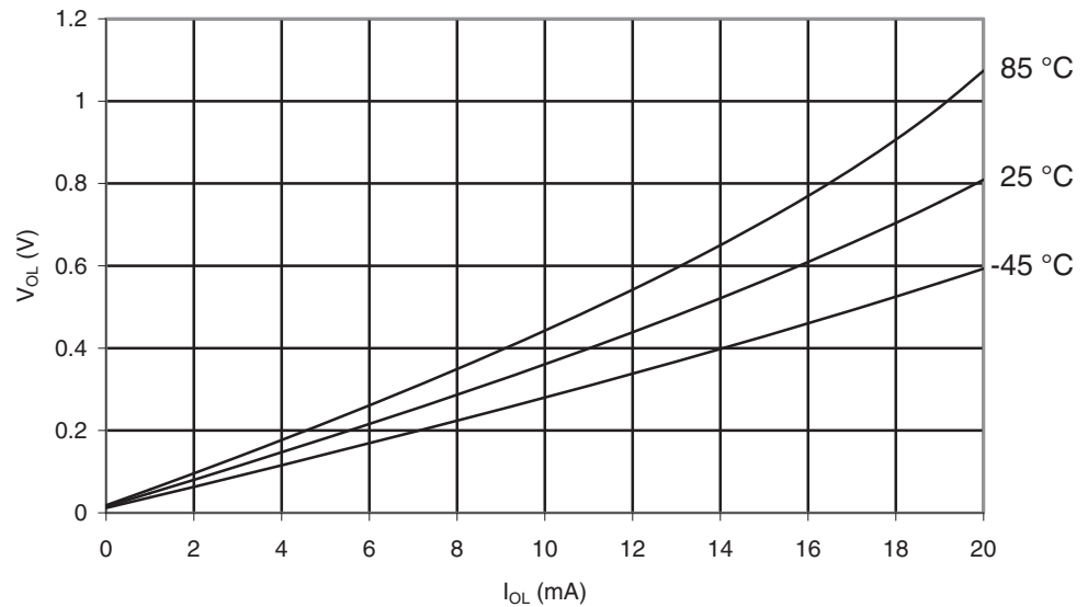
Figure 29-32. ATmega169A: I/O Pin Output Voltage vs. Sink Current, Port B ( V_{CC} = 2.7V9 )
