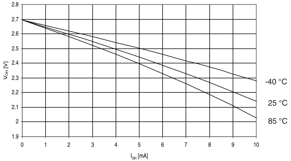
Figure 29-327. ATmega3290PA: I/O Pin Output Voltage vs. Source Current, Ports A, C, D, E, F, G ( V_{CC} = 2.7V )
