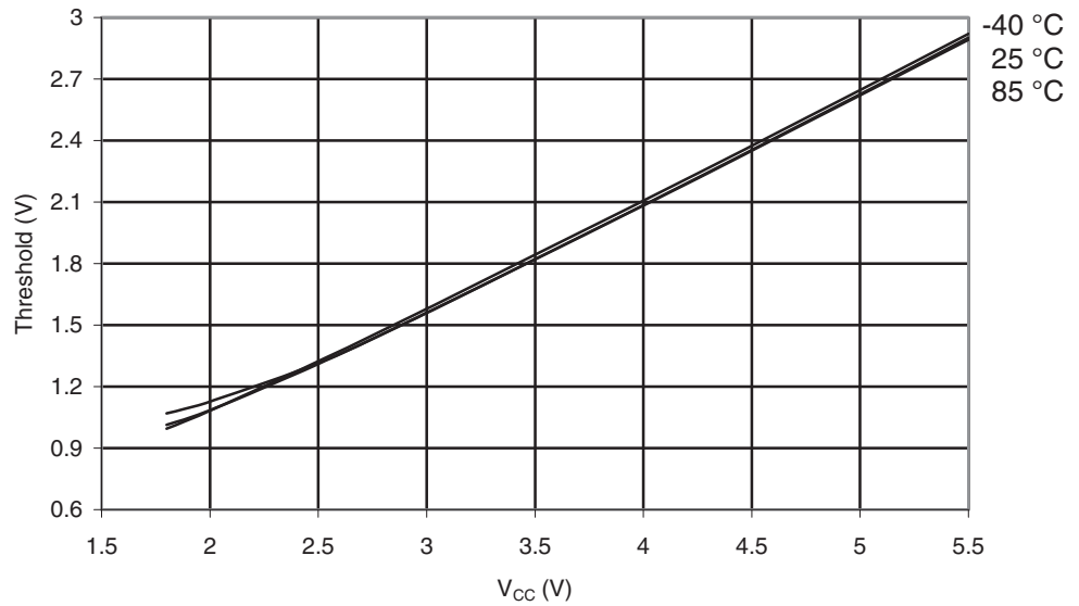
Figure 29-338. ATmega3290PA: I/O Pin Input Threshold Voltage vs. V_{CC} ( V_{IH} , I/O Pin Read as "1")
