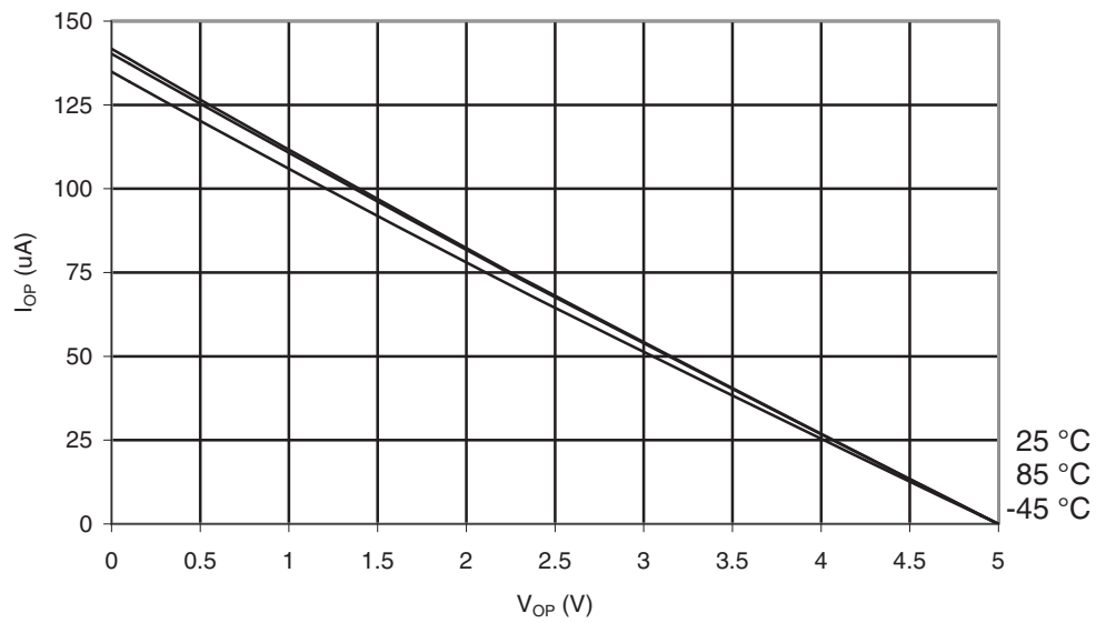
Figure 29-16. ATmega169A: I/O Pin Pull-up Resistor Current vs. Input Voltage ( V_{CC} = 5V )
