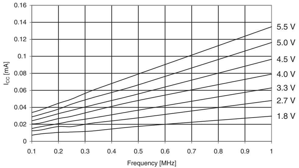
Figure 29-362. ATmega3290PA: Reset Supply Current vs. V_{CC} (0.1 - 1.0 MHz, Excluding Current Through The Reset Pull-up)
