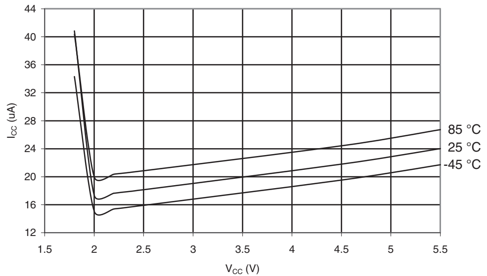
Figure 29-52. ATmega169A: Brownout Detector Current vs. V_{CC}
