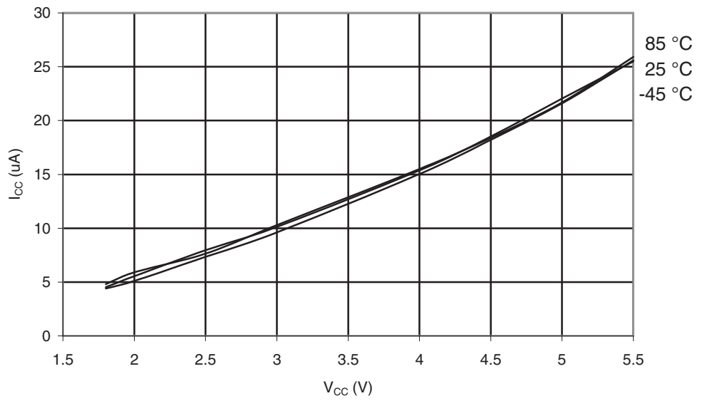
Figure 29-57. ATmega169A: Watchdog Timer Current vs. V_{CC}
