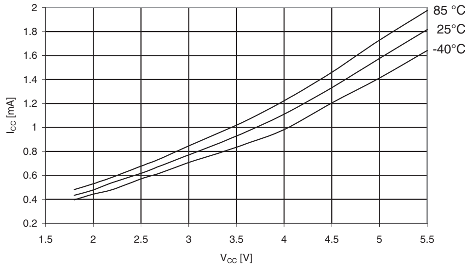
Figure 29-252. ATmega3290A: Idle Supply Current vs. V_{CC} (Internal RC Oscillator, 8 MHz)
