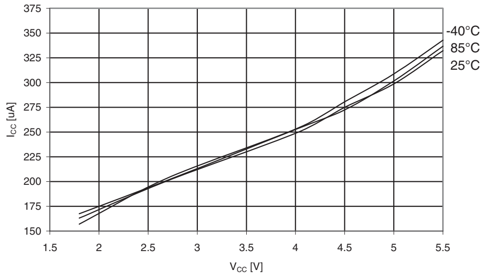
Figure 29-295. ATmega3290A: Active Supply Current with ADC at 50 kHz vs. V_{CC}
