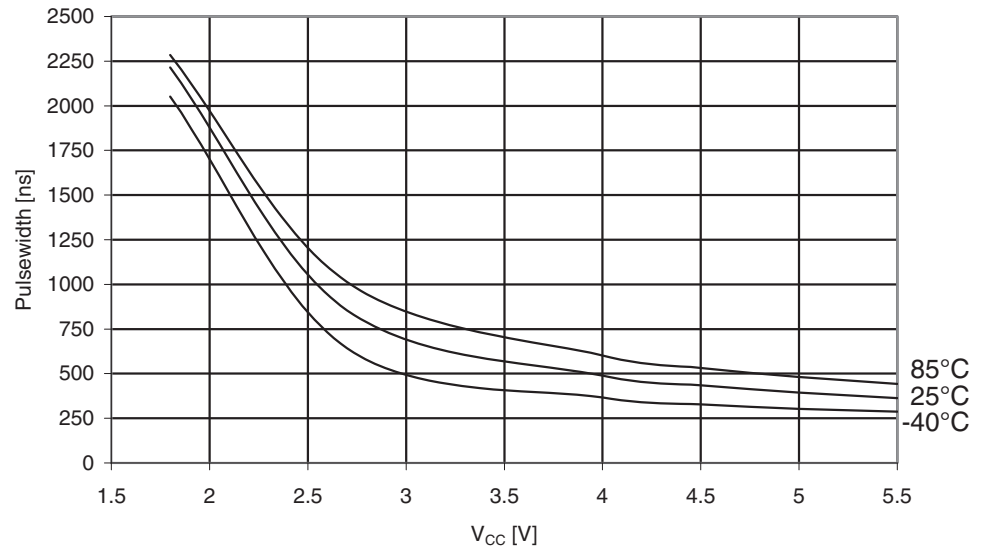
Figure 29-244. ATmega329PA: Minimum Reset Pulse Width vs. V_{CC}
