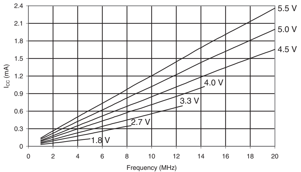
Figure 29-424. ATmega649A: Reset Supply Current vs. V_{CC} (1 - 16 MHz, Excluding Current Through The Reset Pull-up)
