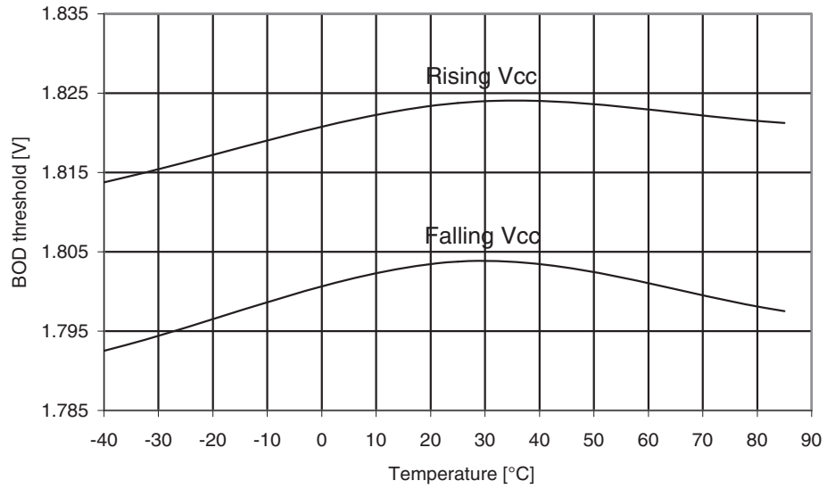
Figure 29-346. ATmega3290PA: BOD Thresholds vs. Temperature (BOD Level is 1.8V)
