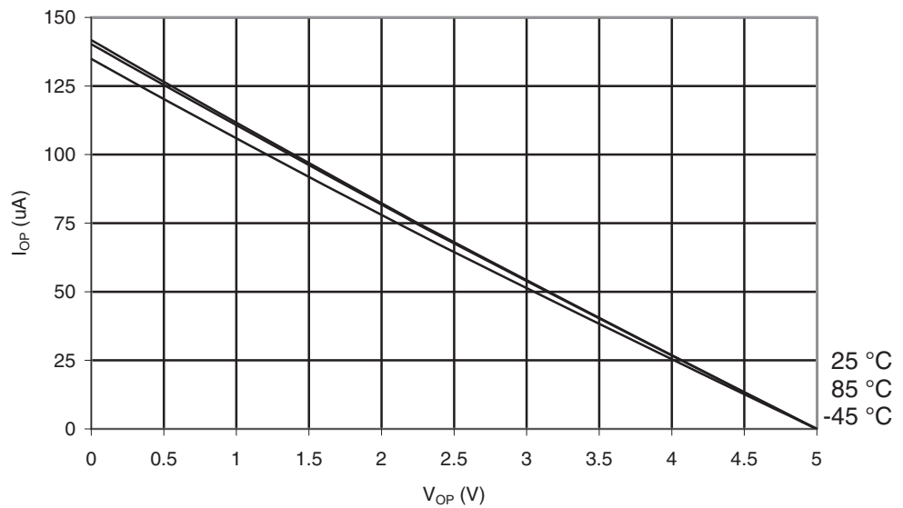
Figure 29-78. ATmega169PA: I/O Pin Pull-up Resistor Current vs. Input Voltage ( V_{CC} = 5V )
