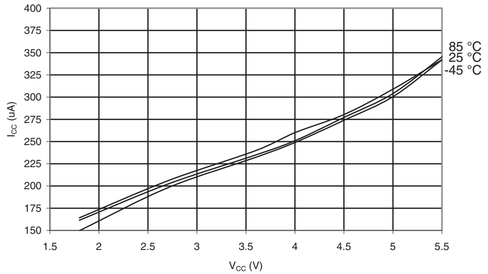
Figure 29-53. ATmega165A: Active Supply Current with ADC at 50kHz vs. V_{CC}
