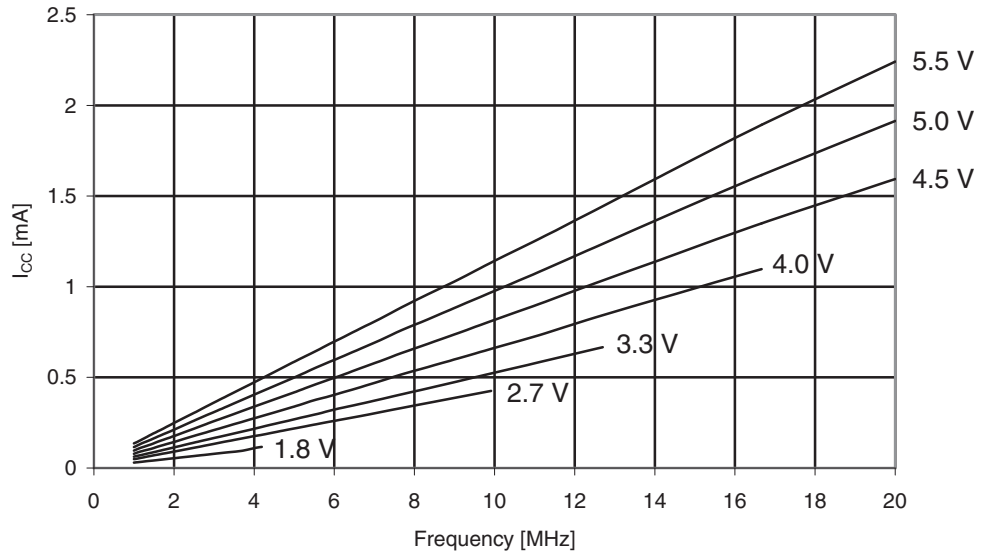
Figure 29-183. ATmega325A: Reset Supply Current vs. V_{CC} (1 - 20MHz, Excluding Current Through The Reset Pull-up)
