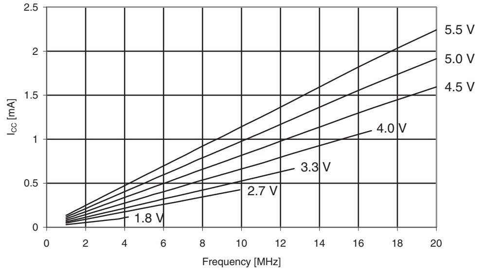
Figure 29-363. ATmega3250PA: Reset Supply Current vs. V_{CC} (1 - 20MHz, Excluding Current Through The Reset Pull-up)
