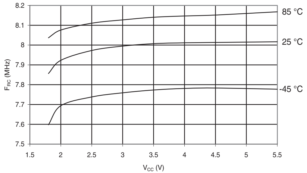
Figure 29-112. ATmega165PA: Calibrated 8MHz RC Oscillator Frequency vs. V_{CC}
