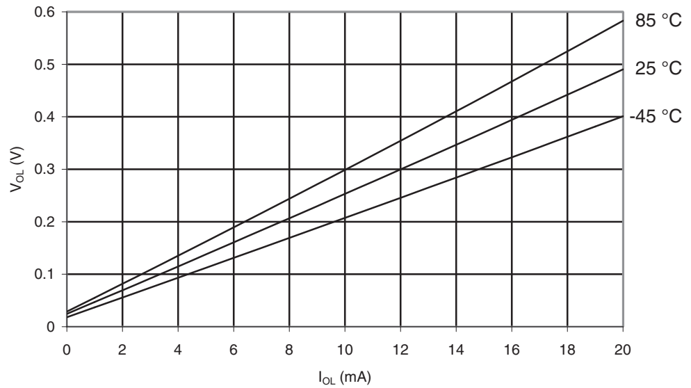
Figure 29-93. ATmega165PA: I/O Pin Output Voltage vs. Sink Current, Port B ( V_{CC} = 5V )
