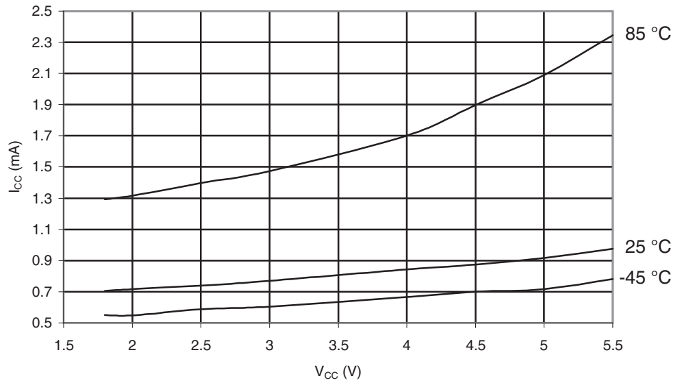
Figure 29-501. ATmega6450A: Standby Supply Current vs. V_{CC} (32kHz Watch Crystal, Watchdog Timer Disabled)
