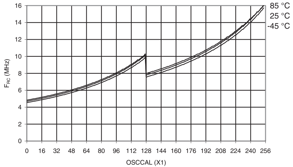
Figure 29-51. ATmega165A: Calibrated 8MHz RC Oscillator Frequency vs. Oscal Value
