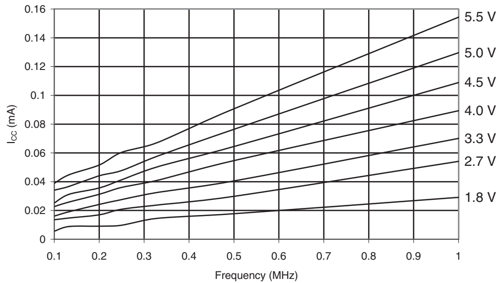
Figure 29-122. ATmega165PA: Reset Supply Current vs. V_{CC} (0.1 - 1.0MHz, Excluding Current Through The Reset Pull-up)
