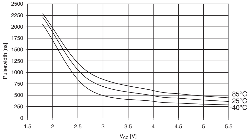
Figure 29-184. ATmega325A: Minimum Reset Pulse Width vs. V_{CC}
