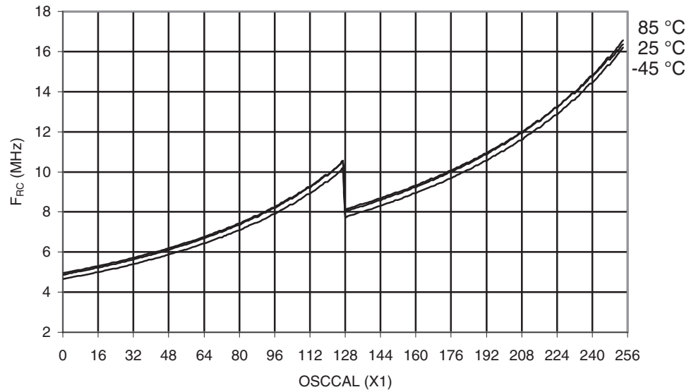
Figure 29-536. ATmega6450A: Calibrated 8MHz RC Oscillator Frequency vs. OSCCAL Value
