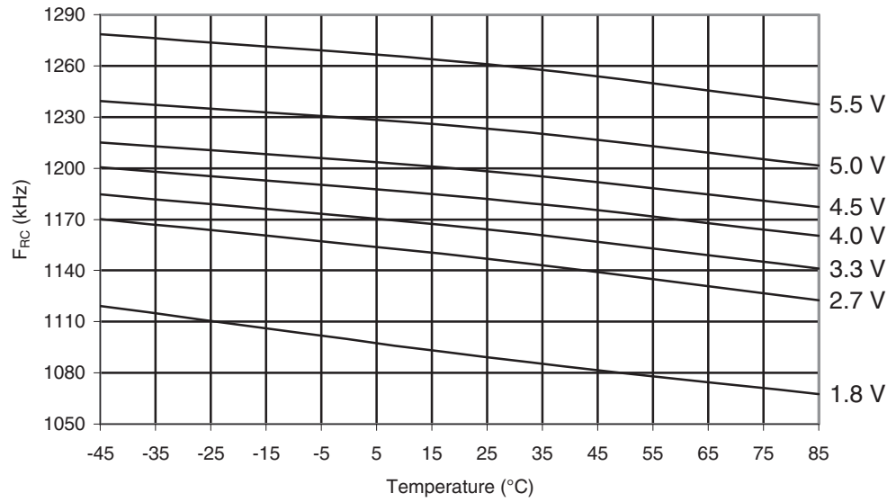
Figure 29-594. ATmega6450P: Watchdog Oscillator Frequency vs. Temperature
