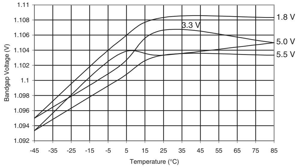
Figure 29-470. ATmega645P: Bandgap Voltage vs. Temperature
