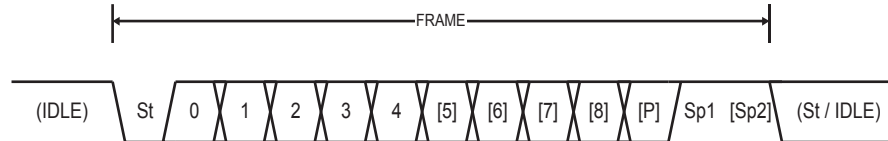
Figure 19-4. Frame Formats
