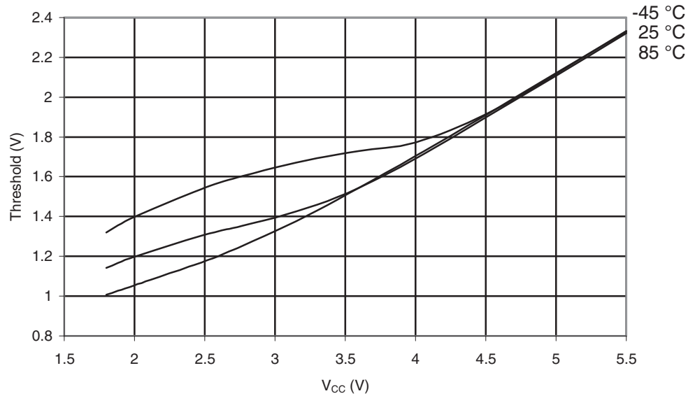
Figure 29-585. ATmega6450P: Reset Input Threshold Voltage vs. V_{CC} ( V_{IH,Reset} , Reset Pin Read as "1")
