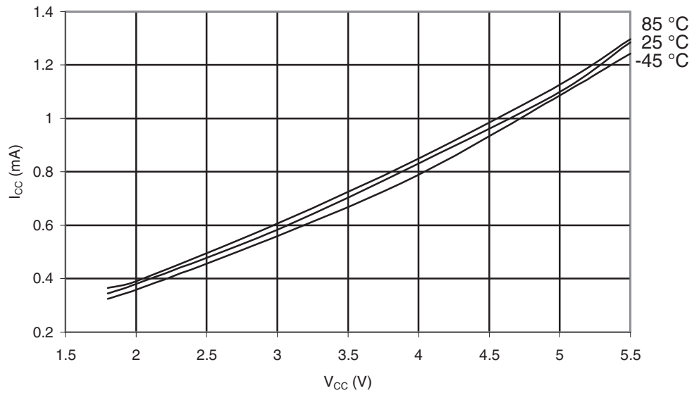
Figure 29-490. ATmega6450A: Active Supply Current vs. V_{CC} (Internal RC Oscillator, 1MHz)
