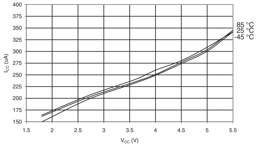
Figure 29-115. ATmega165PA: Active Supply Current with ADC at 50kHz vs. V_{CC}
