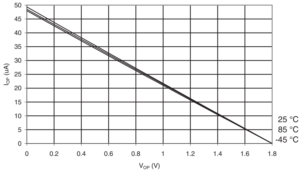
Figure 29-80. ATmega165PA: I/O Pin Pull-up Resistor Current vs. Input Voltage ( V_{CC} = 1.8V )
