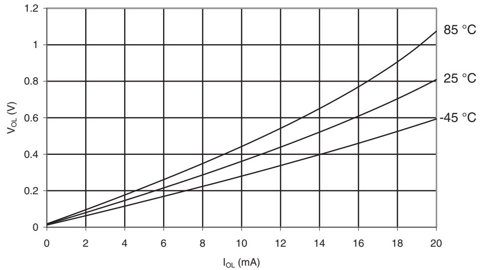
Figure 29-32. ATmega165A: I/O Pin Output Voltage vs. Sink Current, Port B ( V_{CC} = 2.7V )
