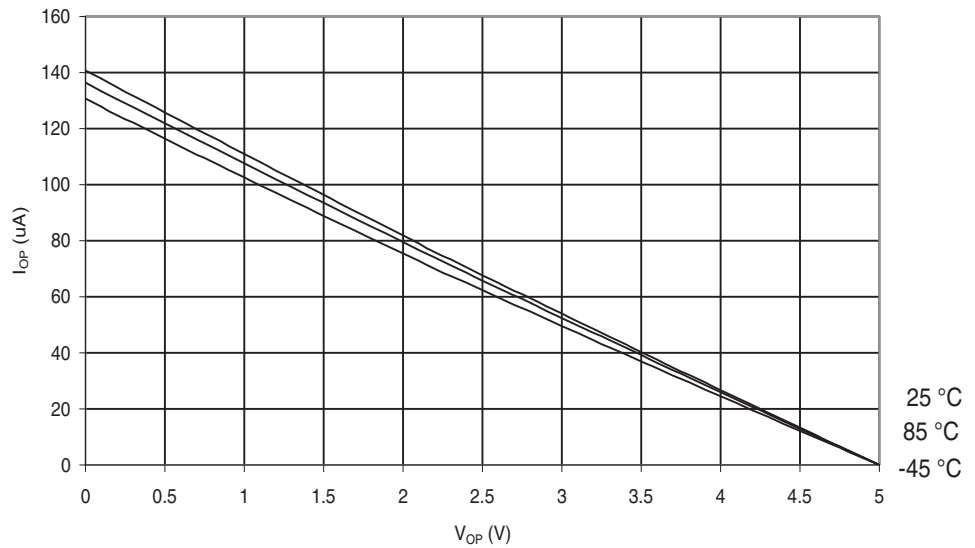
Figure 29-381. ATmega645A: I/O Pin Pull-up Resistor Current vs. Input Voltage ( V_{CC} = 5V )
