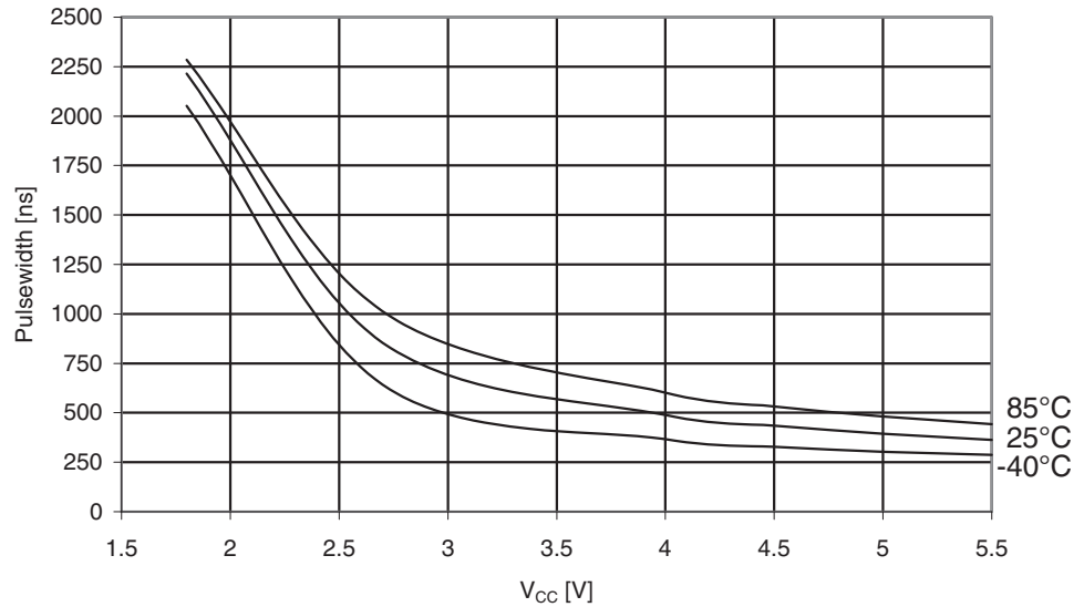
Figure 29-364. ATmega3250PA: Minimum Reset Pulse Width vs. V_{CC}
