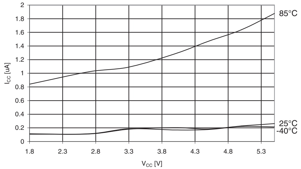
Figure 29-135. ATmega325A: Power-down Supply Current vs. V_{CC} (Watchdog Timer Disabled)
