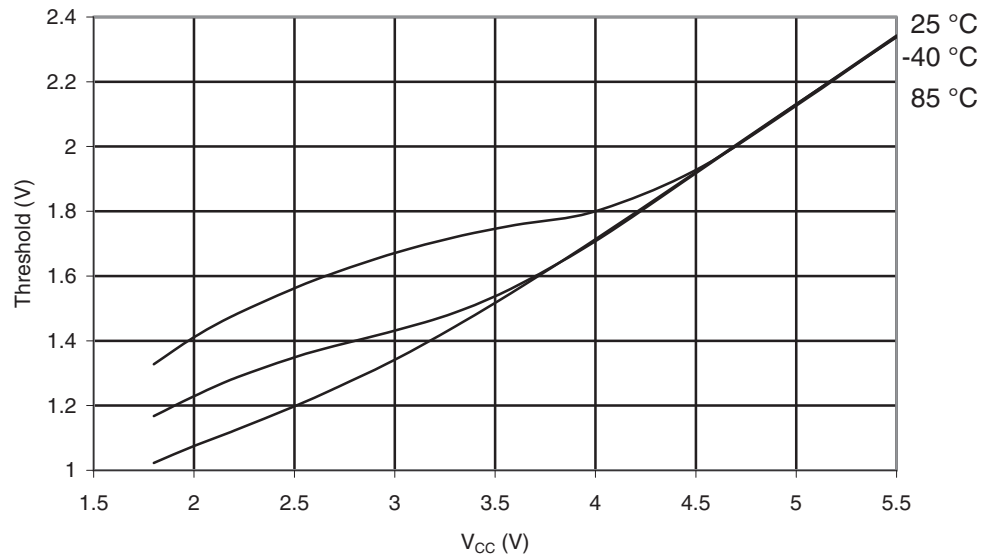
Figure 29-161. ATmega325A: Reset Input Threshold Voltage vs. V_{CC} ( V_{IH} , Reset Pin Read as "1")
