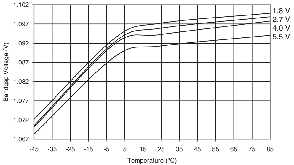
Figure 29-106. ATmega165PA: Bandgap Voltage vs. Temperature
