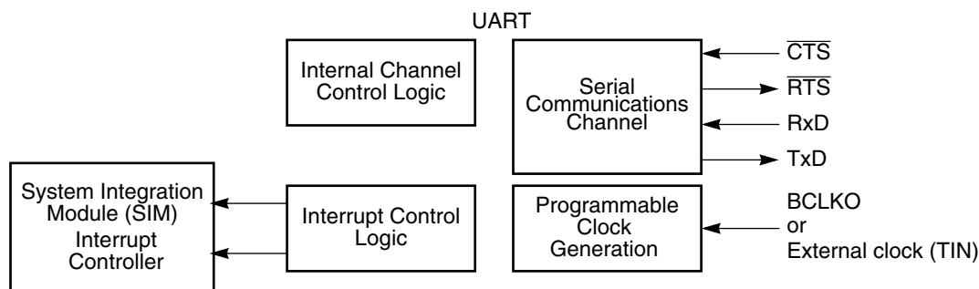
Figure 2. UART Module Block Diagram
