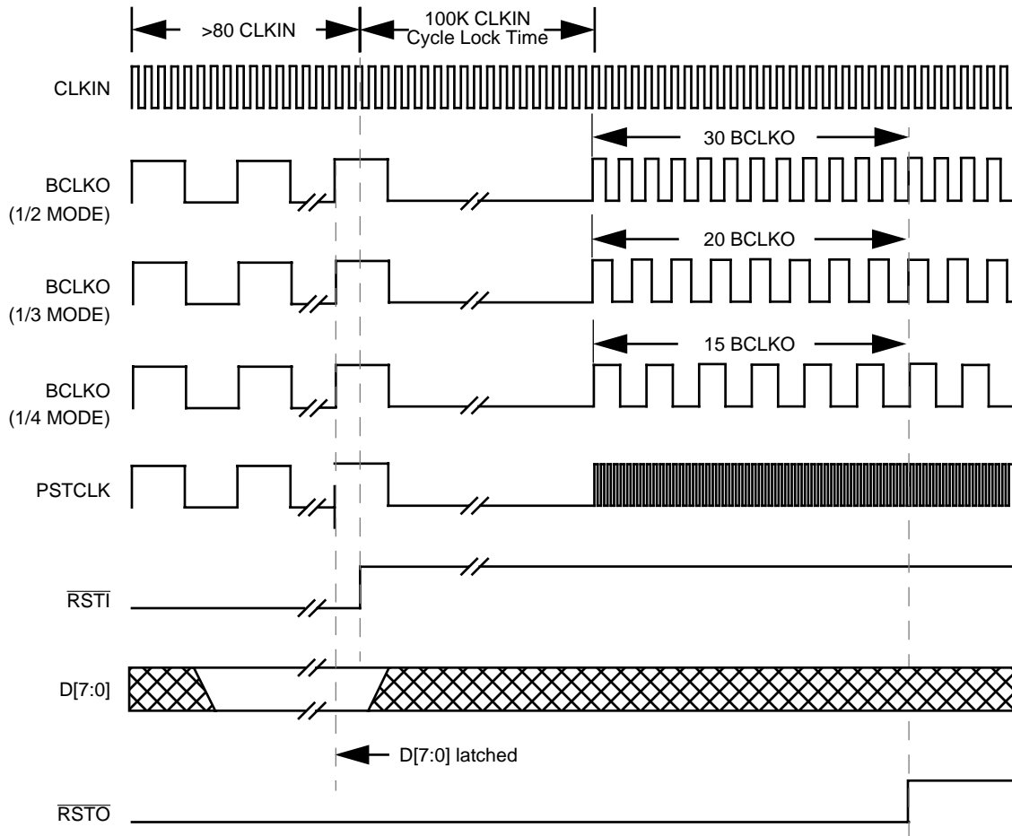
Figure 7-4. Reset and Initialization Timing
