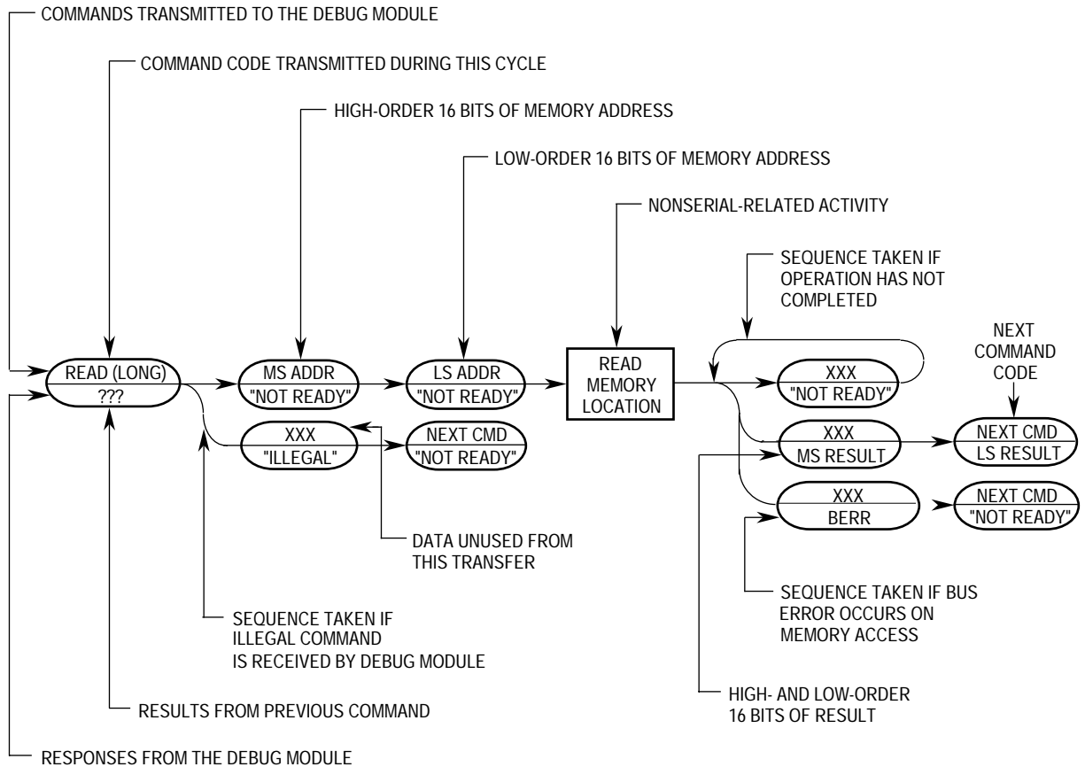
Figure 5-17. Command Sequence Diagram
