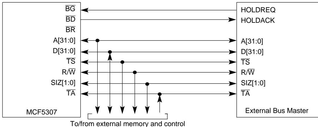
Figure 18-26. MCF5307 Two-Wire Mode Bus Arbitration Interface
