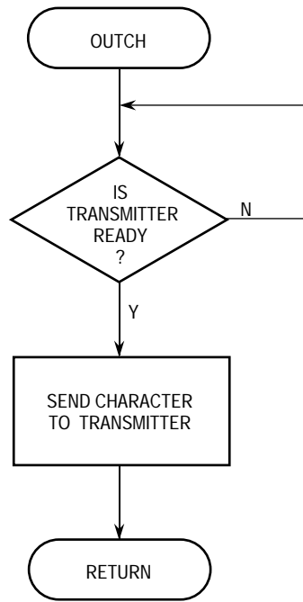
Figure 14-27. UART Mode Programming Flowchart (Sheet 5 of 5)
