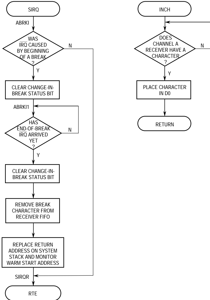
Figure 14-27. UART Mode Programming Flowchart (Sheet 4 of 5)
