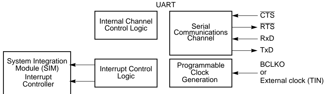
Figure 1-2. UART Module Block Diagram
