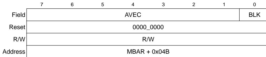
Figure 9-3. Autovector Register (AVR)
