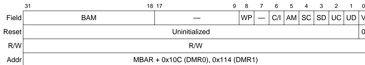
Figure 11-17. DRAM Controller Mask Registers (DMR0 and DMR1)
