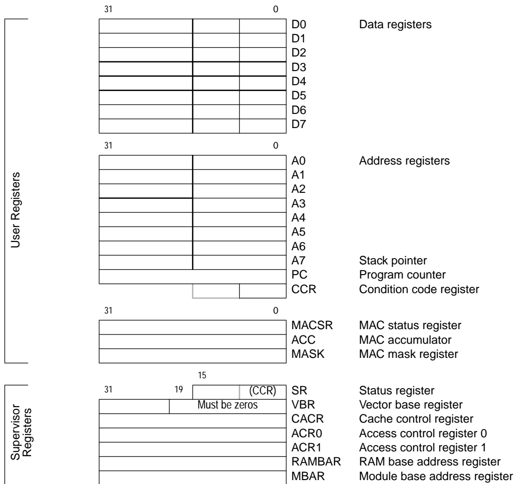
Figure 1-4. ColdFire MCF5307 Programming Model
