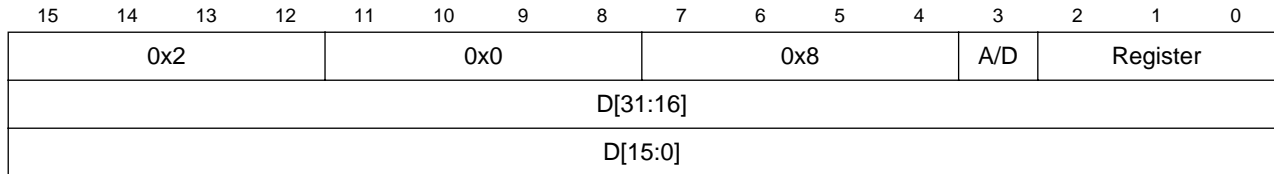
Figure 5-20. WAREG/WDREG Command Format
