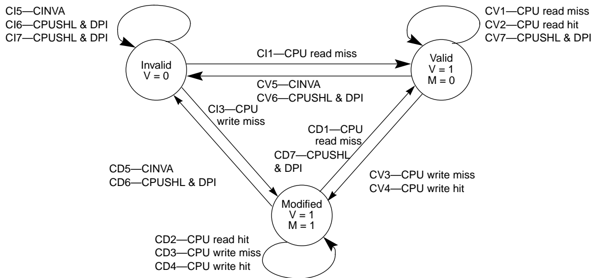
Figure 4-11. Cache Line State Diagram—Copyback Mode
