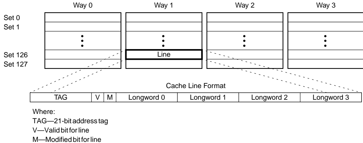
Figure 4-3. Cache Organization and Line Format
