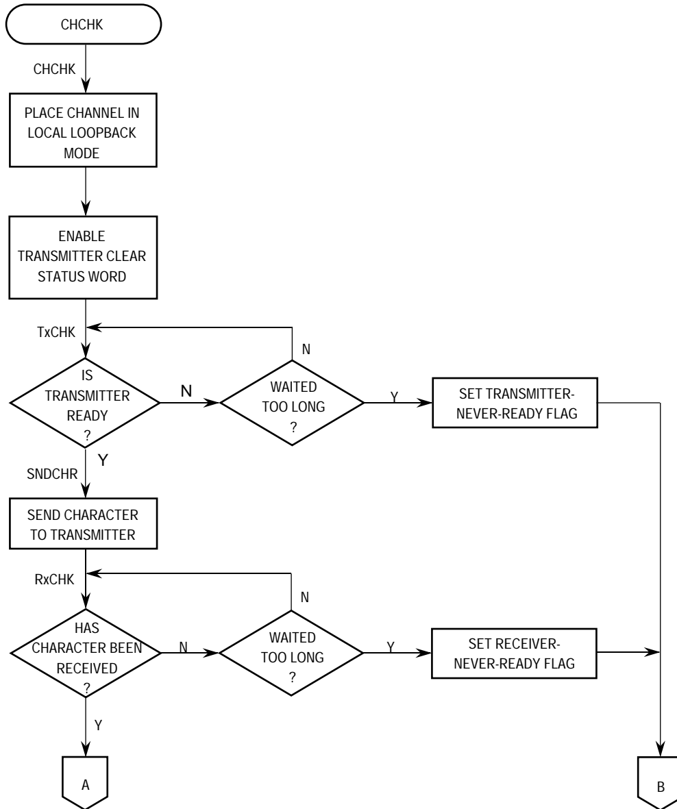
Figure 14-27. UART Mode Programming Flowchart (Sheet 2 of 5)
