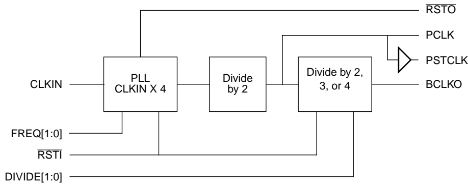
Figure 1-3. PLL Module
