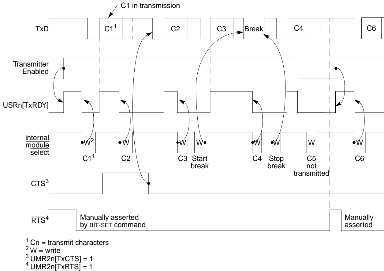
Figure 14-21. Transmitter Timing Diagram
