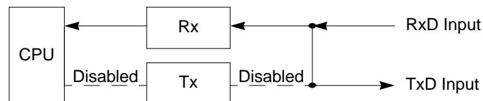
Figure 14-23. Automatic Echo
