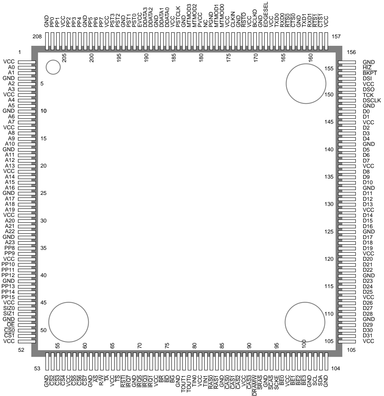
Figure 16-1. Mechanical Diagram
