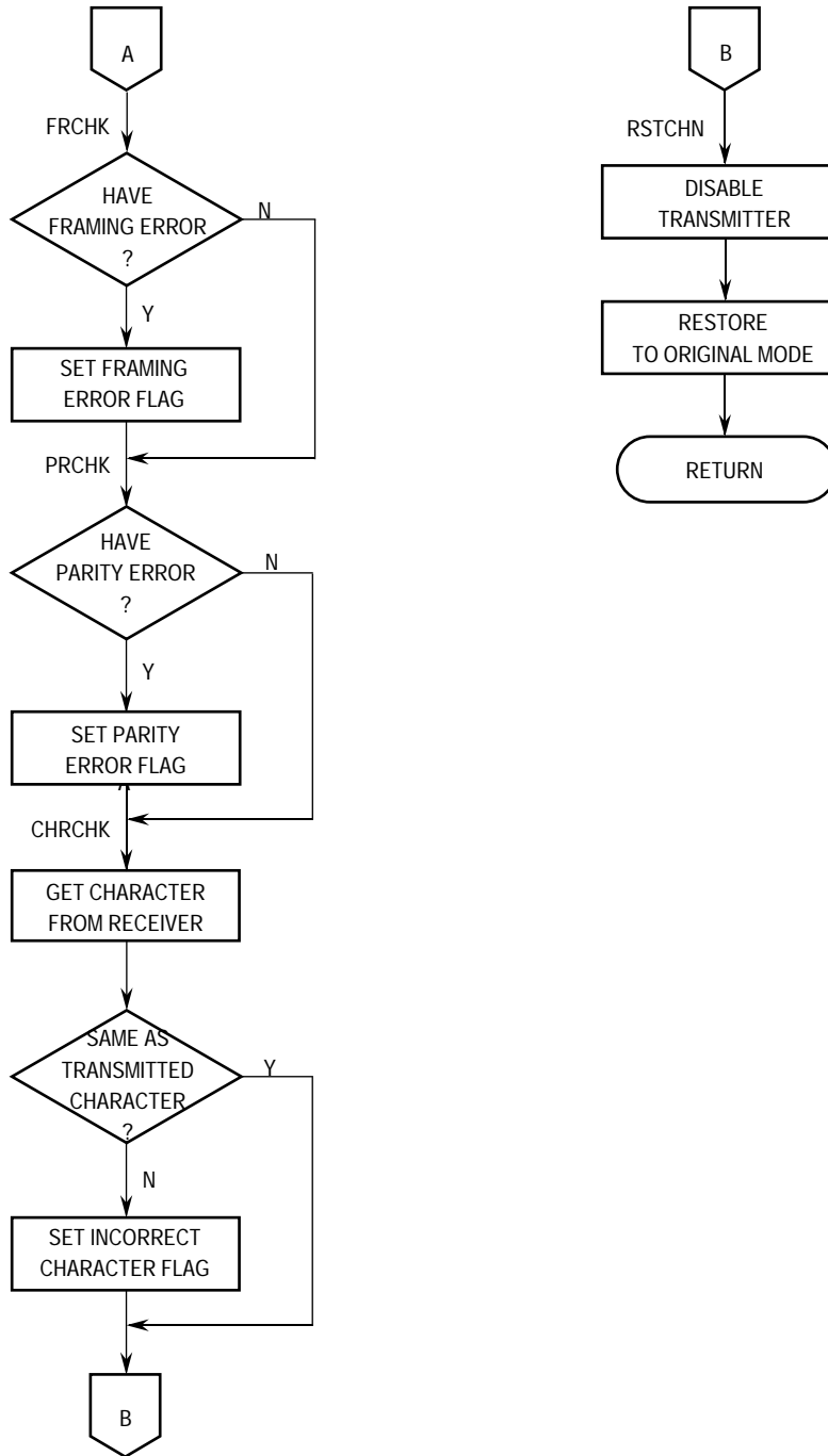
Figure 14-27. UART Mode Programming Flowchart (Sheet 3 of 5)
