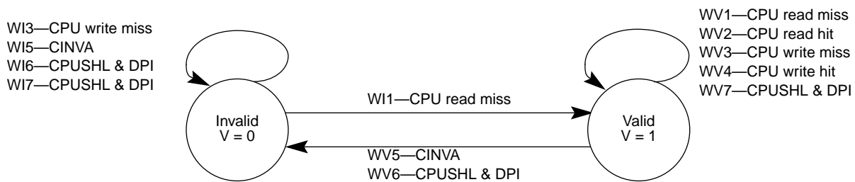
Figure 4-12. Cache Line State Diagram—Write-Through Mode
