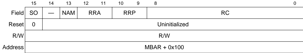
Figure 11-2. DRAM Control Register (DCR) (Asynchronous Mode)
