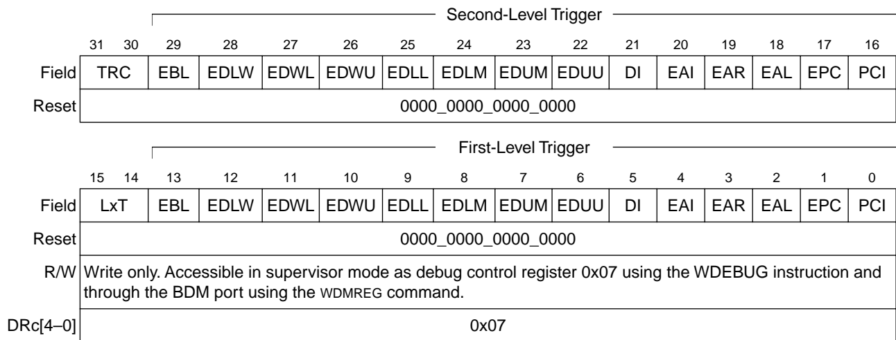
Figure 5-12. Trigger Definition Register (TDR)
