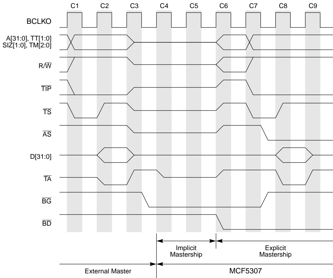
Figure 18-28. Two-Wire Implicit and Explicit Bus Mastership
