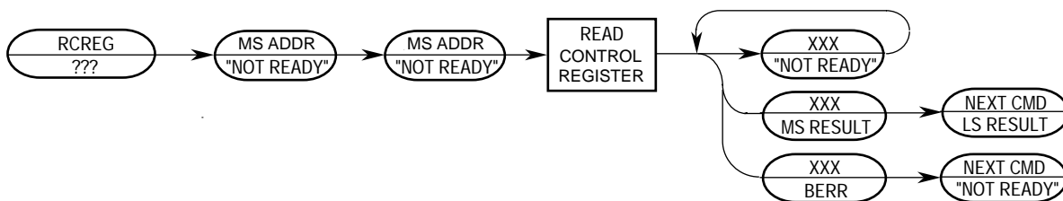
Figure 5-37. RCREG Command Sequence
