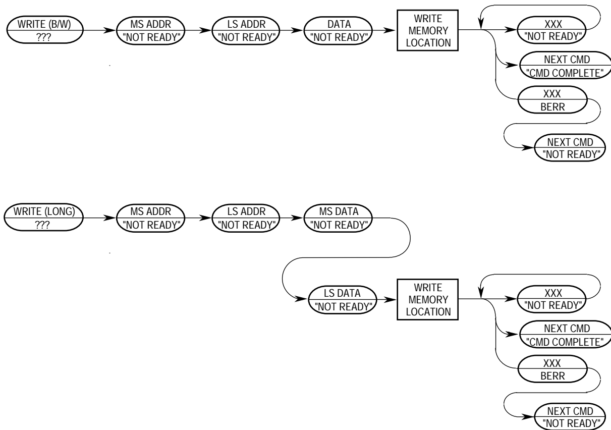
Figure 5-25. WRITE Command Sequence
