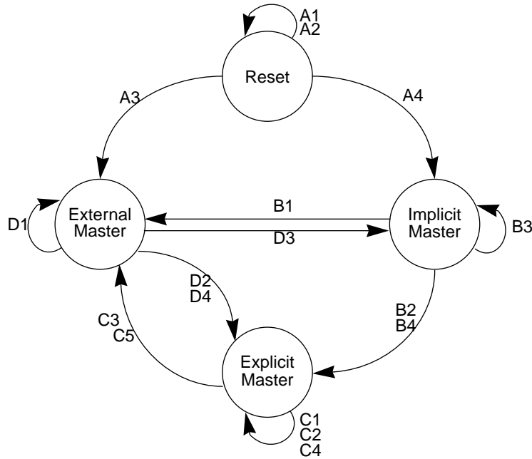
Figure 18-29. MCF5307 Two-Wire Bus Arbitration Protocol State Diagram
