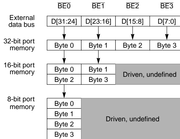
Figure 10-1. Connections for External Memory Port Sizes
