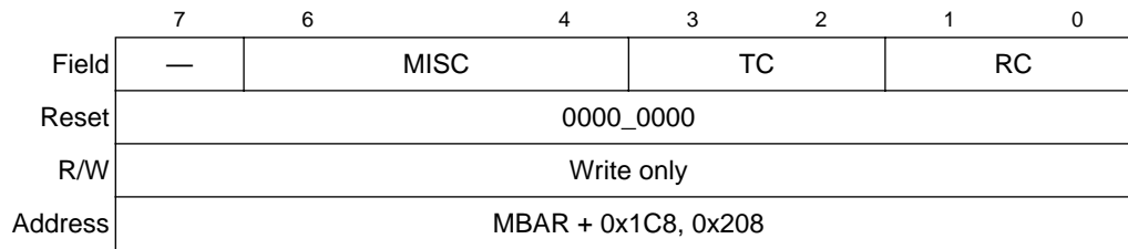
Figure 14-6. UART Command Register (UCR n )
