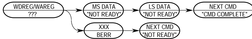
Figure 5-21. WAREG/WDREG Command Sequence
