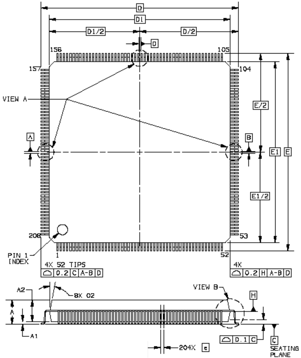
Figure 16-2. MCF5307 Case Drawing (General View)
