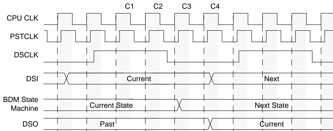
Figure 5-13. BDM Serial Interface Timing
