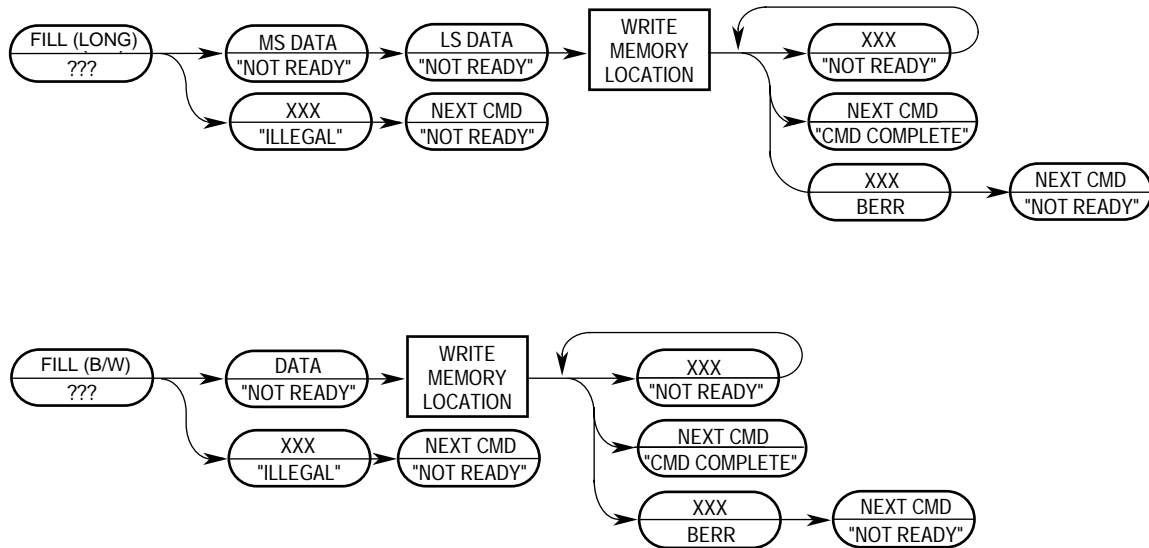
Figure 5-29. FILL Command Sequence
