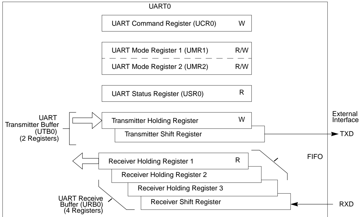
Figure 14-20. Transmitter and Receiver Functional Diagram
