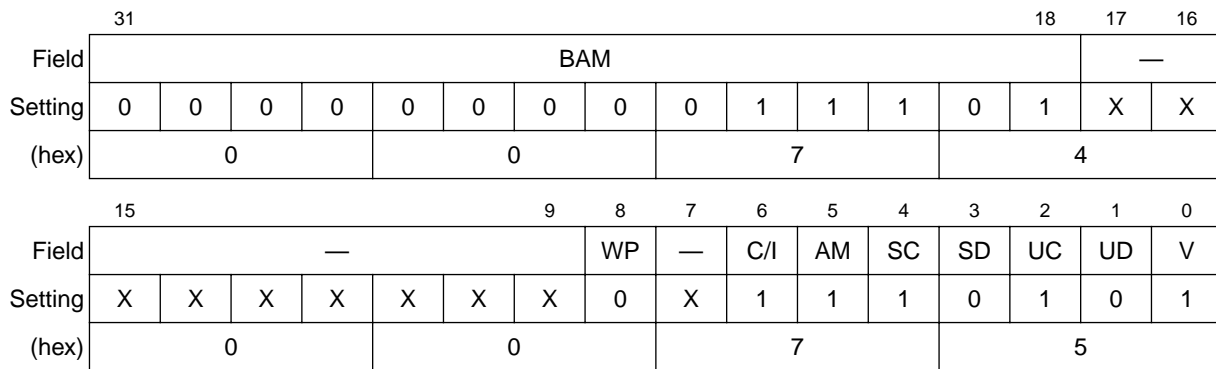
Figure 11-28. DMR0 Register
