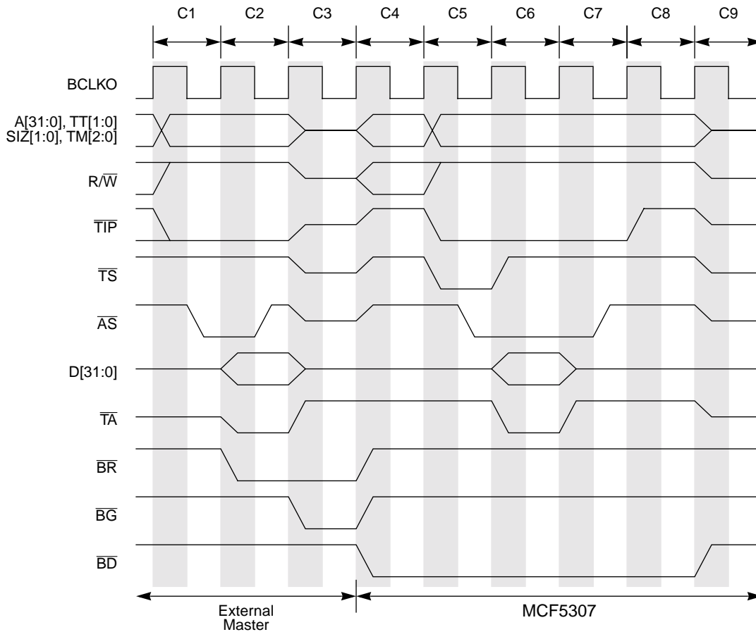
Figure 18-31. Three-Wire Bus Arbitration
