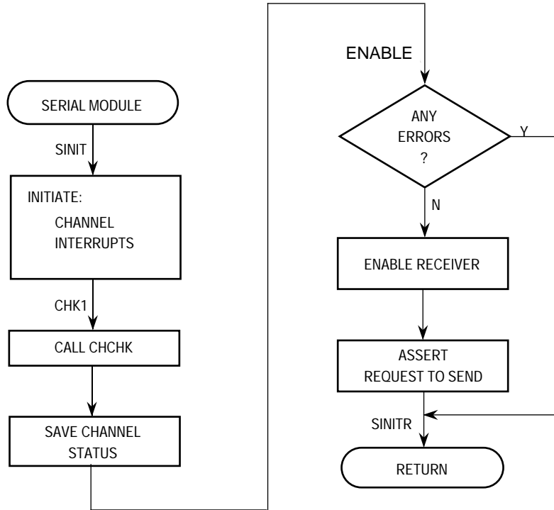
Figure 14-27. UART Mode Programming Flowchart (Sheet 1 of 5)
