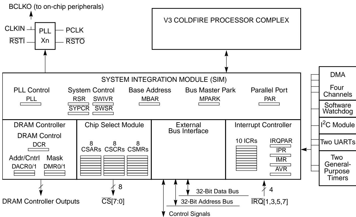
Figure 6-1. SIM Block Diagram
