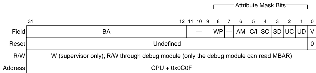
Figure 6-2. Module Base Address Register (MBAR)
