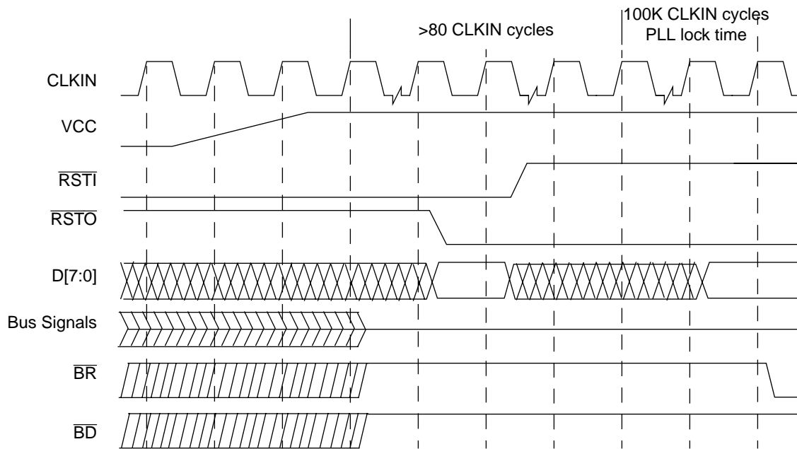
Figure 18-33. Master Reset Timing
