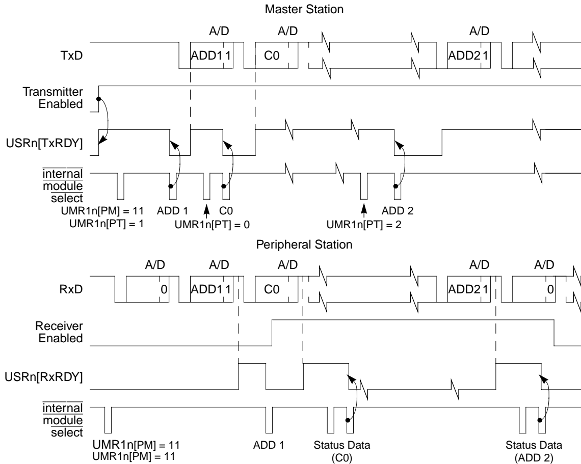
Figure 14-26. Multidrop Mode Timing Diagram
