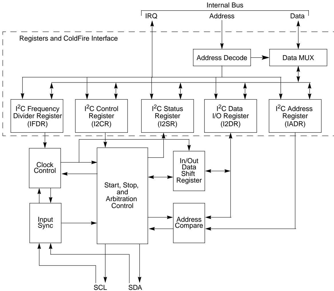
Figure 8-1. I 2 C Module Block Diagram
