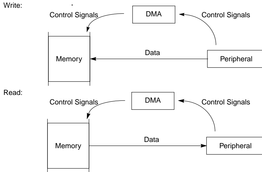
Figure 12-3. Single-Address Transfers
