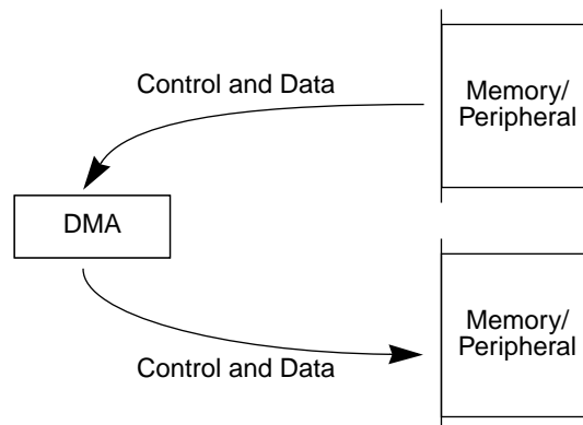
Figure 12-2. Dual-Address Transfer
