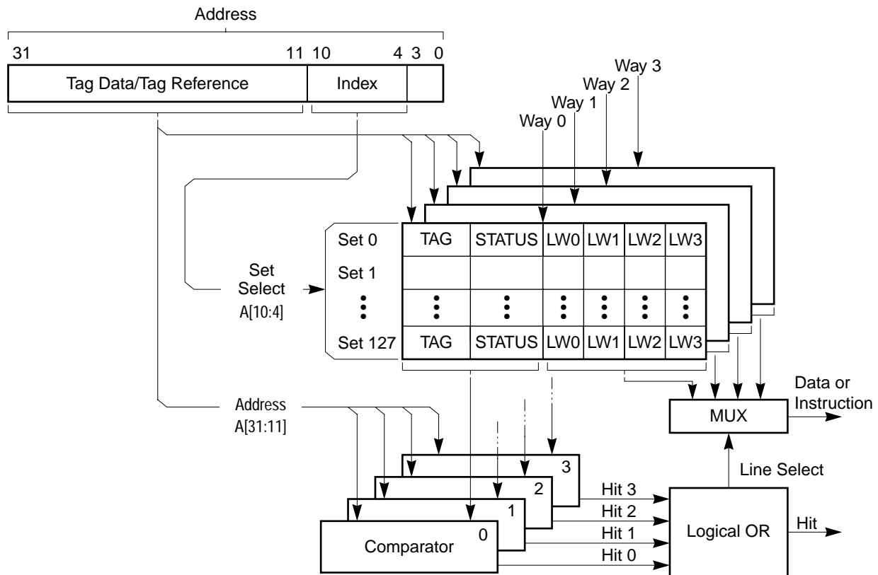
Figure 4-5. Caching Operation
