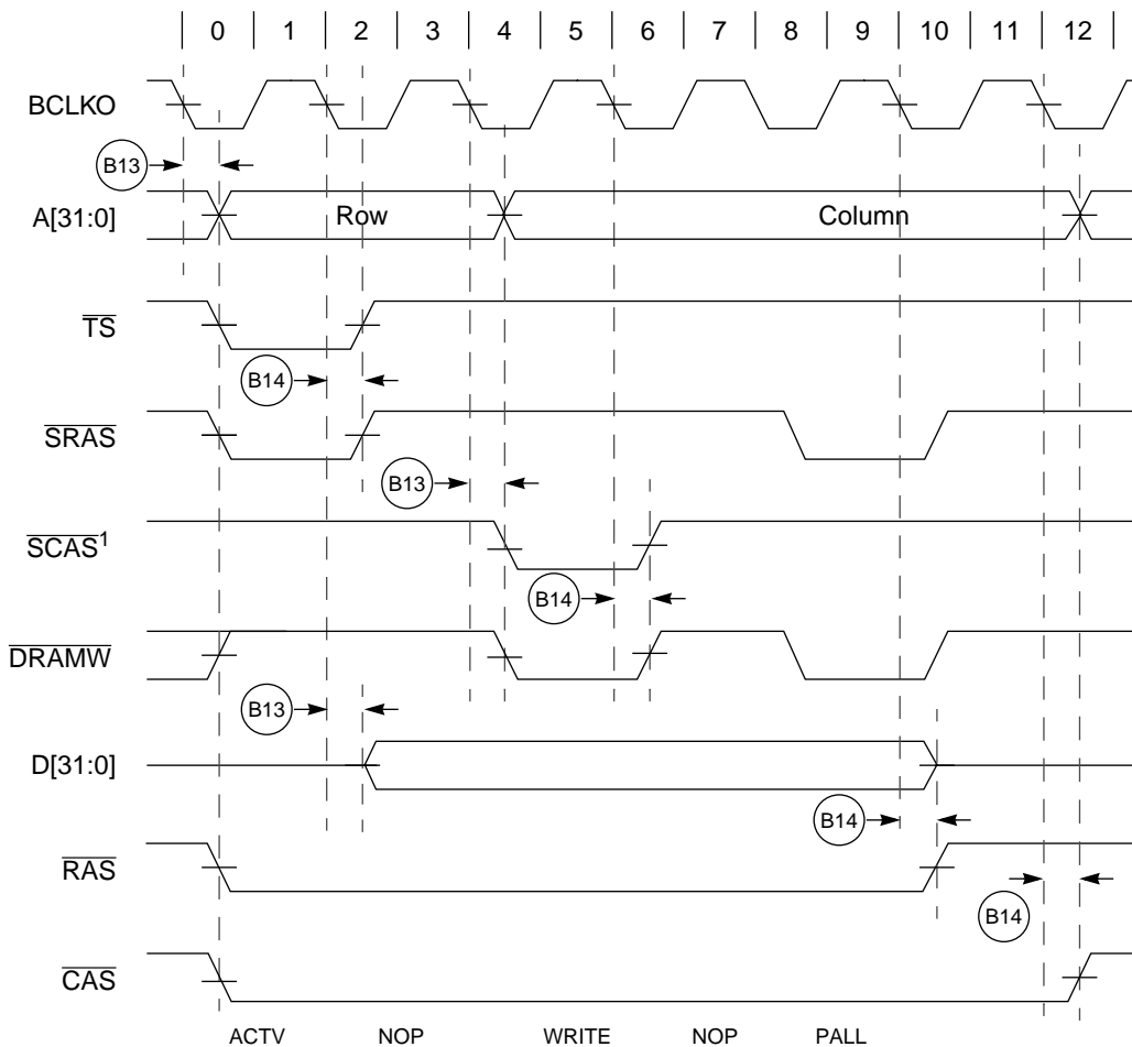
Figure 20-9. SDRAM Write Cycle with EDGESEL Tied Low
