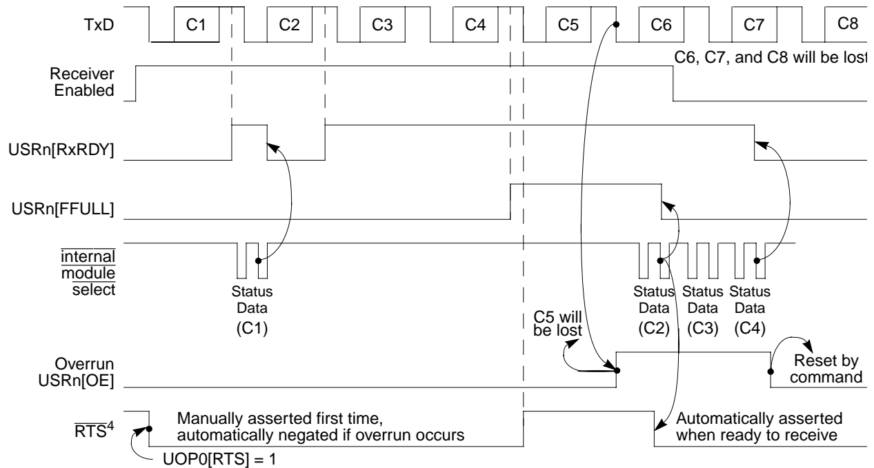
Figure 14-22. Receiver Timing
