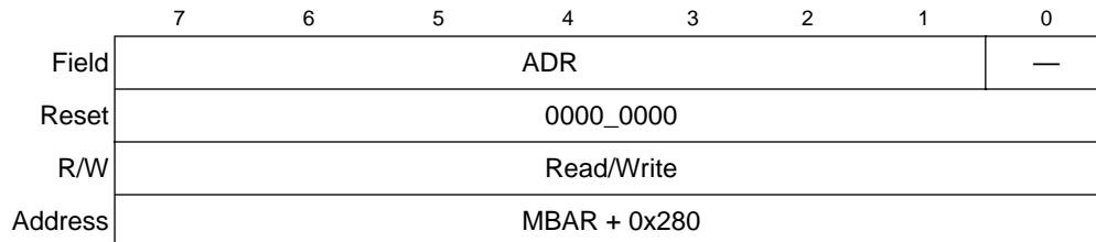
Figure 8-5. I 2 C Address Register (IADR)
