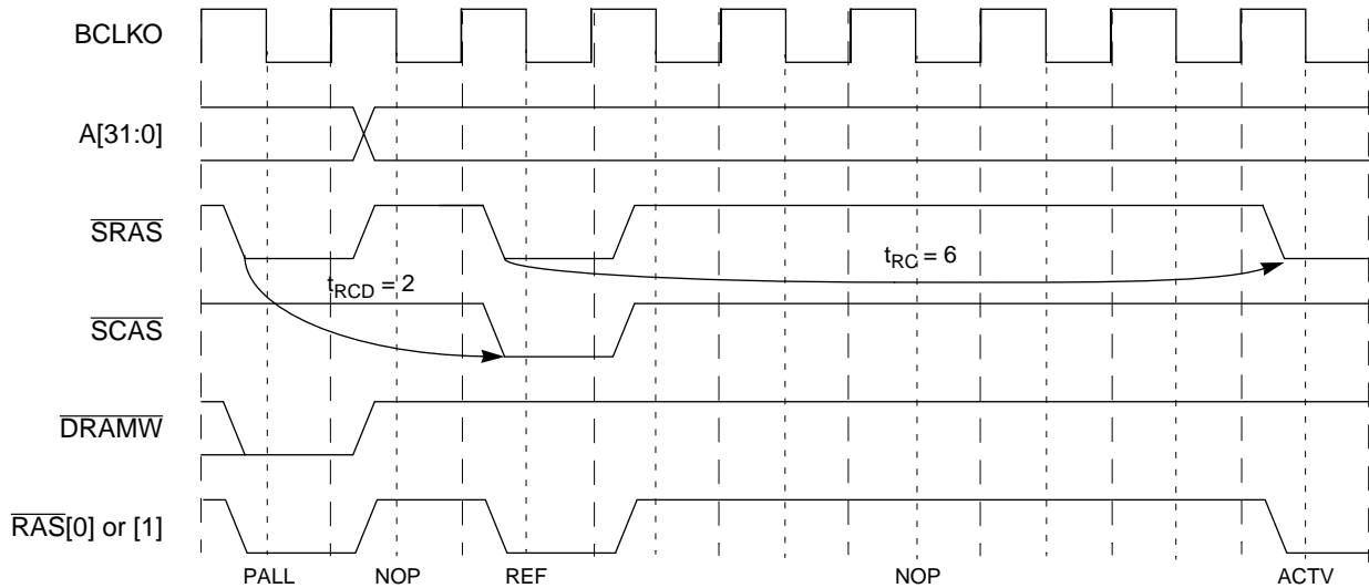
Figure 11-22. Auto-Refresh Operation
