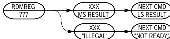
Figure 5-41. RDMREG Command Sequence
