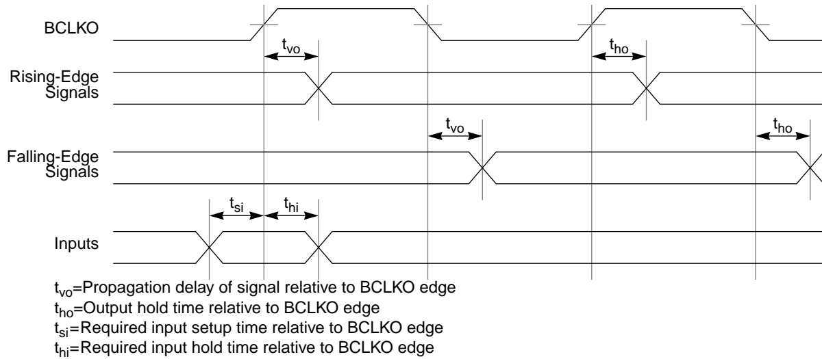
Figure 18-1. Signal Relationship to BCLKO for Non-DRAM Access
