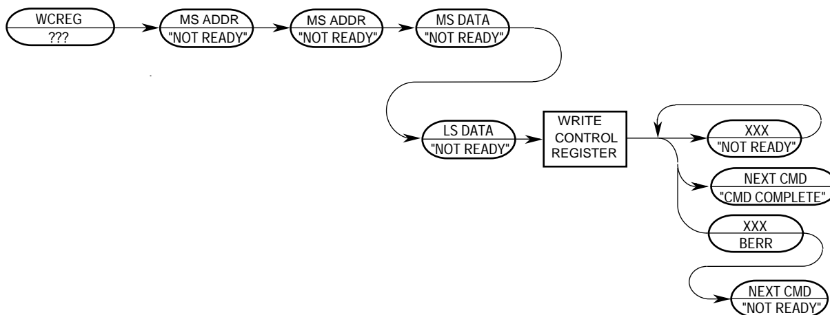
Figure 5-39. WCREG Command Sequence
