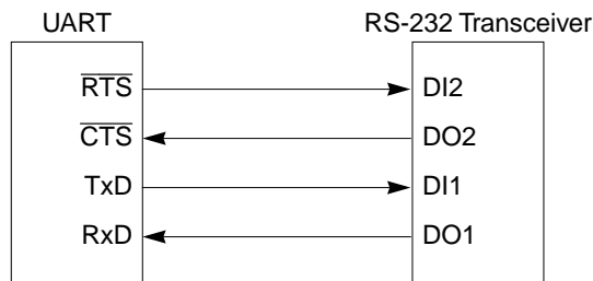
Figure 14-18. UART/RS-232 Interface
