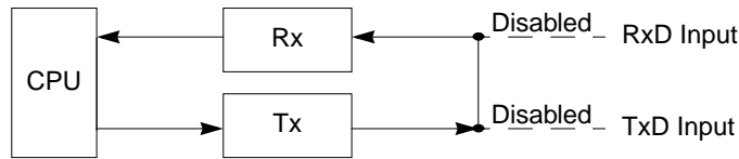
Figure 14-24. Local Loop-Back
