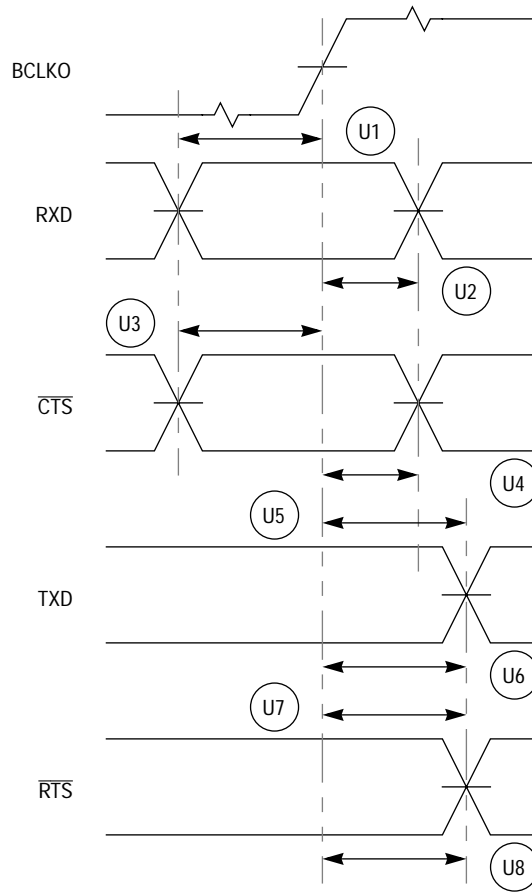
Figure 20-16. UART0/1 Module AC Timing—UART Mode
