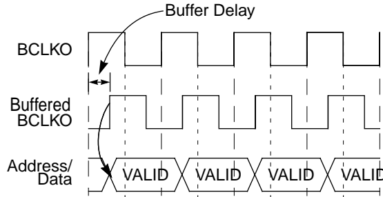
Figure 11-14. Using EDGESEL to Change Signal Timing
