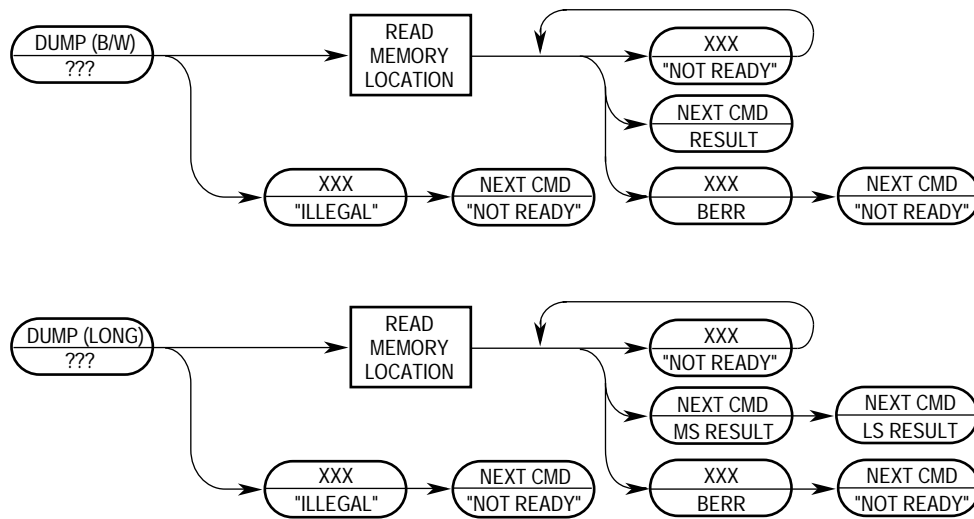
Figure 5-27. DUMP Command Sequence
