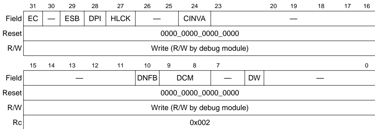
Figure 4-8. Cache Control Register (CACR)
