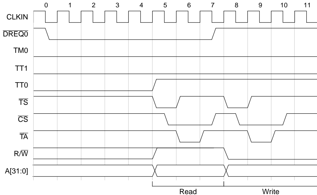
Figure 12-11. \overline{DREQ} Timing Constraints, Dual-Address DMA Transfer
