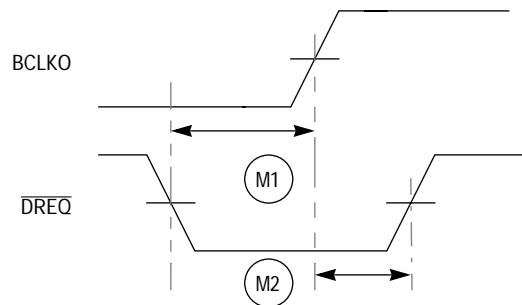
Figure 20-18. DMA Timing
