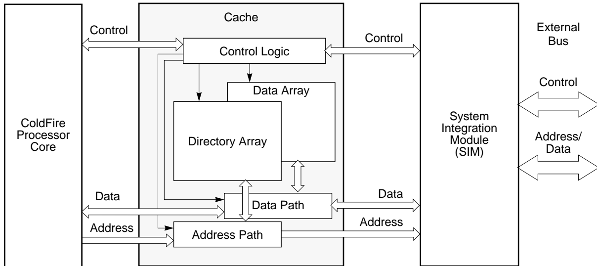
Figure 4-2. Unified Cache Organization
