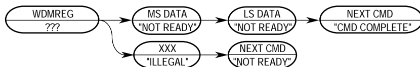
Figure 5-43. WDMREG Command Sequence
