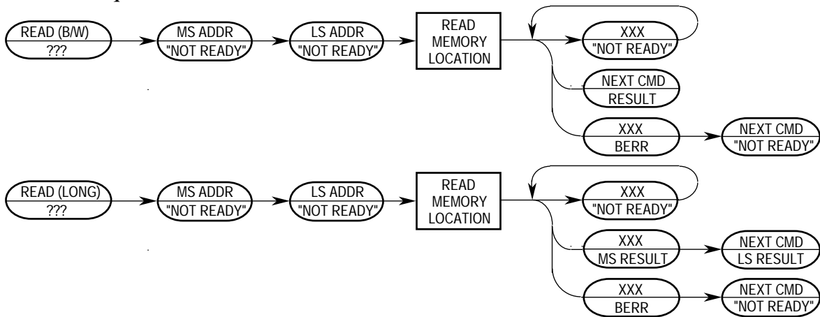
Figure 5-23. READ Command Sequence
