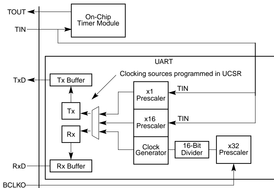
Figure 14-19. Clocking Source Diagram
