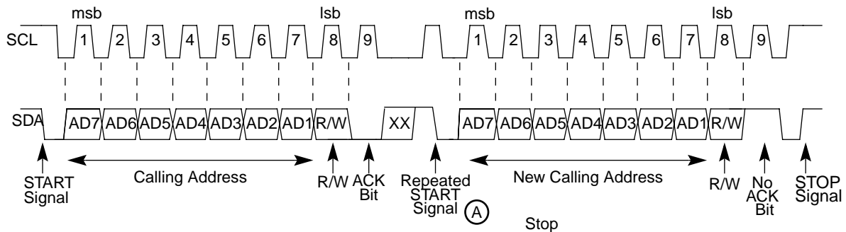
Figure 8-3. Repeated START
