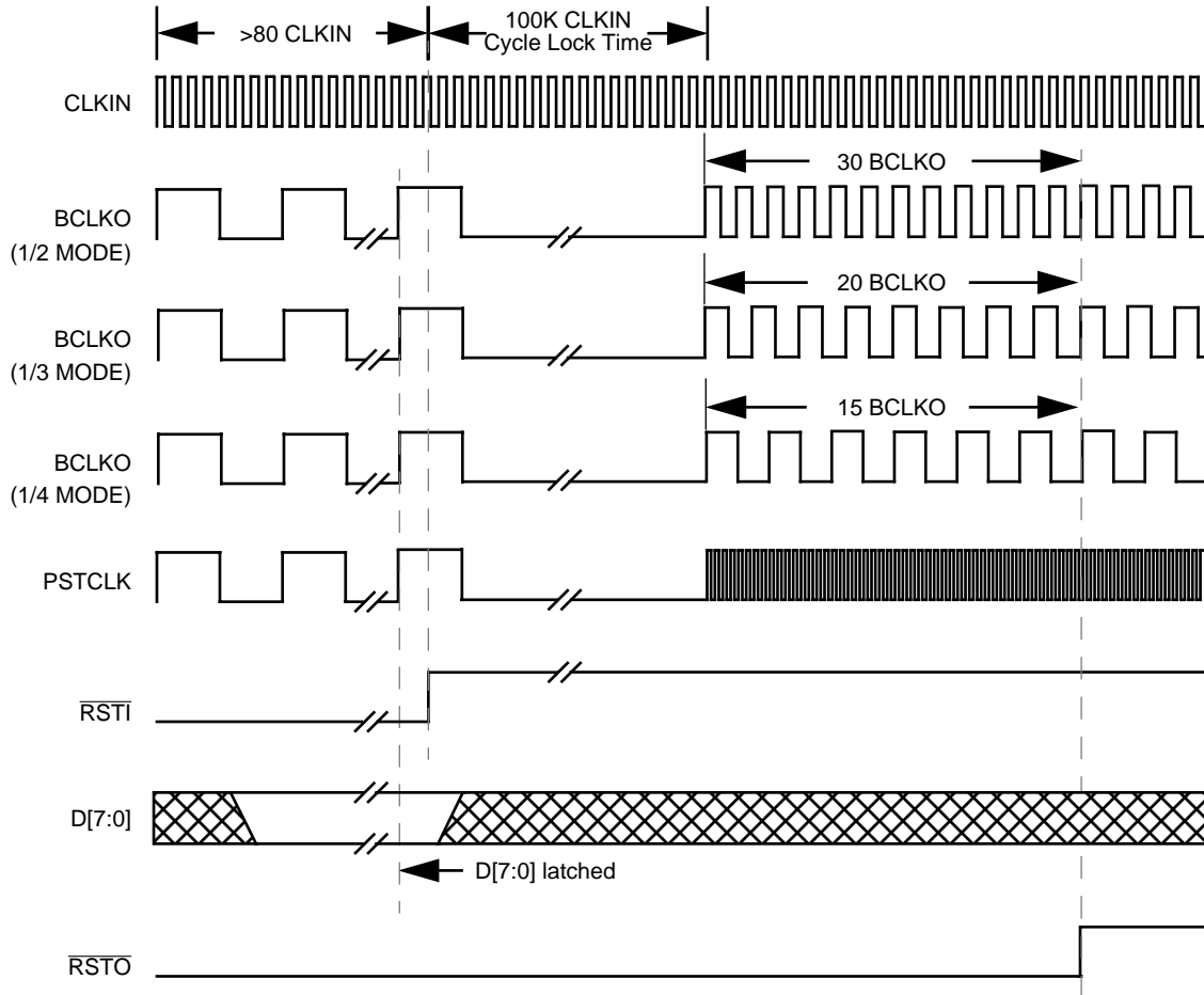
Figure 18-34. Software Watchdog Reset Timing
