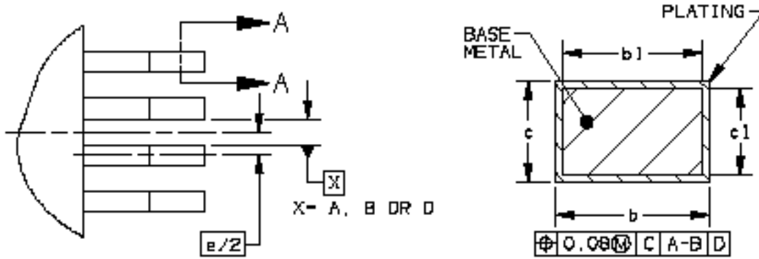
View A: Three Places
