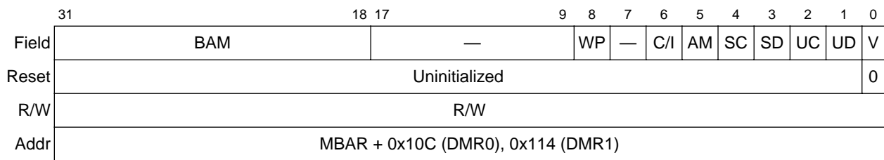
Figure 11-4. DRAM Controller Mask Registers (DMR0 and DMR1)
