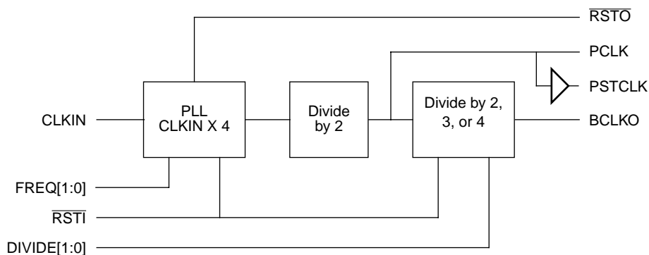
Figure 7-1. PLL Module Block Diagram
