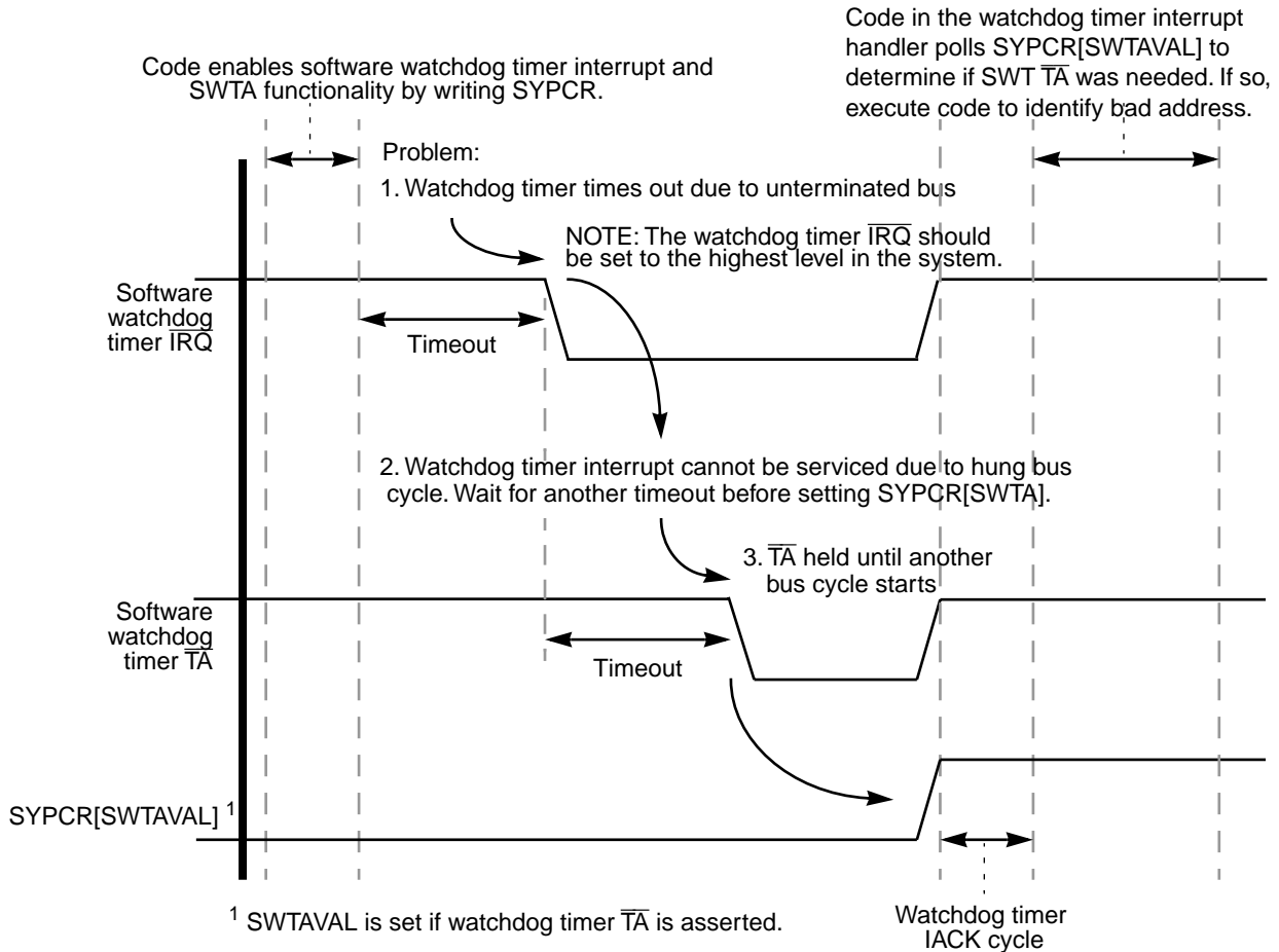
Figure 6-4. MCF5307 Embedded System Recovery from Unterminated Access
