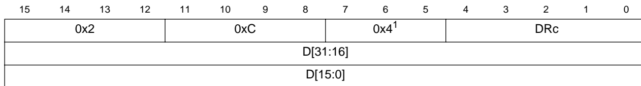
Figure 5-42. WDMREG BDM Command Format
