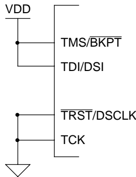
Figure 19-4. Disabling JTAG in JTAG Mode
