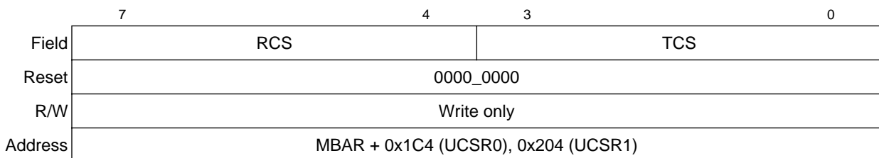
Figure 14-5. UART Clock-Select Register (UCSR n )
