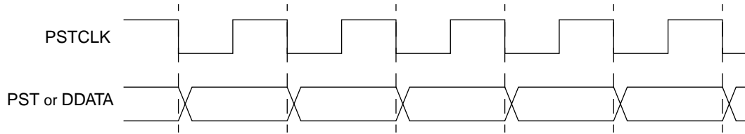
Figure 5-2. PSTCLK Timing
