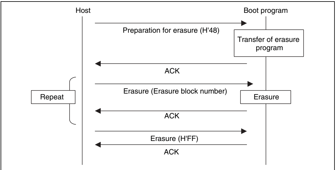
Figure 14.26 Erasure Sequence
