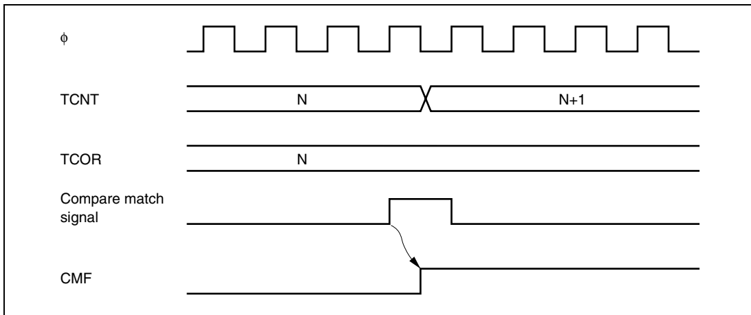
Figure 9.5 Timing of CMF Setting
