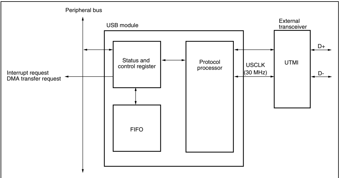
Figure 12.1 Block Diagram of USB2
