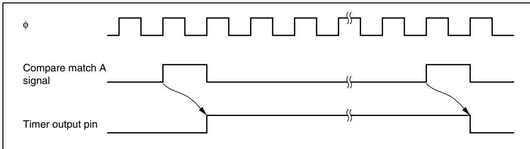
Figure 9.6 Timing of Timer Output
