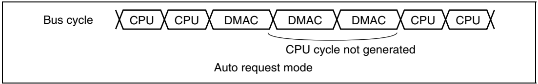
Figure 7.6 Examples of Timing in Burst Mode
