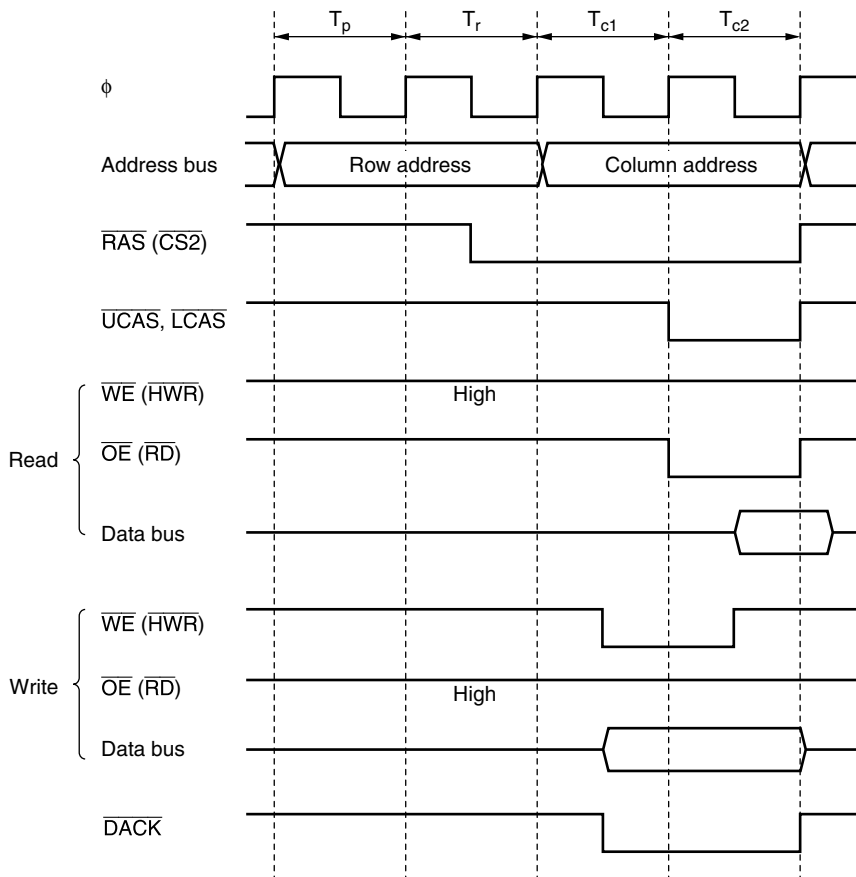
Figure 6.42 Example of \overline{\text{DACK}} Output Timing when \text{DDS} = 1 ( \text{RAST} = 0 , \text{CAST} = 0 )
