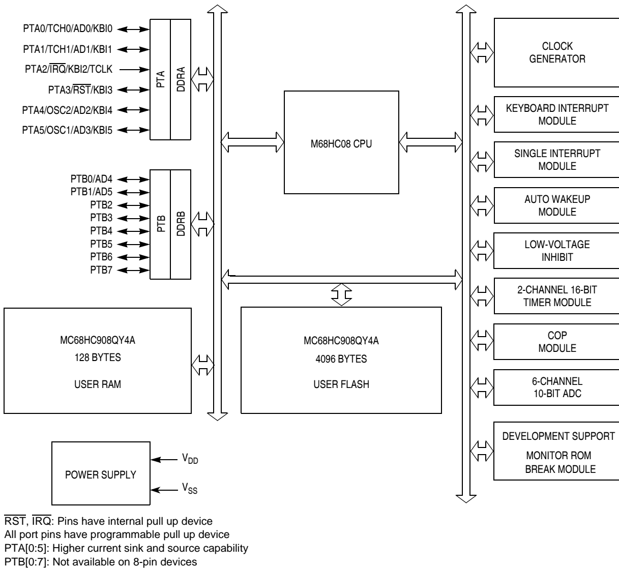
Figure 1-1. Block Diagram
