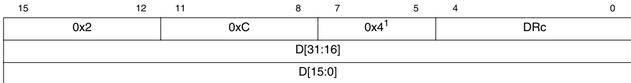
Figure 5-44. WDMREG BDM Command Format
