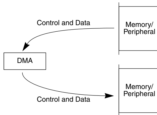
Figure 12-3. Dual-Address Transfer
