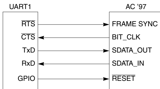
Figure 14-27. UART1/AC '97 Interface
