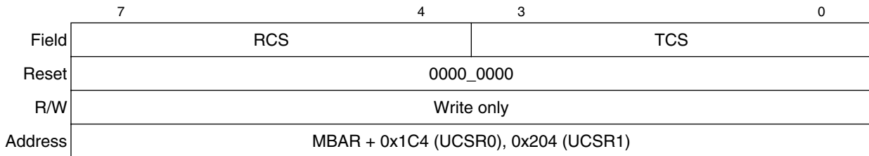
Figure 14-8. UART Clock-Select Register (UCSRn)
