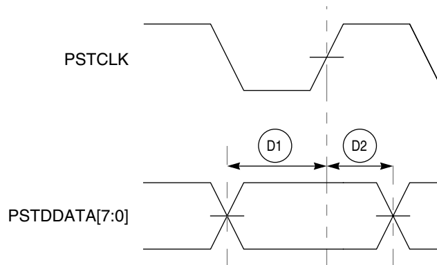
Figure 20-15. Real-Time Trace AC Timing
