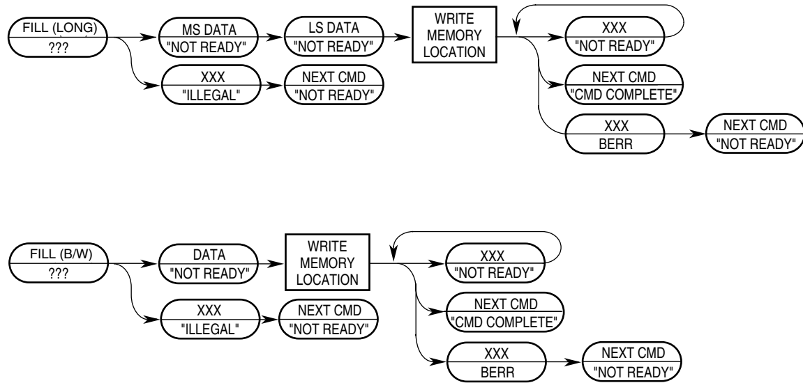
Figure 5-31. FILL Command Sequence
