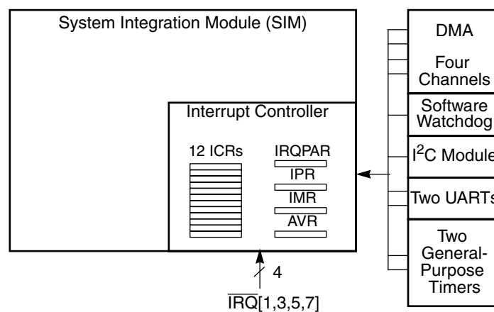
Figure 9-1. Interrupt Controller Block Diagram
