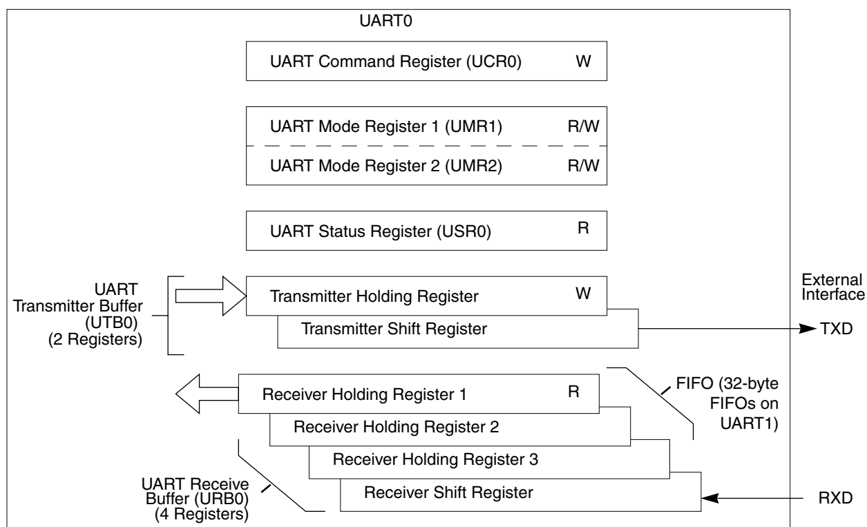
Figure 14-29. Transmitter and Receiver Functional Diagram
