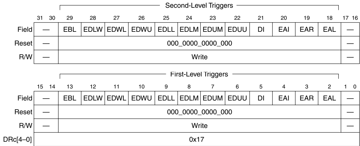
Figure 5-14. Extended Trigger Definition Register (XTDR)
