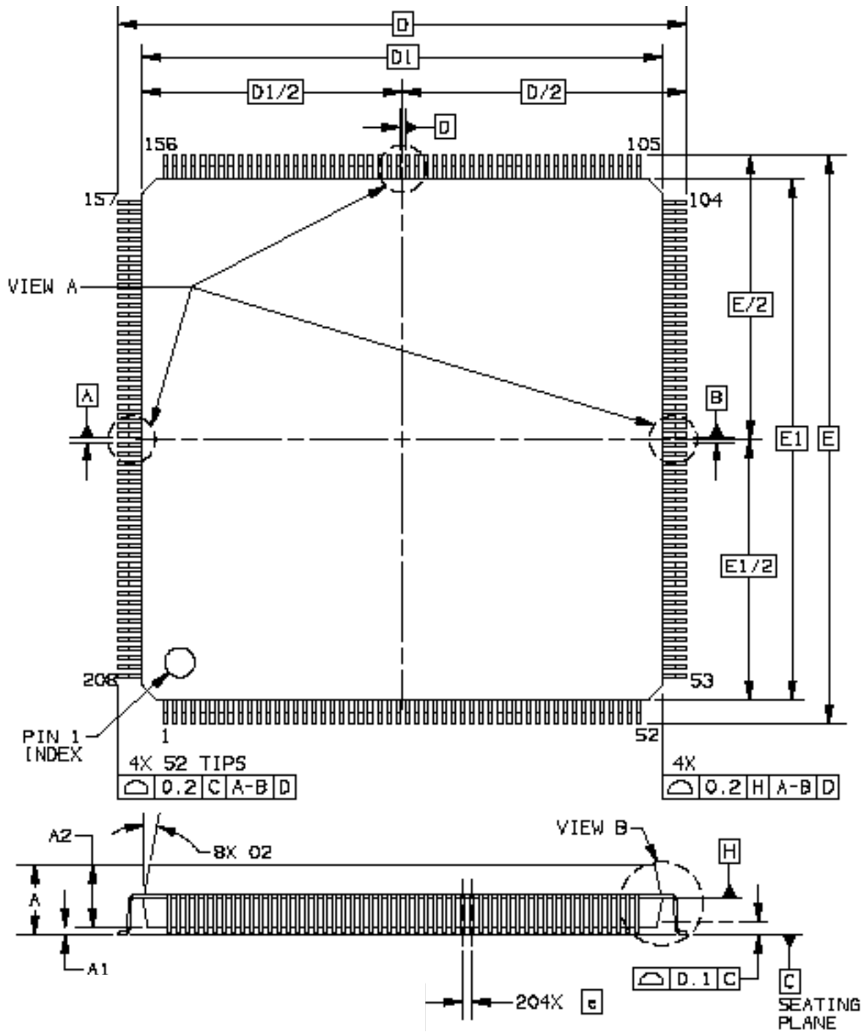
Figure 16-2. MCF5407 Case Drawing (General View)
