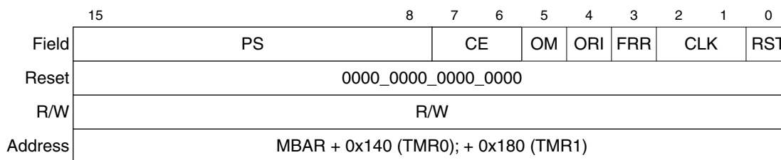
Figure 13-2. Timer Mode Registers (TMR0/TMR1)
