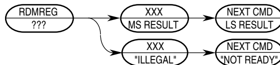
Figure 5-43. RDMREG Command Sequence
