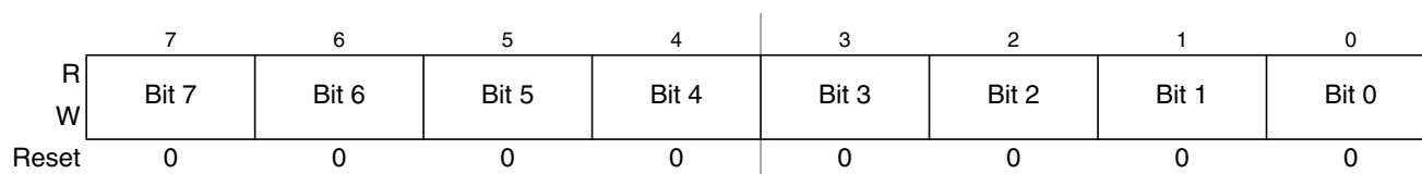
Figure 14-35. Timer Input Capture/Output Compare Register 7 Low (TC7)
