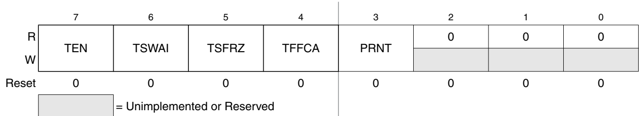
Figure 22-12. Timer System Control Register 1 (TSCR1)
