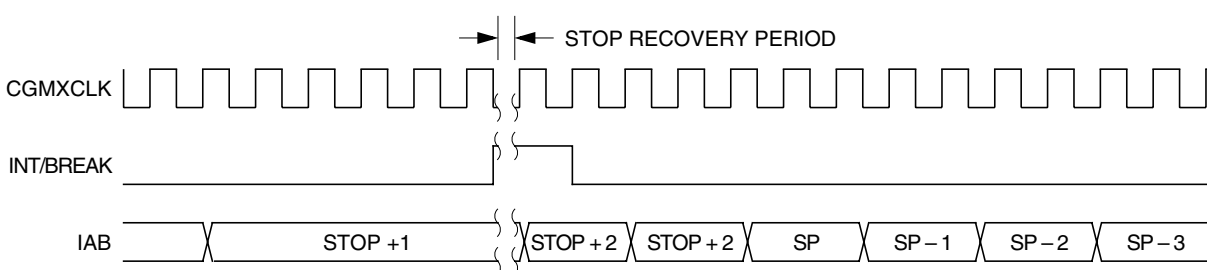
Figure 14-19. Stop Mode Recovery from Interrupt or Break
