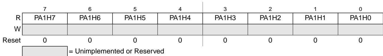
Figure 7-53. 8-Bit Pulse Accumulators Holding Register 1 (PA1H)
