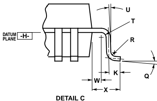
Figure B-3. 80-Pin QFP Mechanical Dimensions (Case No. 841B)
