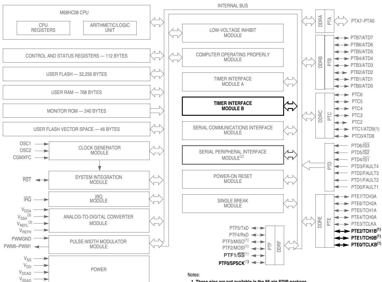
Figure 17-1. Block Diagram Highlighting TIMB Block and Pins
