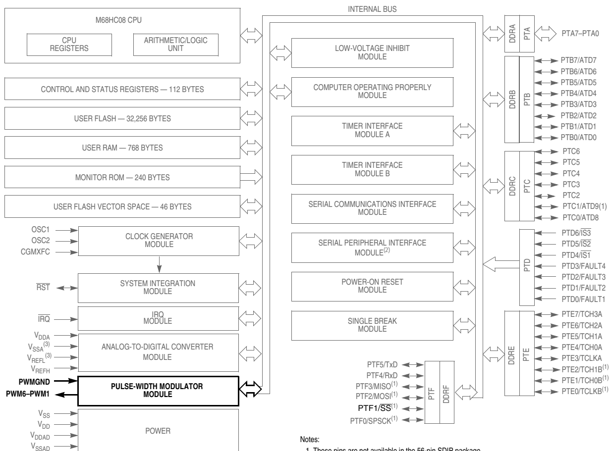
Figure 12-1. Block Diagram Highlighting PWMMC Block and Pins
