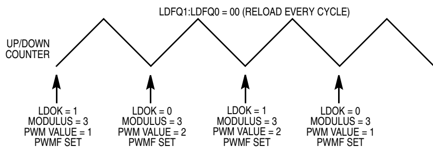
Figure 12-8. Center-Aligned PWM Value Loading
